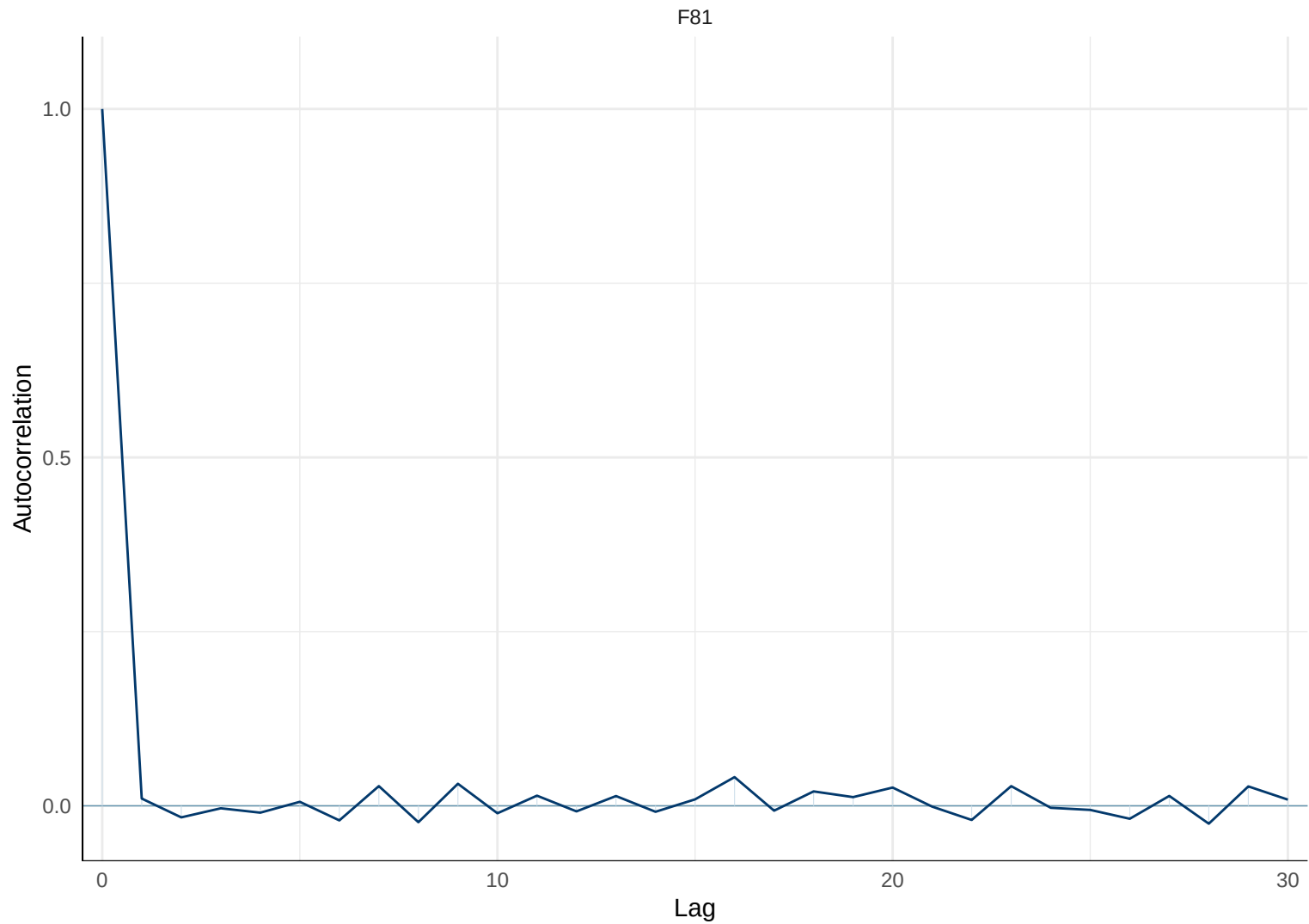
Autocorrelation: F81
