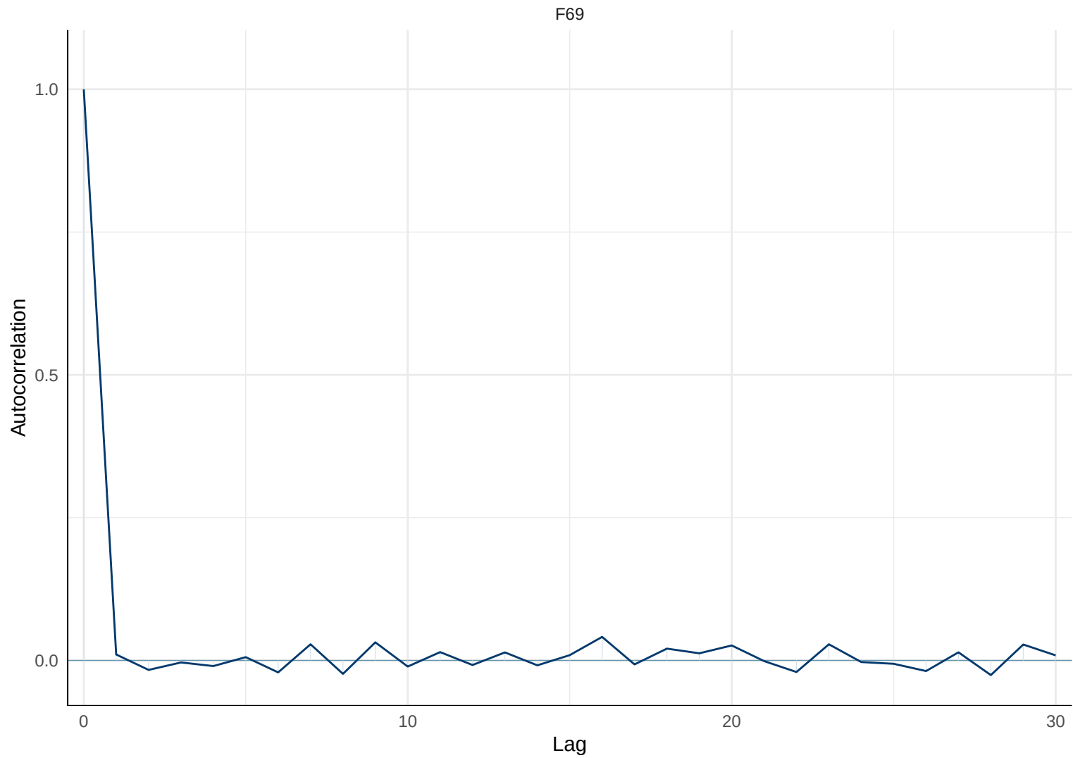
Autocorrelation: F69
