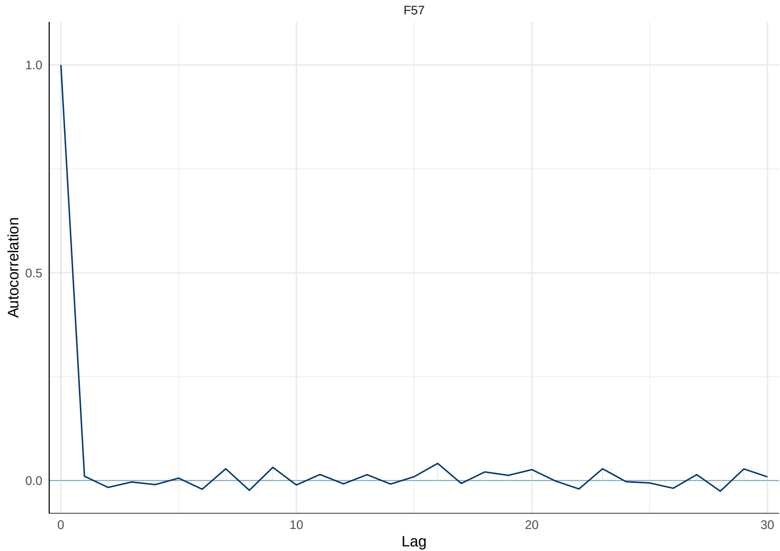
Autocorrelation: F57
