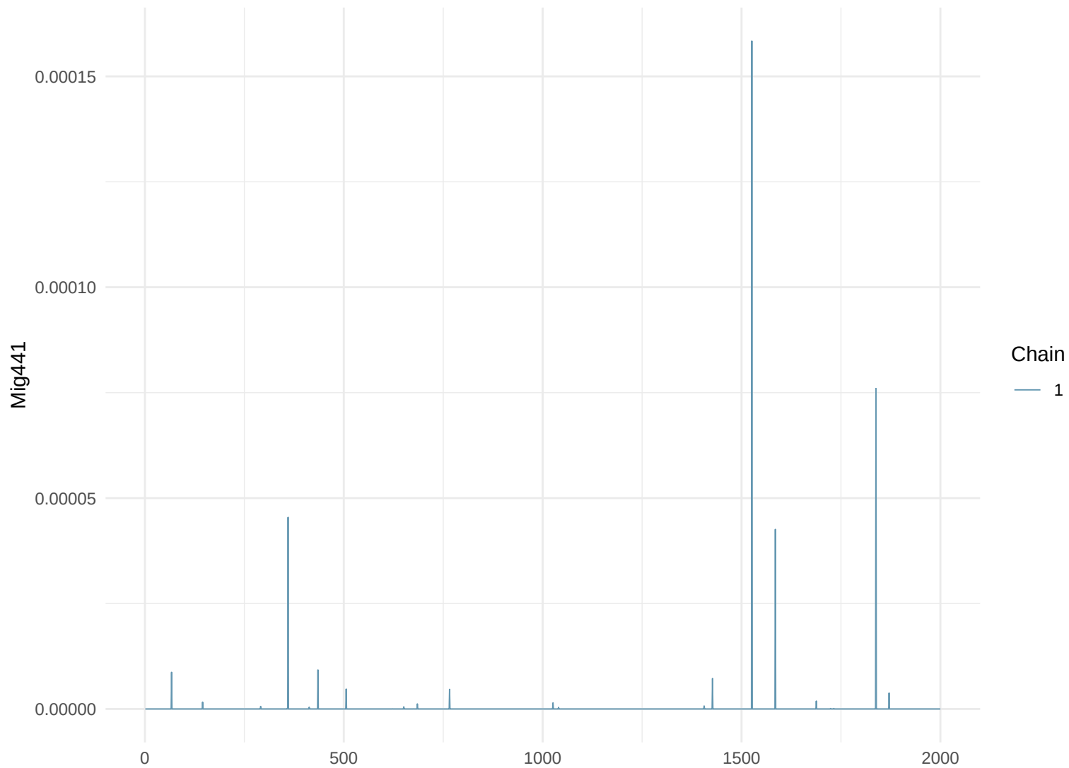
Trace Plot: Mig441
