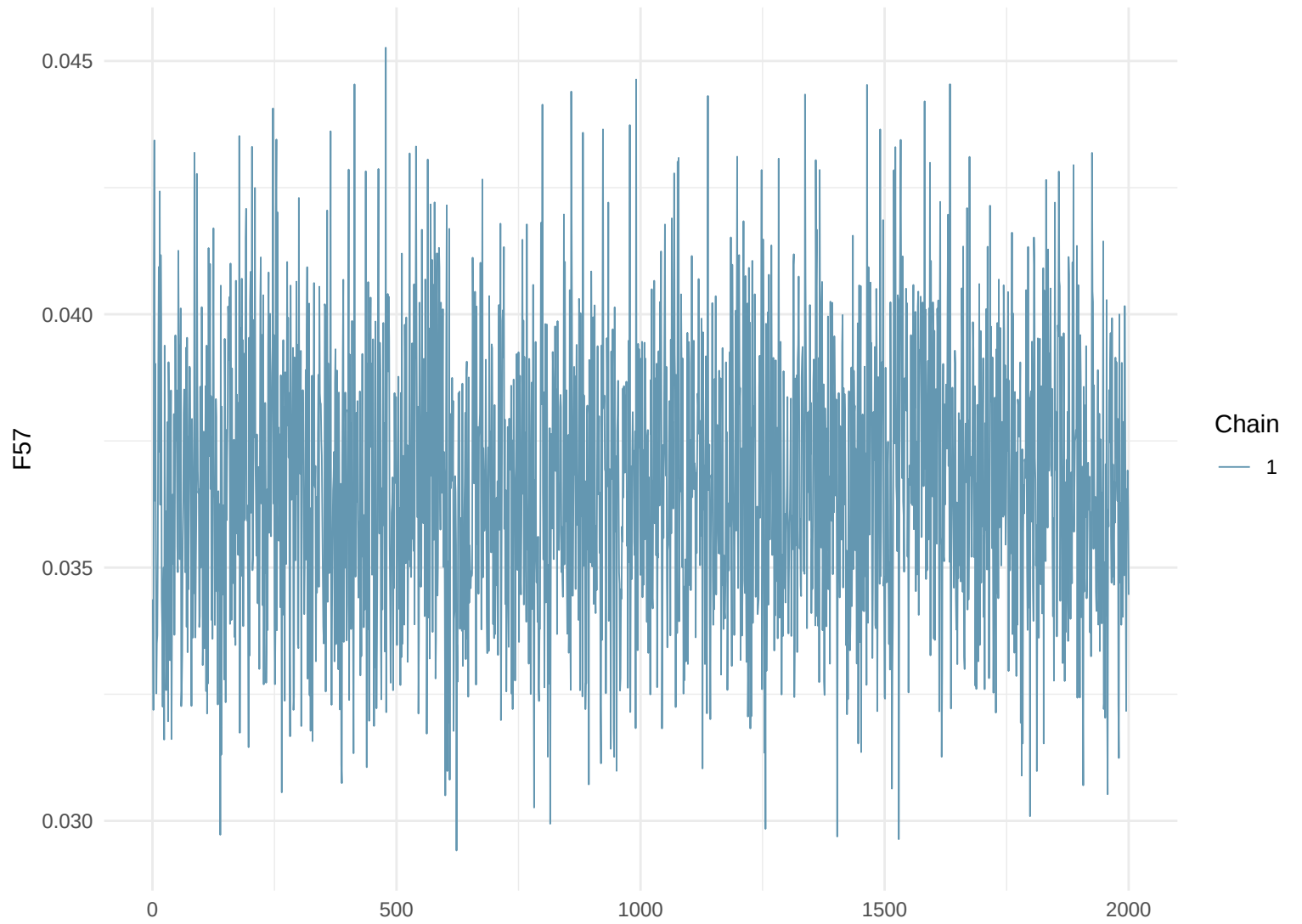
Trace Plot: F57
