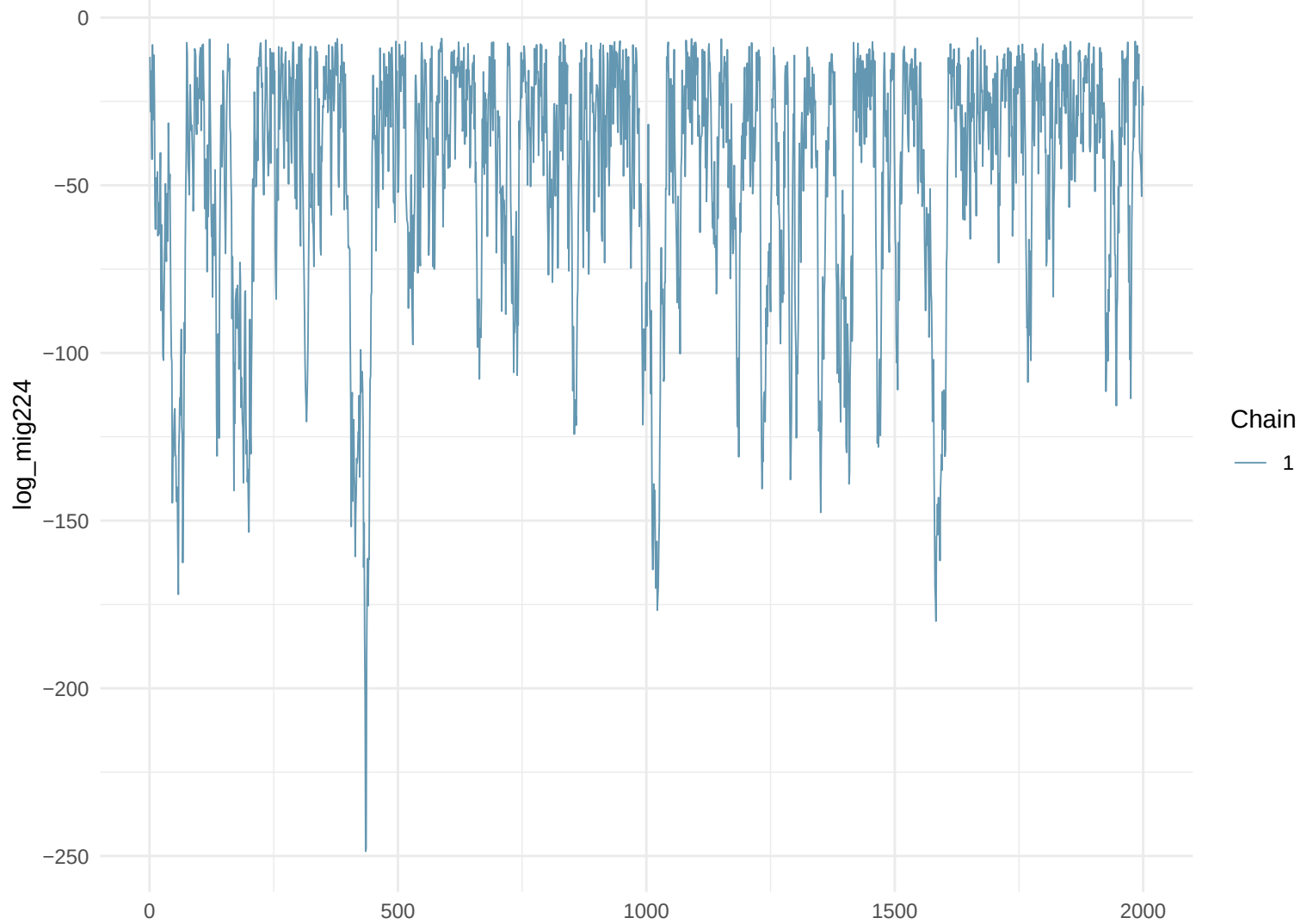
Trace Plot: log_mig224
