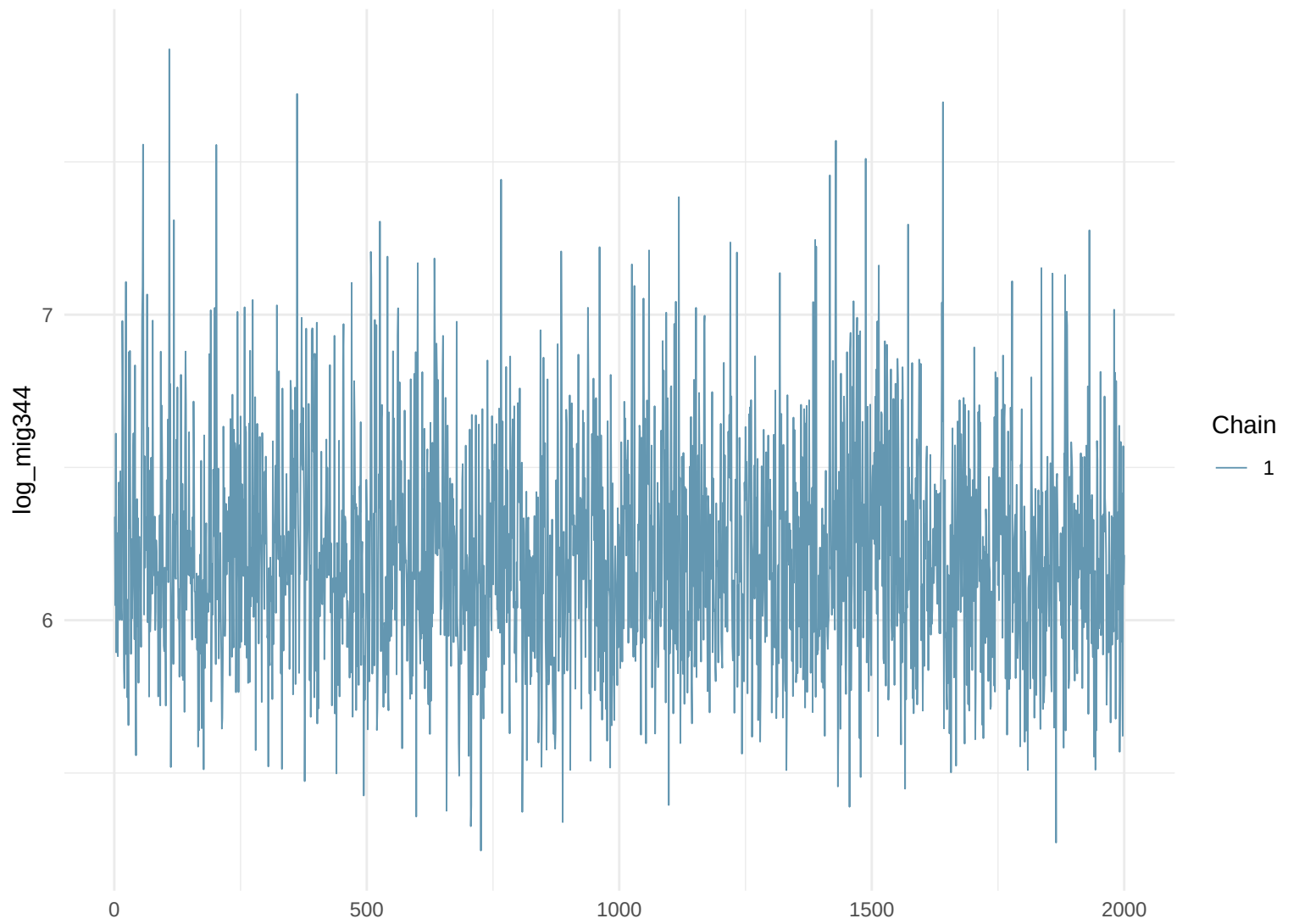
Trace Plot: log_mig344
