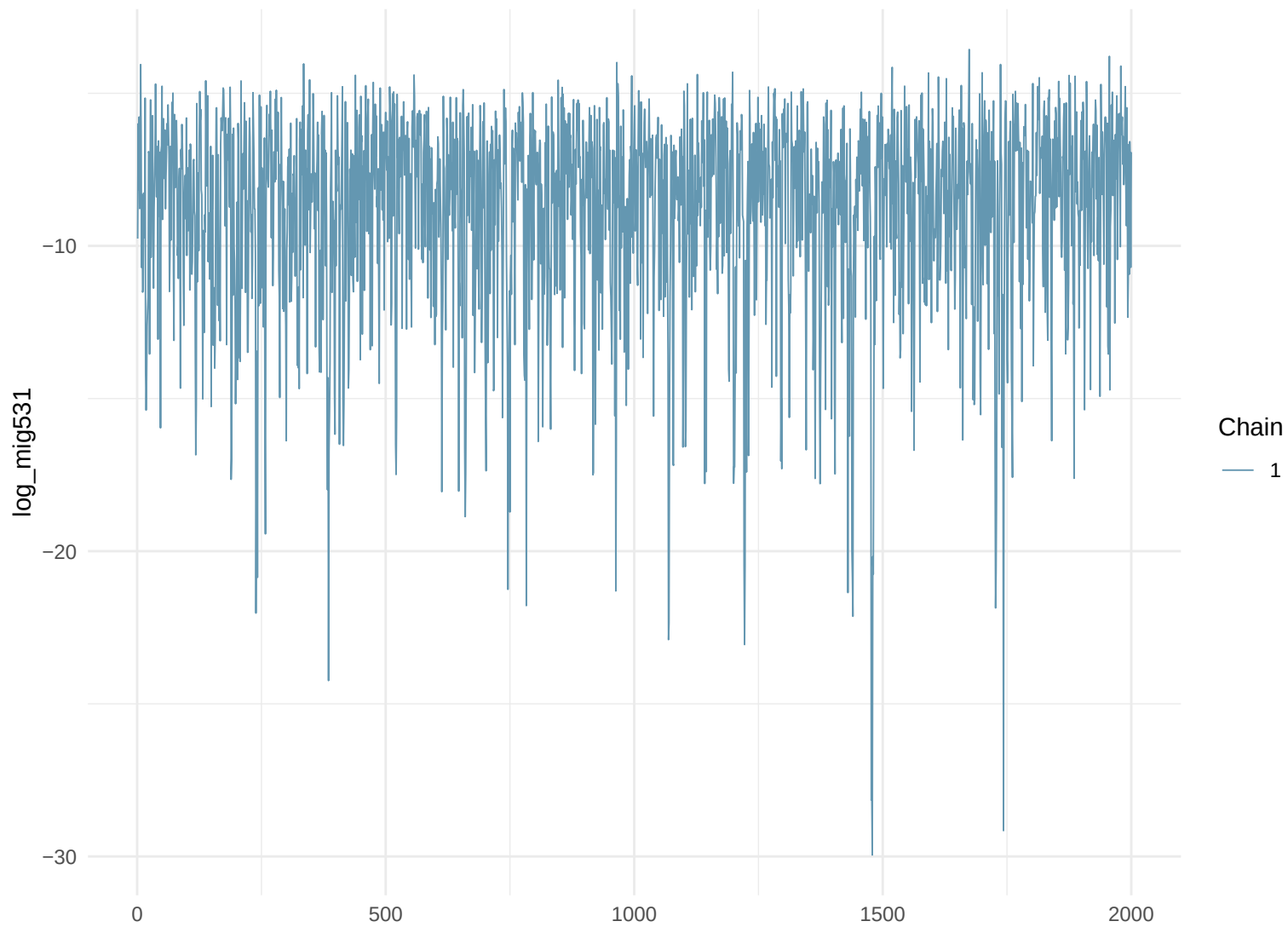
Trace Plot: log_mig531
