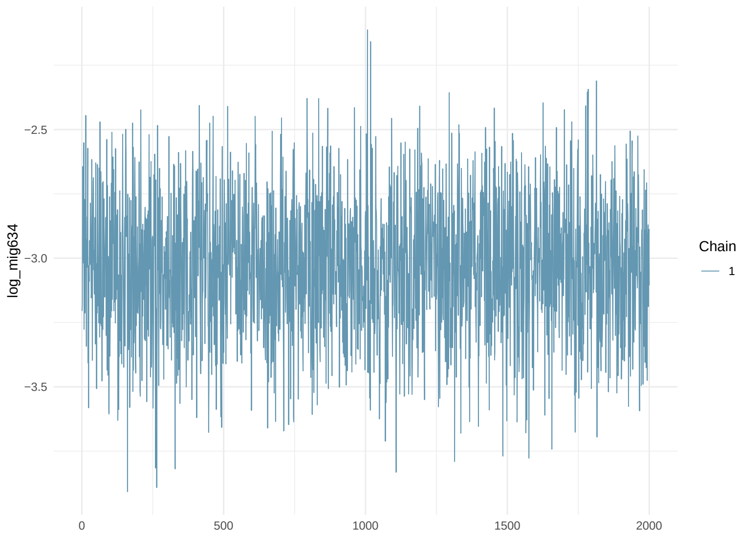
Trace Plot: log_mig634
