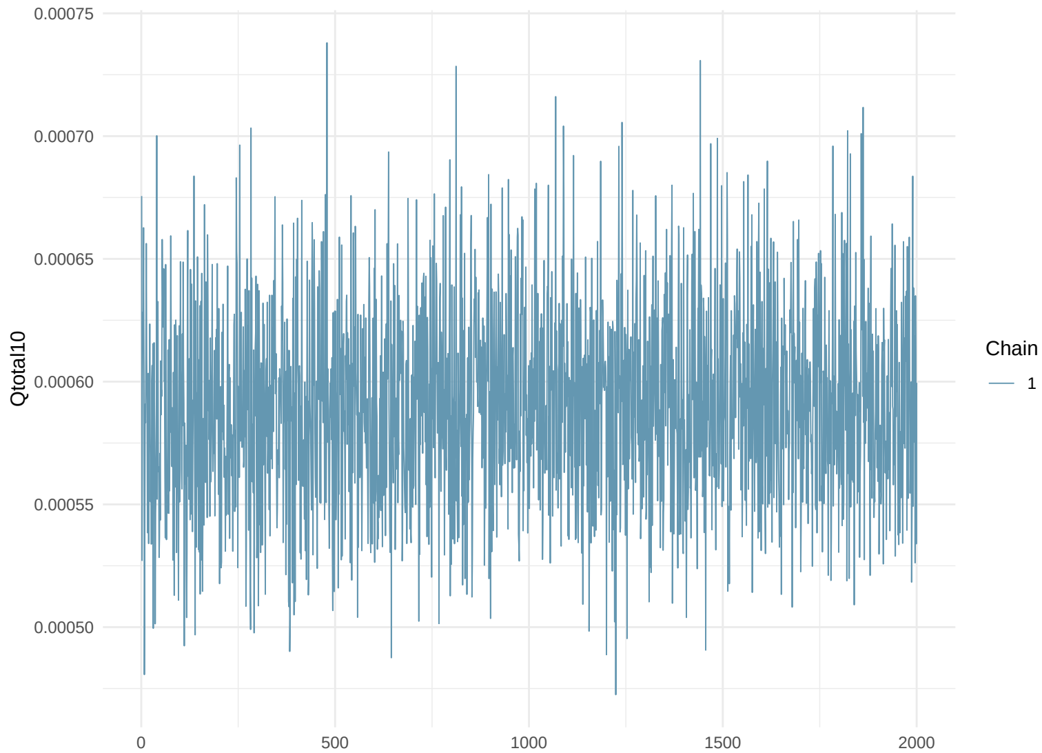
Trace Plot: Qtotal10
