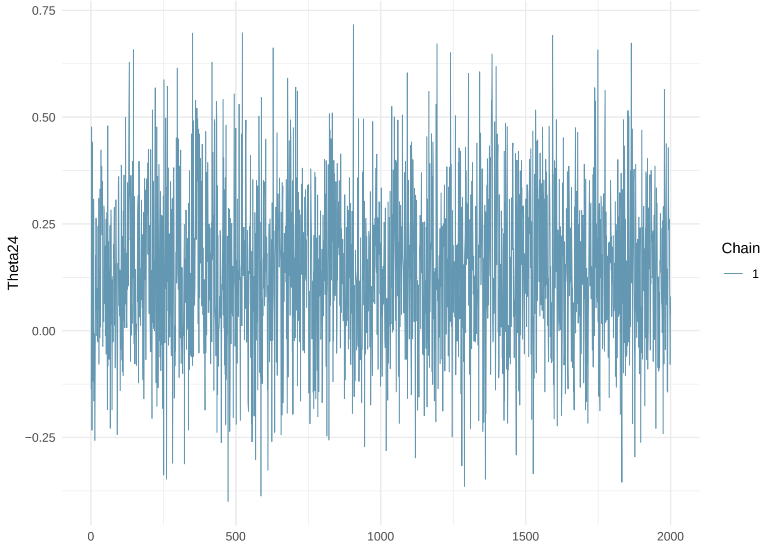
Trace Plot: Theta24
