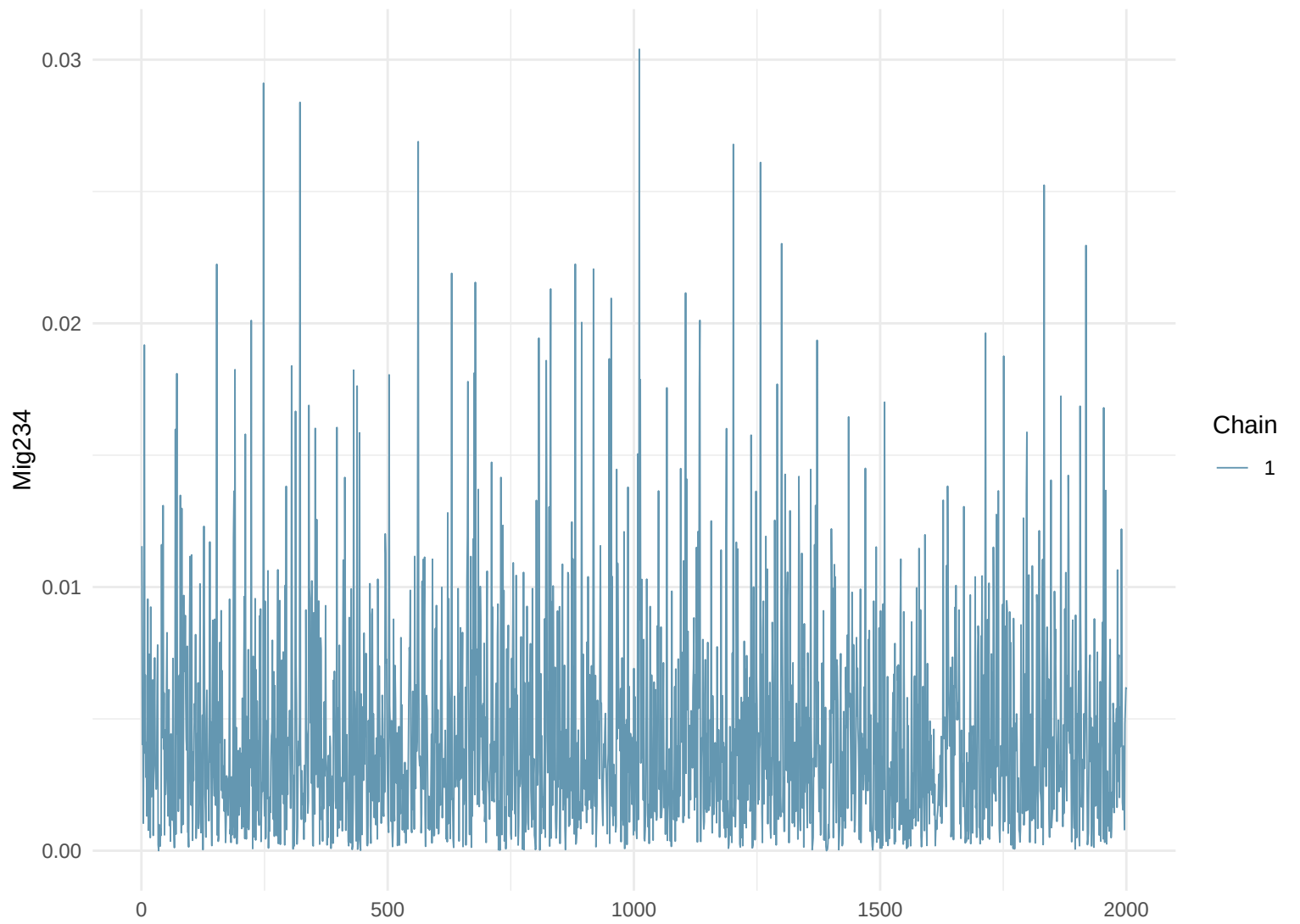
Trace Plot: Mig234
