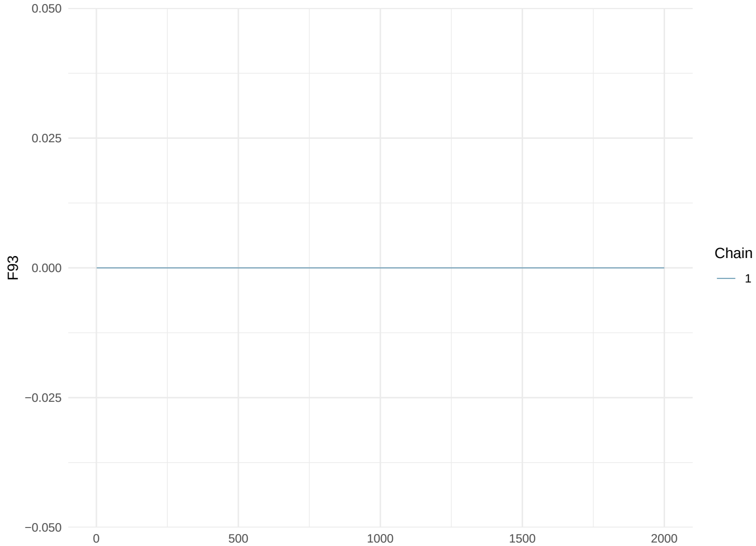
Trace Plot: F93
