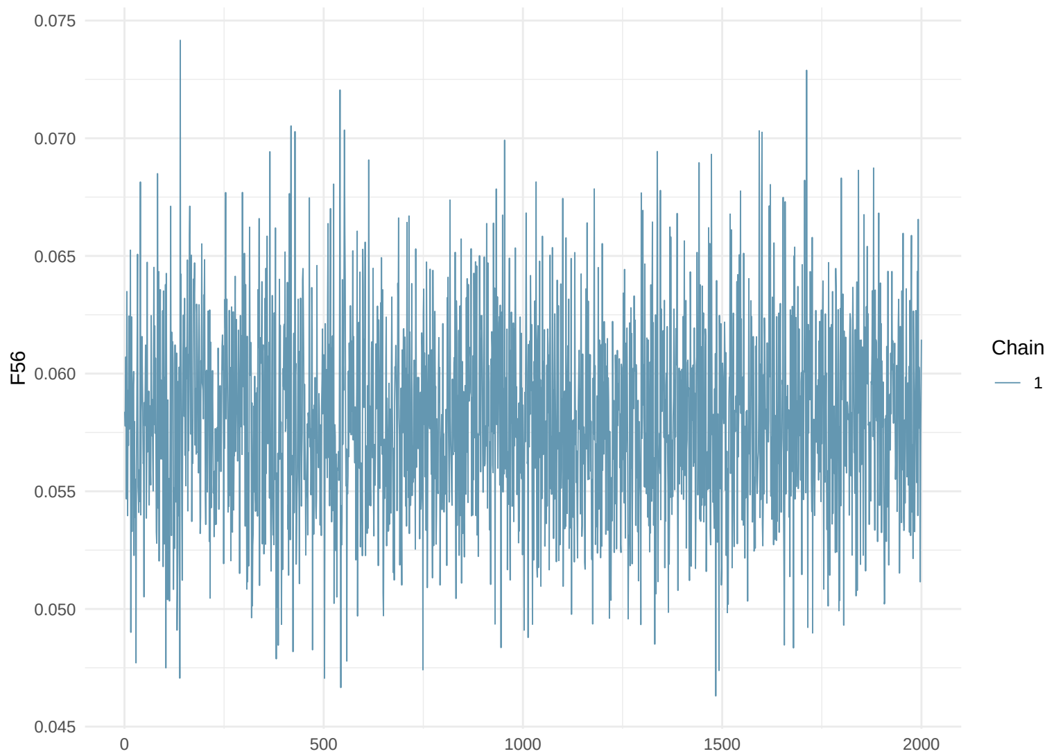
Trace Plot: F56
