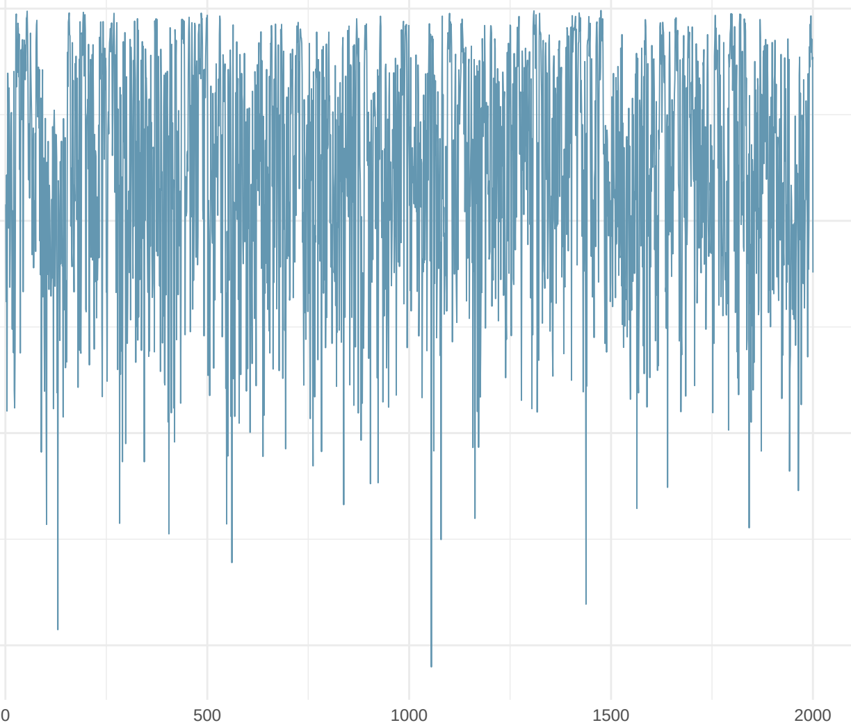
Trace Plot: Mig433
