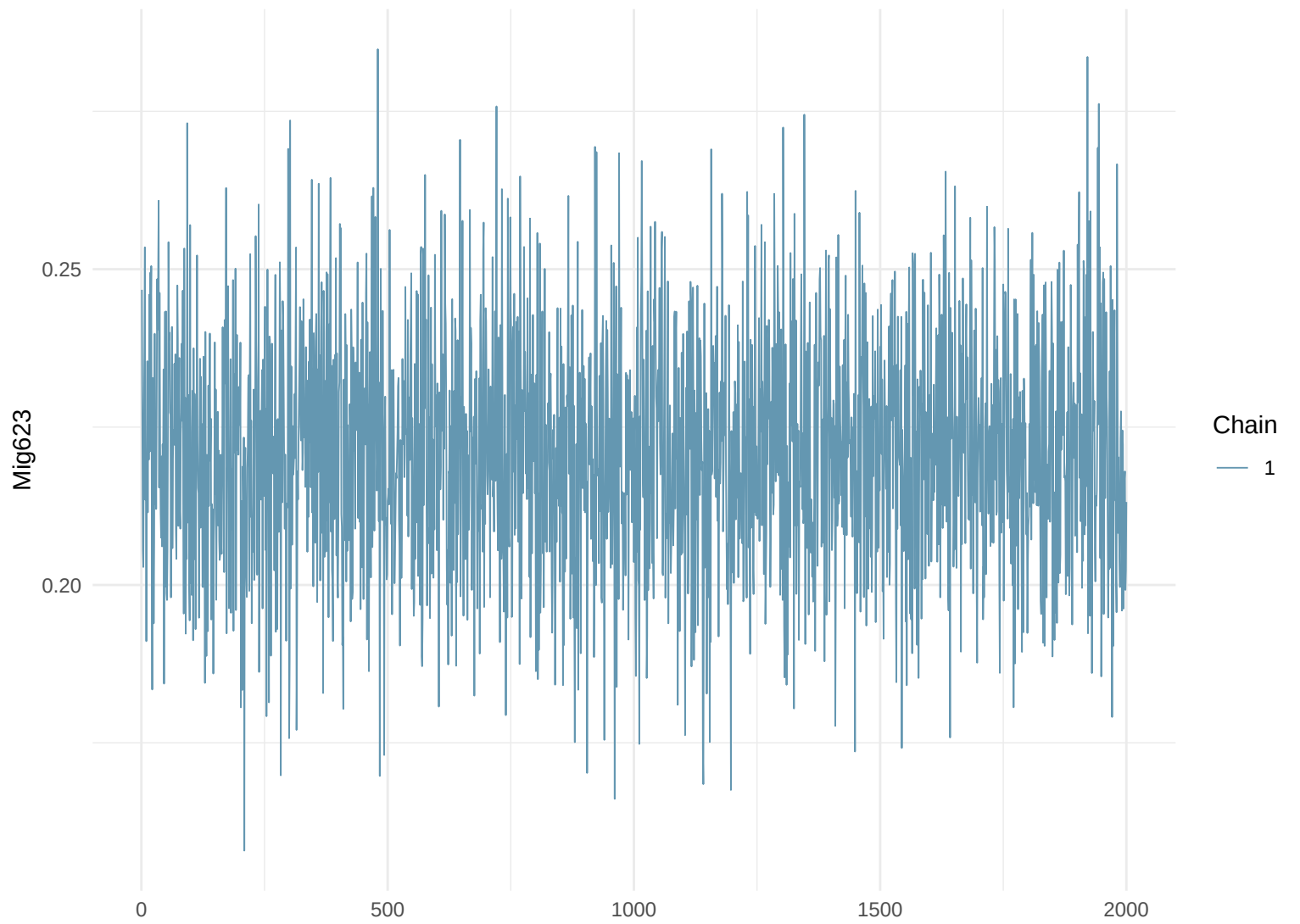
Trace Plot: Mig623
