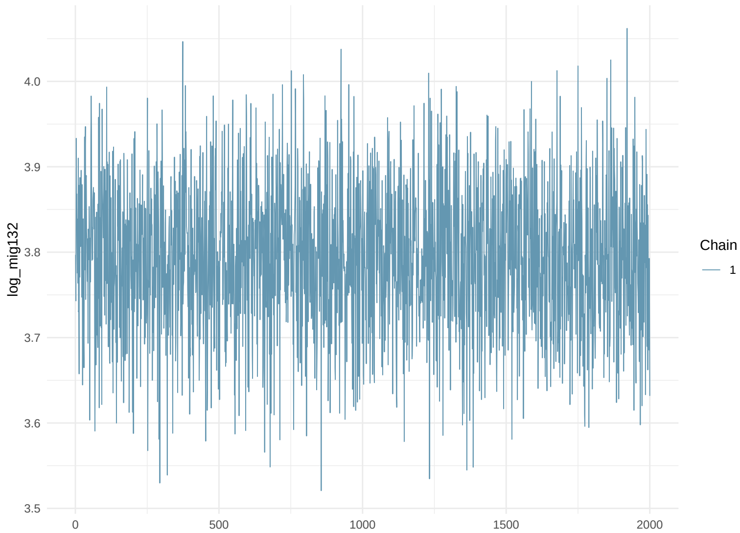
Trace Plot: log_mig132
