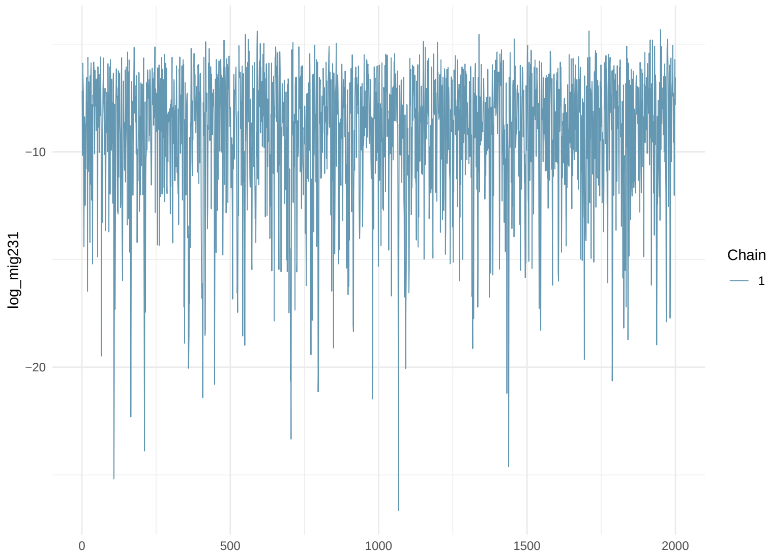
Trace Plot: log_mig231
