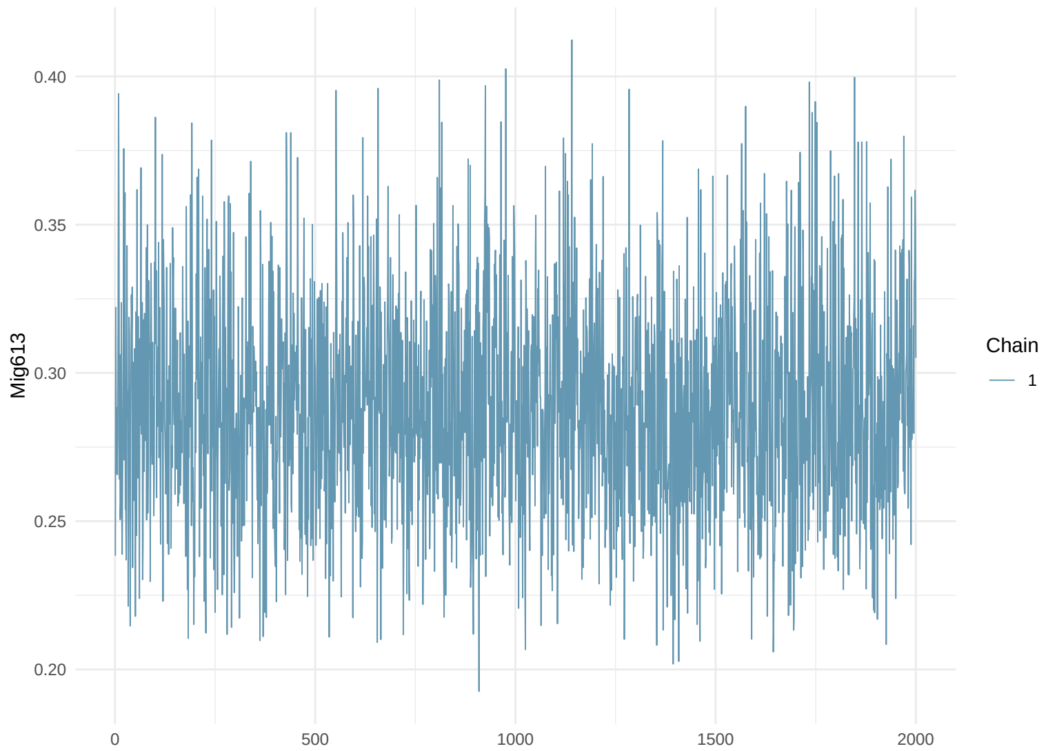
Trace Plot: Mig613
