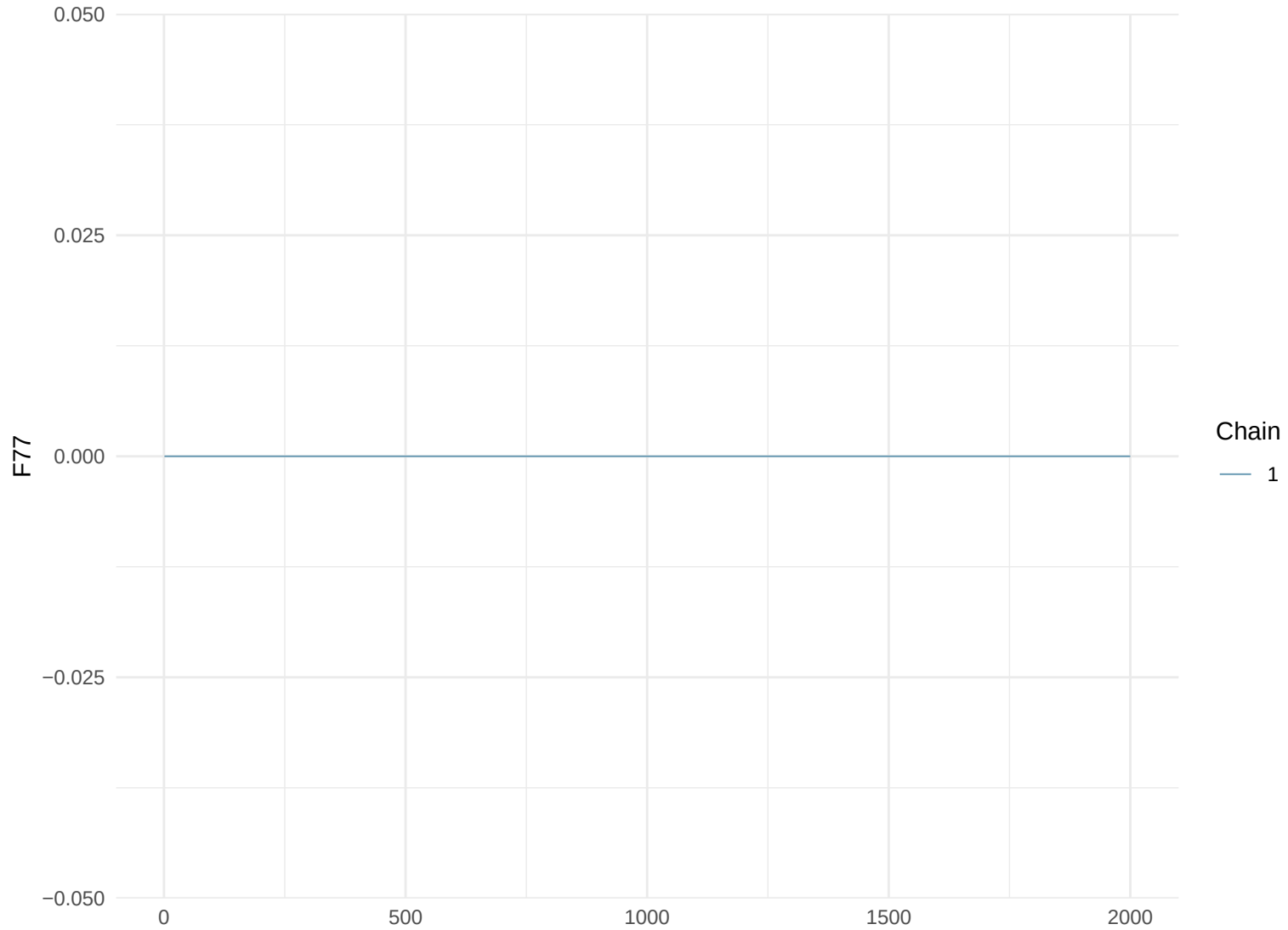
Trace Plot: F77
