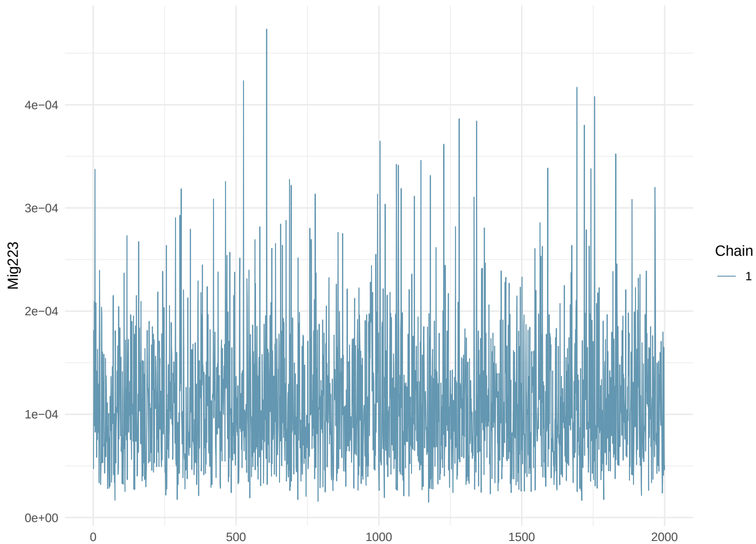
Trace Plot: Mig223
