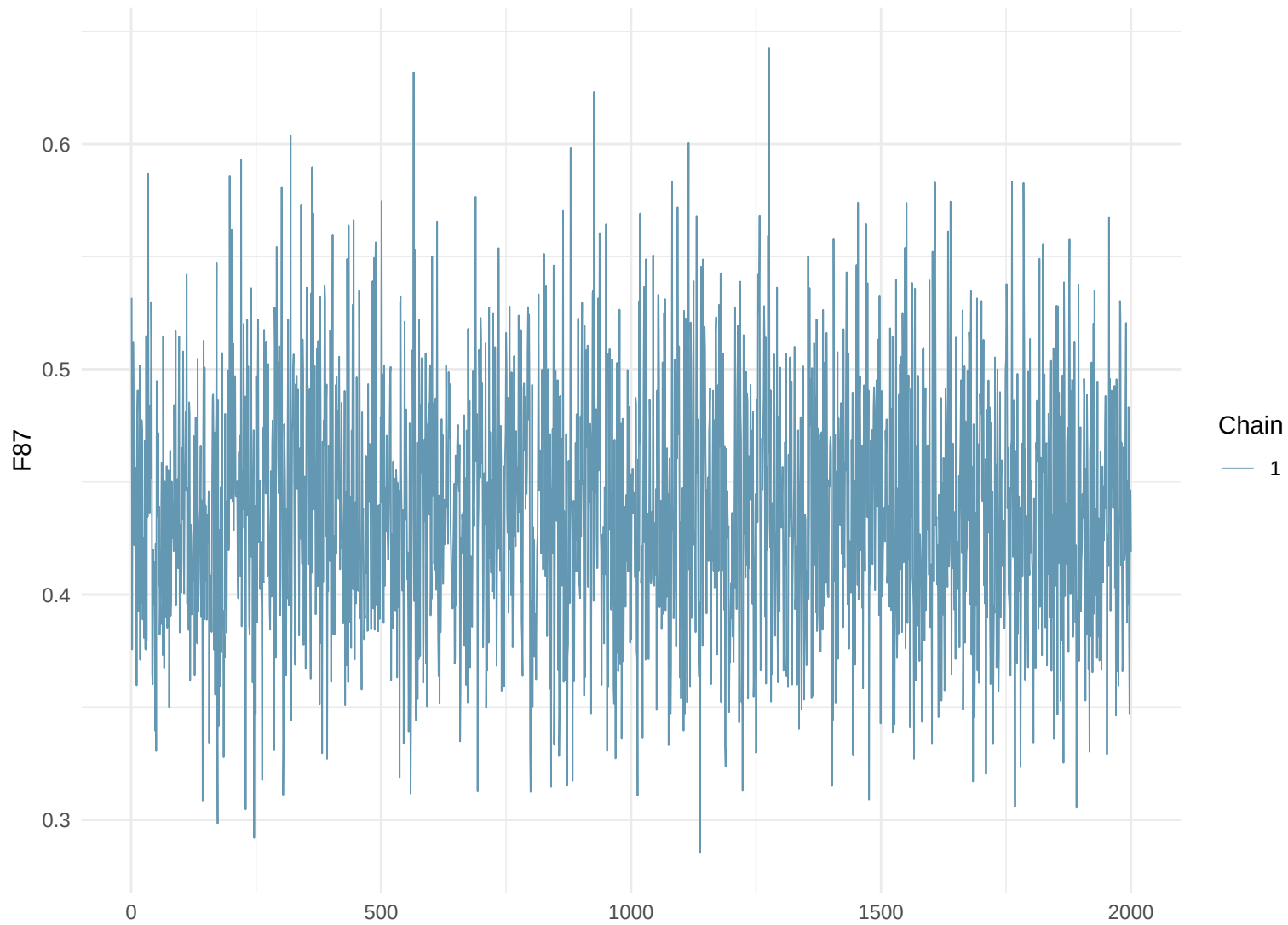
Trace Plot: F87
