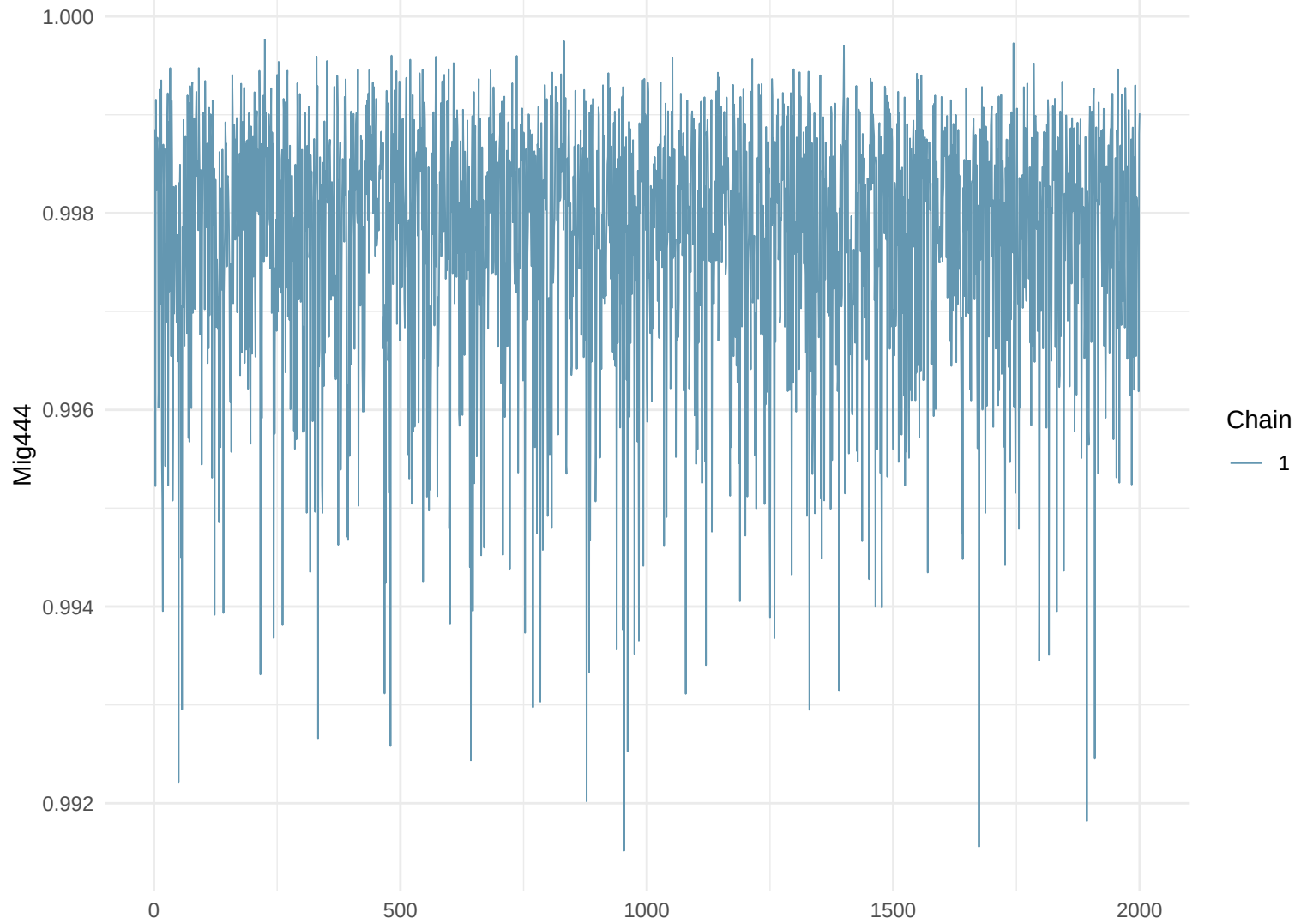
Trace Plot: Mig444
