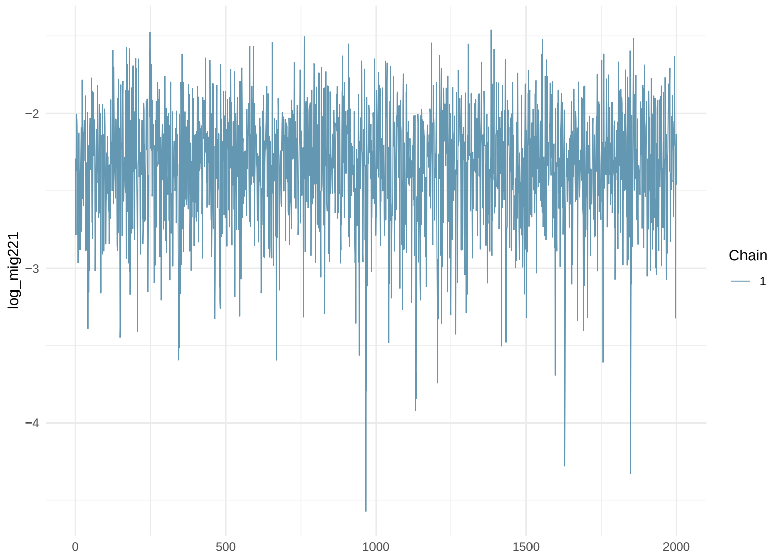
Trace Plot: log_mig221
