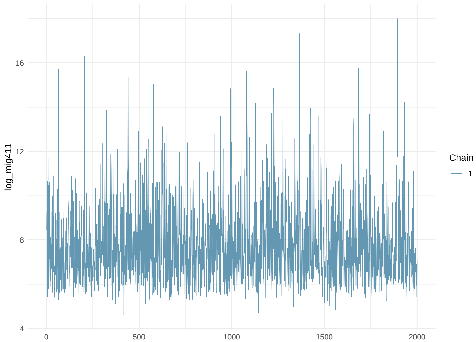
Trace Plot: log_mig411
