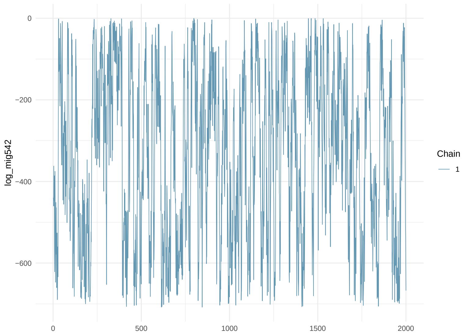
Trace Plot: log_mig542
