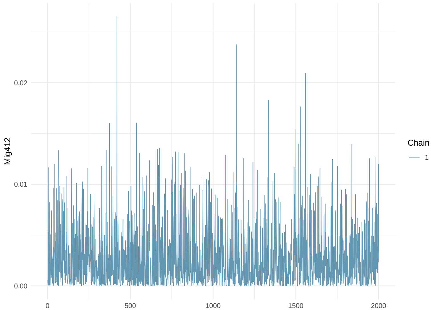
Trace Plot: Mig412
