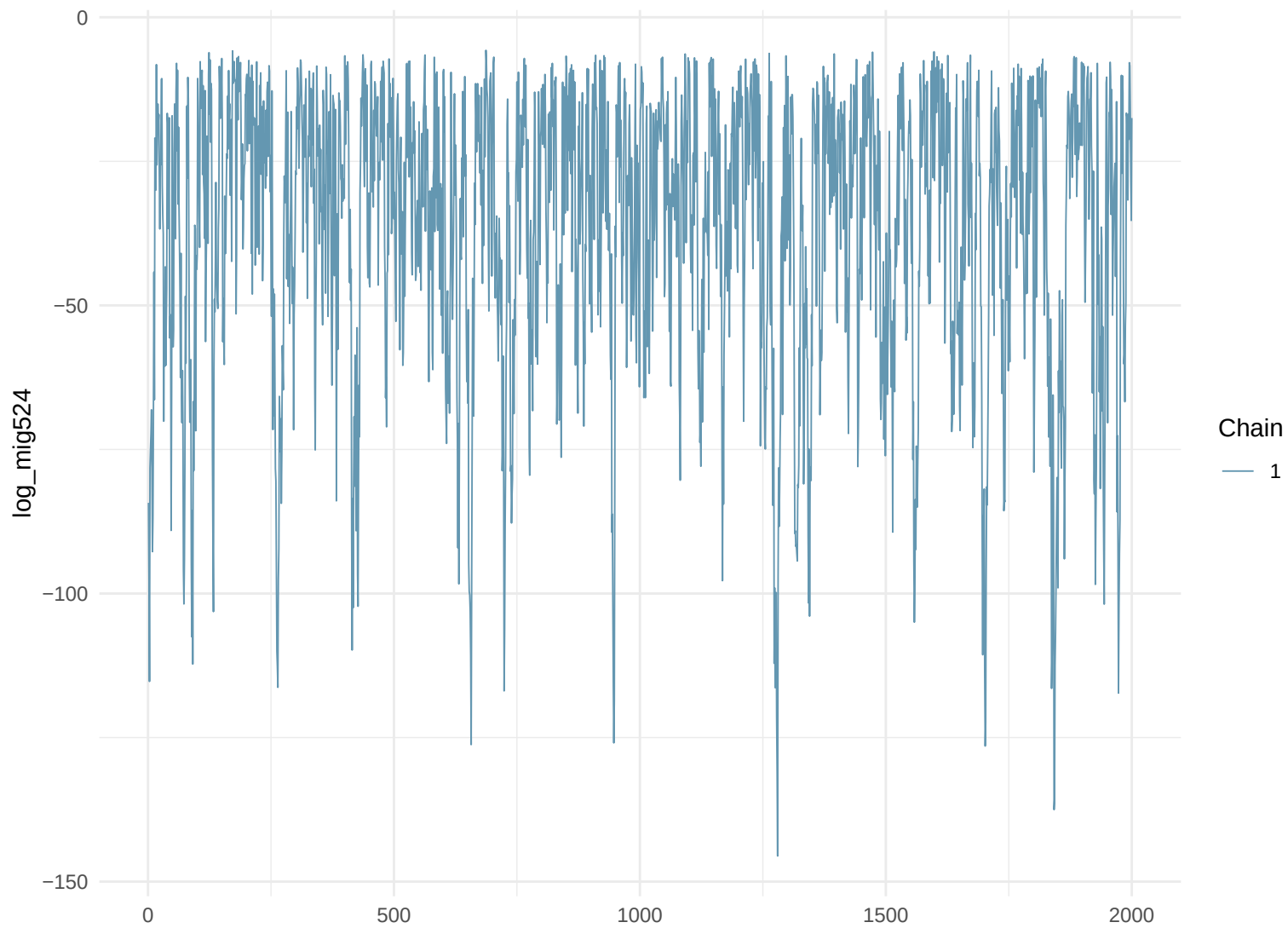
Trace Plot: log_mig524
