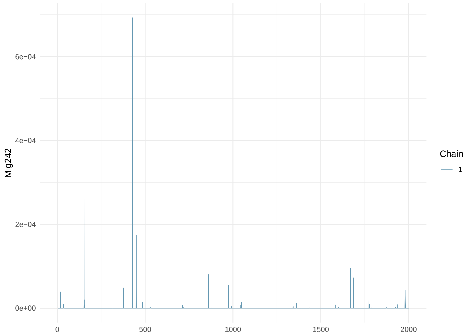
Trace Plot: Mig242
