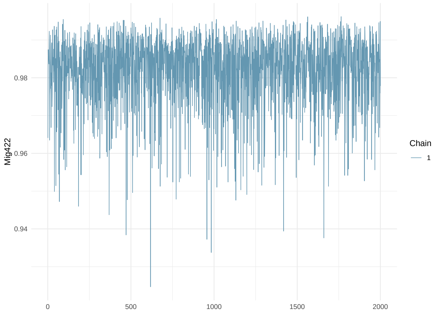
Trace Plot: Mig422
