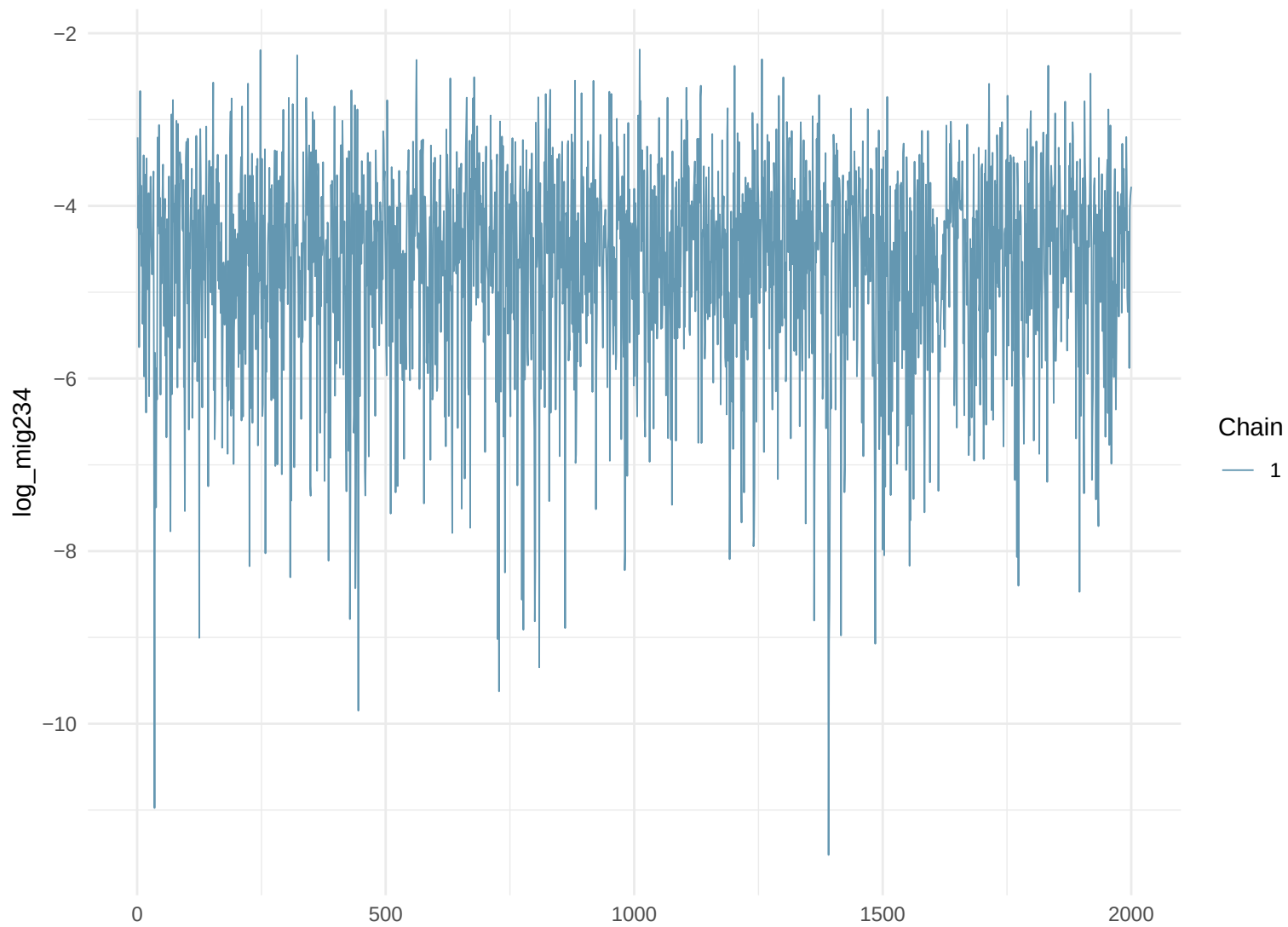
Trace Plot: log_mig234
