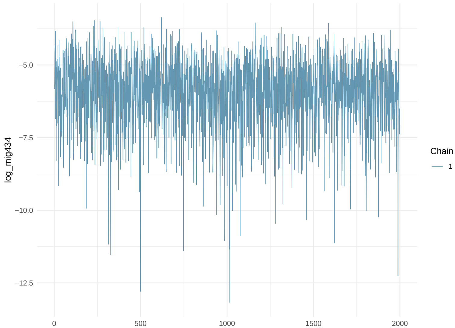
Trace Plot: log_mig434
