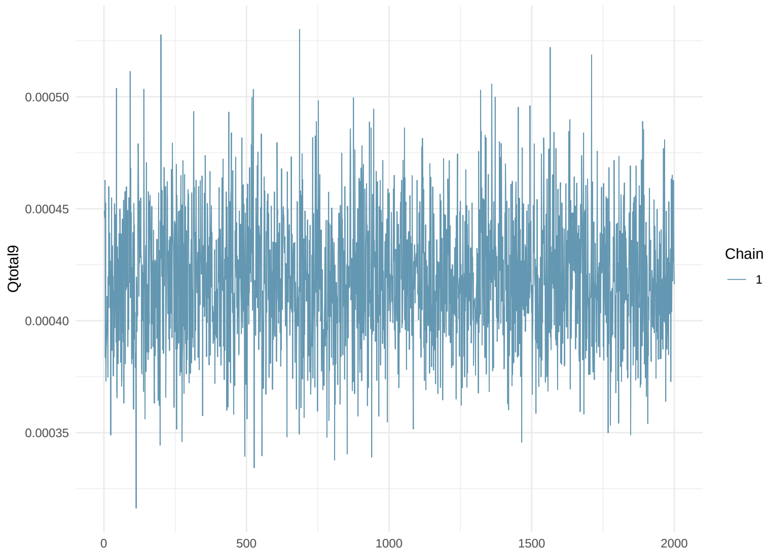
Trace Plot: Qtotal9
