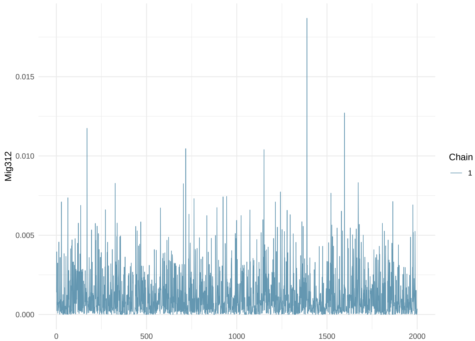
Trace Plot: Mig312
