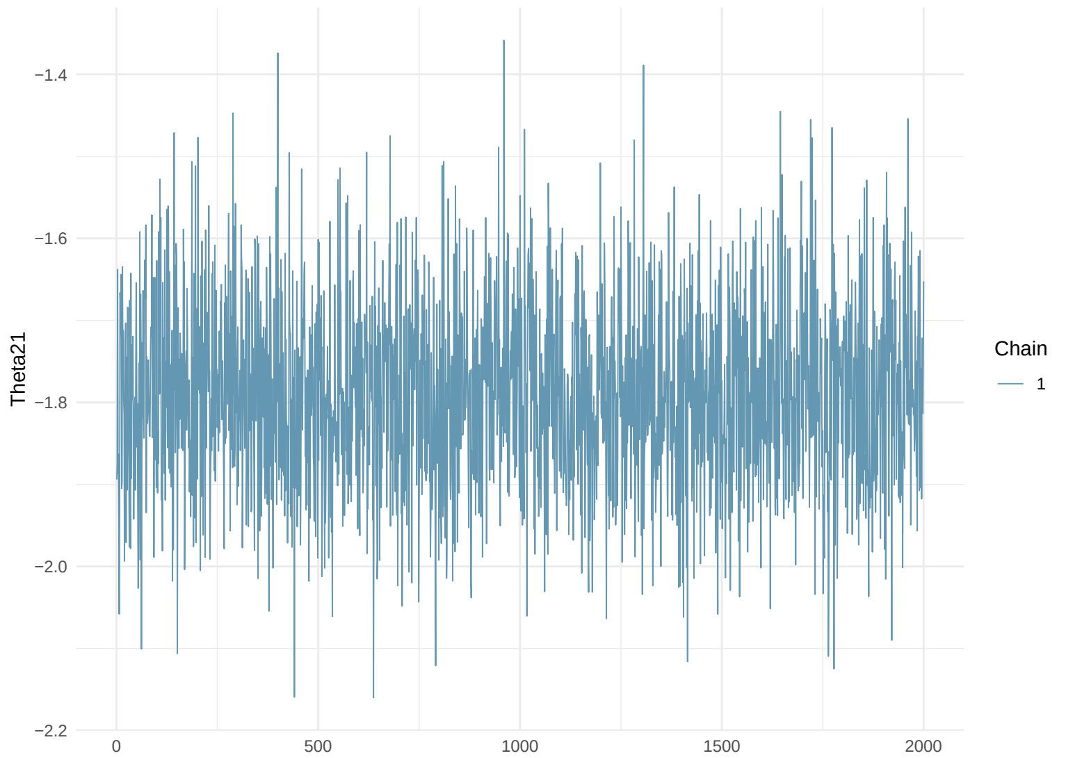
Trace Plot: Theta21
