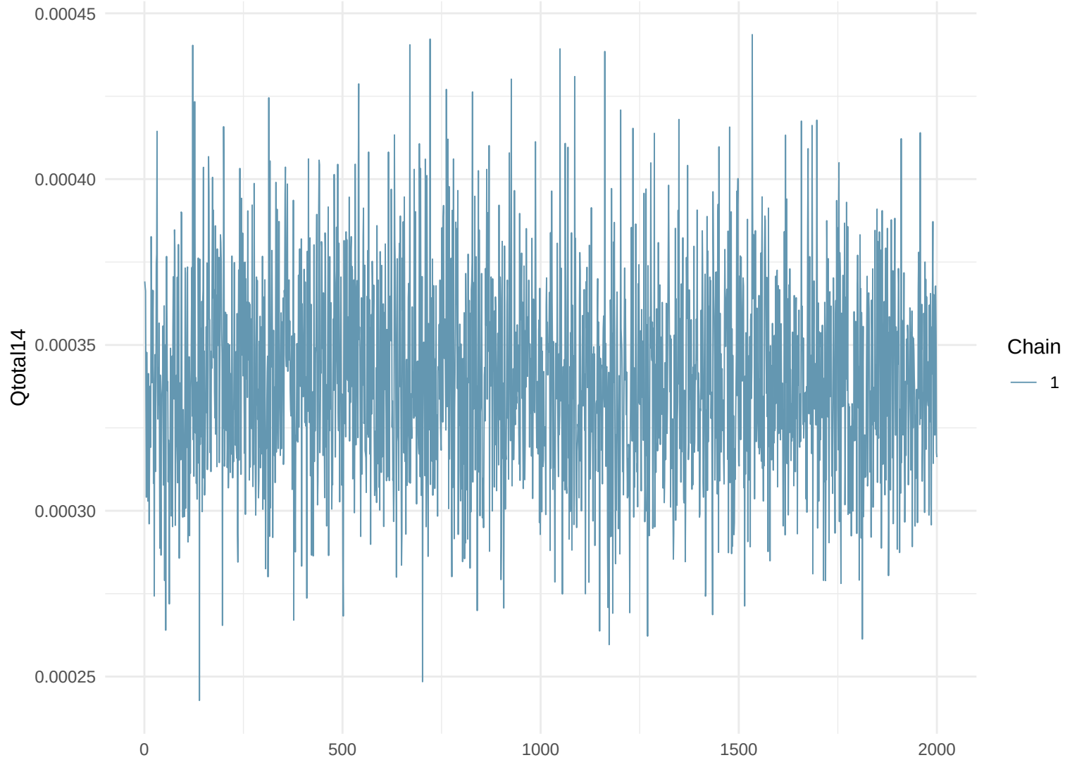
Trace Plot: Qtotal14
