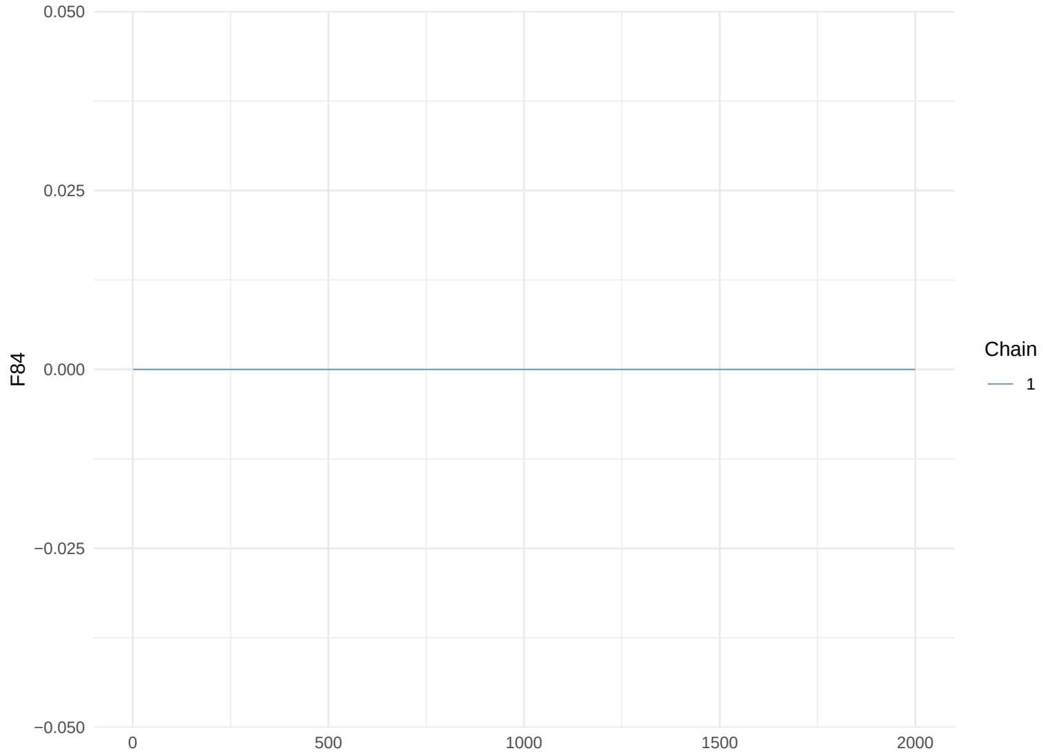
Trace Plot: F84
