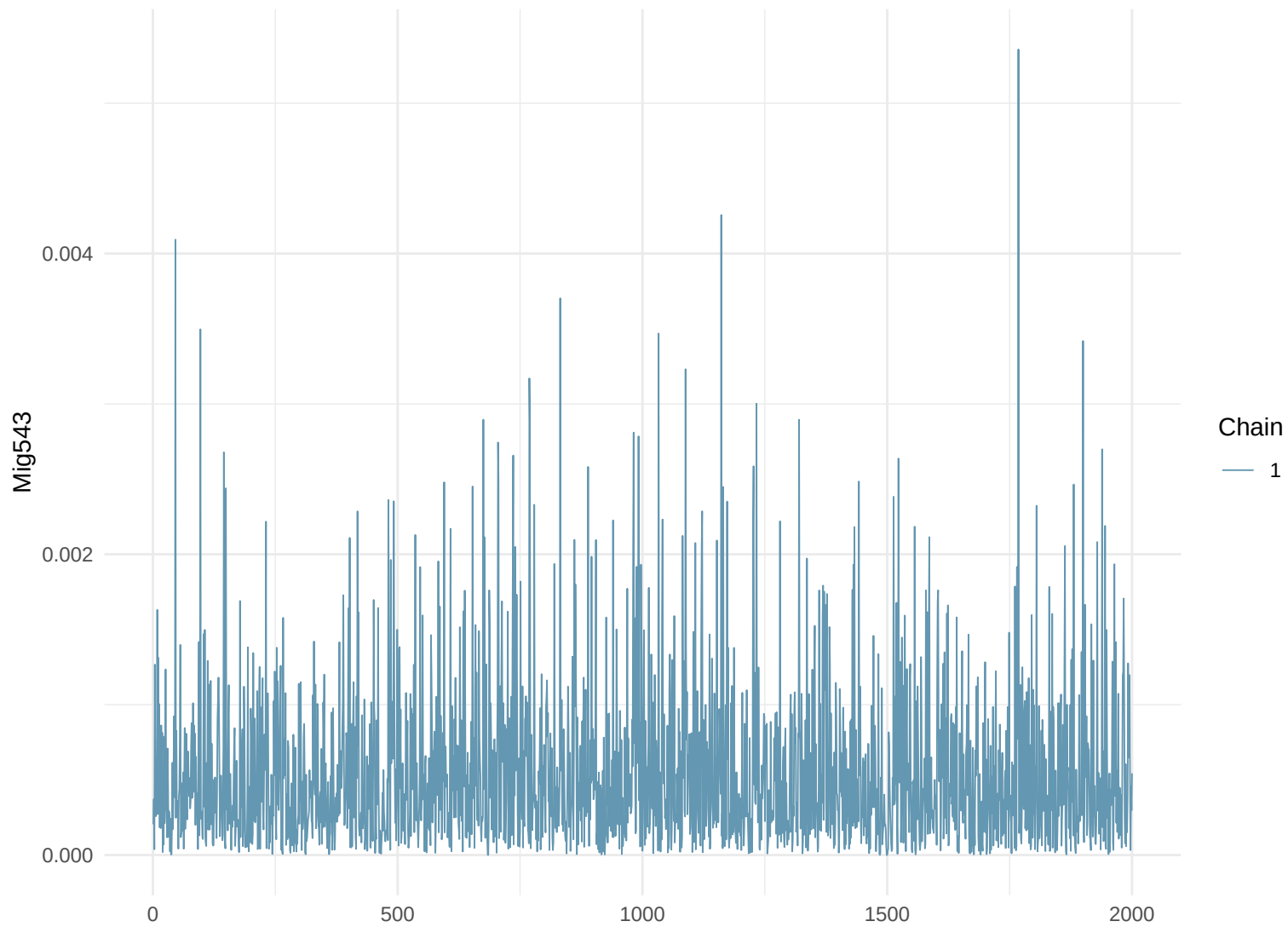
Trace Plot: Mig543
