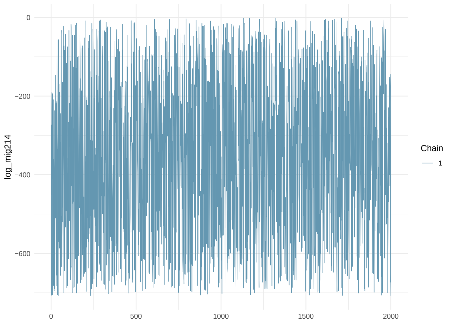
Trace Plot: log_mig214
