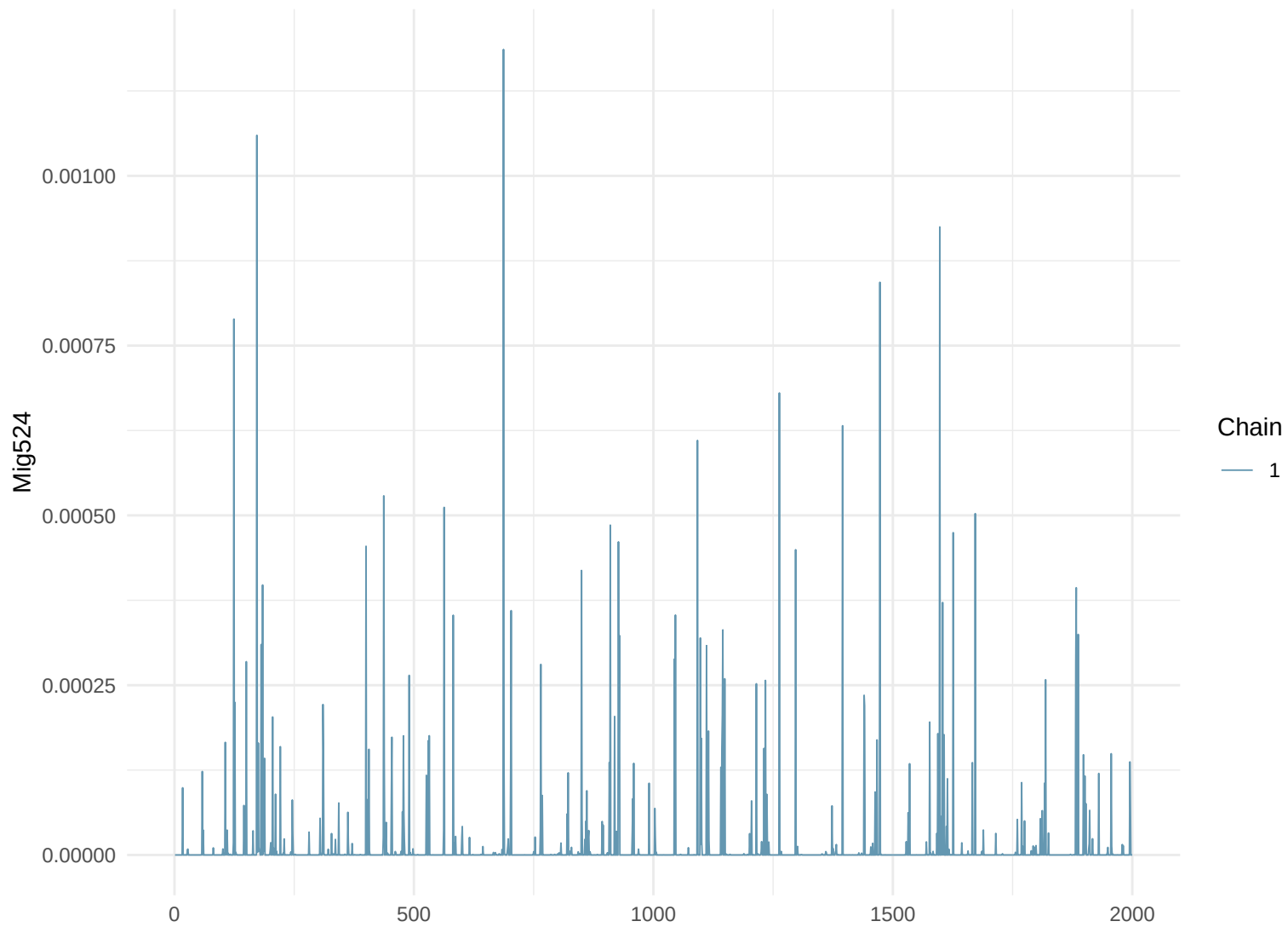
Trace Plot: Mig524
