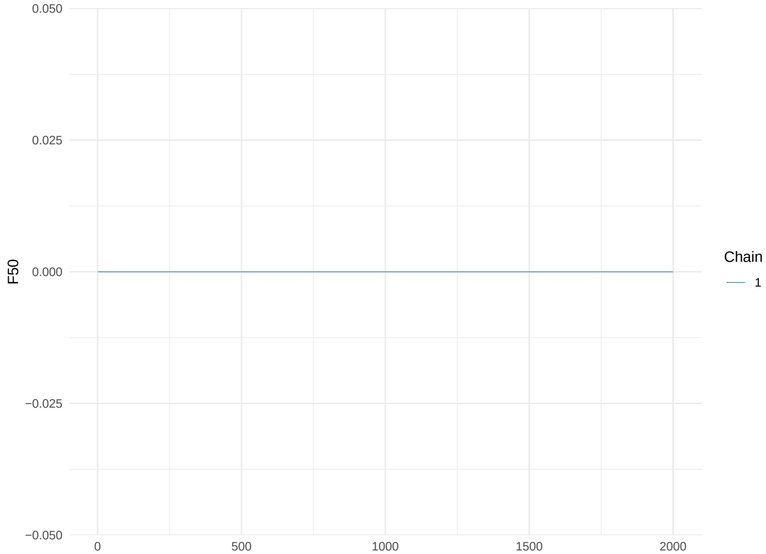
Trace Plot: F50
