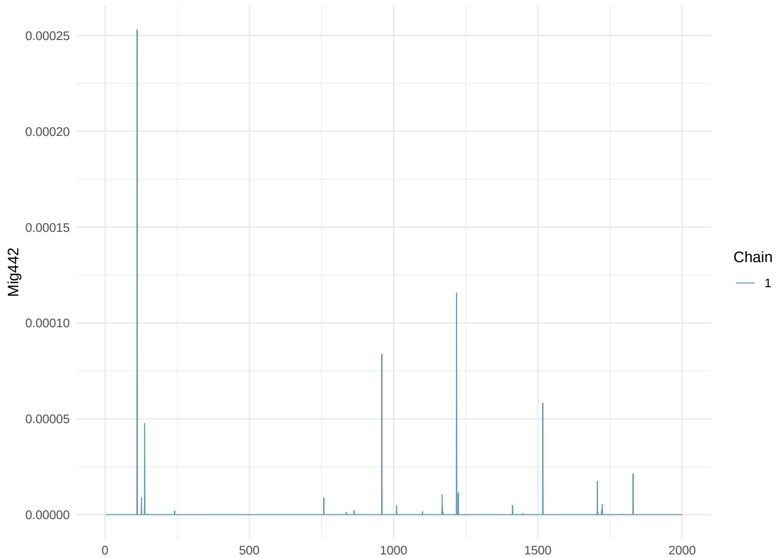
Trace Plot: Mig442
