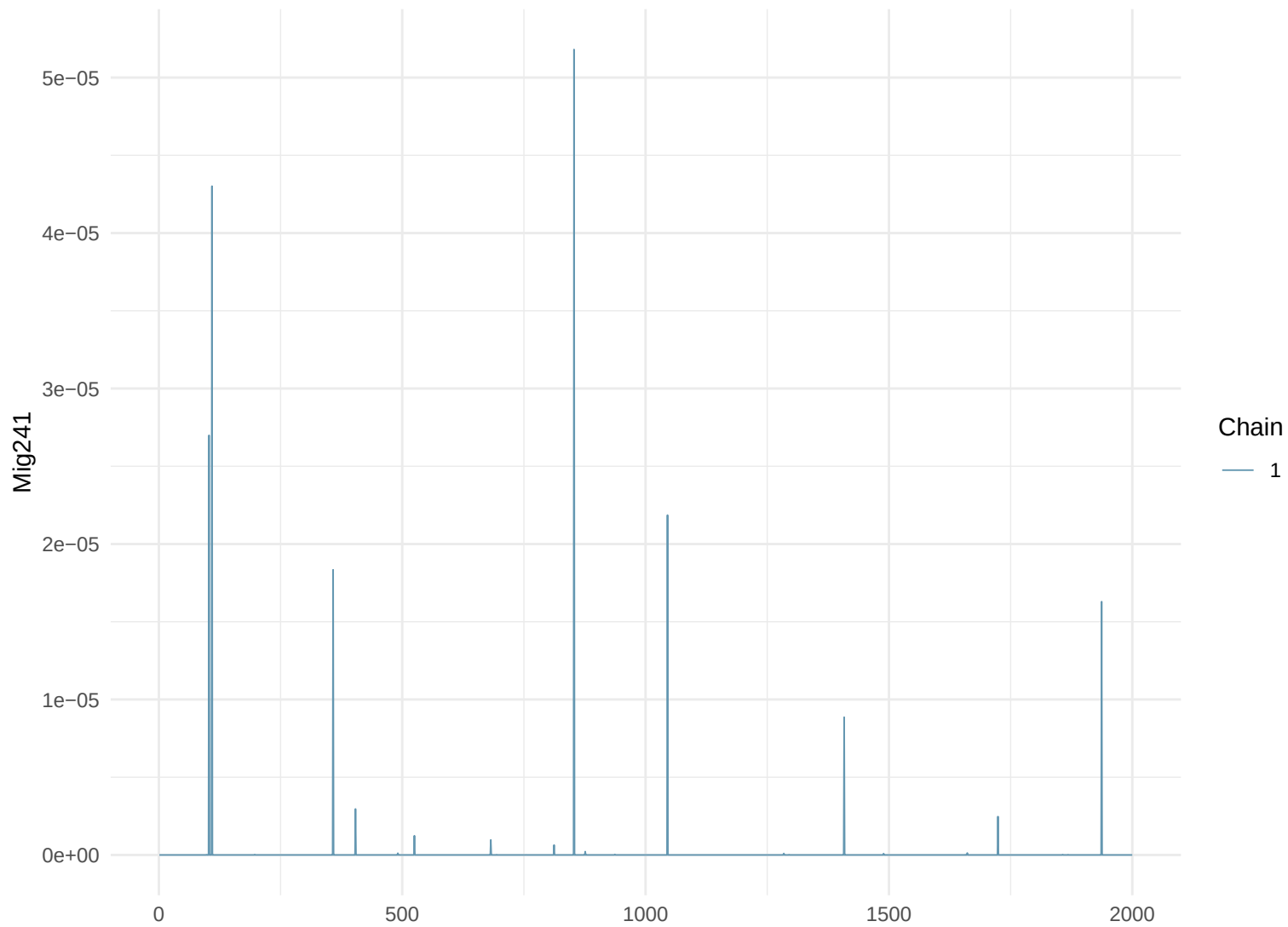
Trace Plot: Mig241
