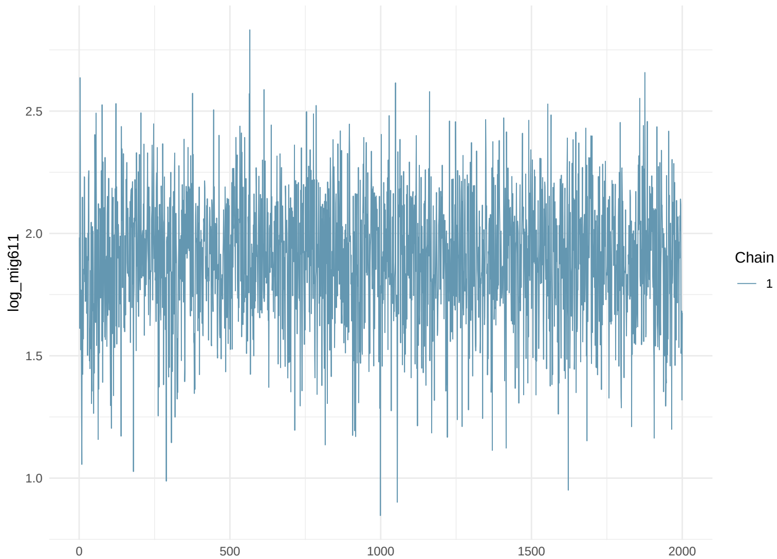
Trace Plot: log_mig611
