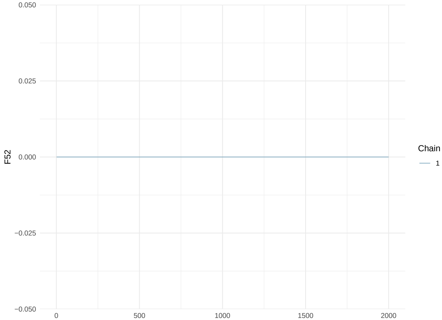
Trace Plot: F52
