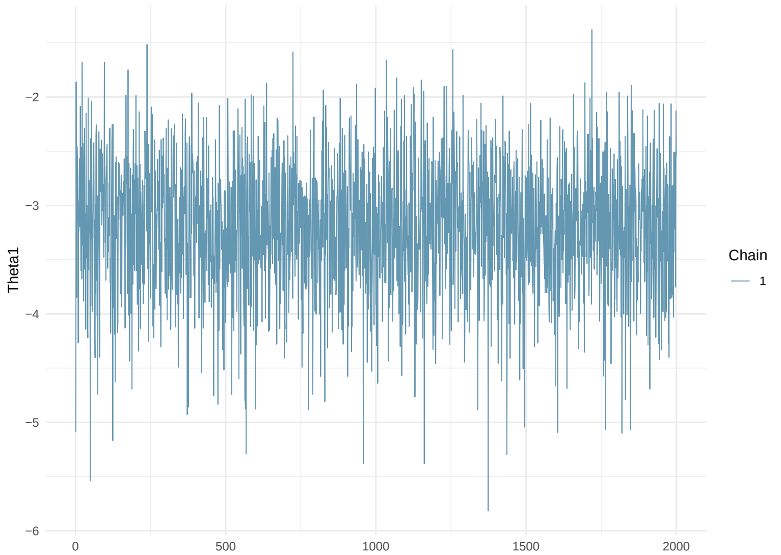
Trace Plot: Theta1
