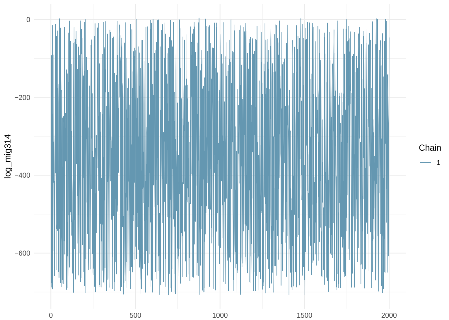
Trace Plot: log_mig314
