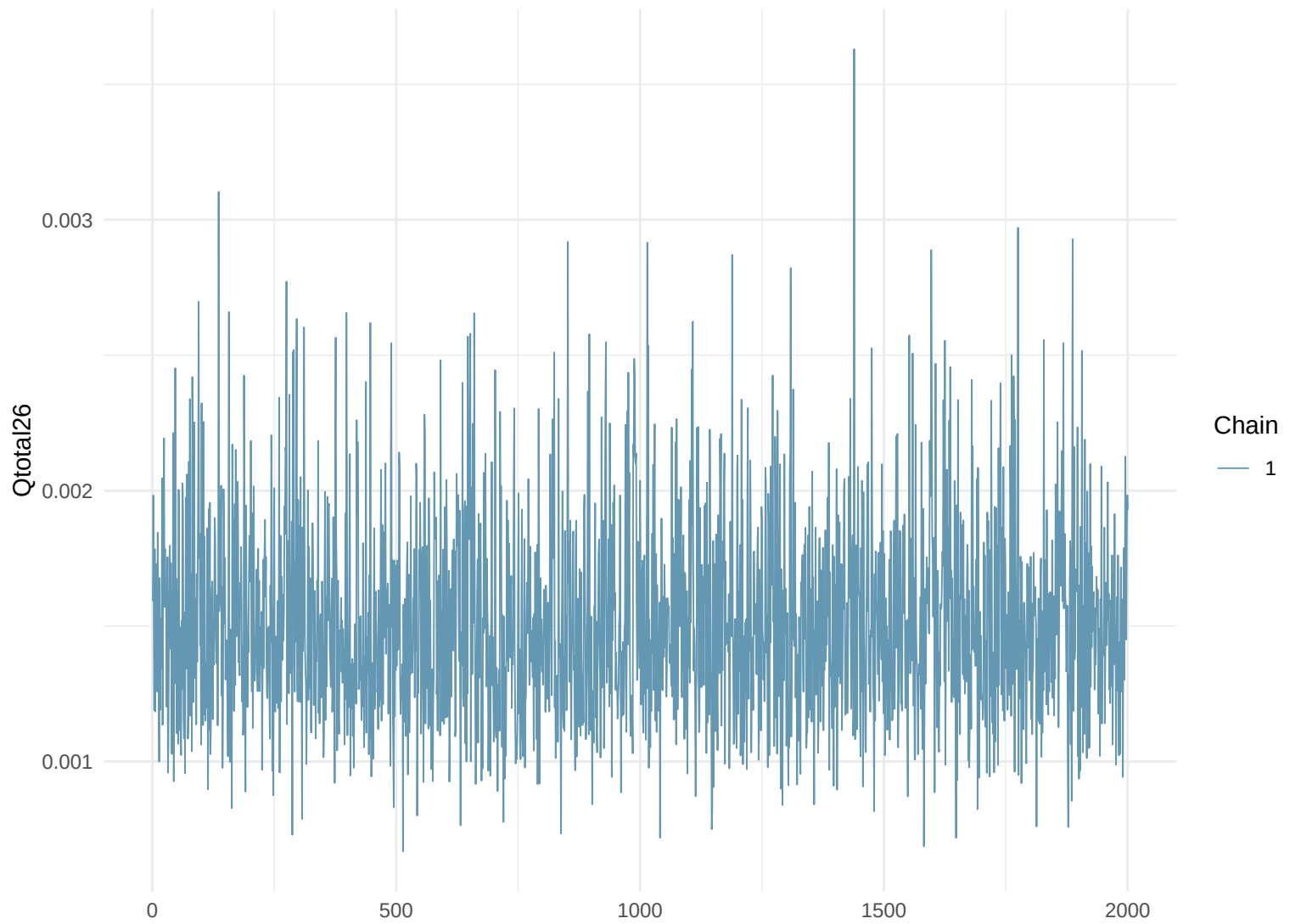
Trace Plot: Qtotal26
