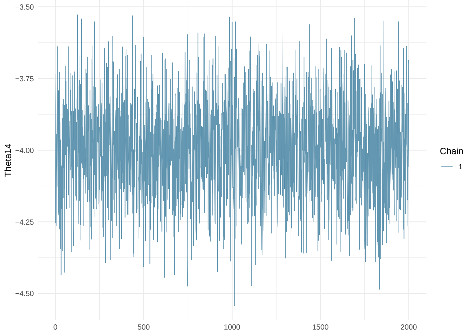
Trace Plot: Theta14
