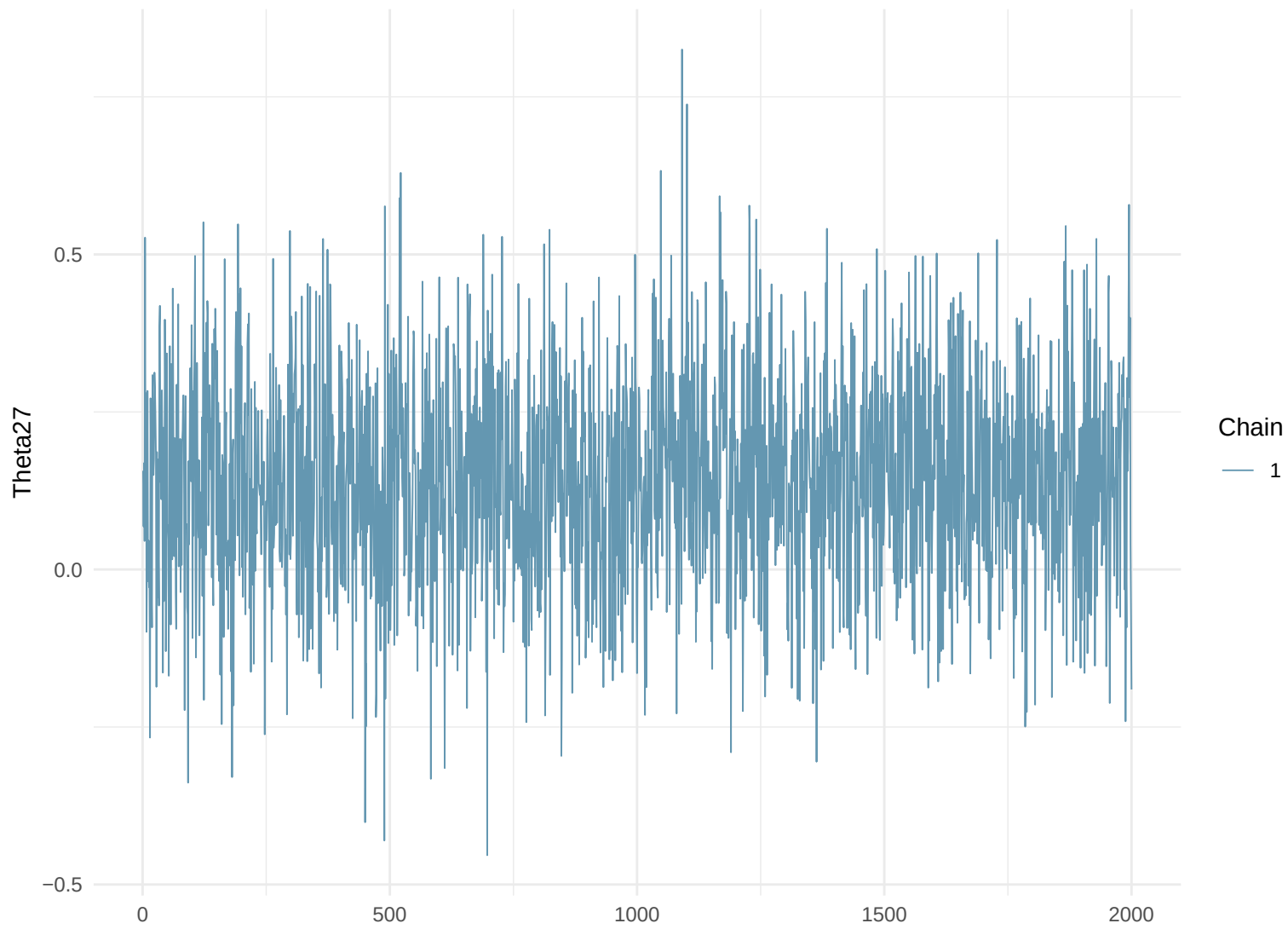
Trace Plot: Theta27
