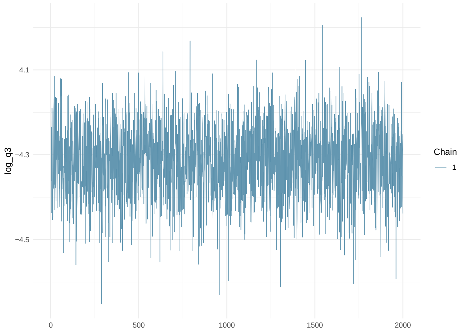
Trace Plot: log_q3
