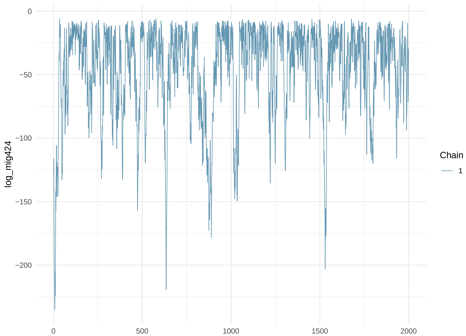
Trace Plot: log_mig424
