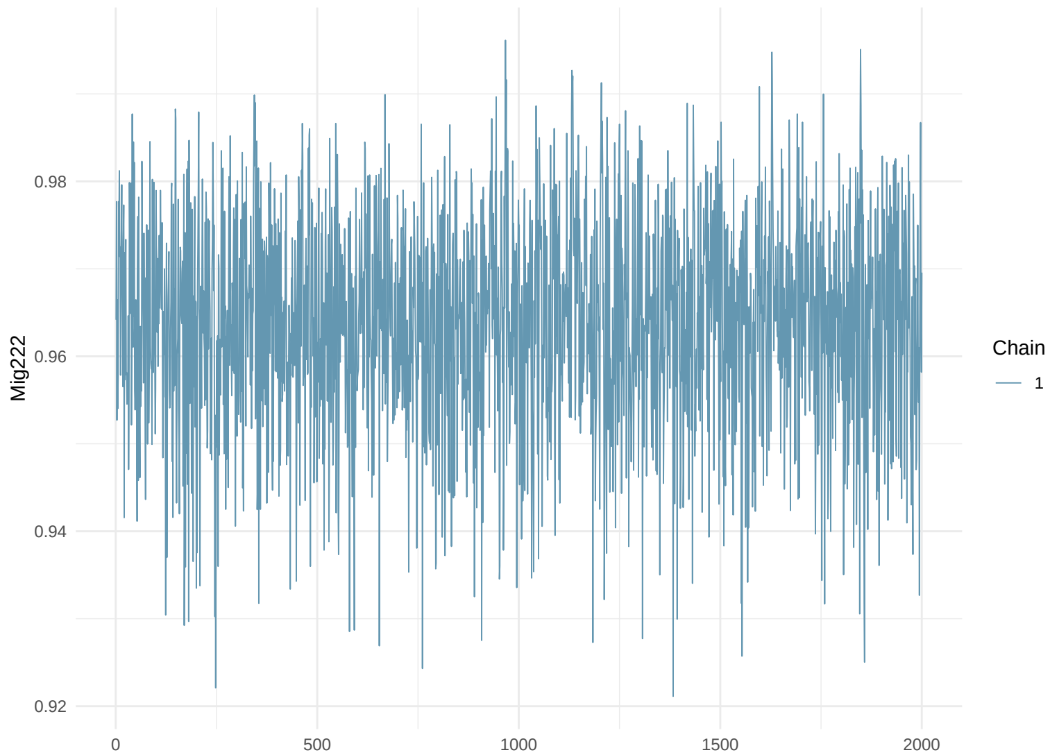
Trace Plot: Mig222
