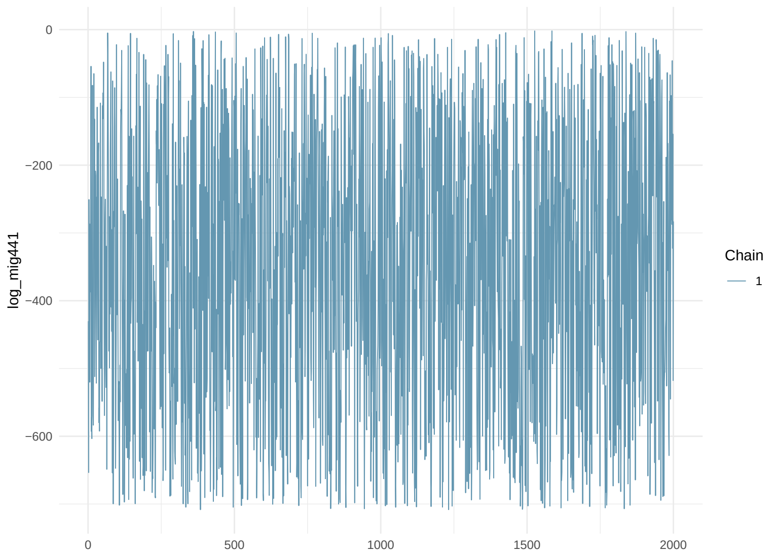
Trace Plot: log_mig441
