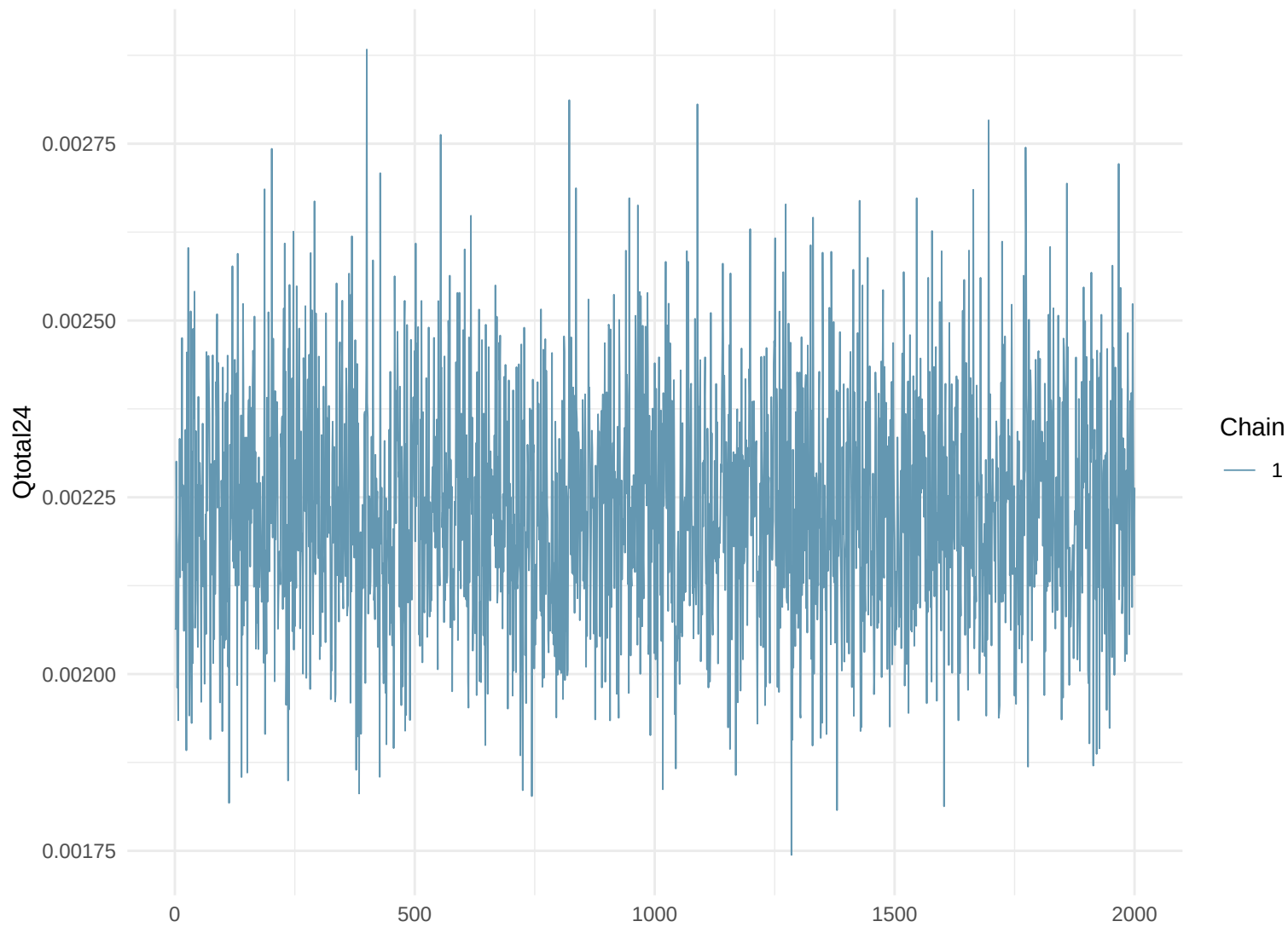
Trace Plot: Qtotal24
