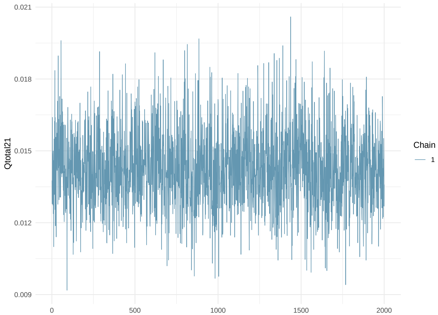
Trace Plot: Qtotal21
