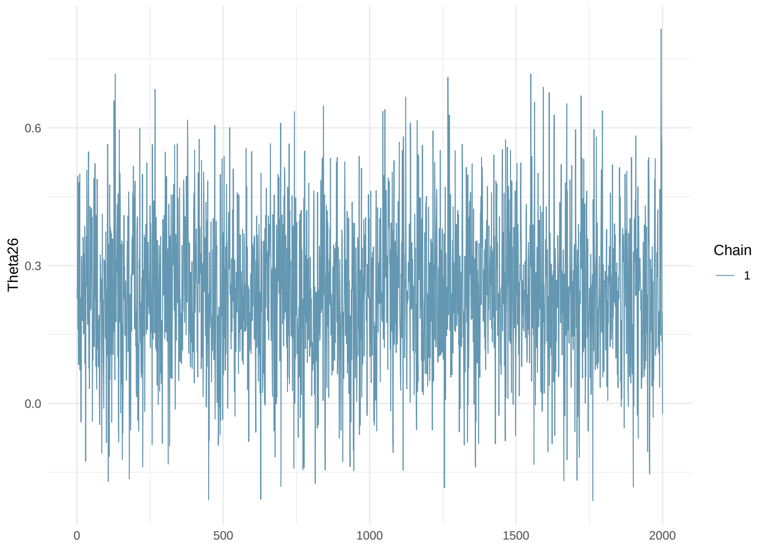
Trace Plot: Theta26
