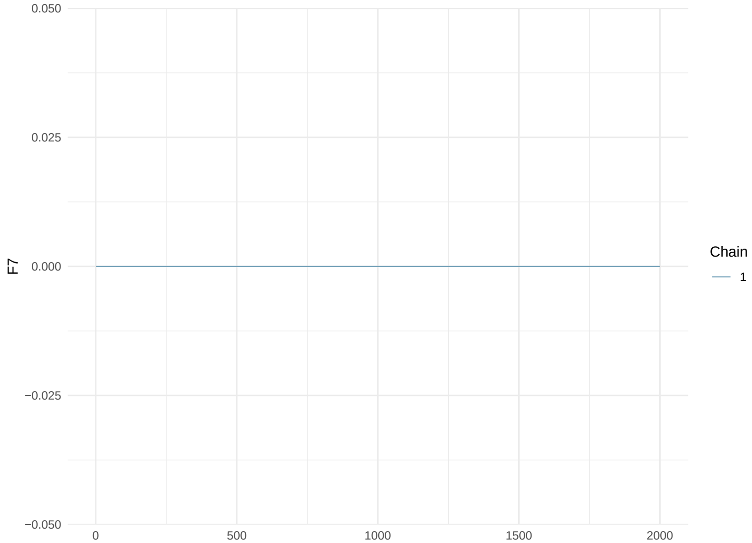
Trace Plot: F7
