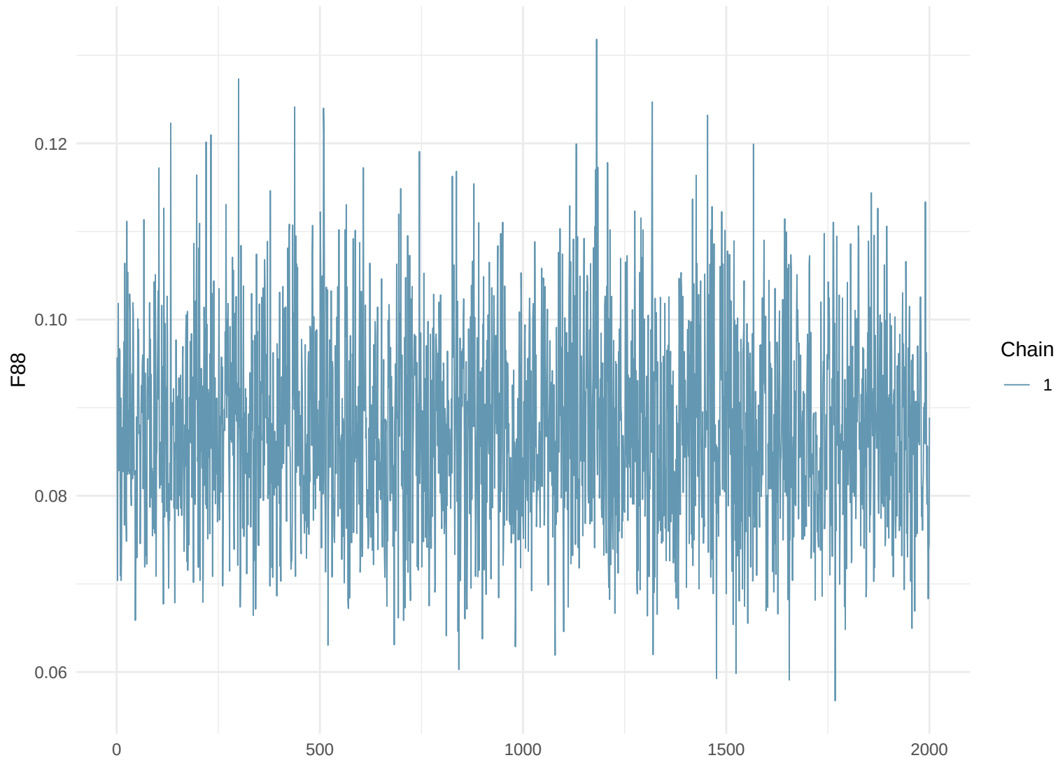
Trace Plot: F88
