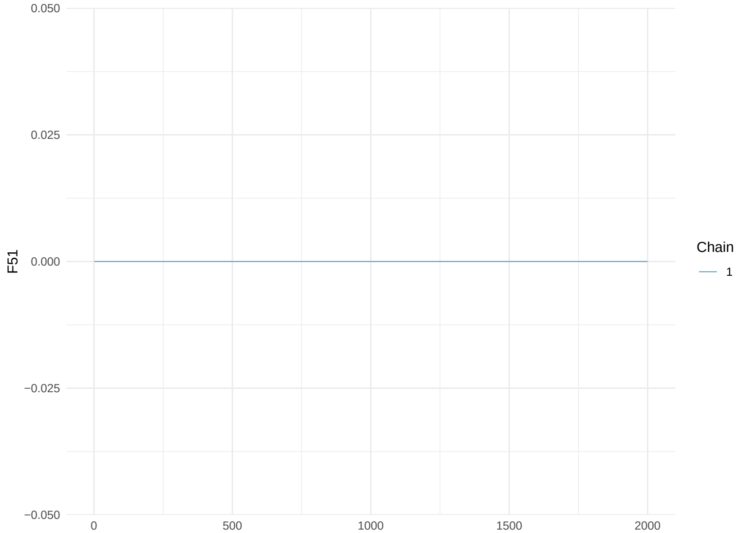
Trace Plot: F51
