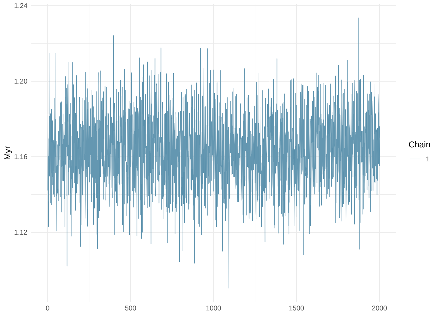
Trace Plot: Myr
