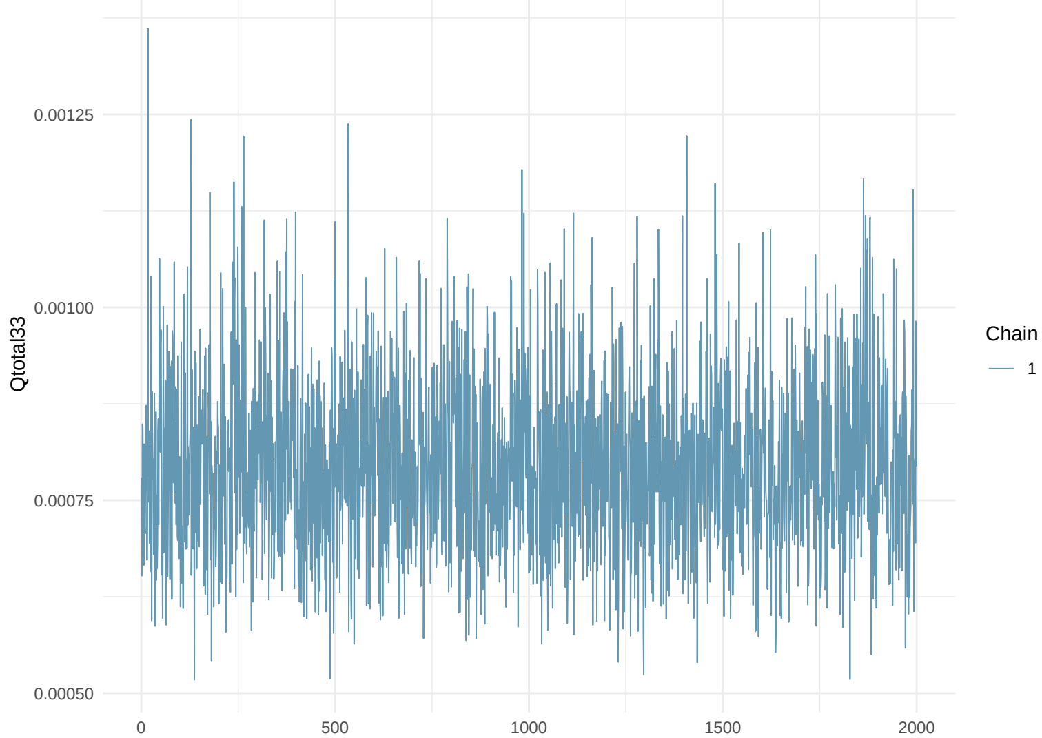
Trace Plot: Qtotal33
