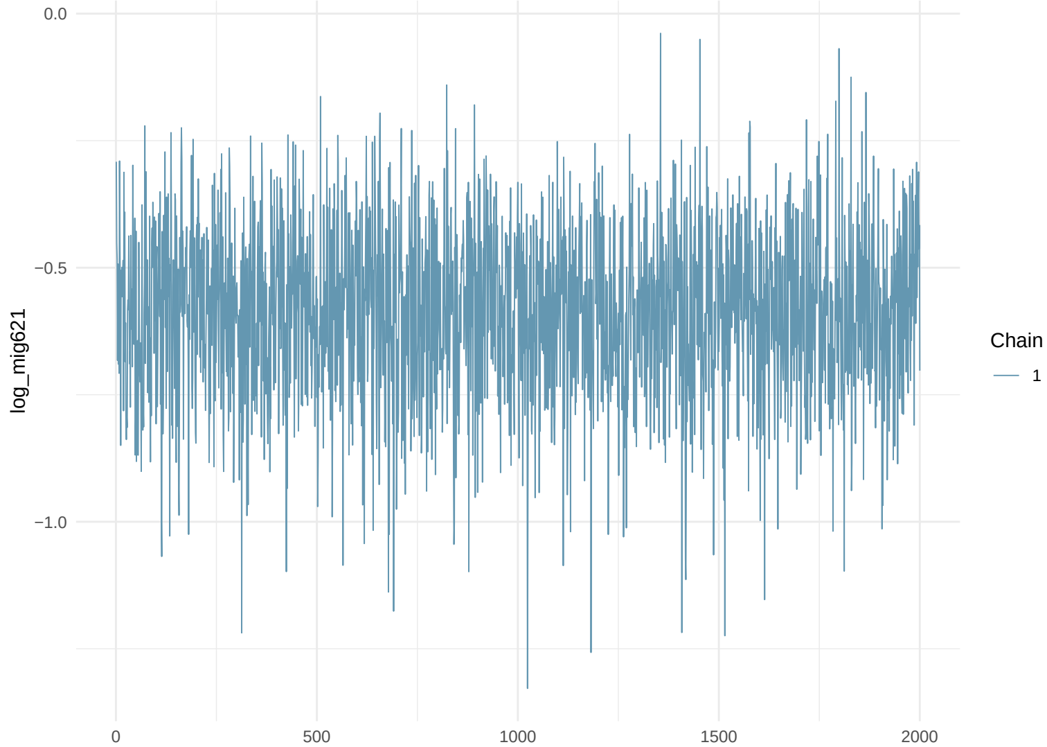
Trace Plot: log_mig621
