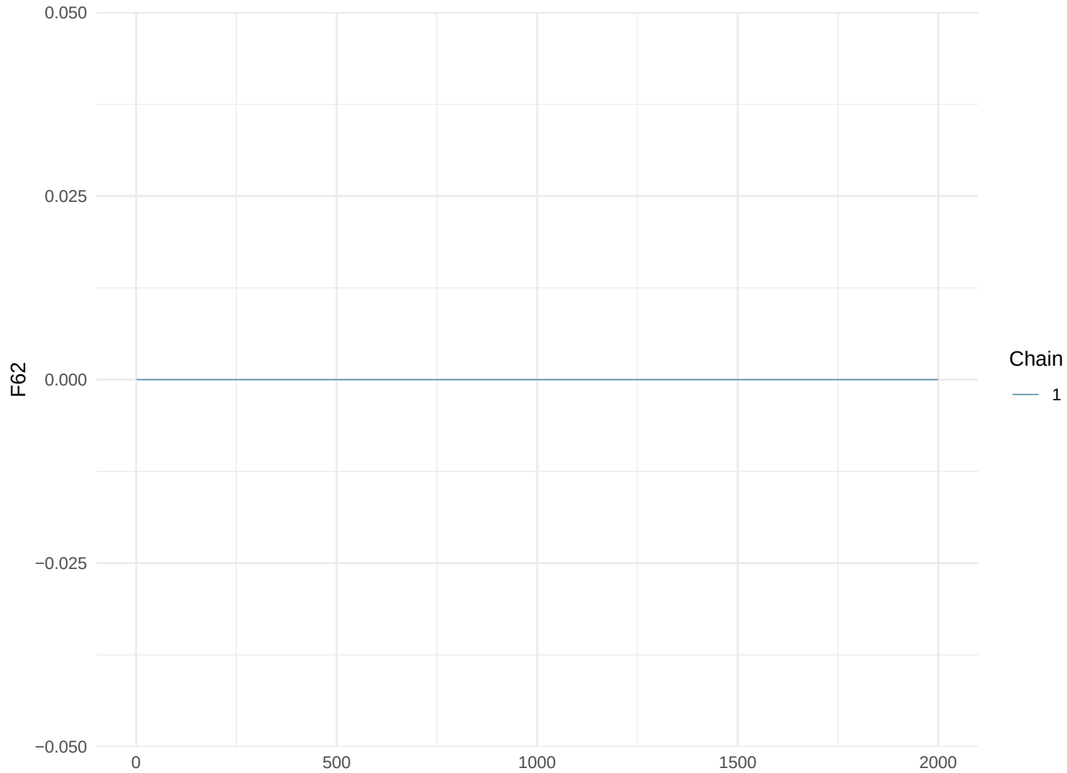
Trace Plot: F62
