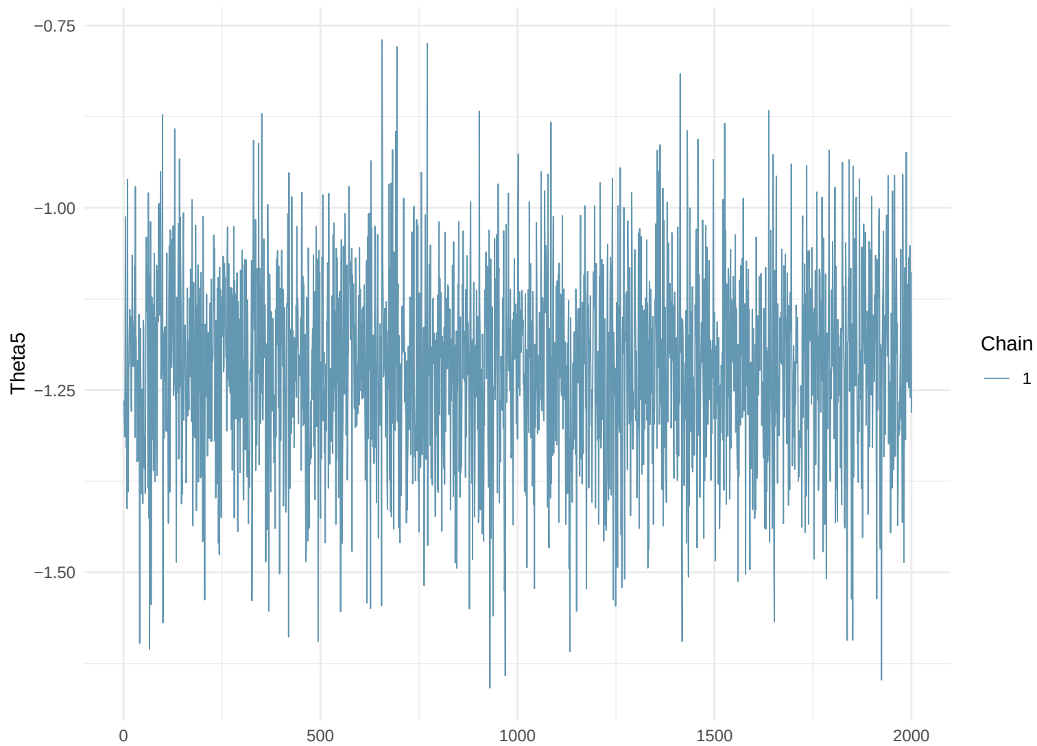
Trace Plot: Theta5
