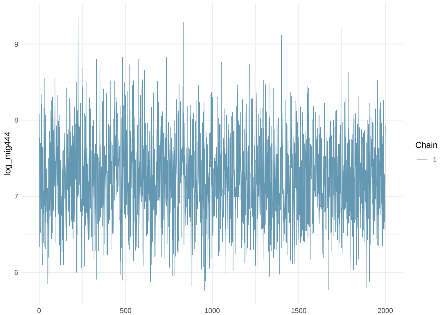
Trace Plot: log_mig444
