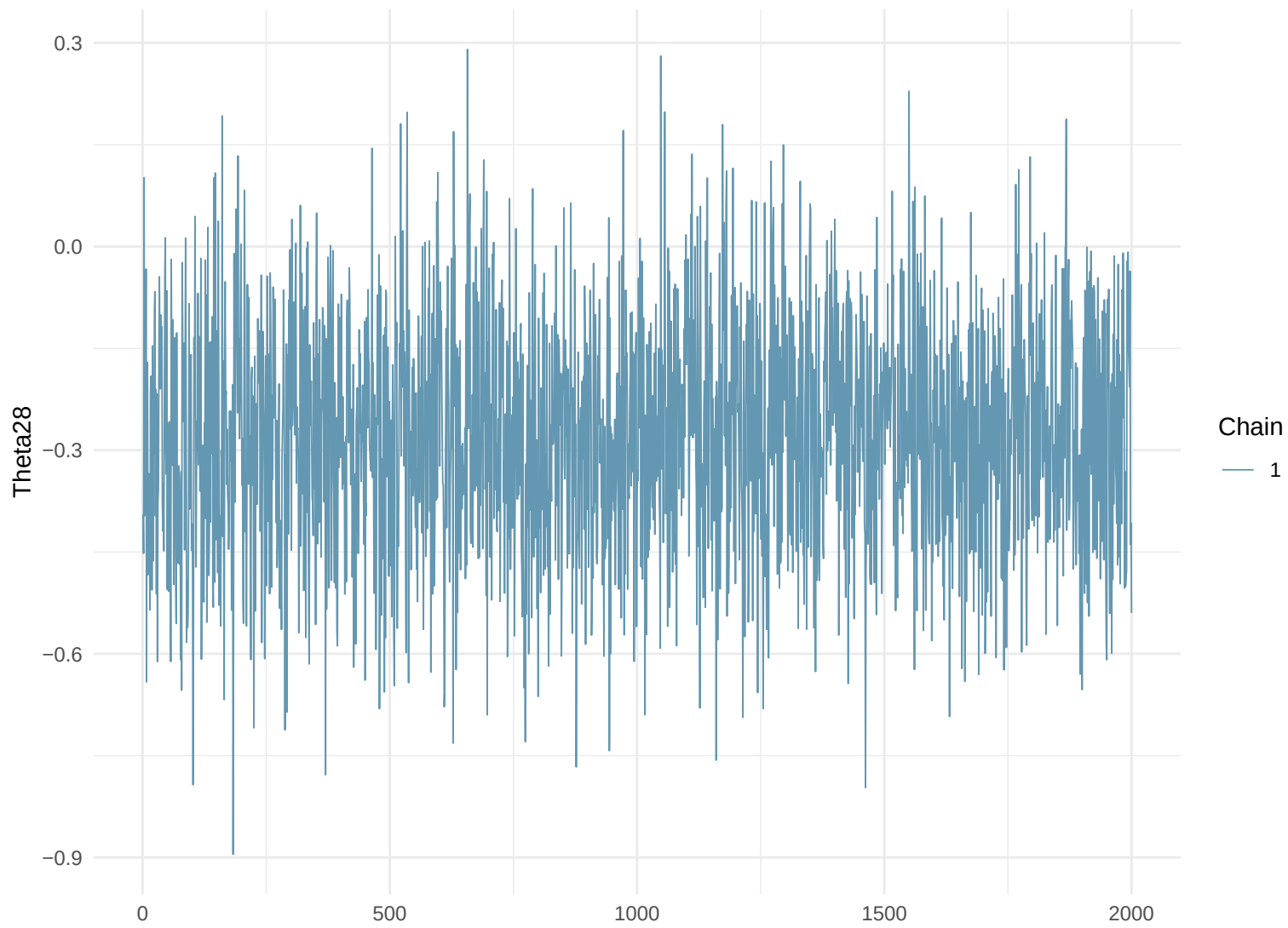
Trace Plot: Theta28
