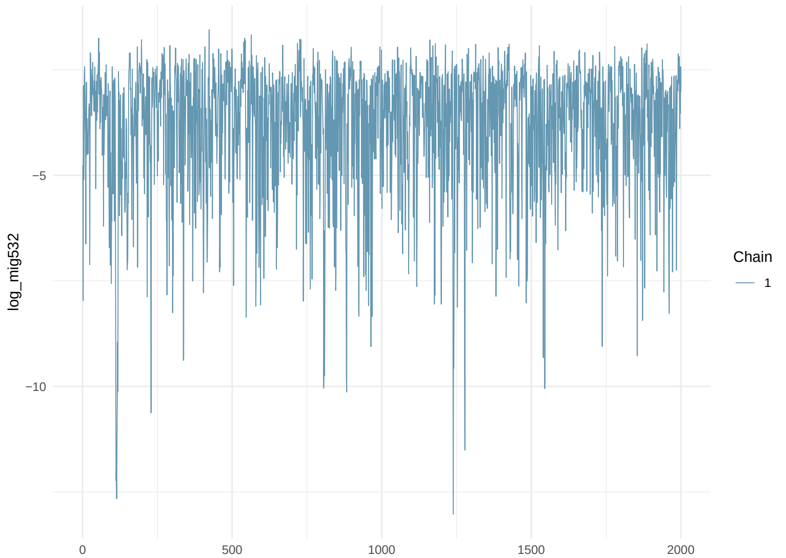
Trace Plot: log_mig532
