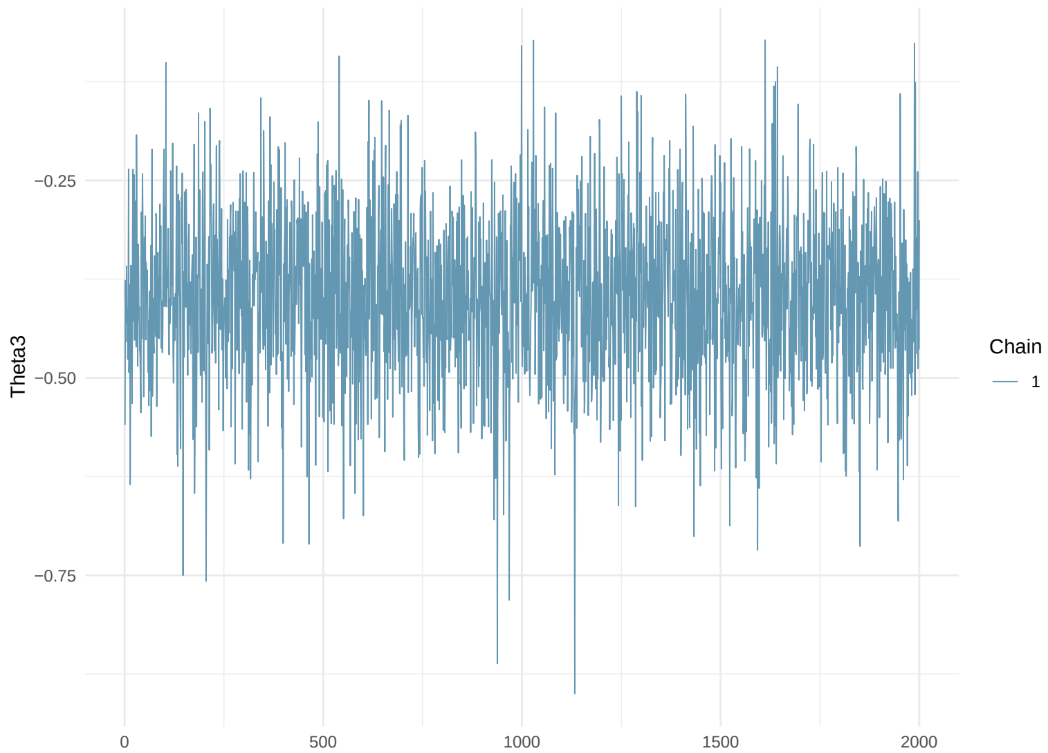
Trace Plot: Theta3
