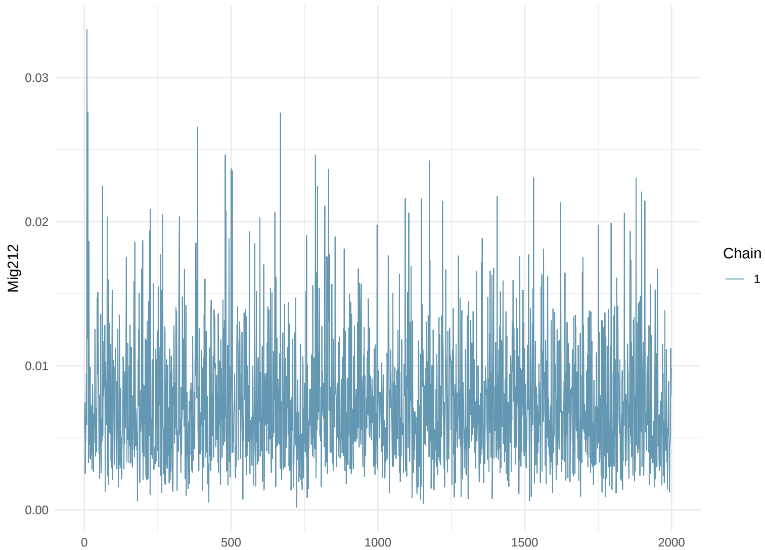
Trace Plot: Mig212
