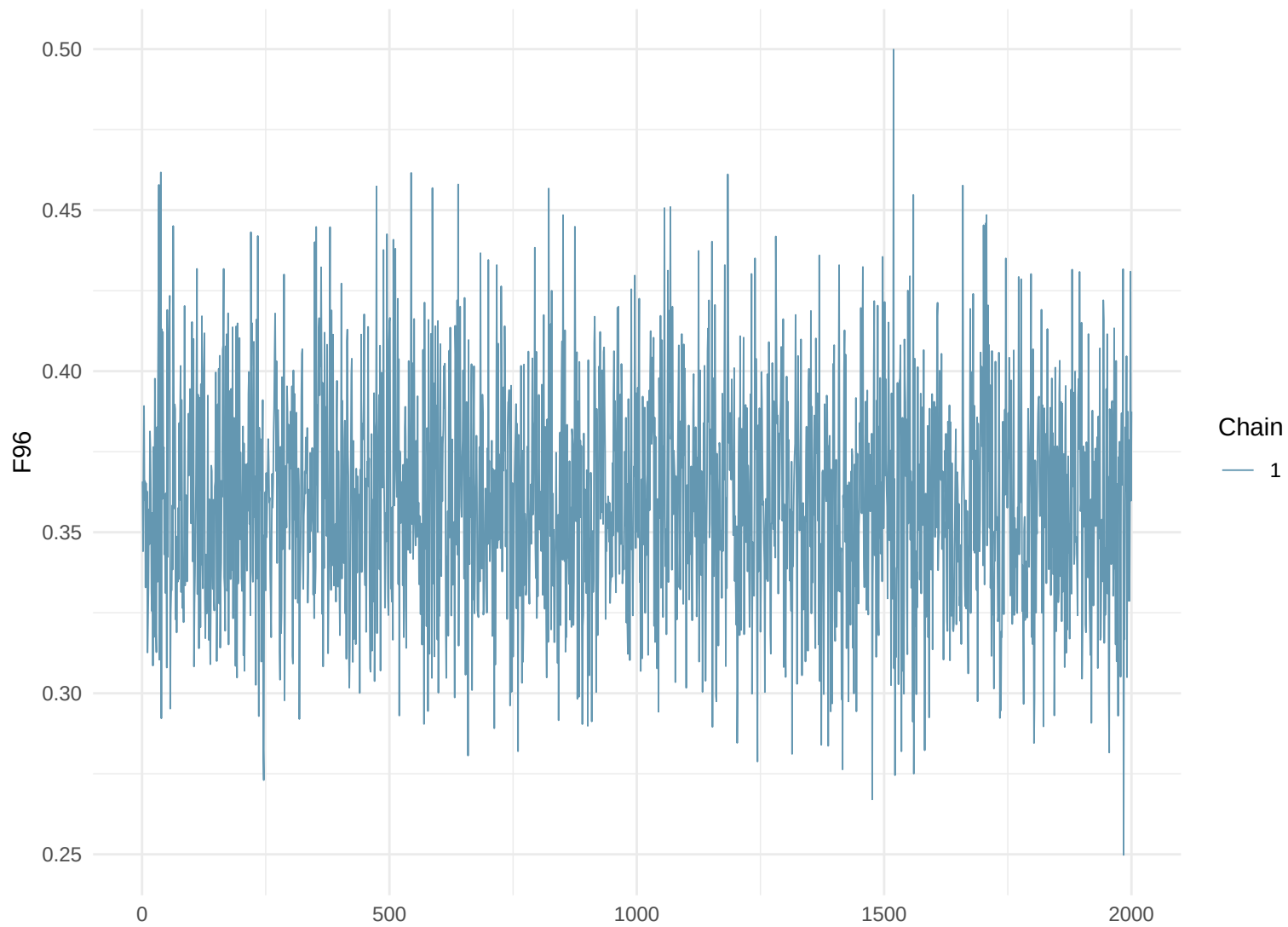
Trace Plot: F96
