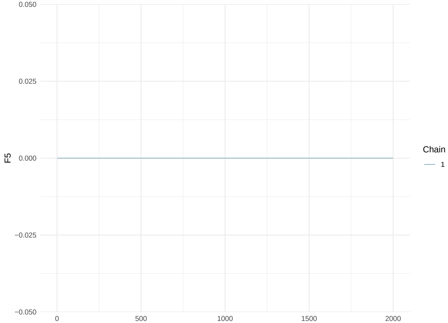
Trace Plot: F5
