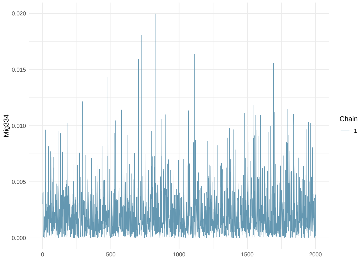
Trace Plot: Mig334
