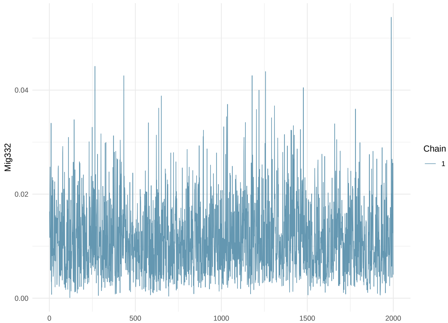
Trace Plot: Mig332
