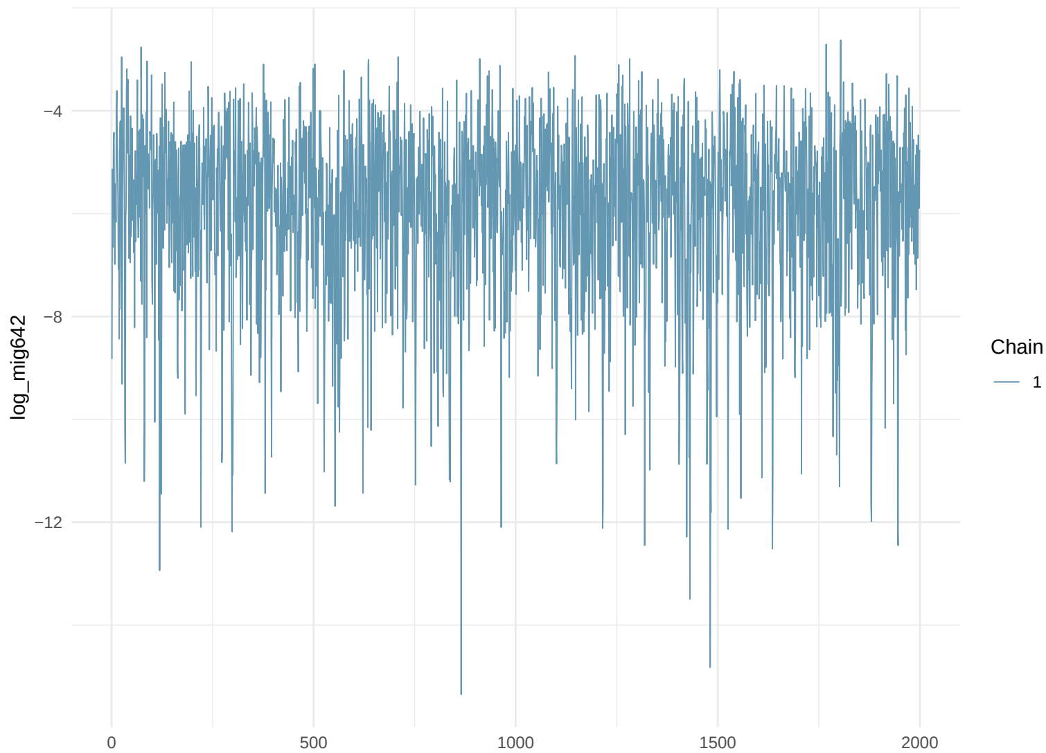
Trace Plot: log_mig642
