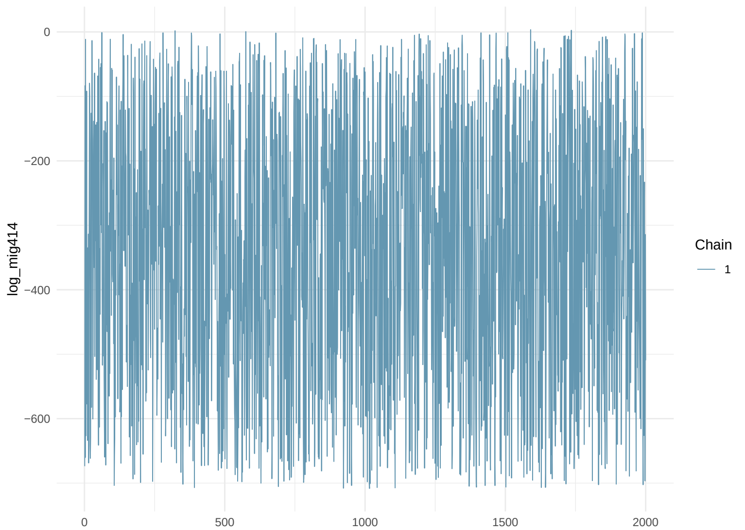
Trace Plot: log_mig414
