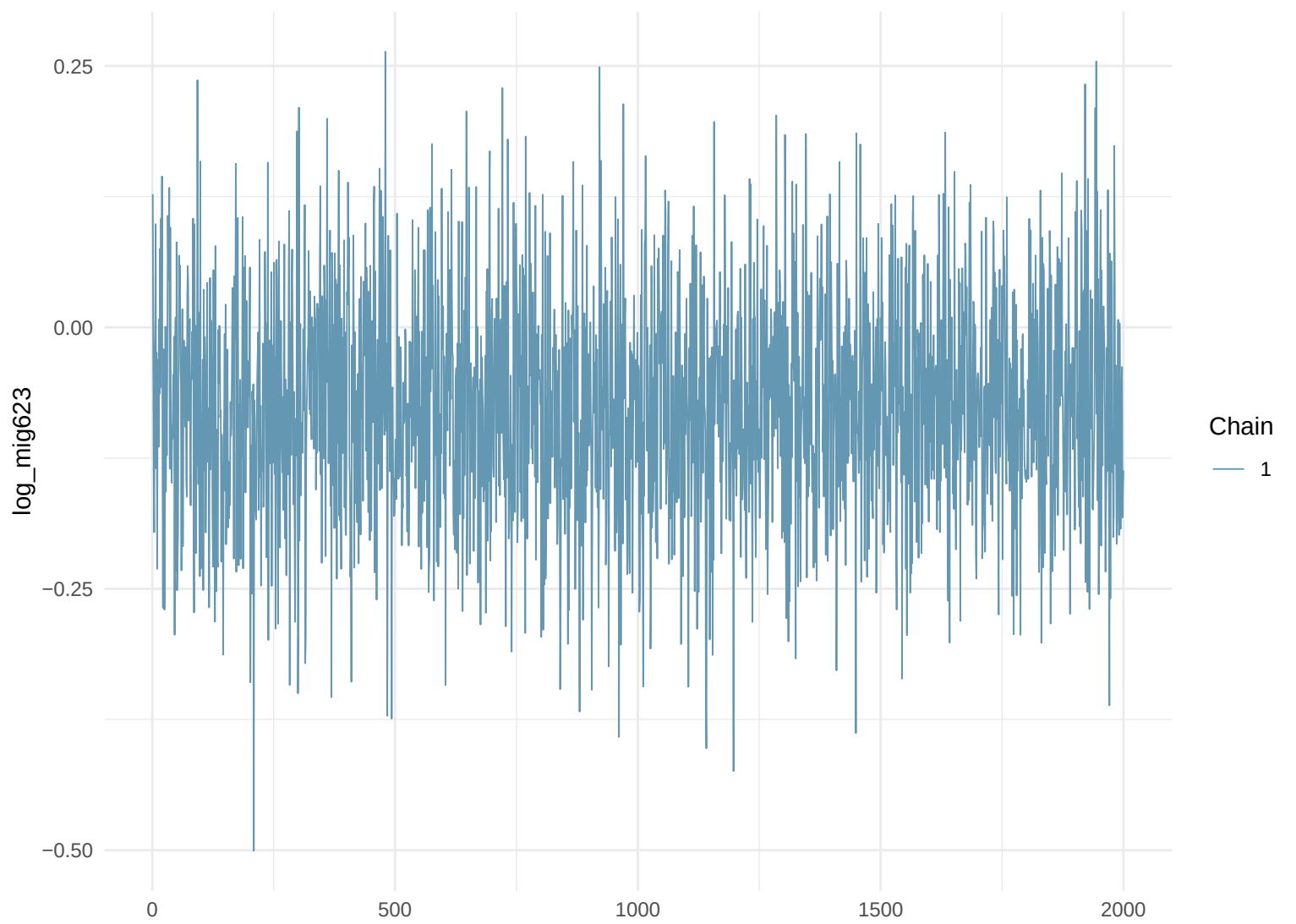
Trace Plot: log_mig623
