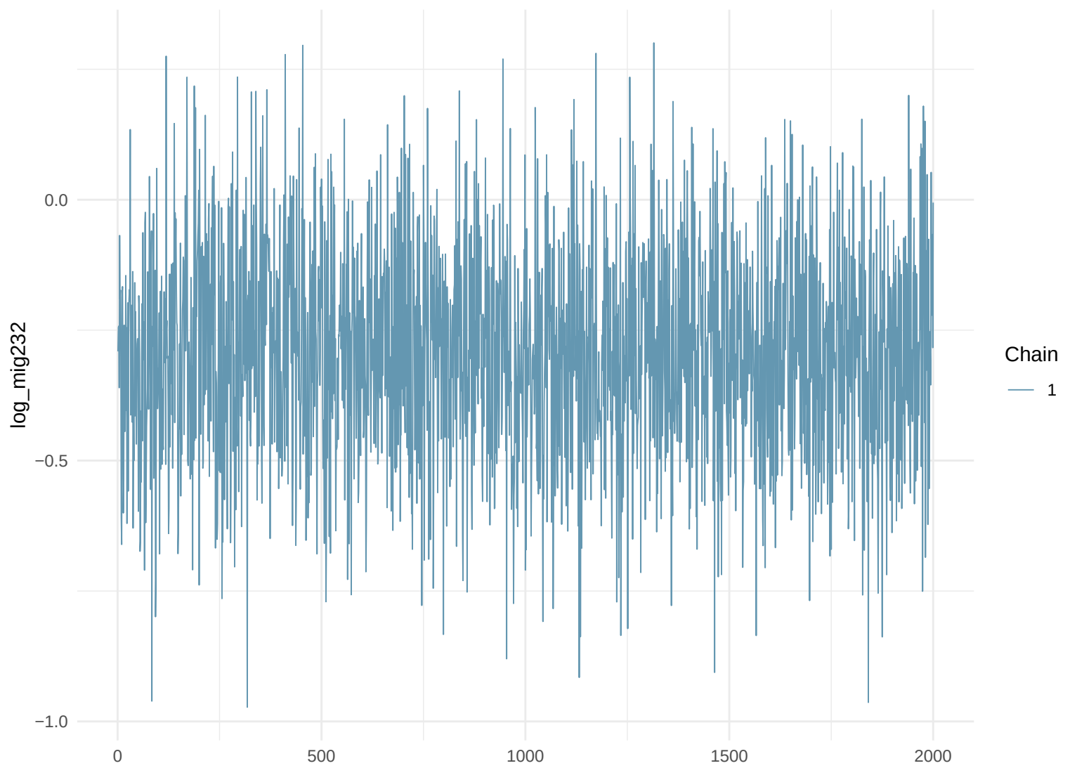
Trace Plot: log_mig232
