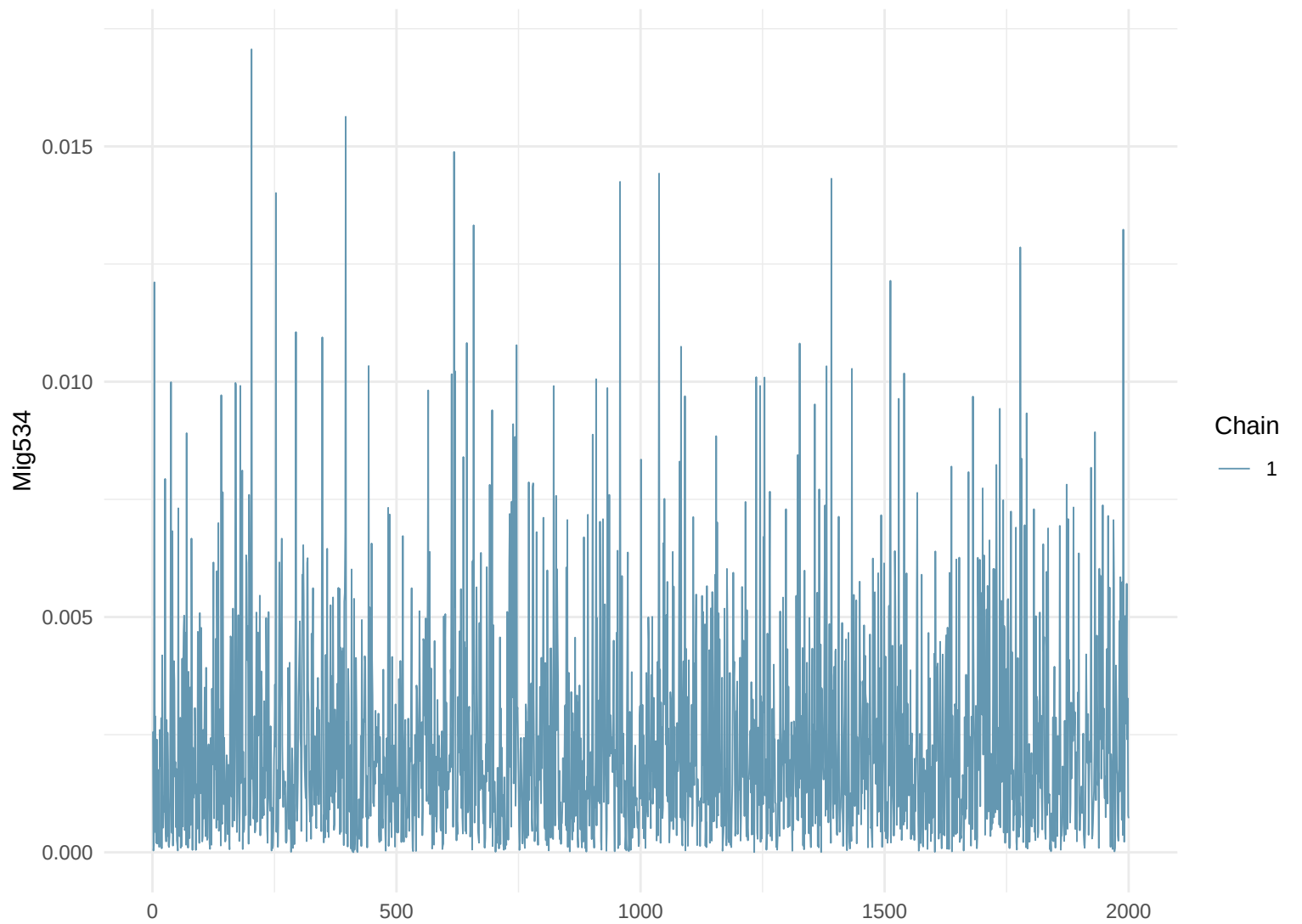
Trace Plot: Mig534
