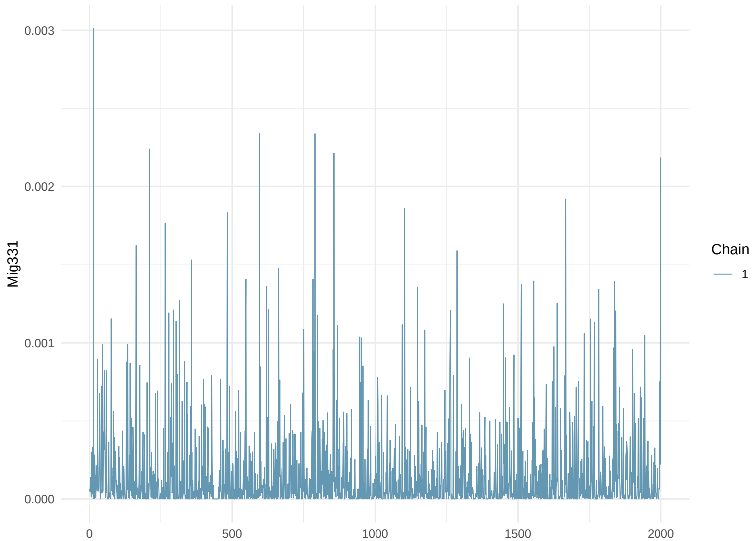
Trace Plot: Mig331
