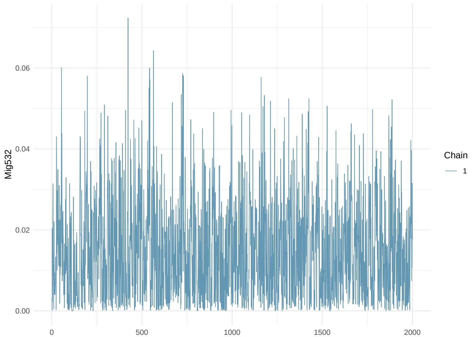
Trace Plot: Mig532
