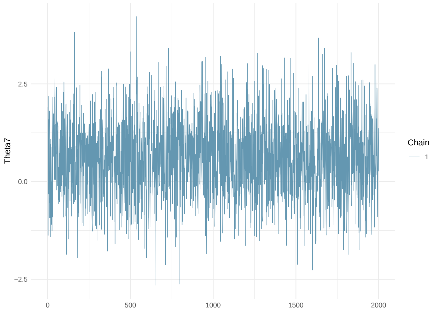
Trace Plot: Theta7
