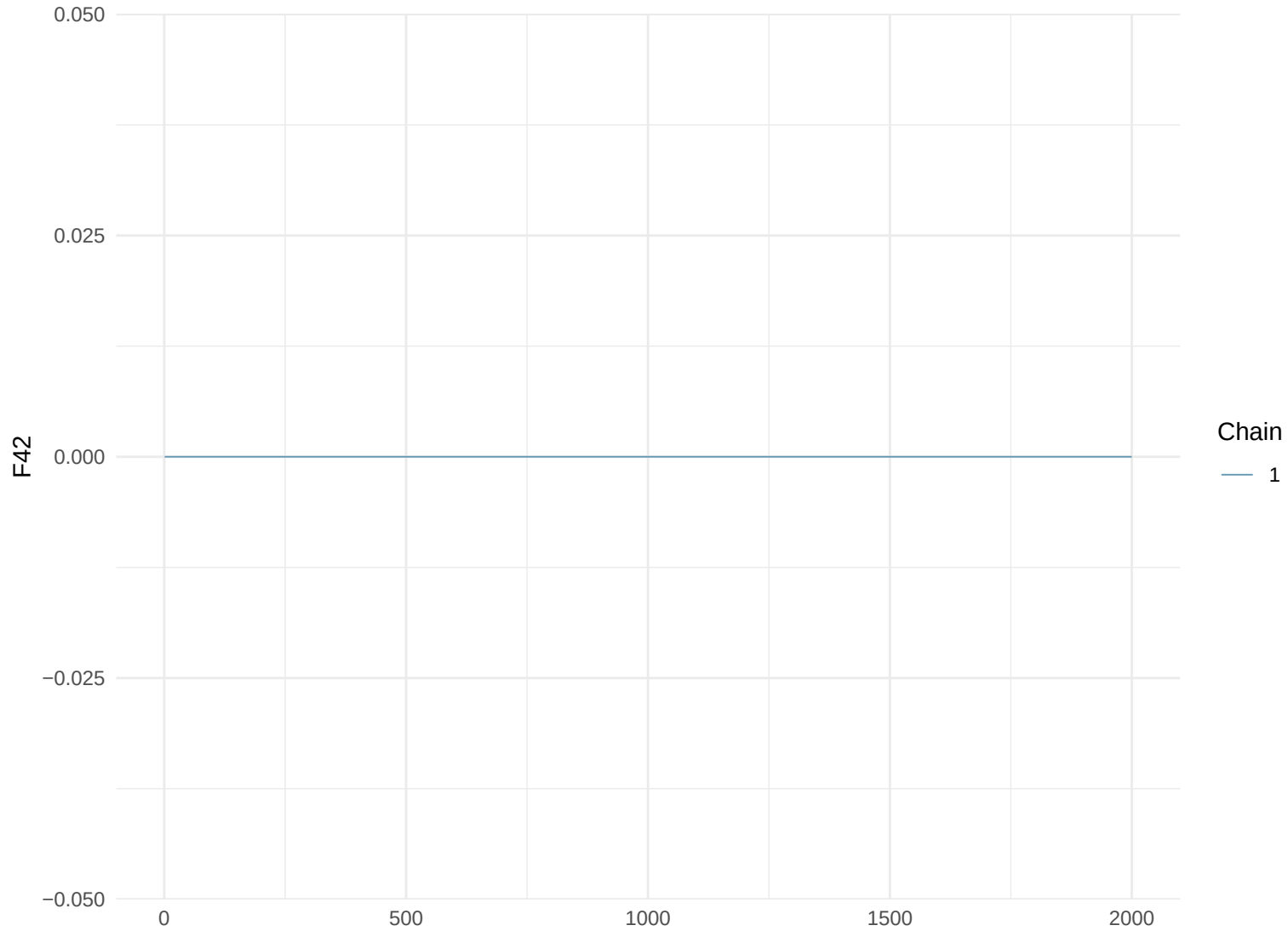
Trace Plot: F42
