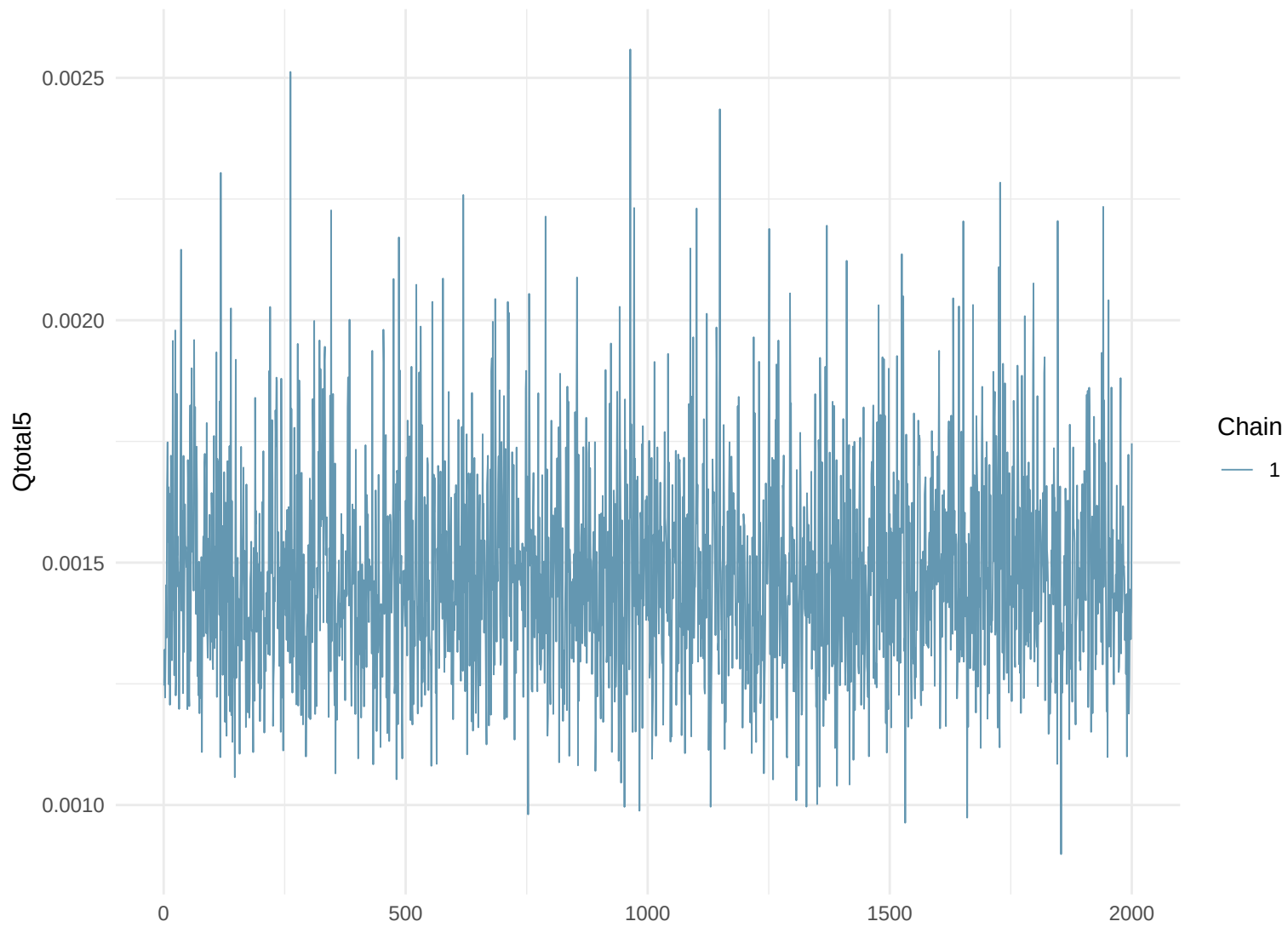
Trace Plot: Qtotal5
