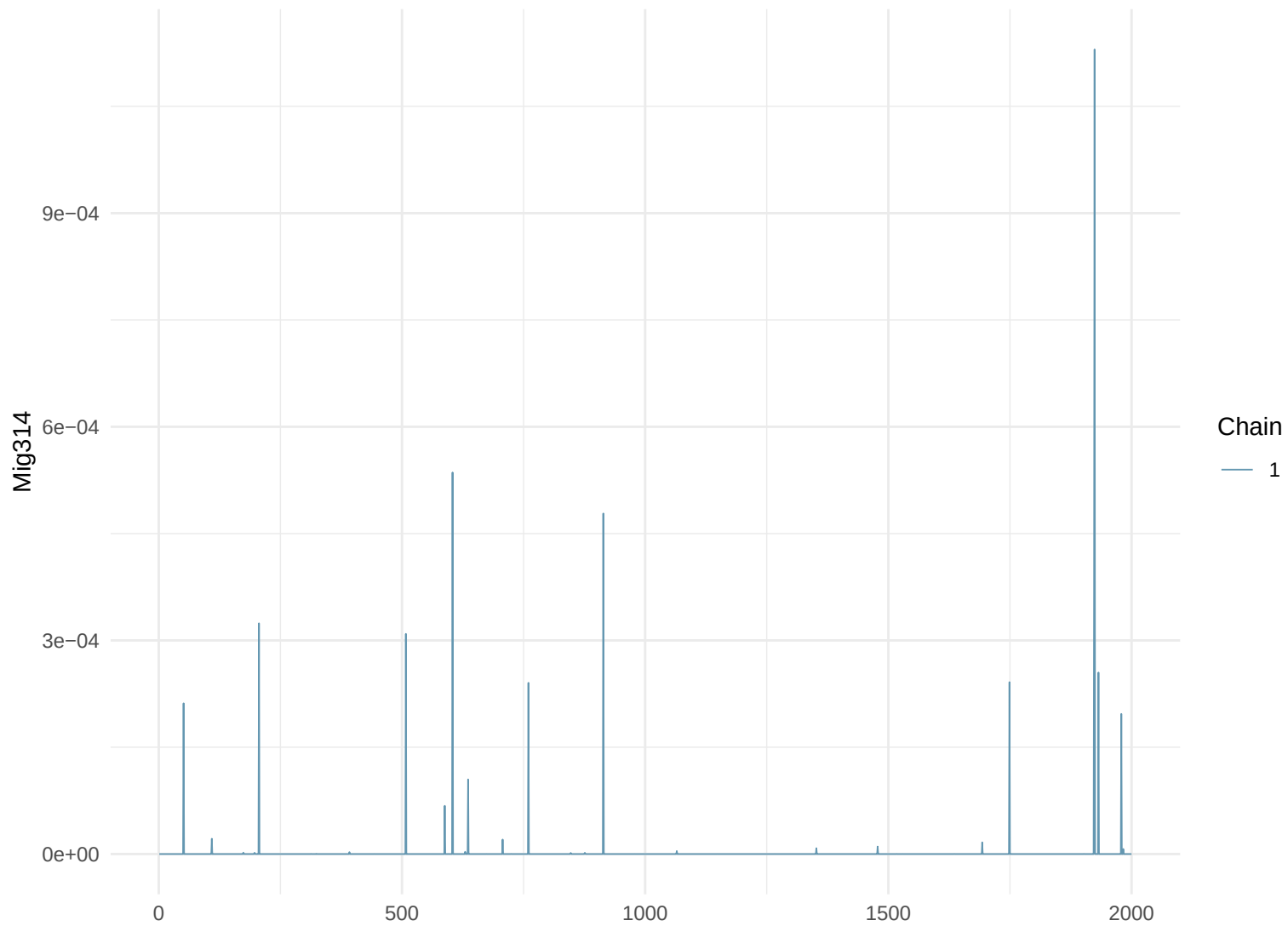
Trace Plot: Mig314
