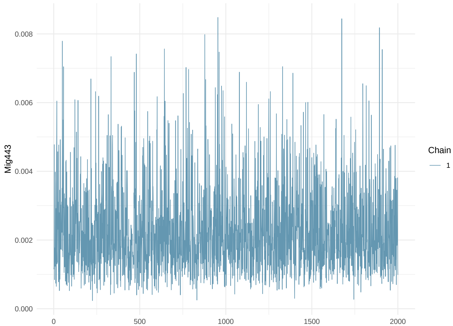
Trace Plot: Mig443
