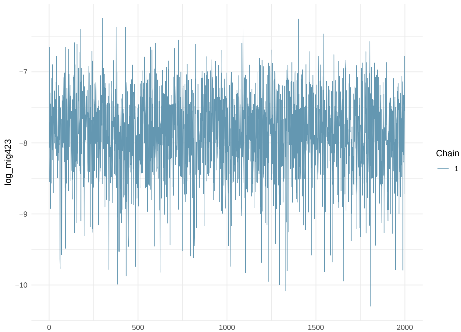
Trace Plot: log_mig423
