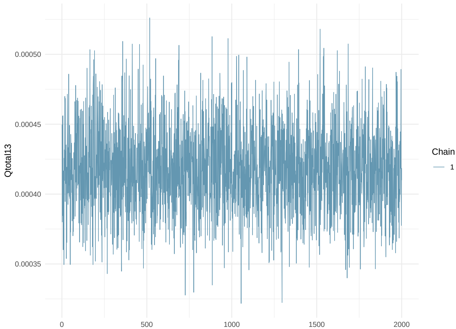
Trace Plot: Qtotal13
