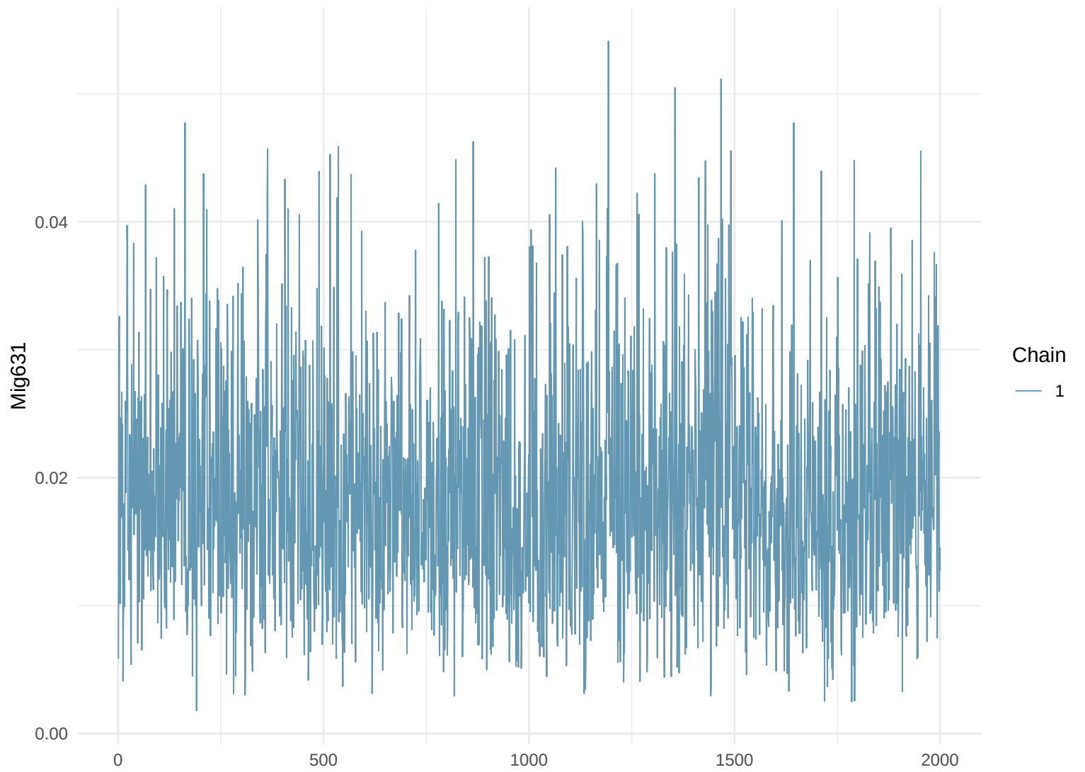
Trace Plot: Mig631
