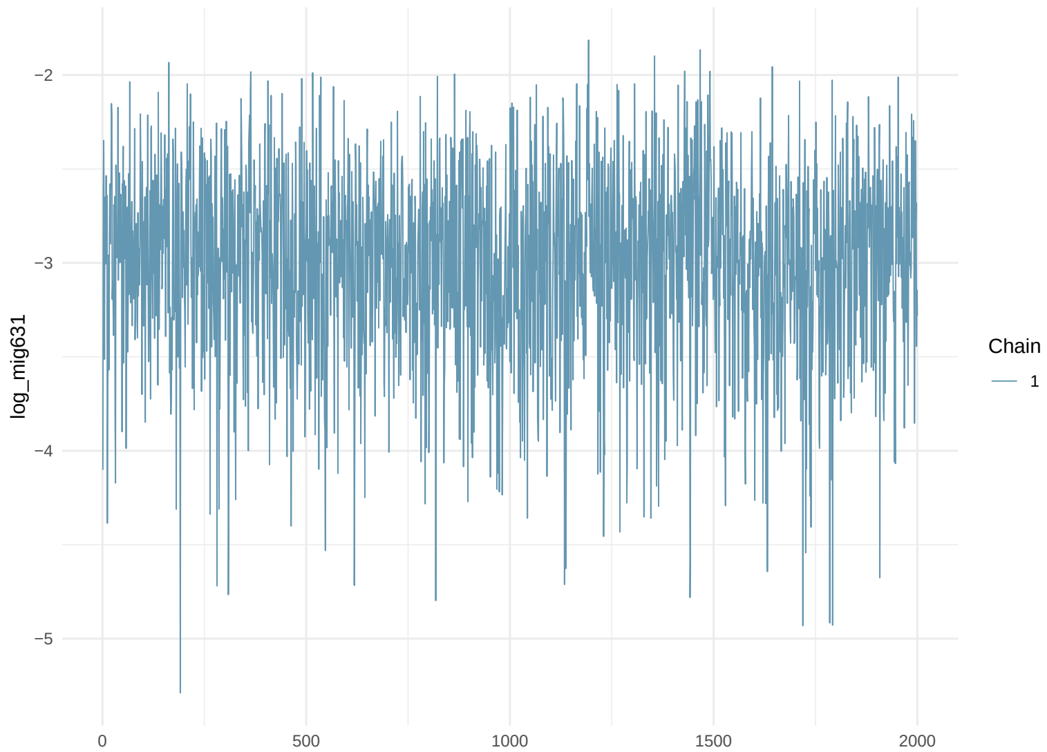
Trace Plot: log_mig631
