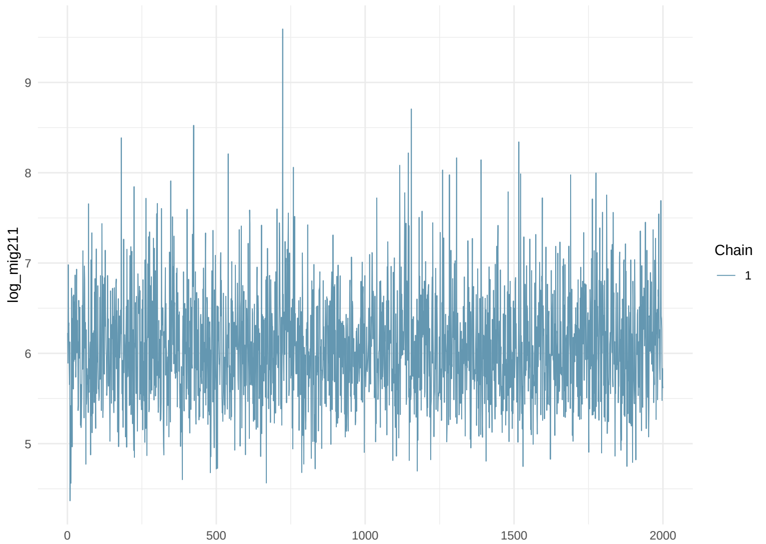
Trace Plot: log_mig211
