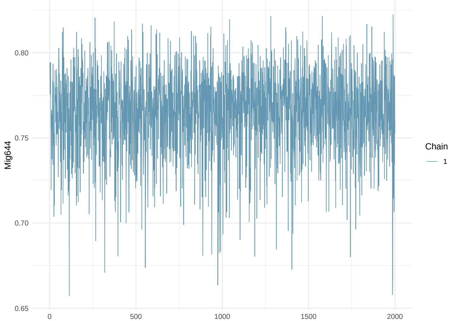
Trace Plot: Mig644
