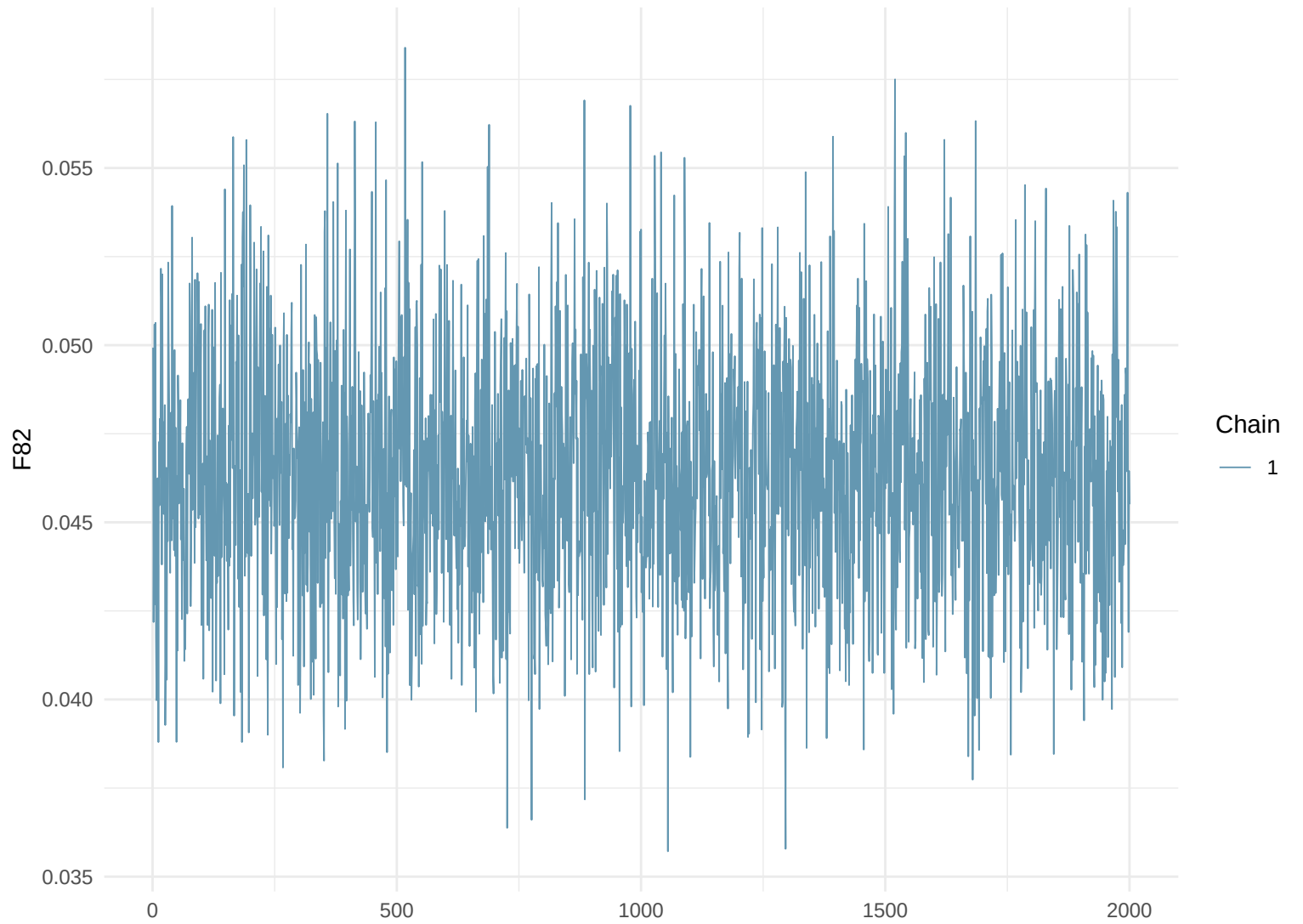
Trace Plot: F82
