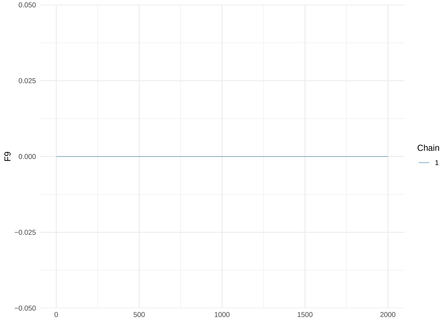
Trace Plot: F9
