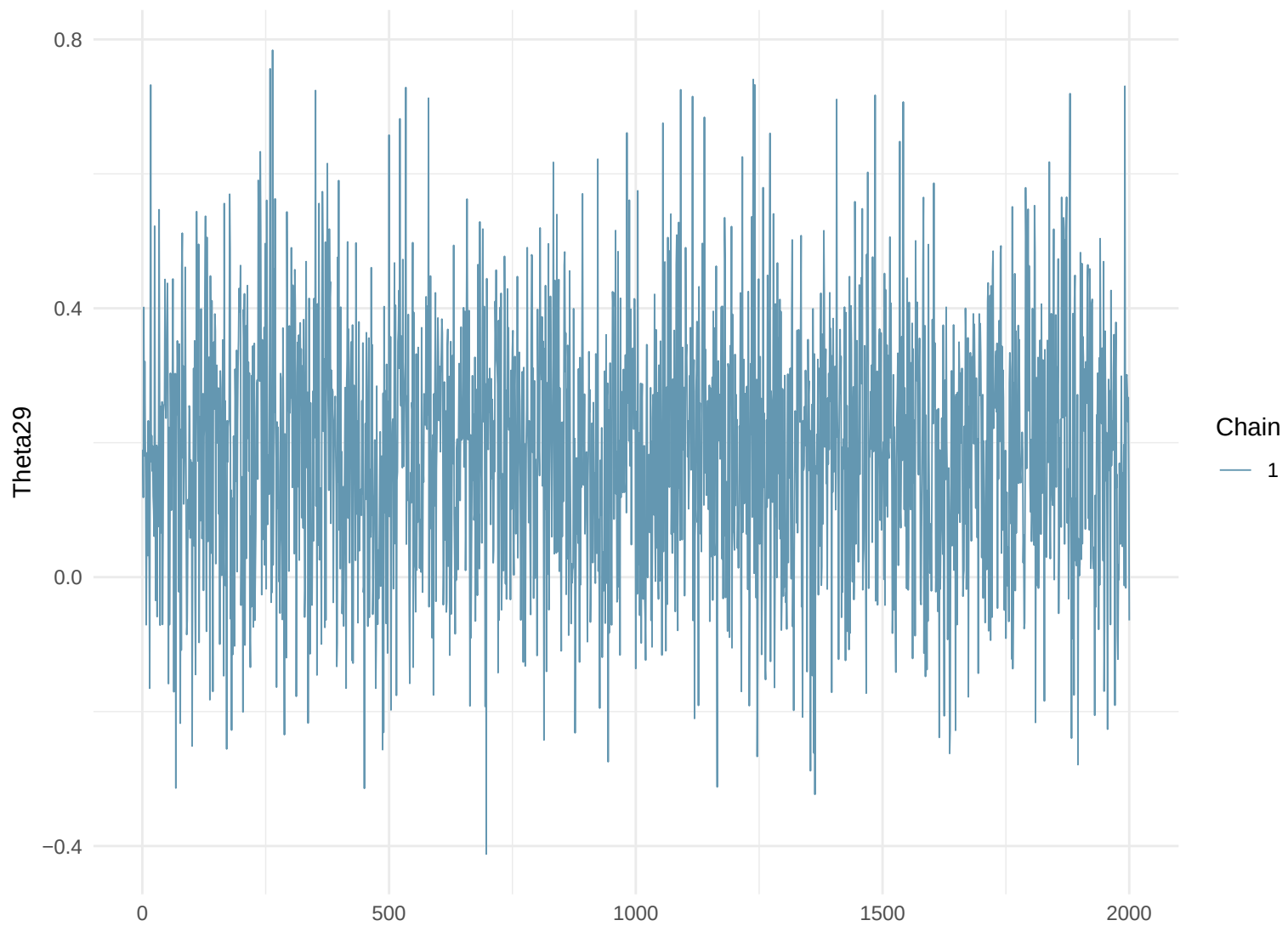
Trace Plot: Theta29
