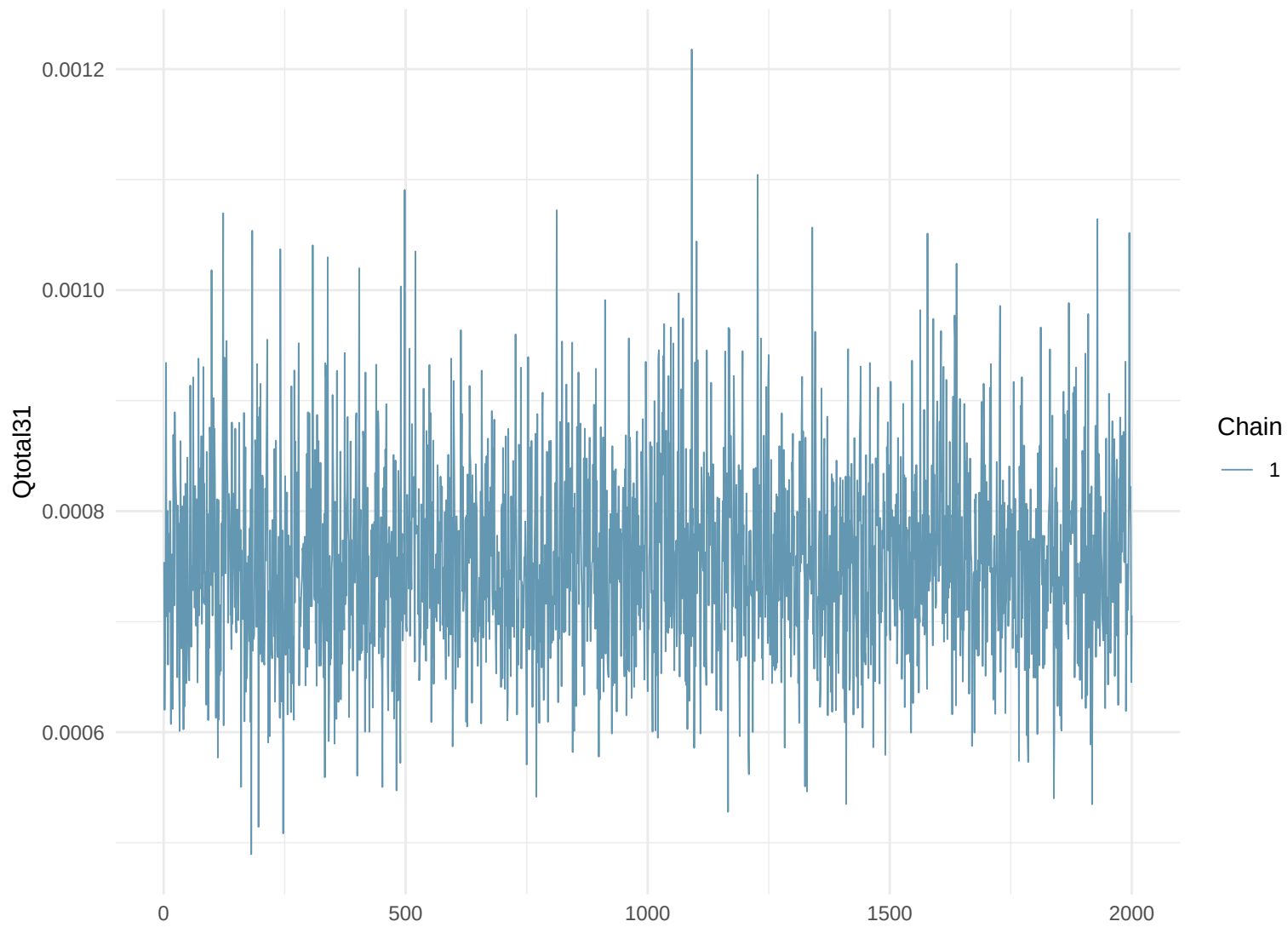
Trace Plot: Qtotal31
