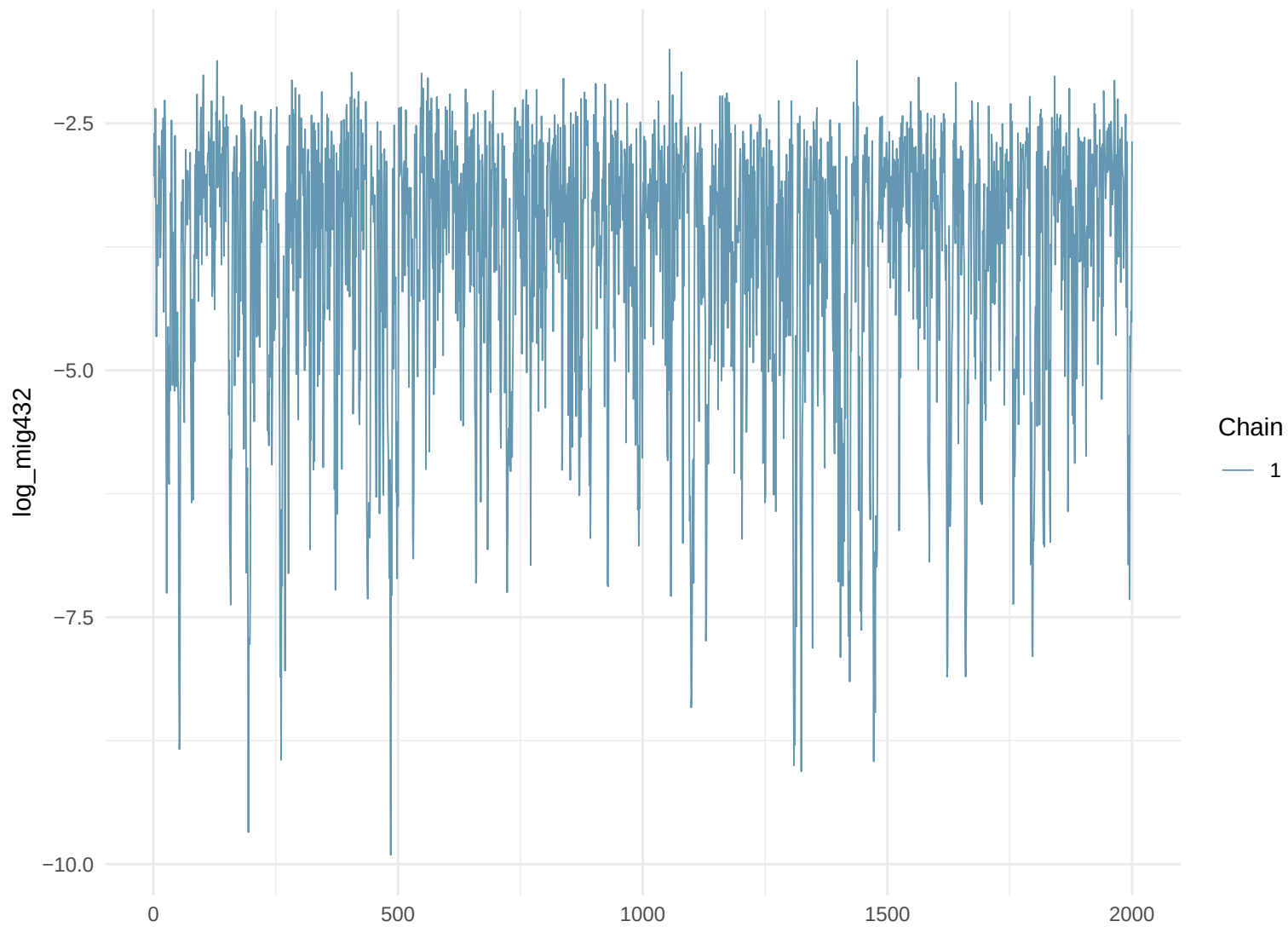
Trace Plot: log_mig432
