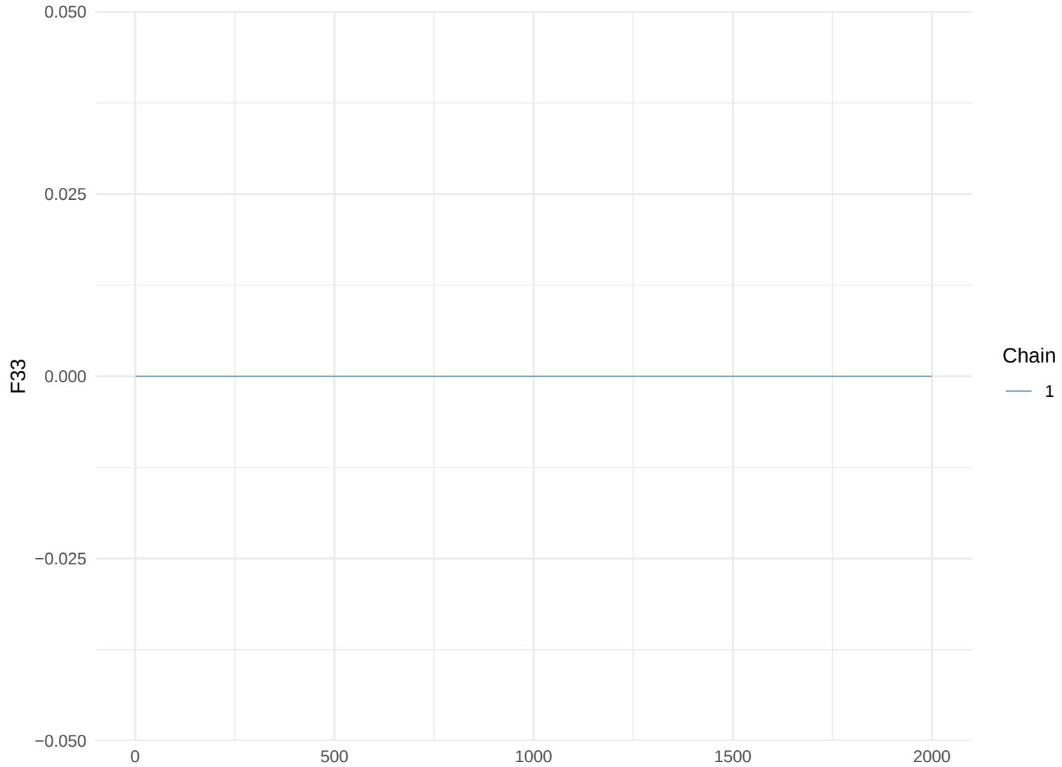
Trace Plot: F33
