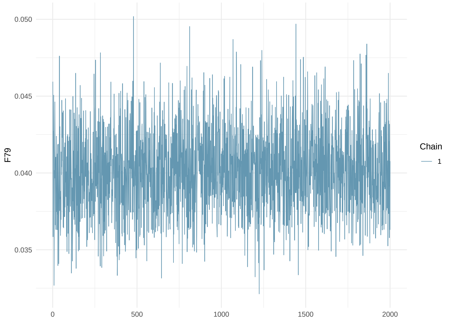
Trace Plot: F79
