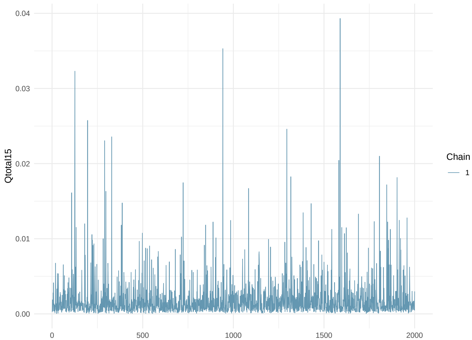
Trace Plot: Qtotal15
