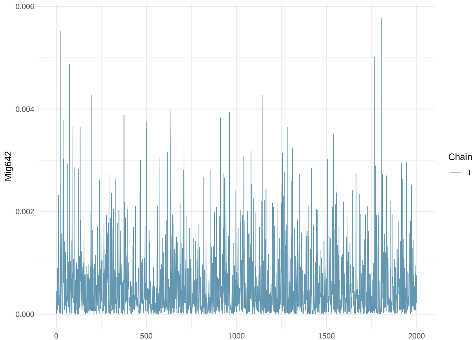
Trace Plot: Mig642
