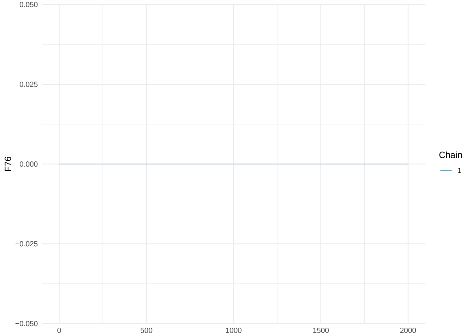
Trace Plot: F76
