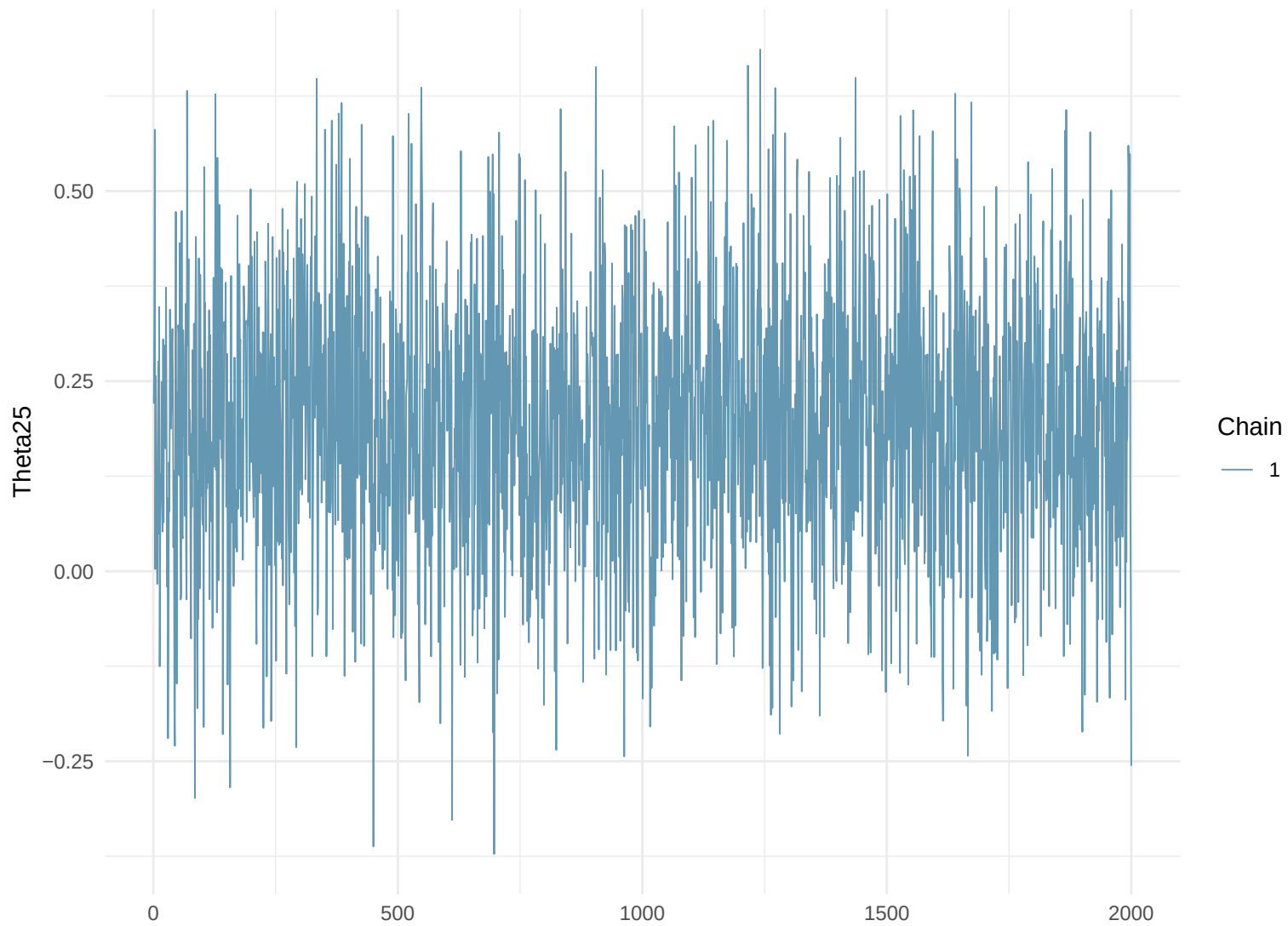
Trace Plot: Theta25
