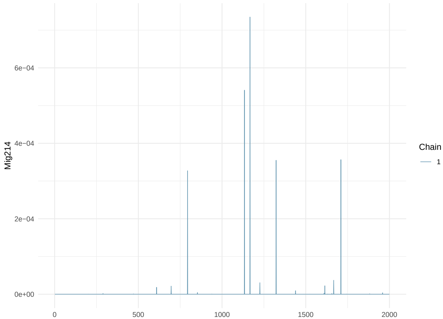
Trace Plot: Mig214
