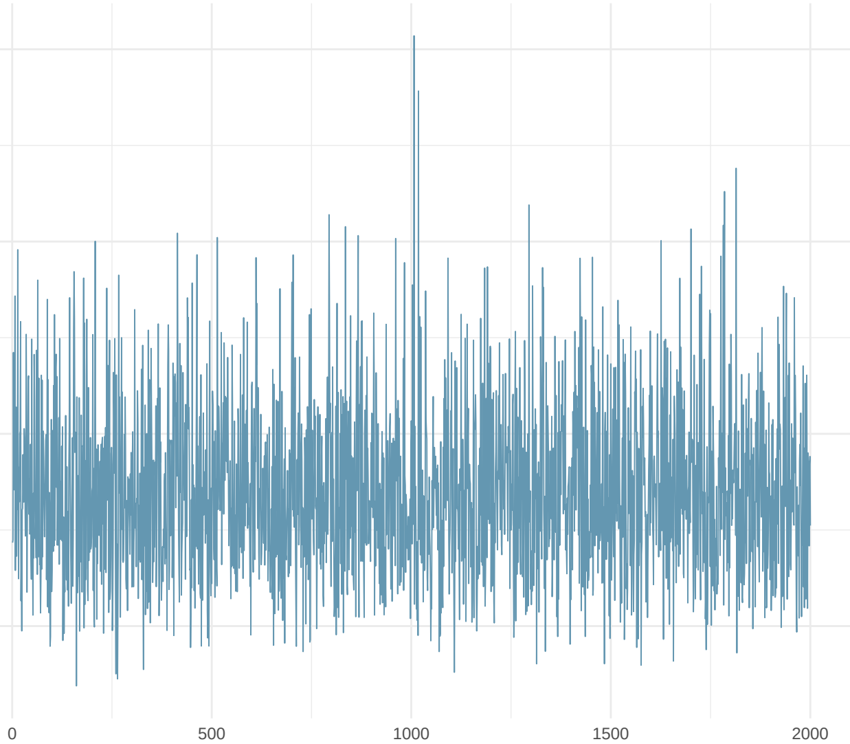
Trace Plot: Mig634
