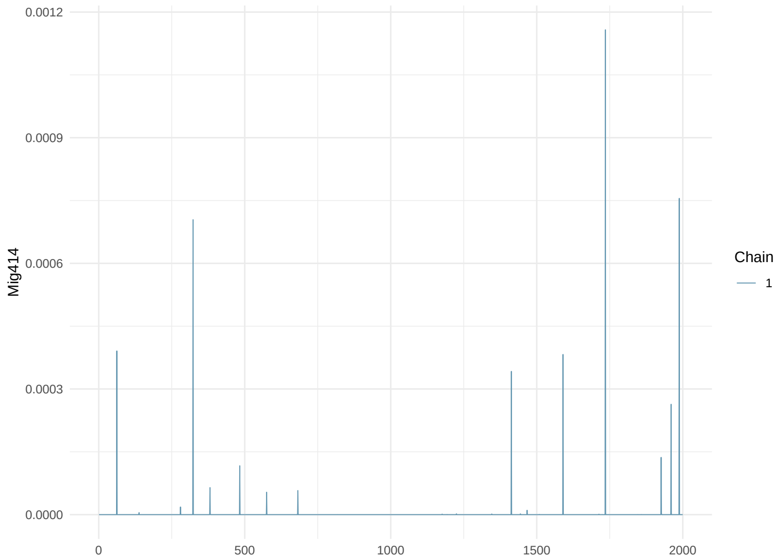
Trace Plot: Mig414
