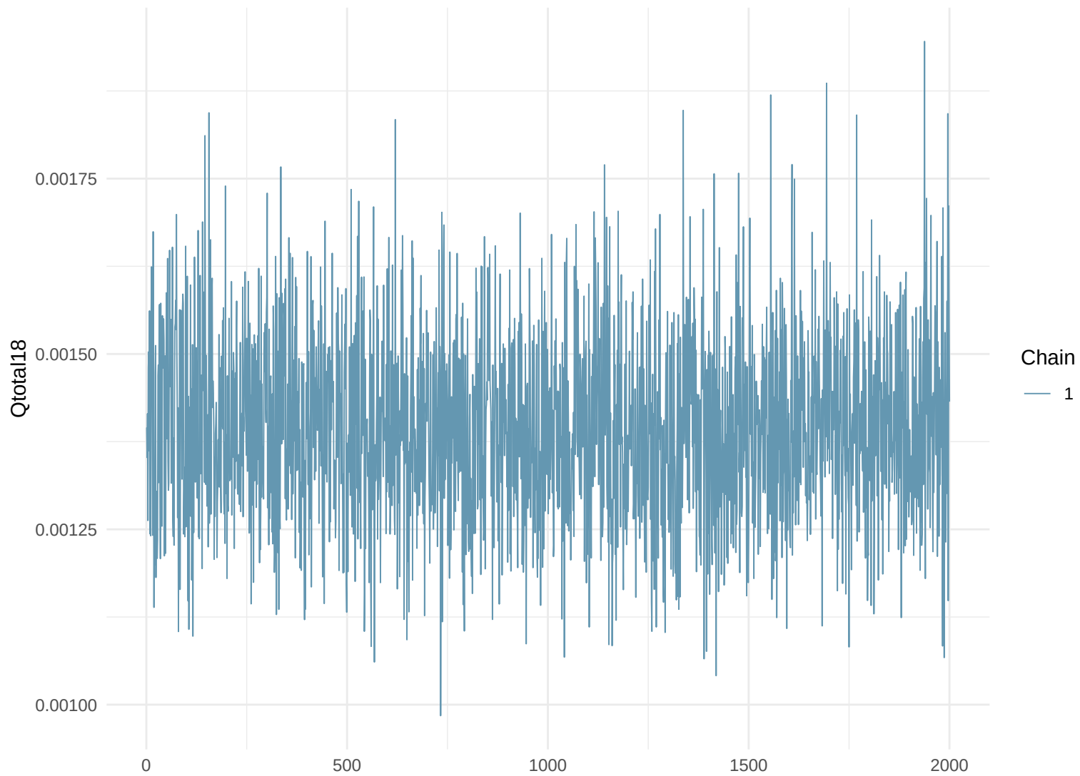
Trace Plot: Qtotal18
