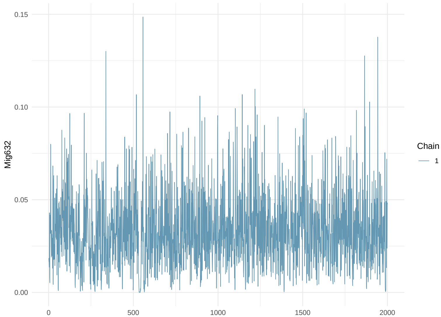
Trace Plot: Mig632
