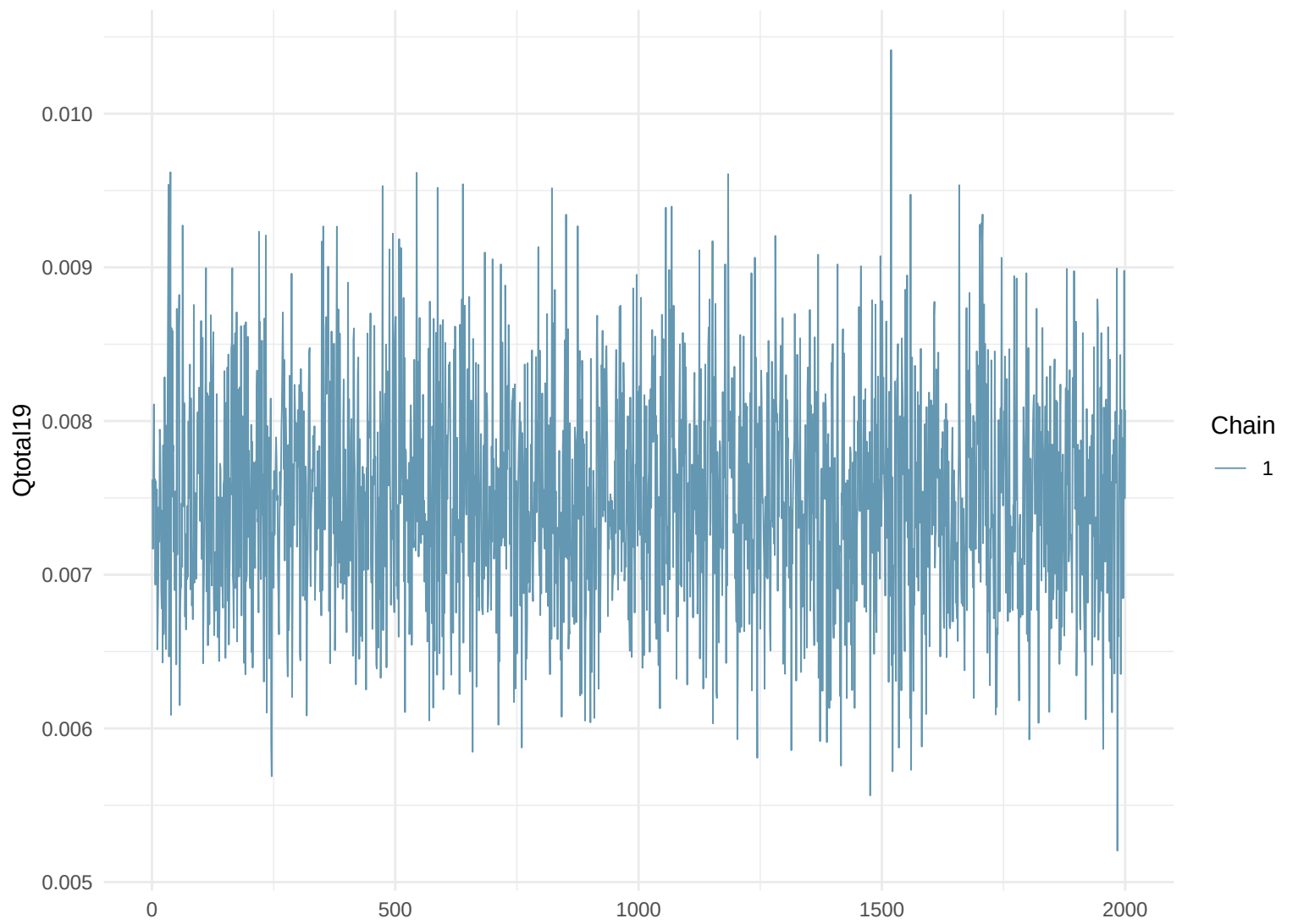
Trace Plot: Qtotal19
