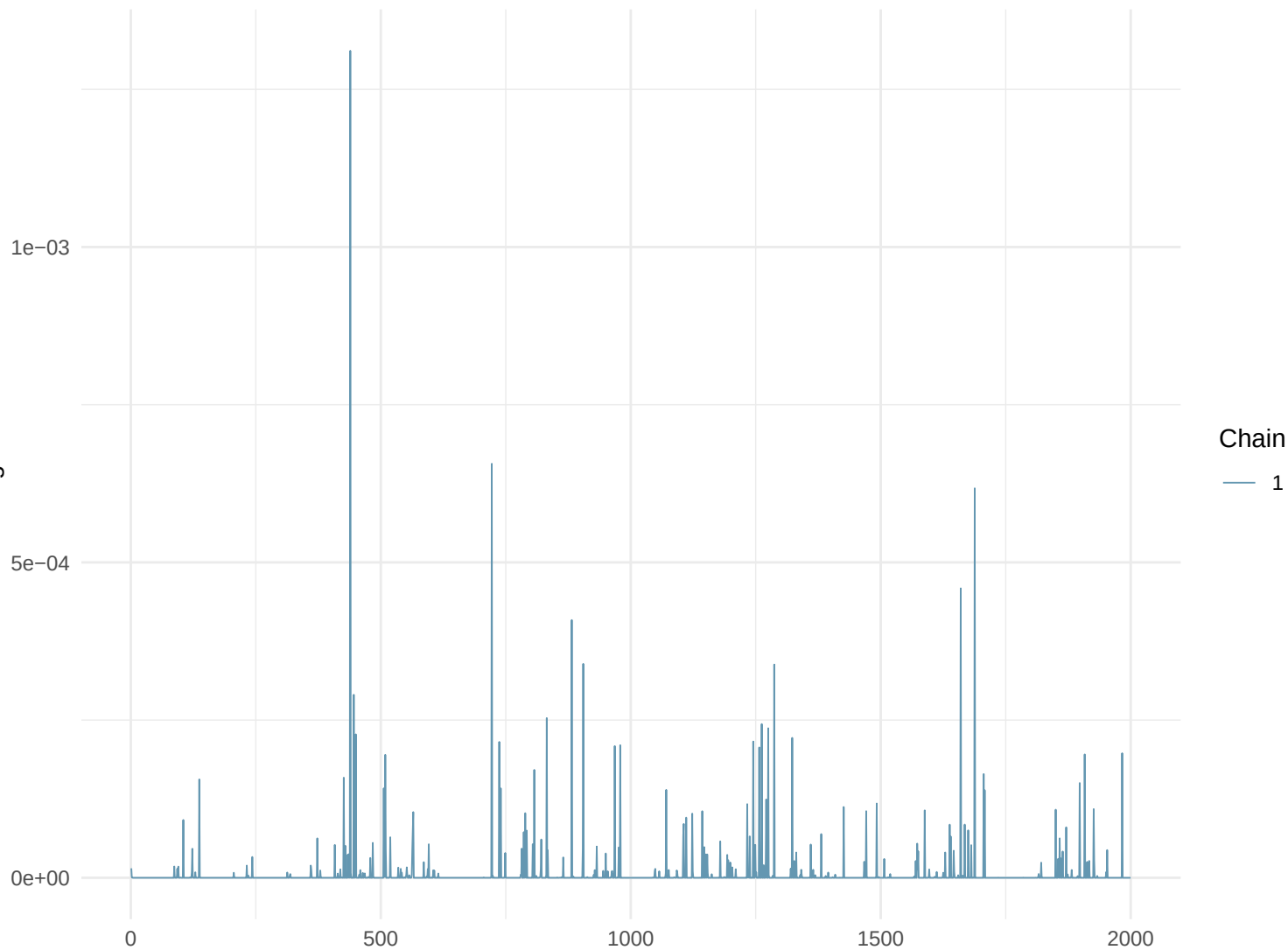
Trace Plot: Mig324
