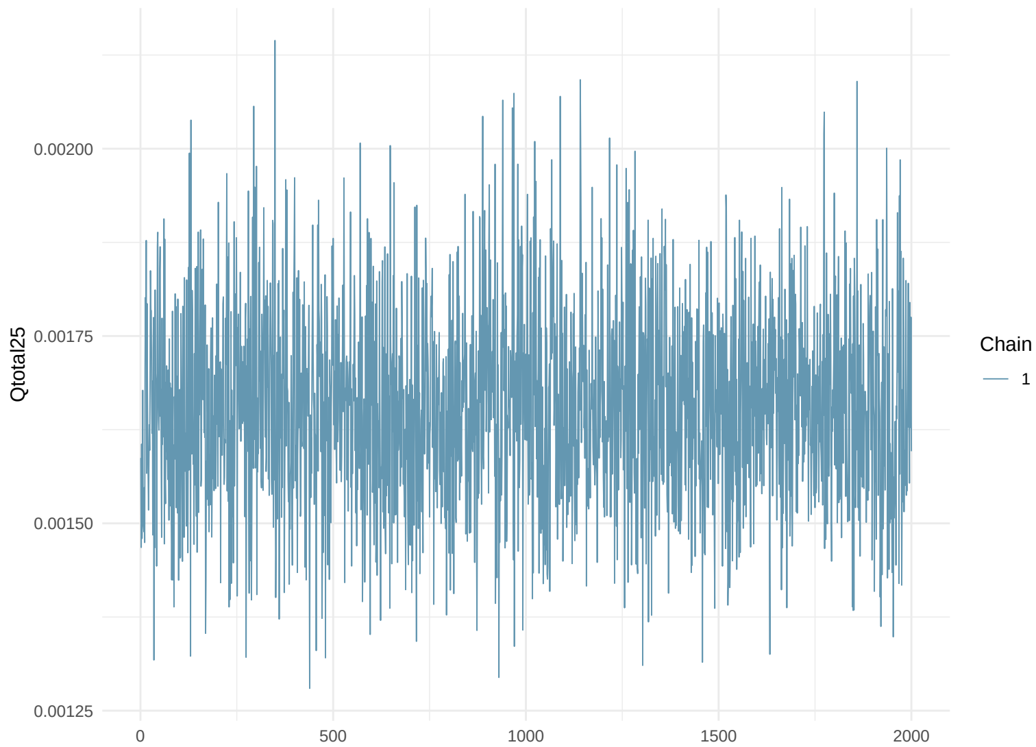
Trace Plot: Qtotal25
