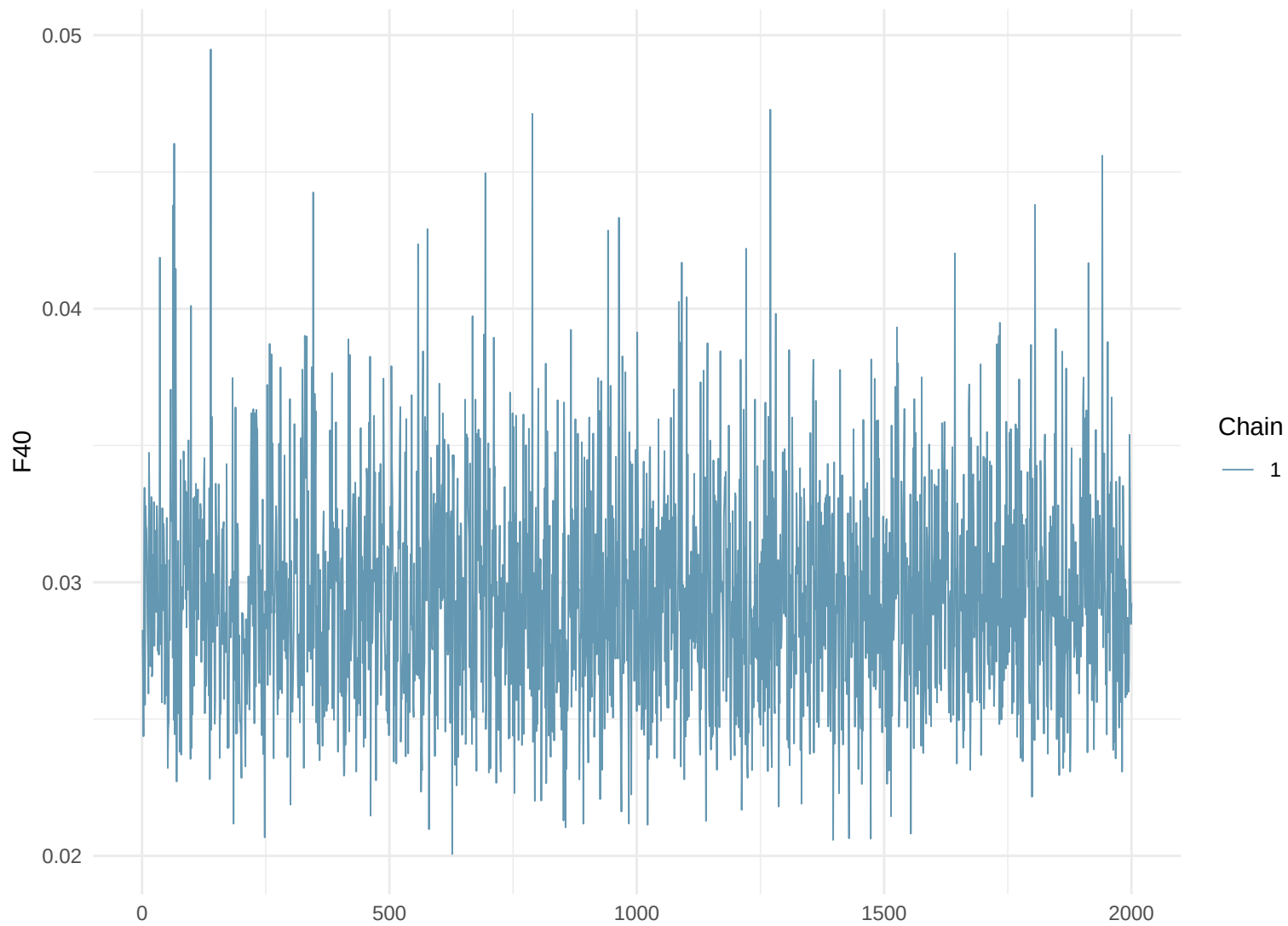
Trace Plot: F40
