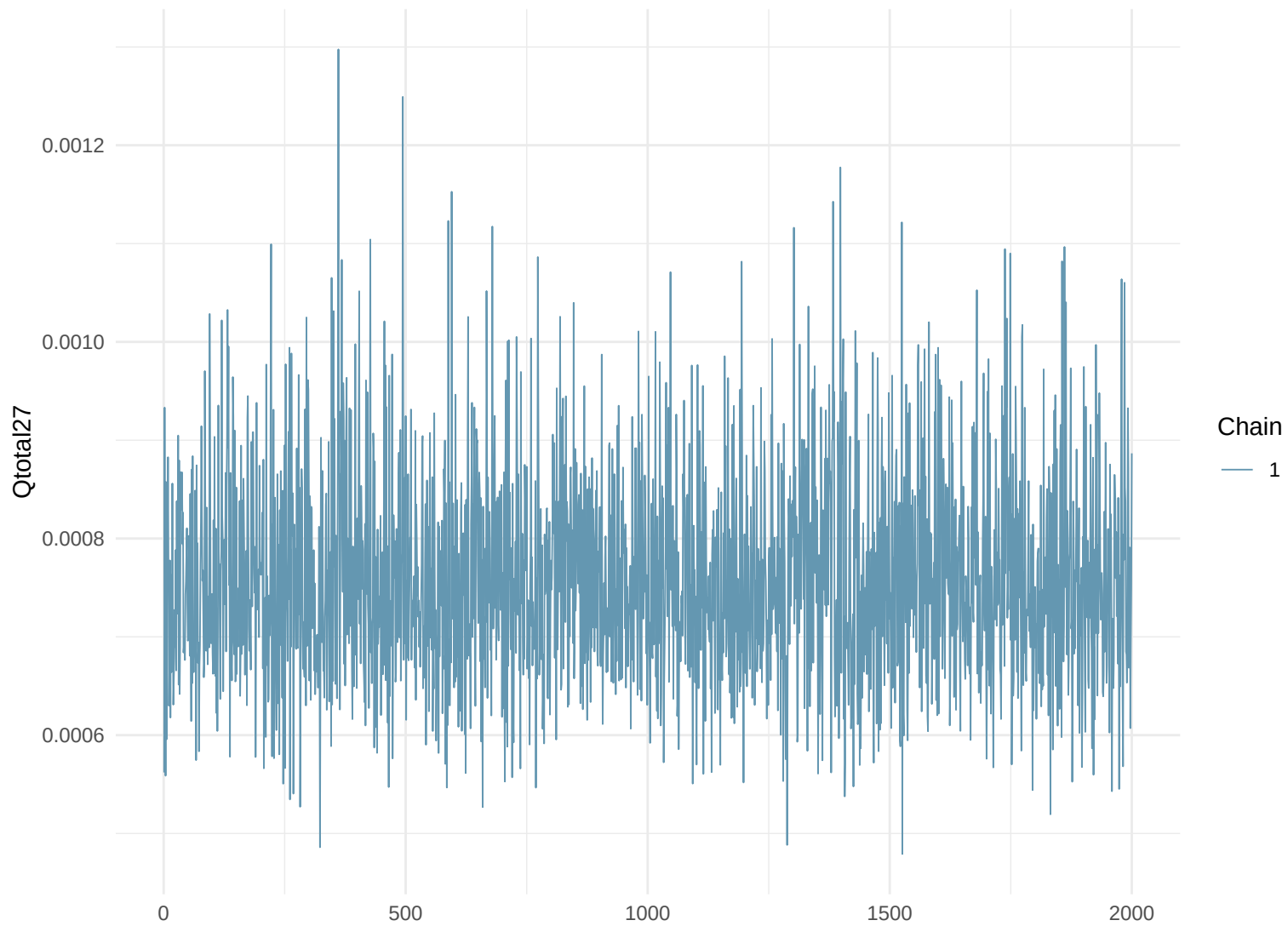
Trace Plot: Qtotal27
