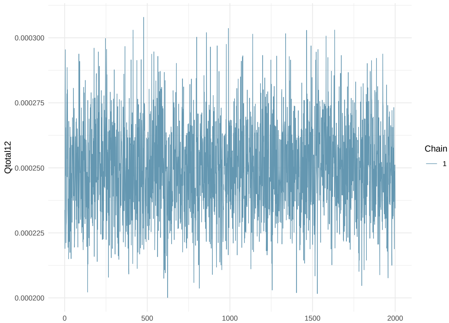
Trace Plot: Qtotal12
