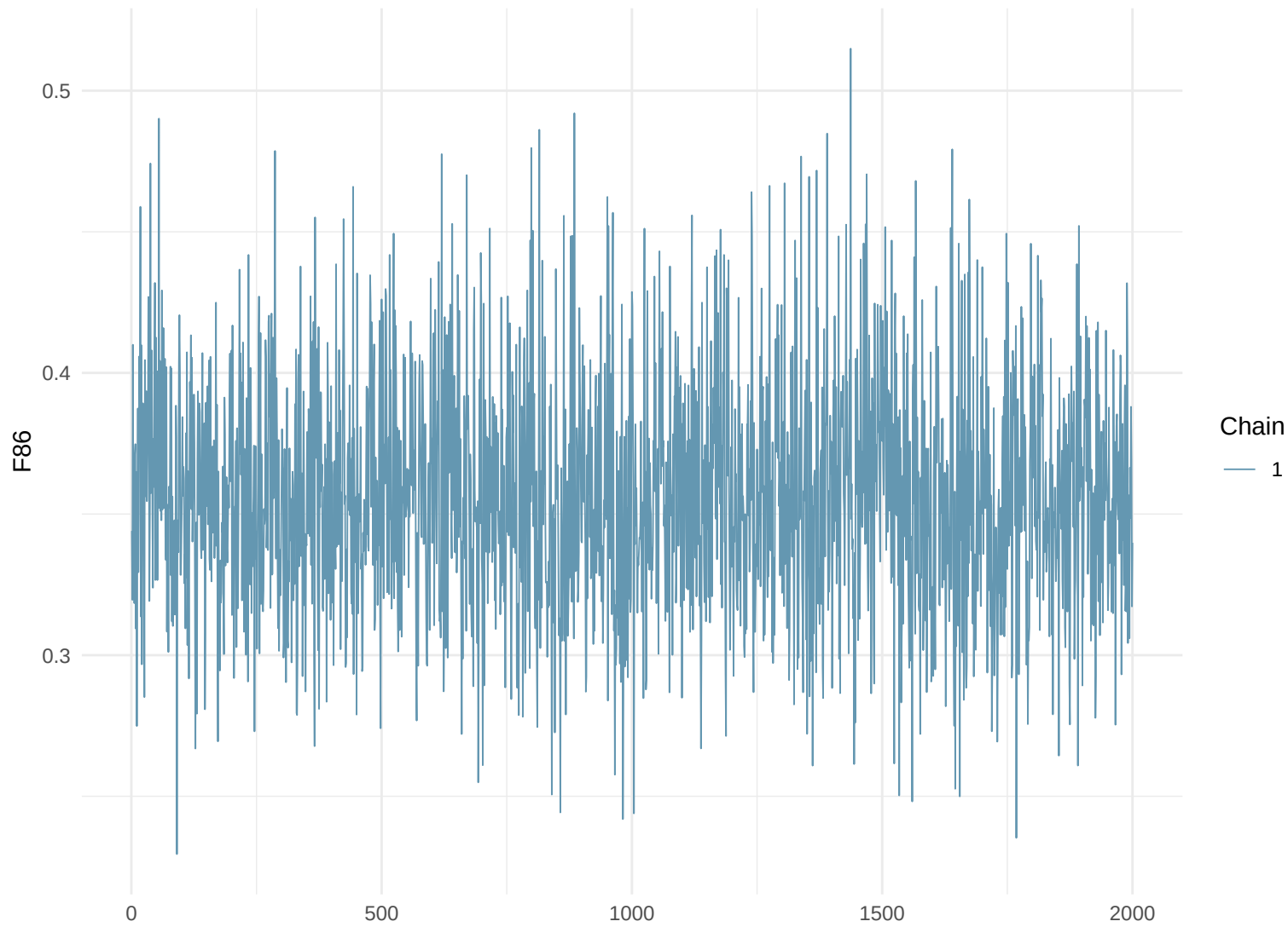
Trace Plot: F86
