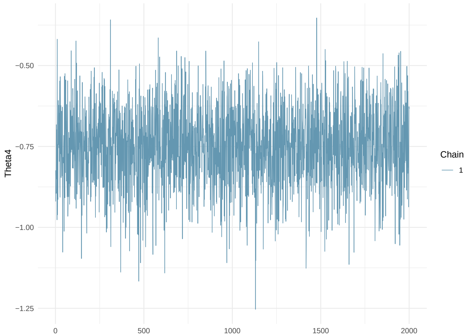
Trace Plot: Theta4
