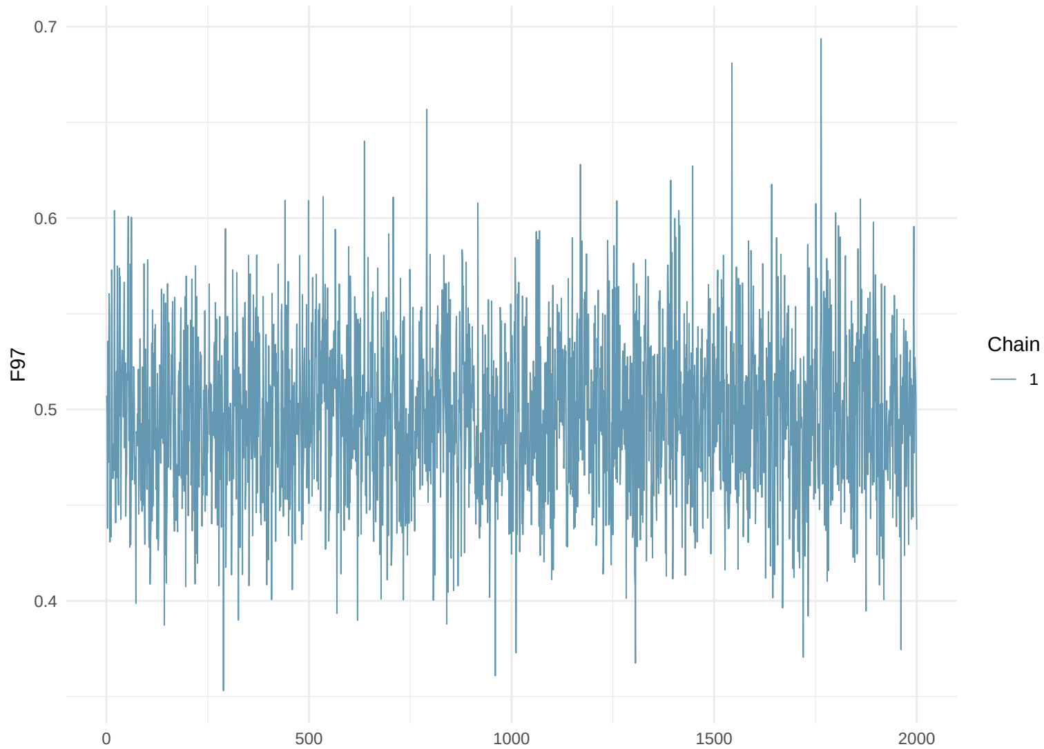
Trace Plot: F97
