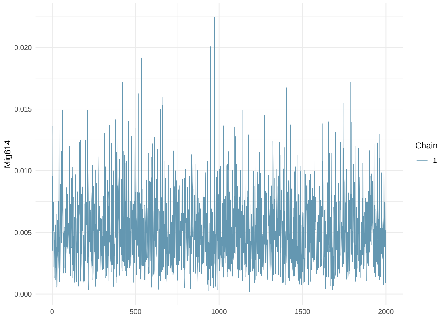
Trace Plot: Mig614
