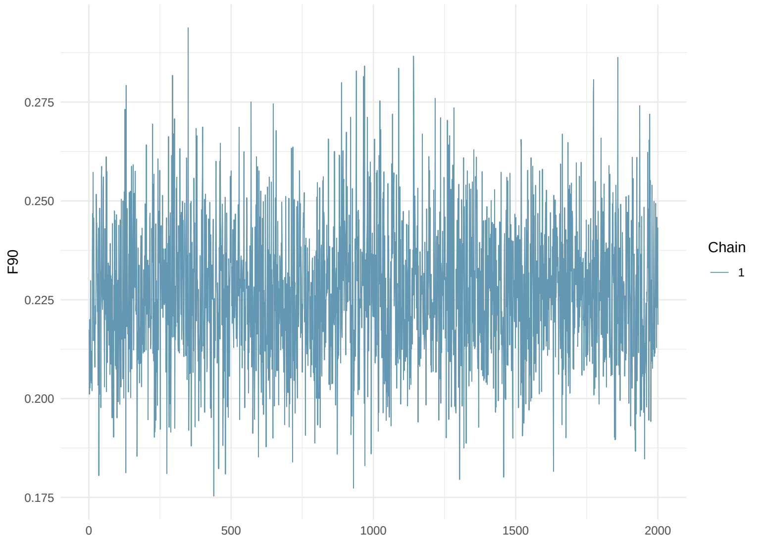
Trace Plot: F90
