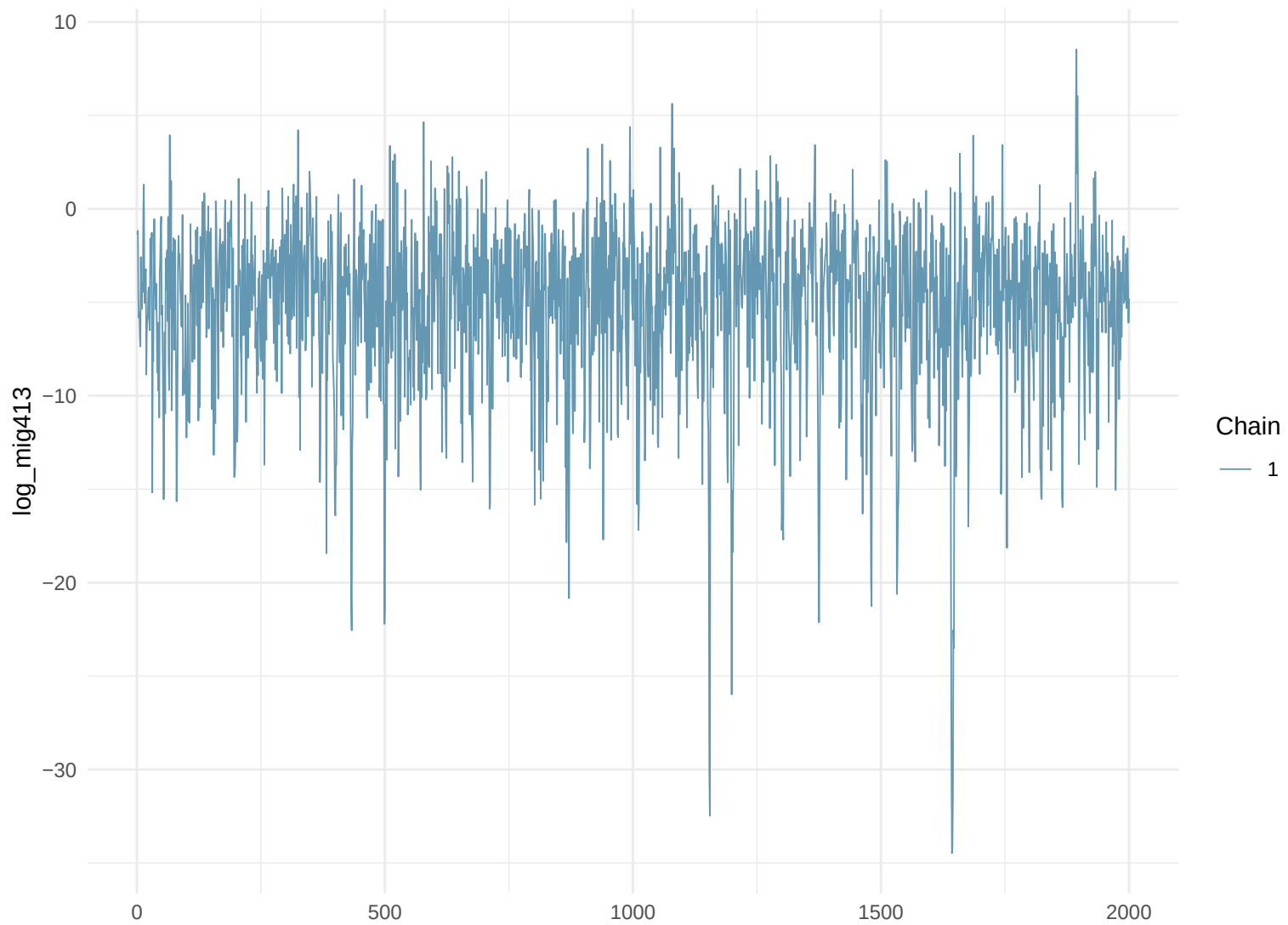
Trace Plot: log_mig413
