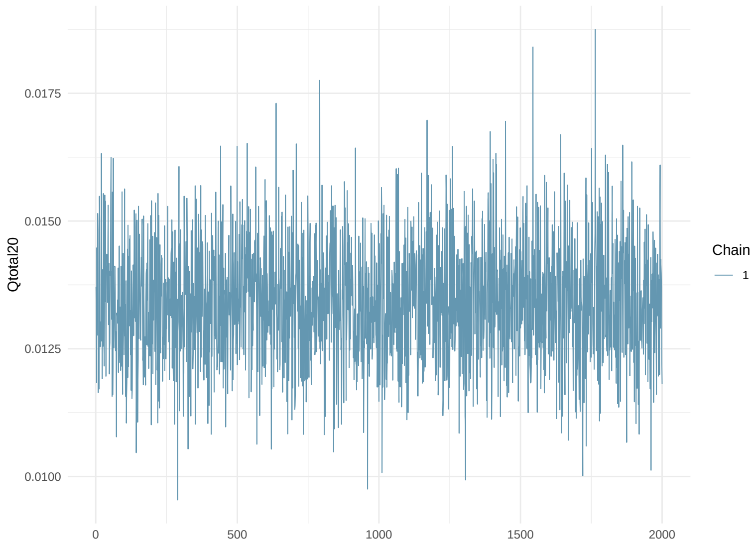
Trace Plot: Qtotal20
