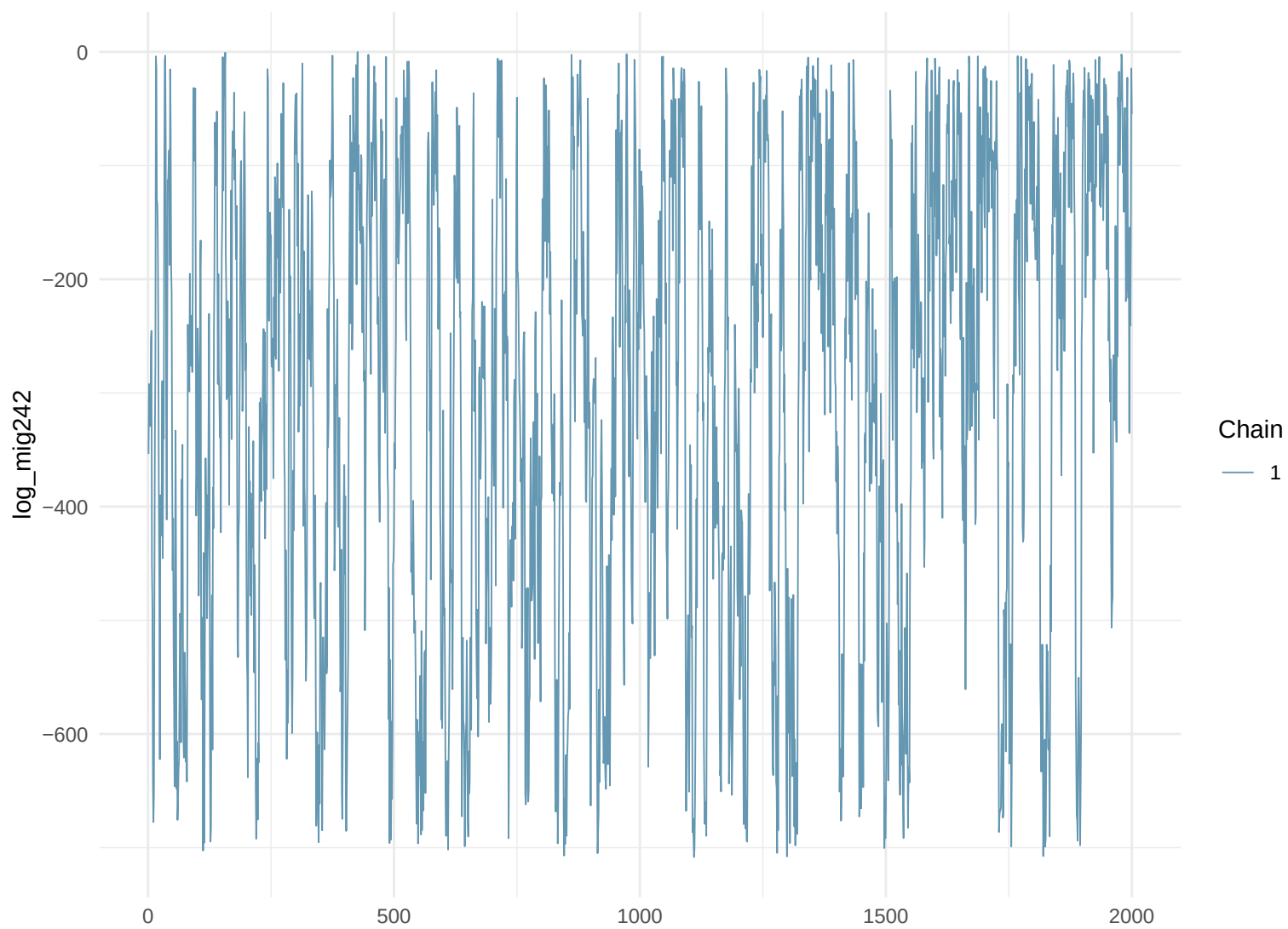
Trace Plot: log_mig242
