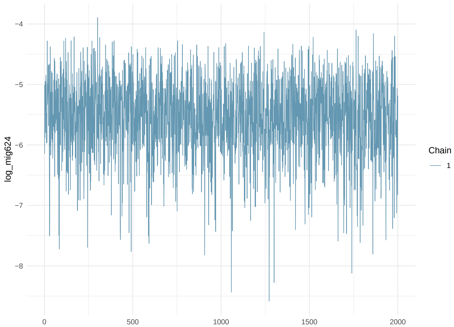
Trace Plot: log_mig624
