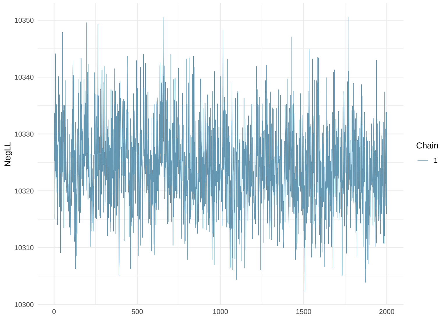
Trace Plot: NegLL
