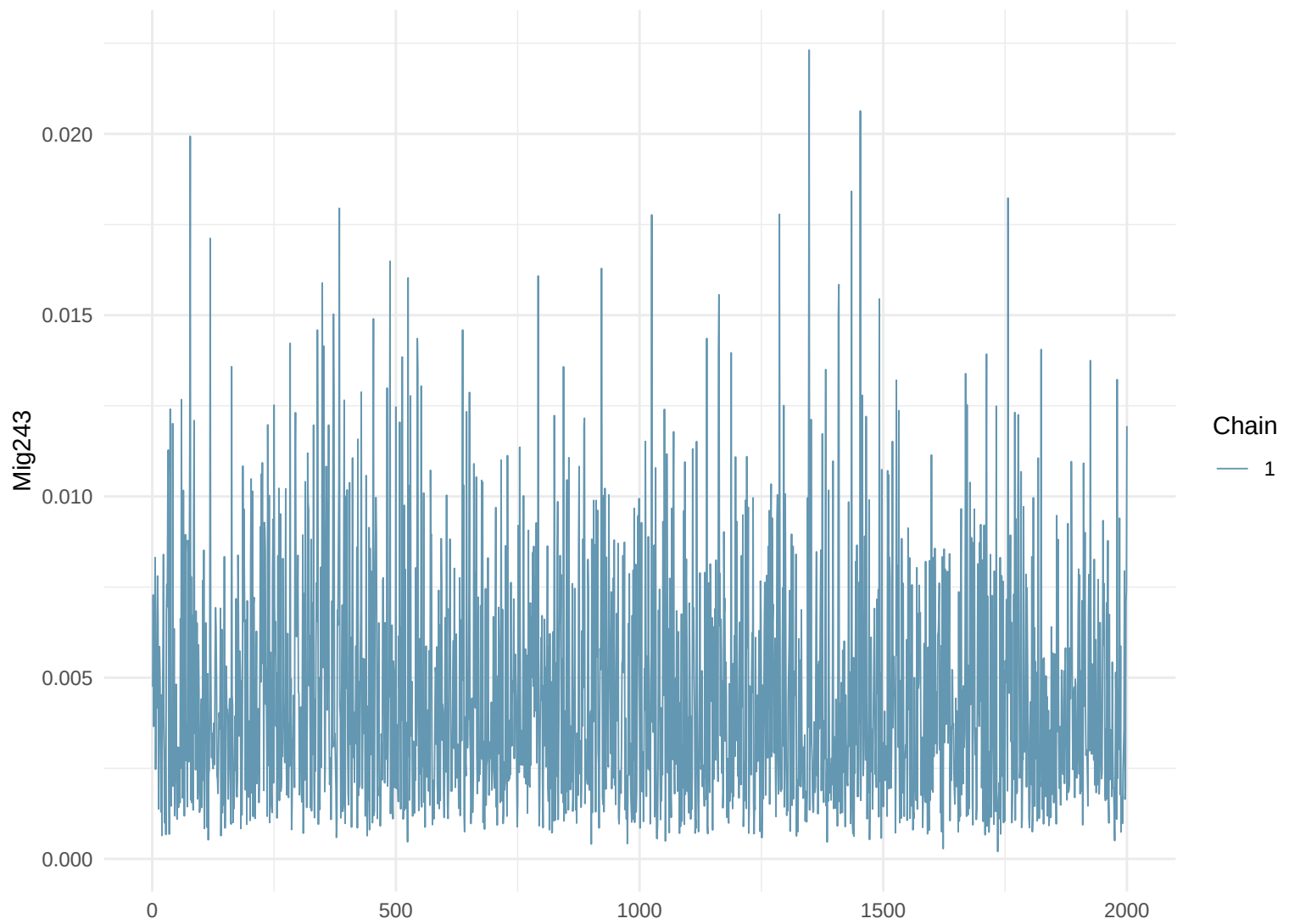
Trace Plot: Mig243
