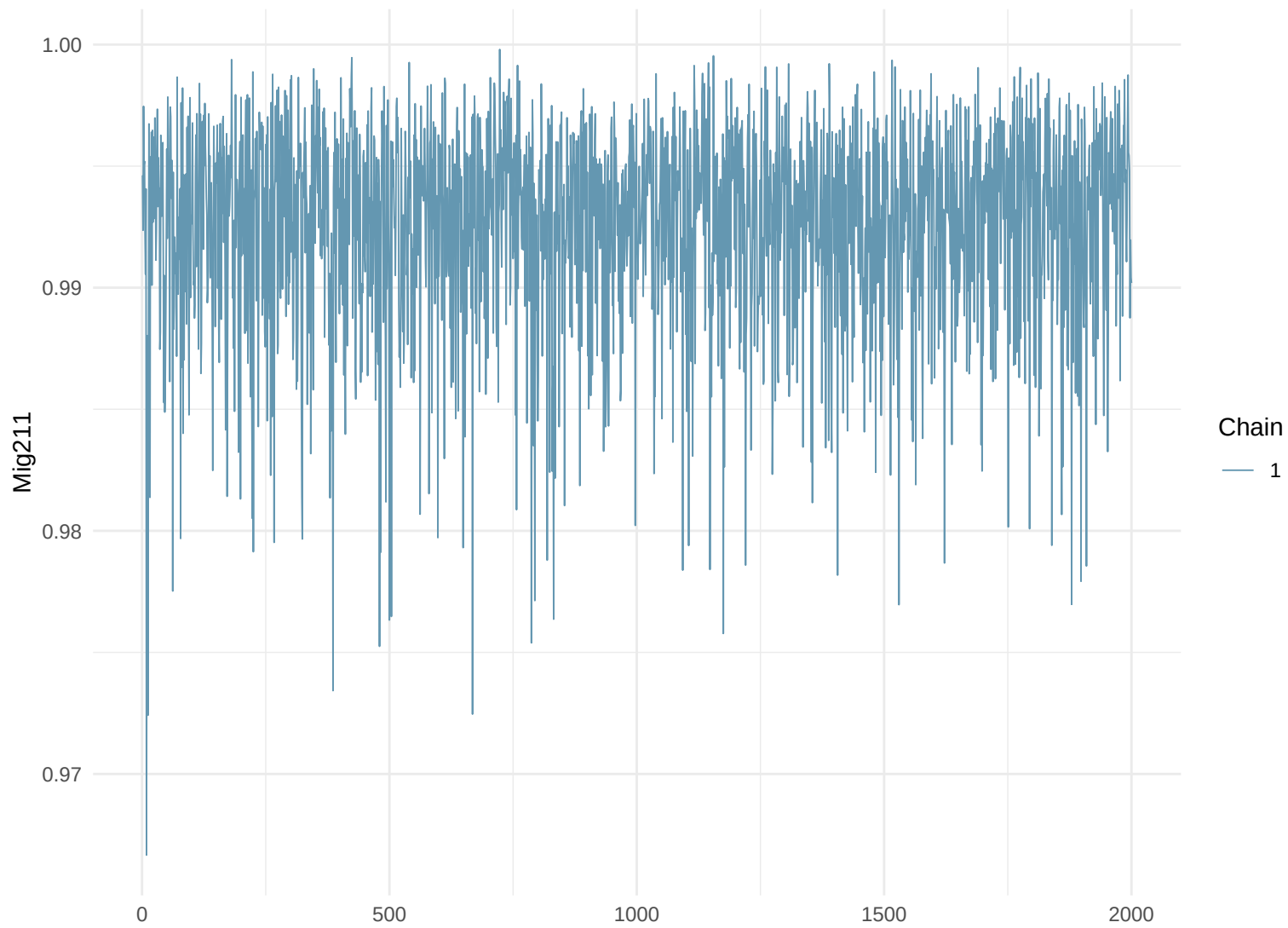
Trace Plot: Mig211
