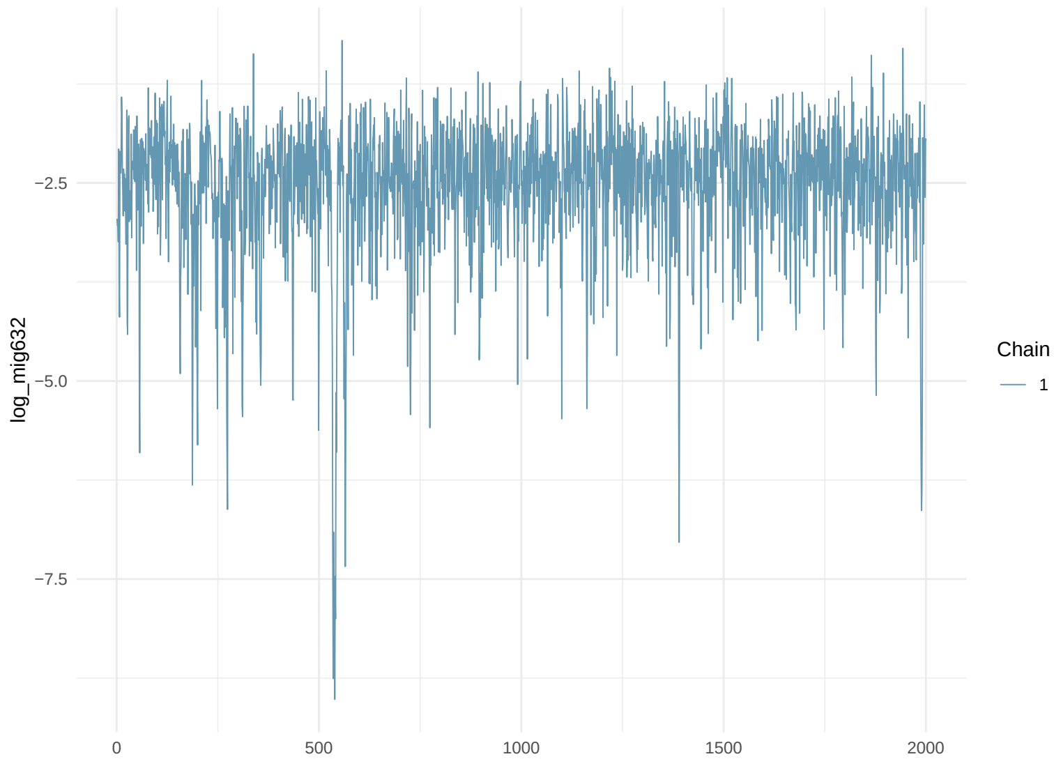
Trace Plot: log_mig632
