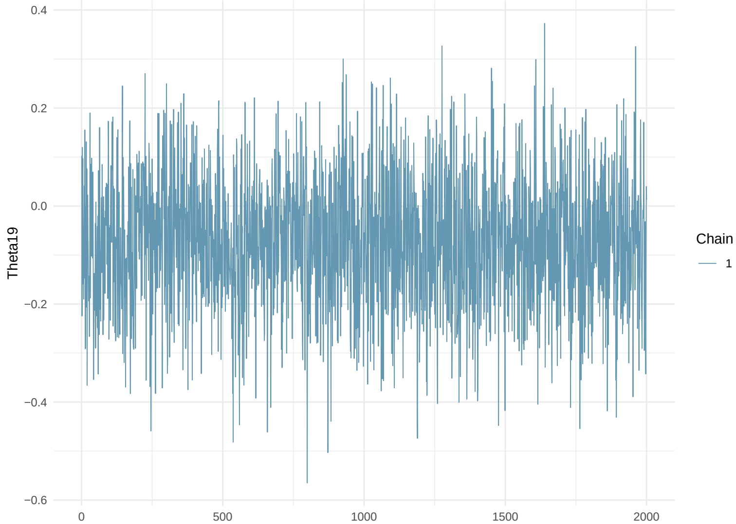
Trace Plot: Theta19
