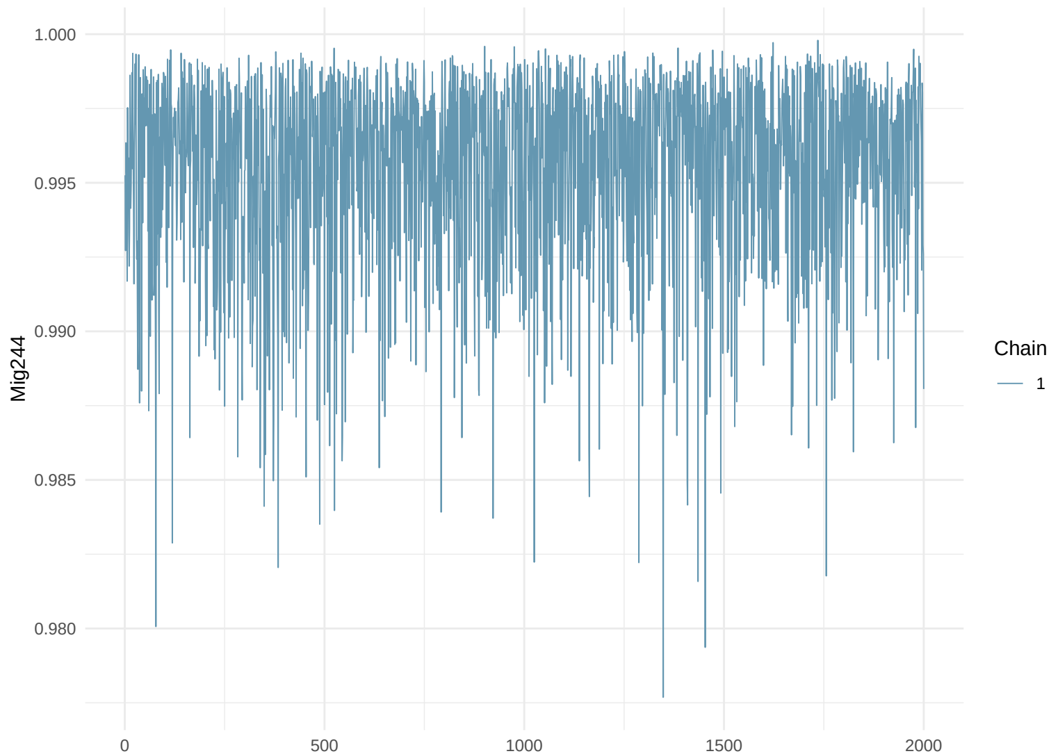
Trace Plot: Mig244
