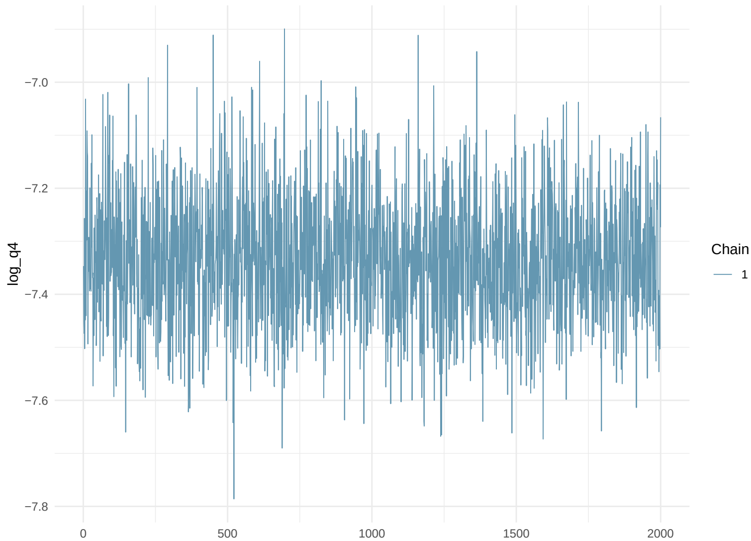
Trace Plot: log_q4
