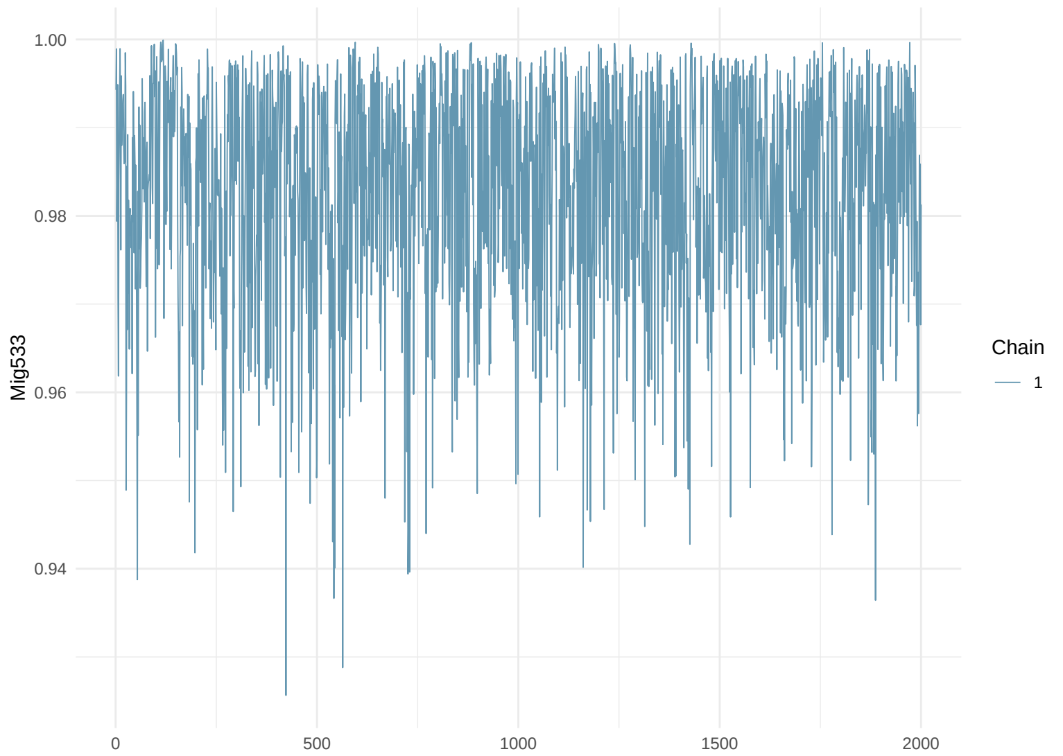
Trace Plot: Mig533
