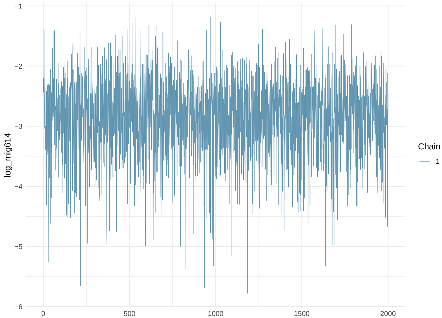
Trace Plot: log_mig614
