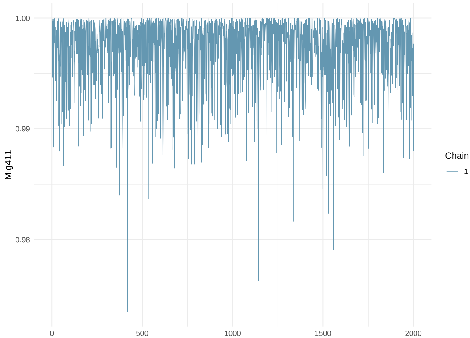
Trace Plot: Mig411
