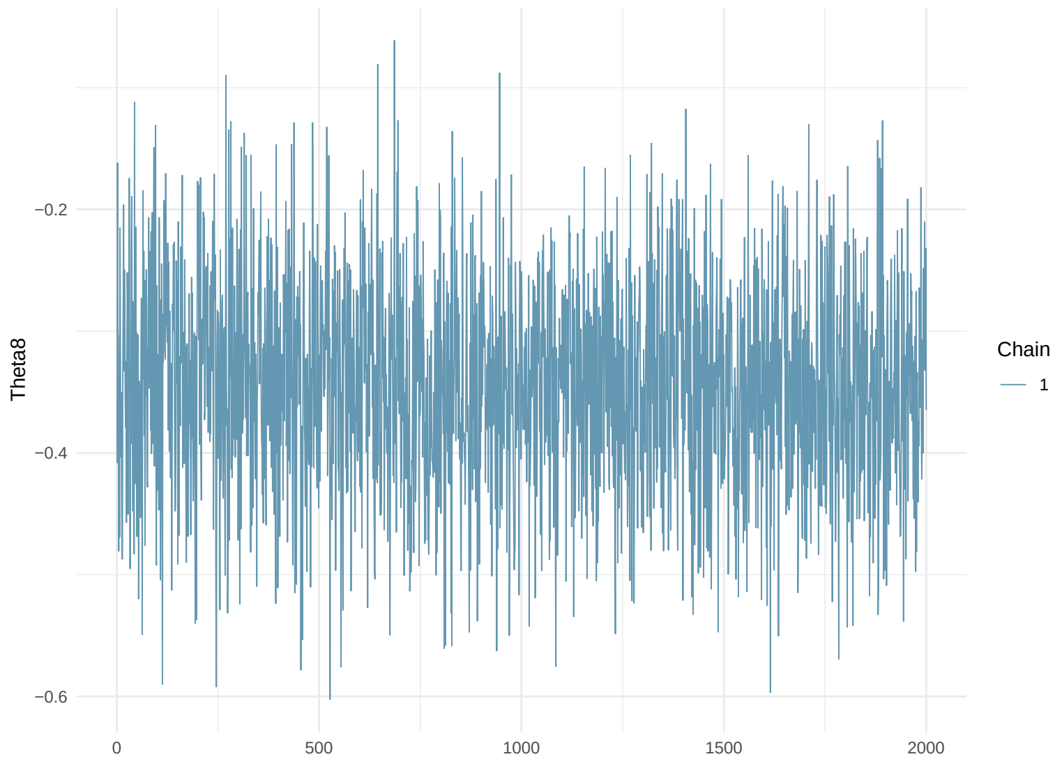
Trace Plot: Theta8
