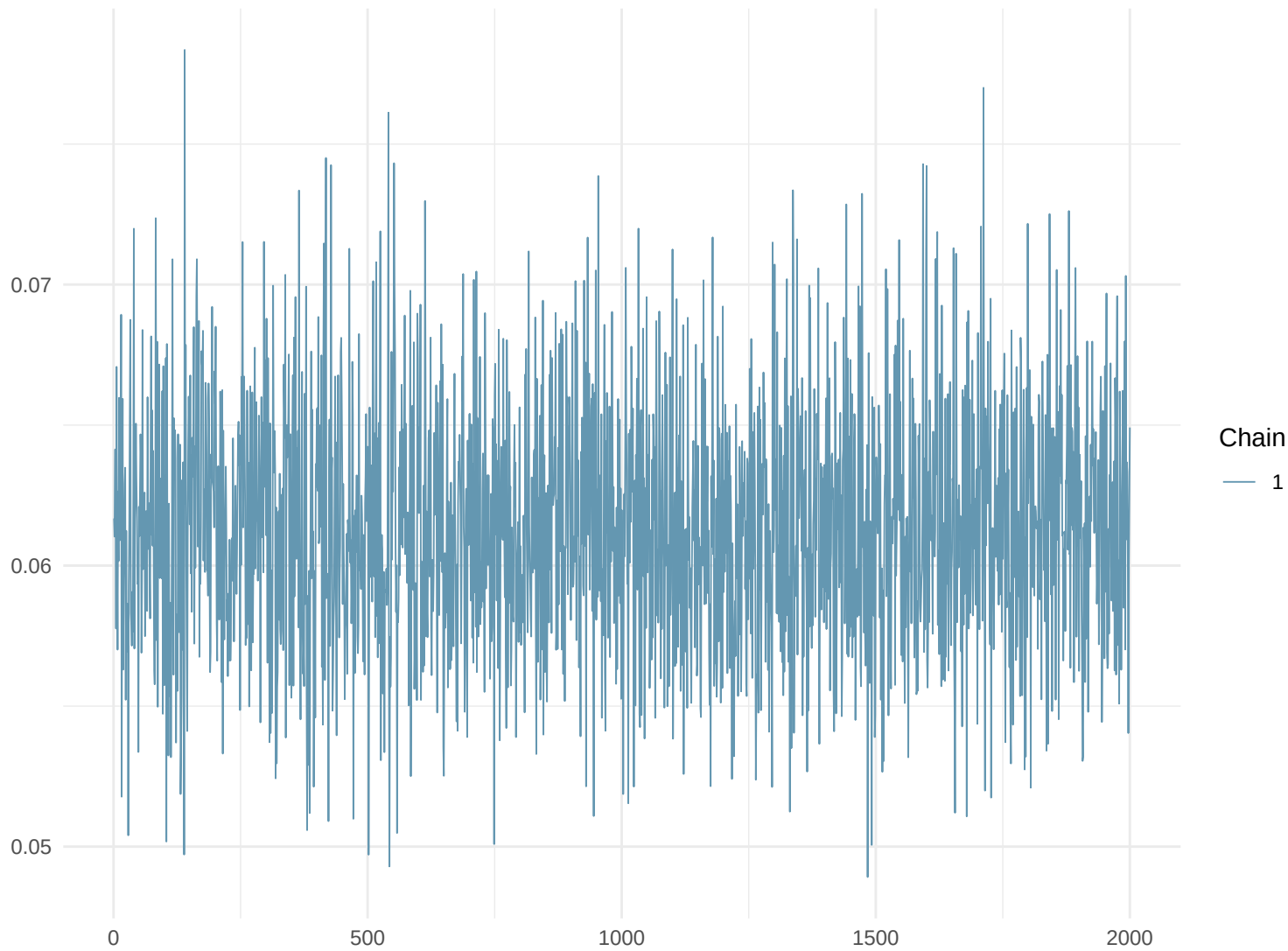
Trace Plot: F44
