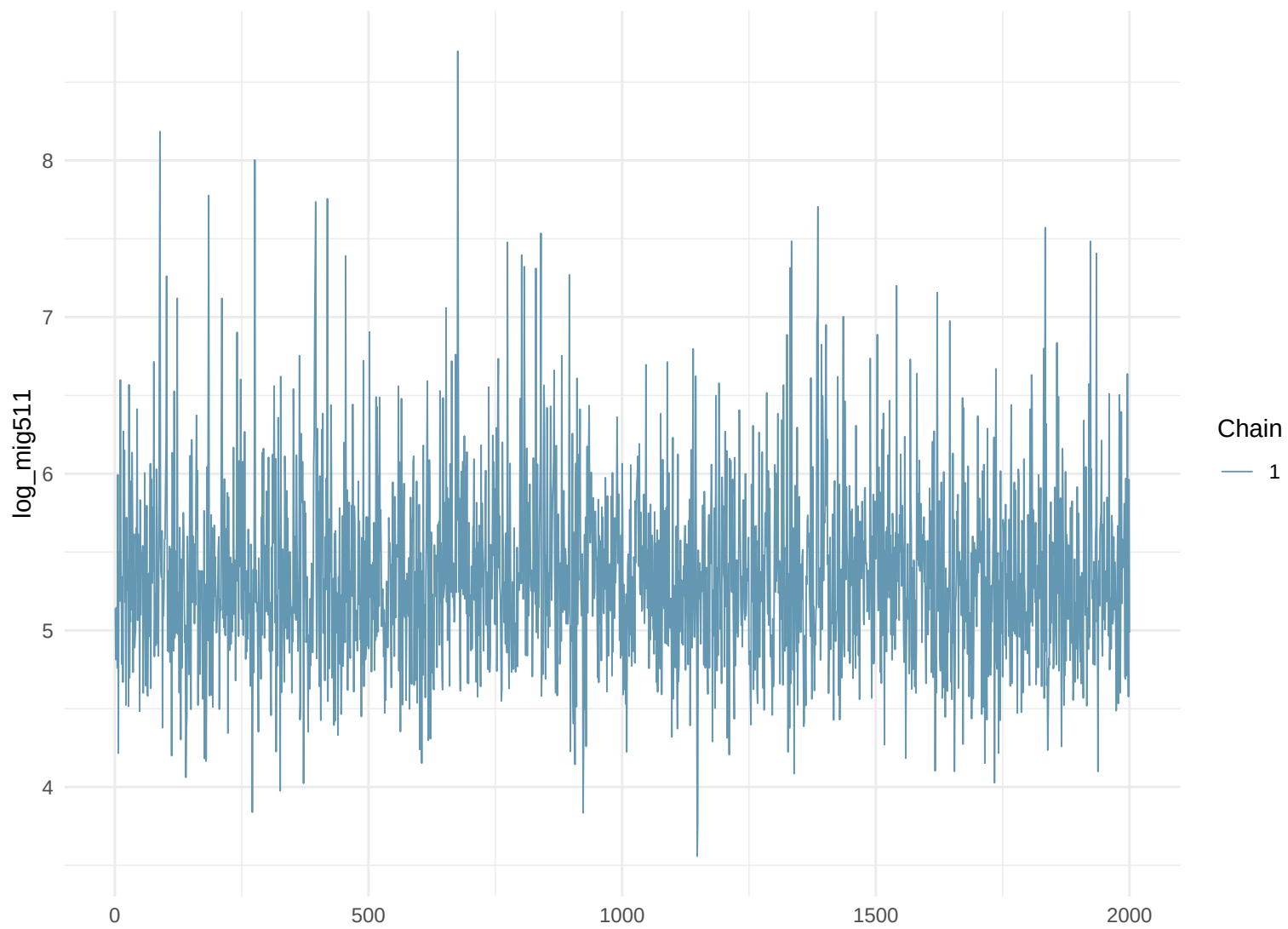
Trace Plot: log_mig511
