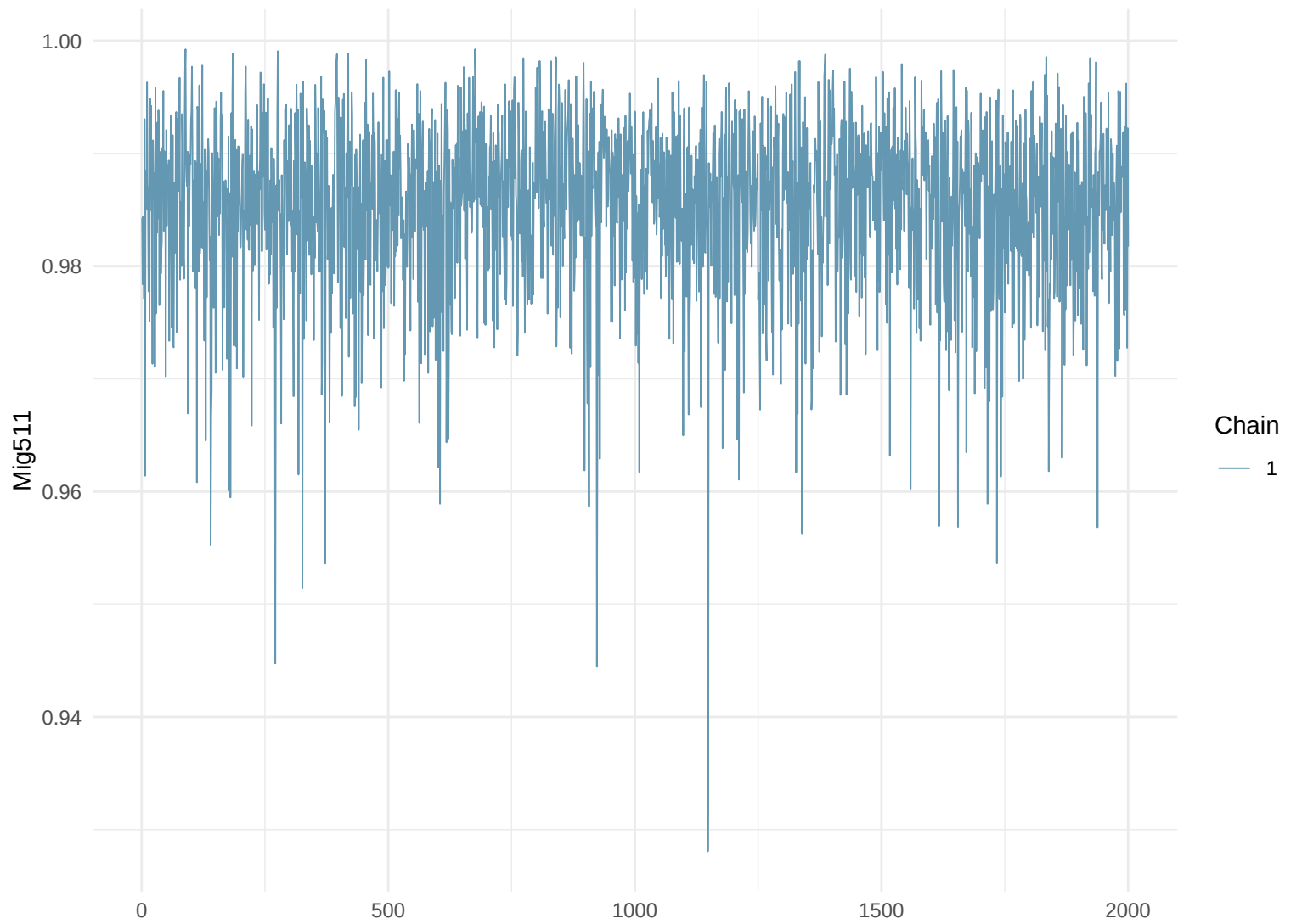
Trace Plot: Mig511
