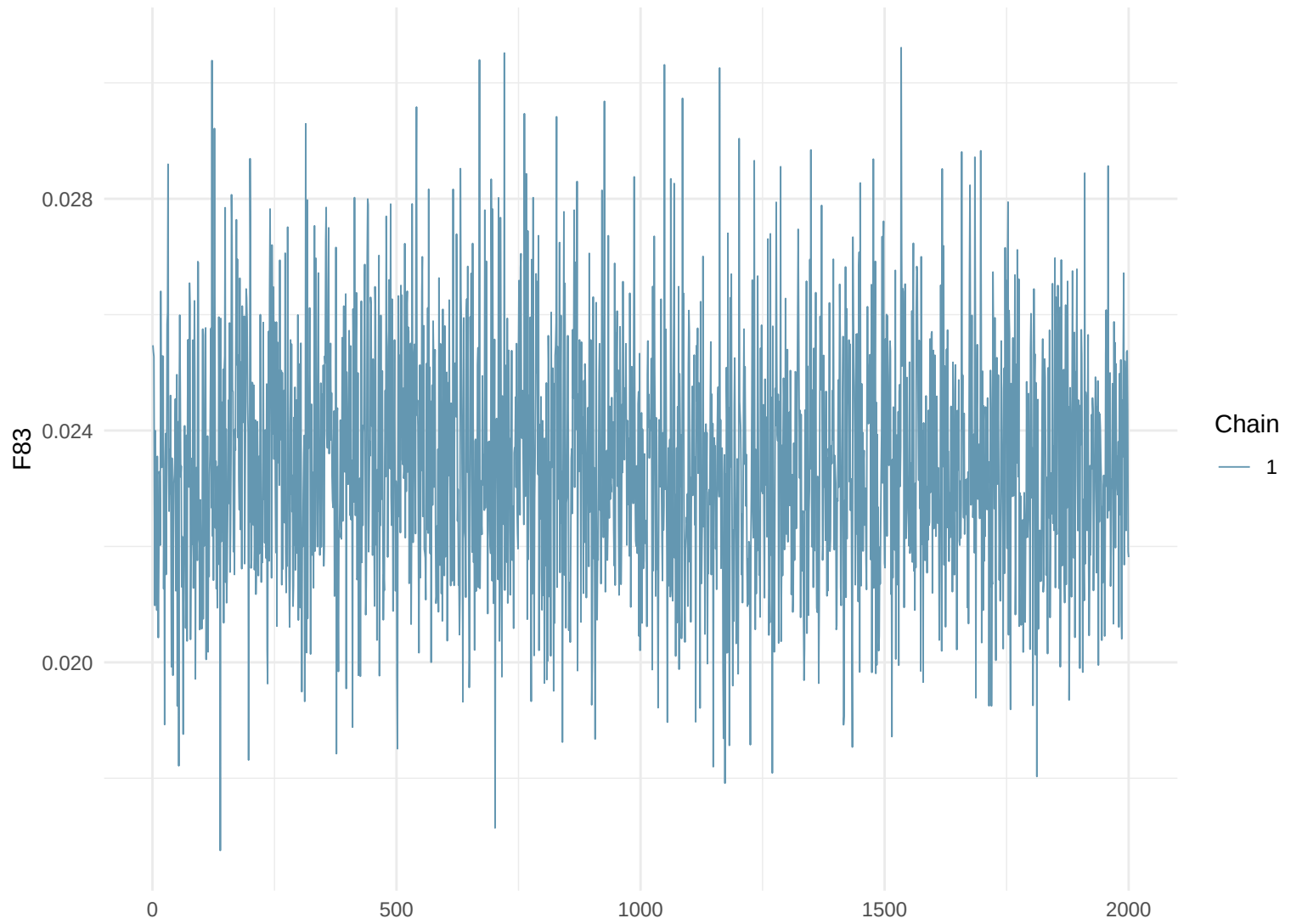
Trace Plot: F83
