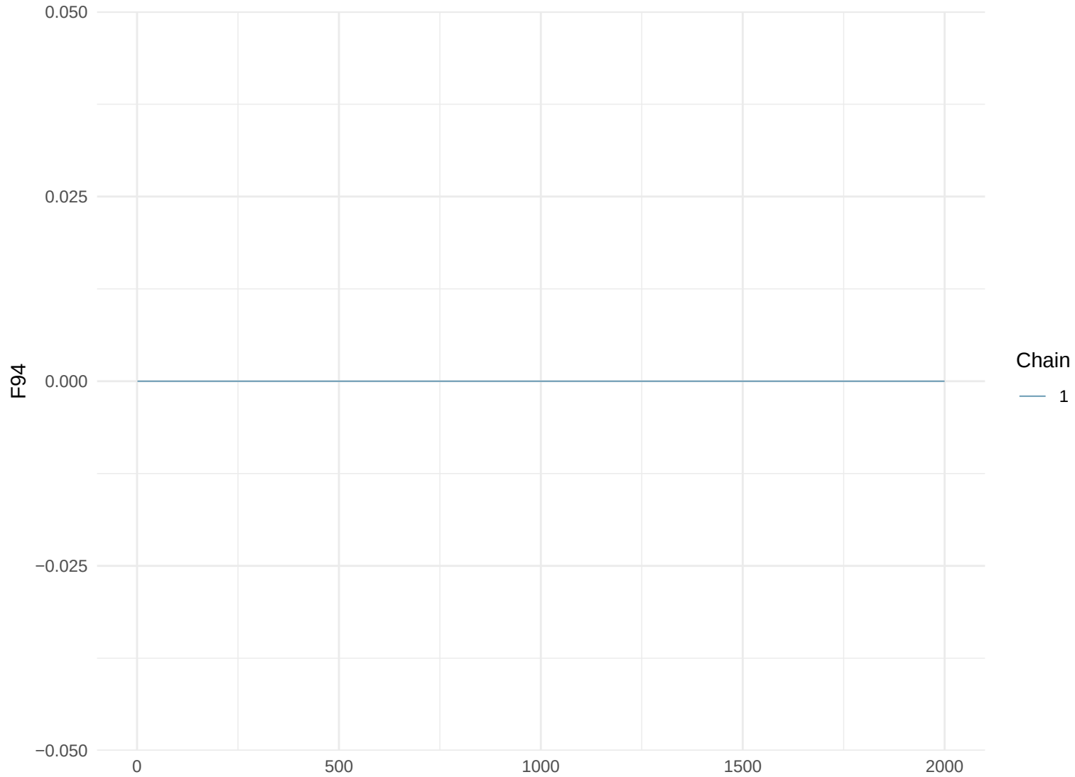
Trace Plot: F94
