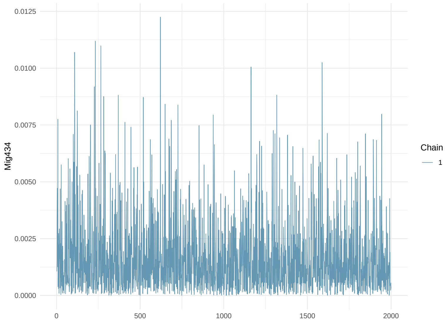
Trace Plot: Mig434
