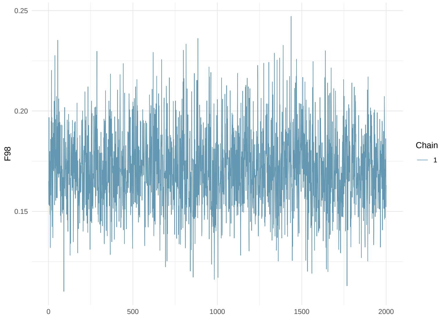
Trace Plot: F98
