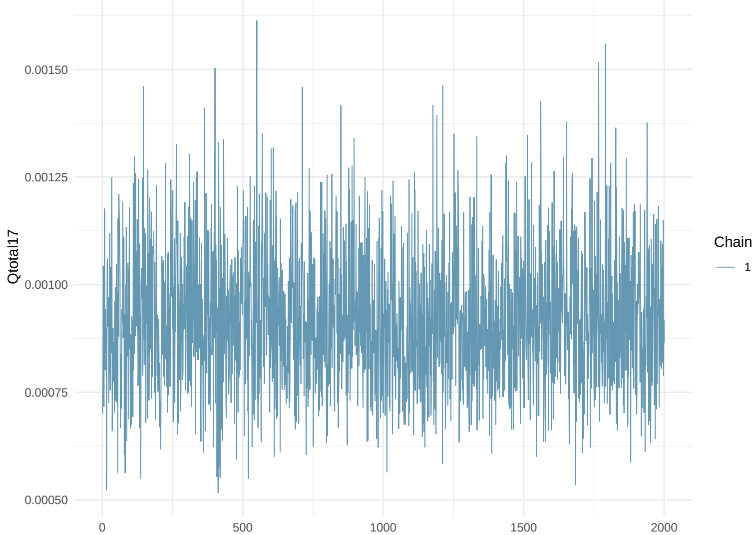
Trace Plot: Qtotal17
