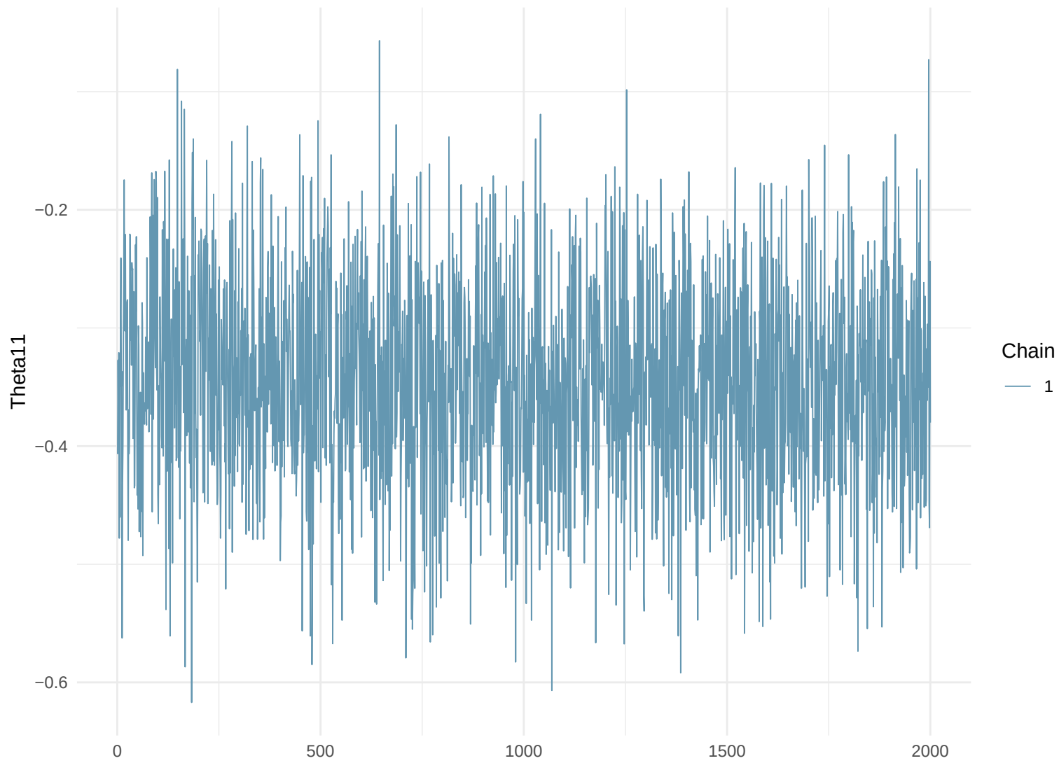
Trace Plot: Theta11
