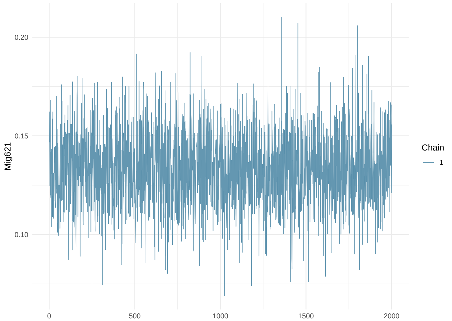
Trace Plot: Mig621
