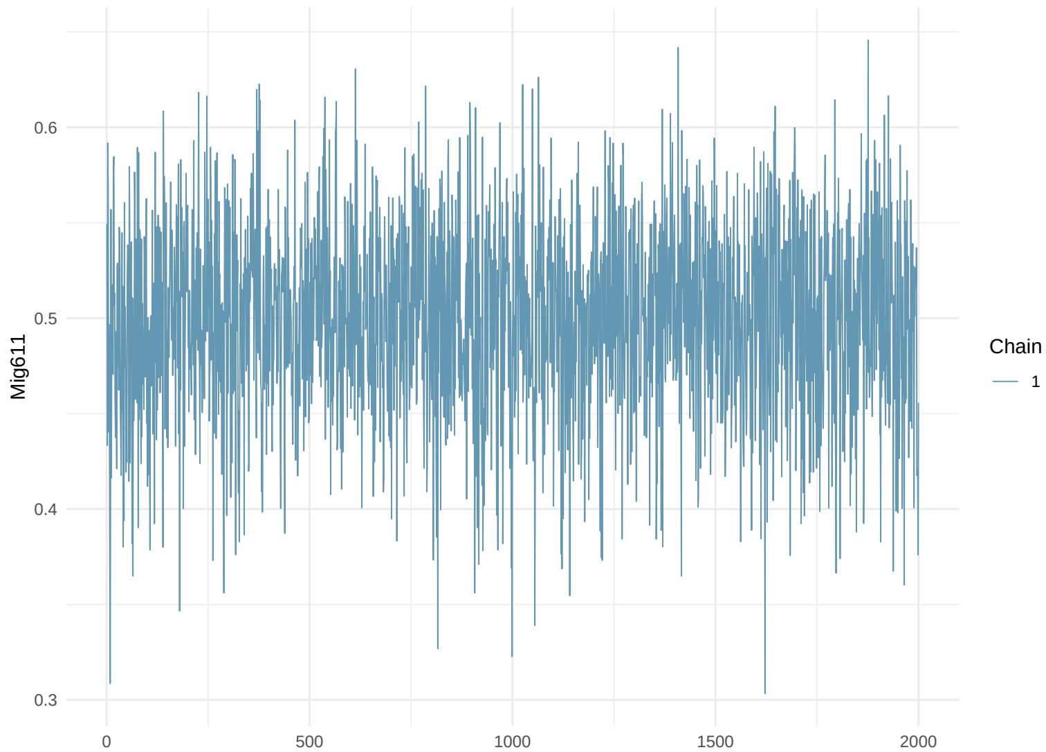
Trace Plot: Mig611
