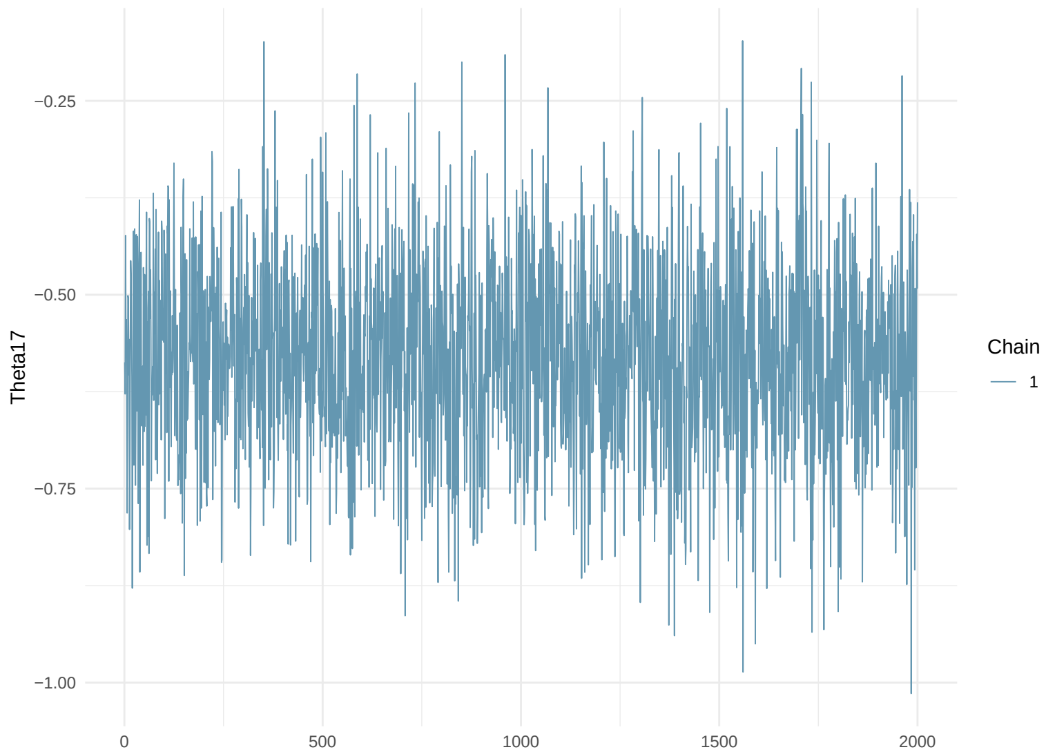
Trace Plot: Theta17
