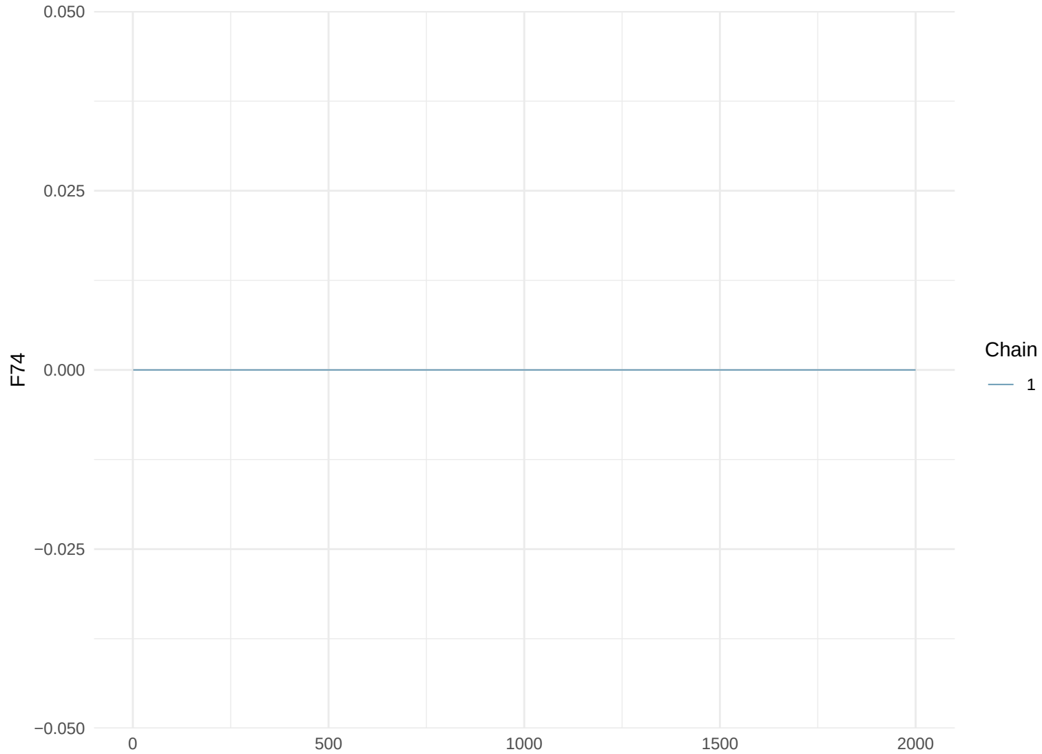
Trace Plot: F74
