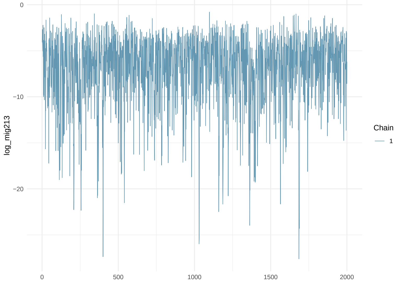
Trace Plot: log_mig213
