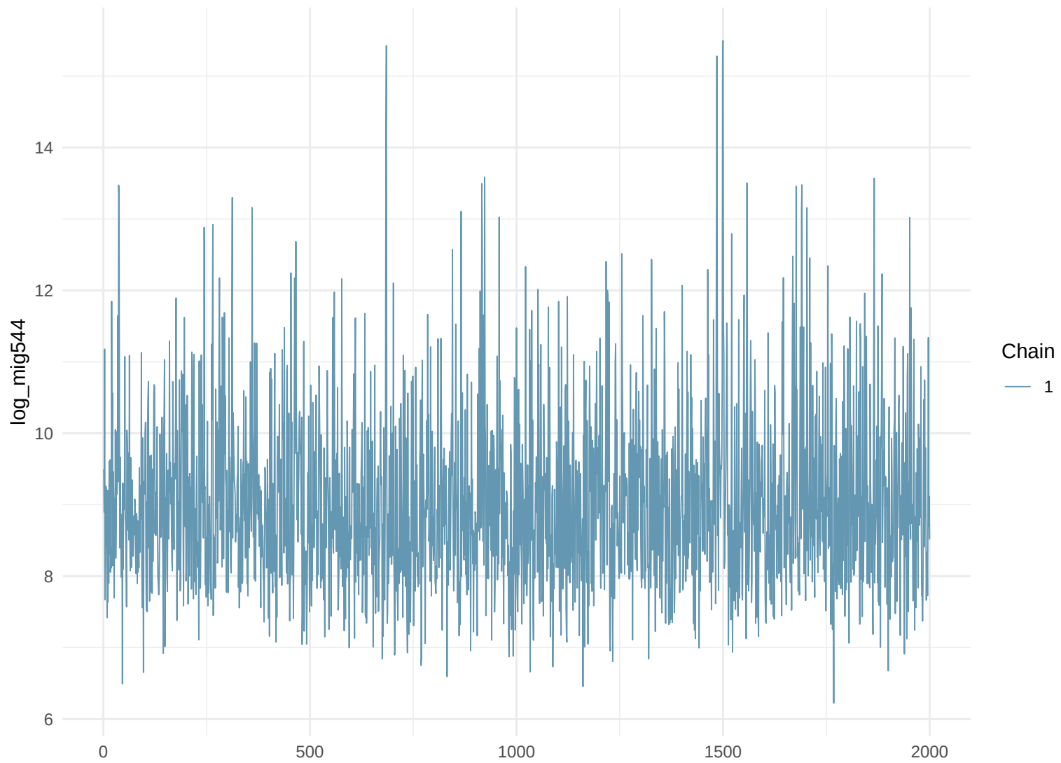
Trace Plot: log_mig544
