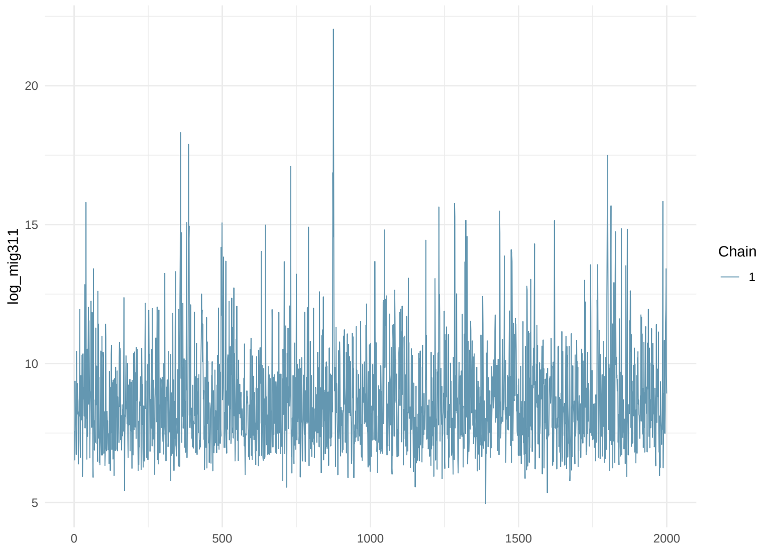
Trace Plot: log_mig311
