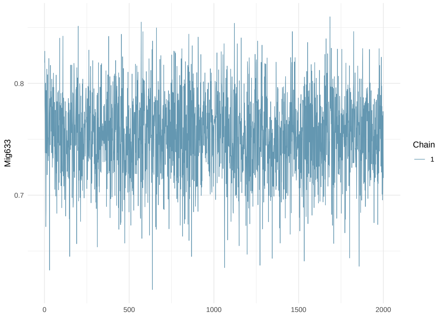
Trace Plot: Mig633
