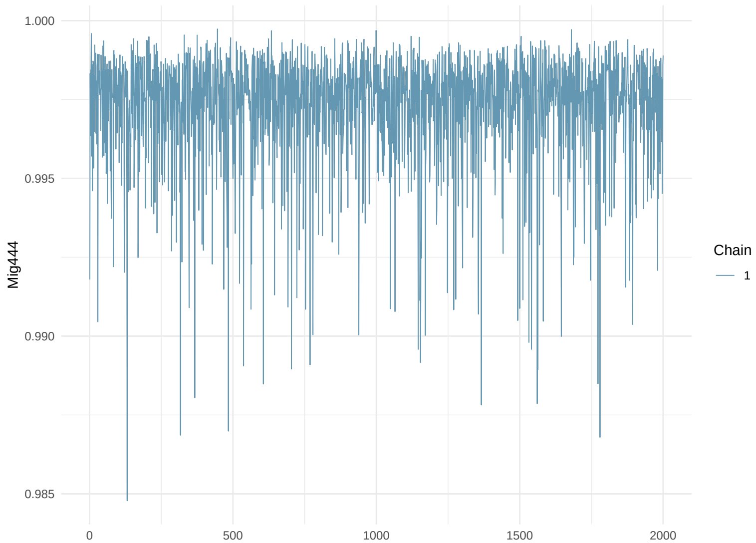
Trace Plot: Mig444
