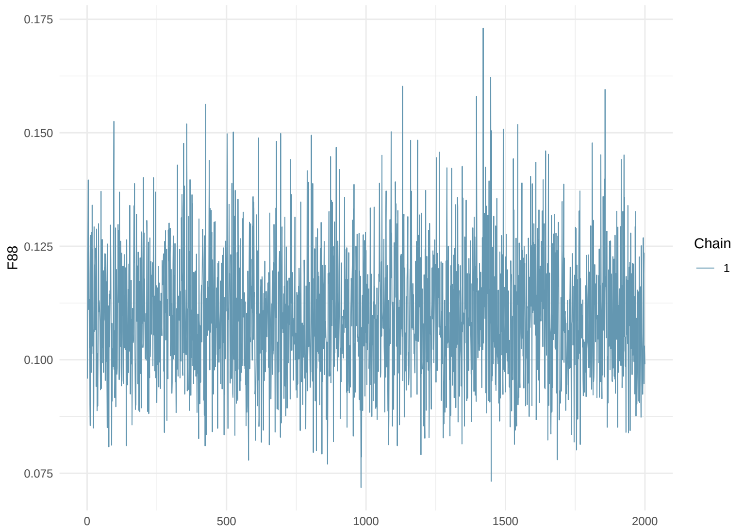
Trace Plot: F88
