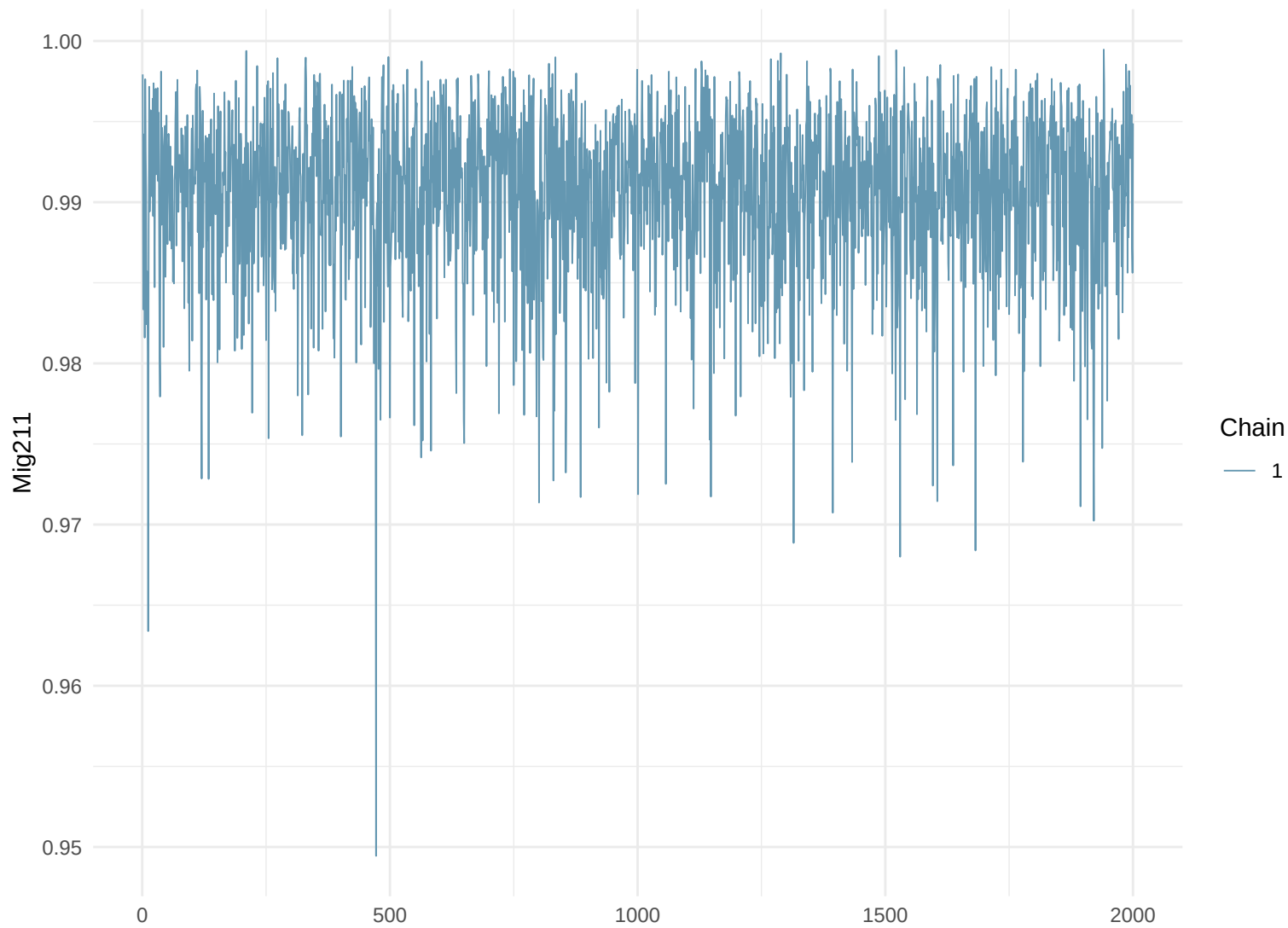
Trace Plot: Mig211
