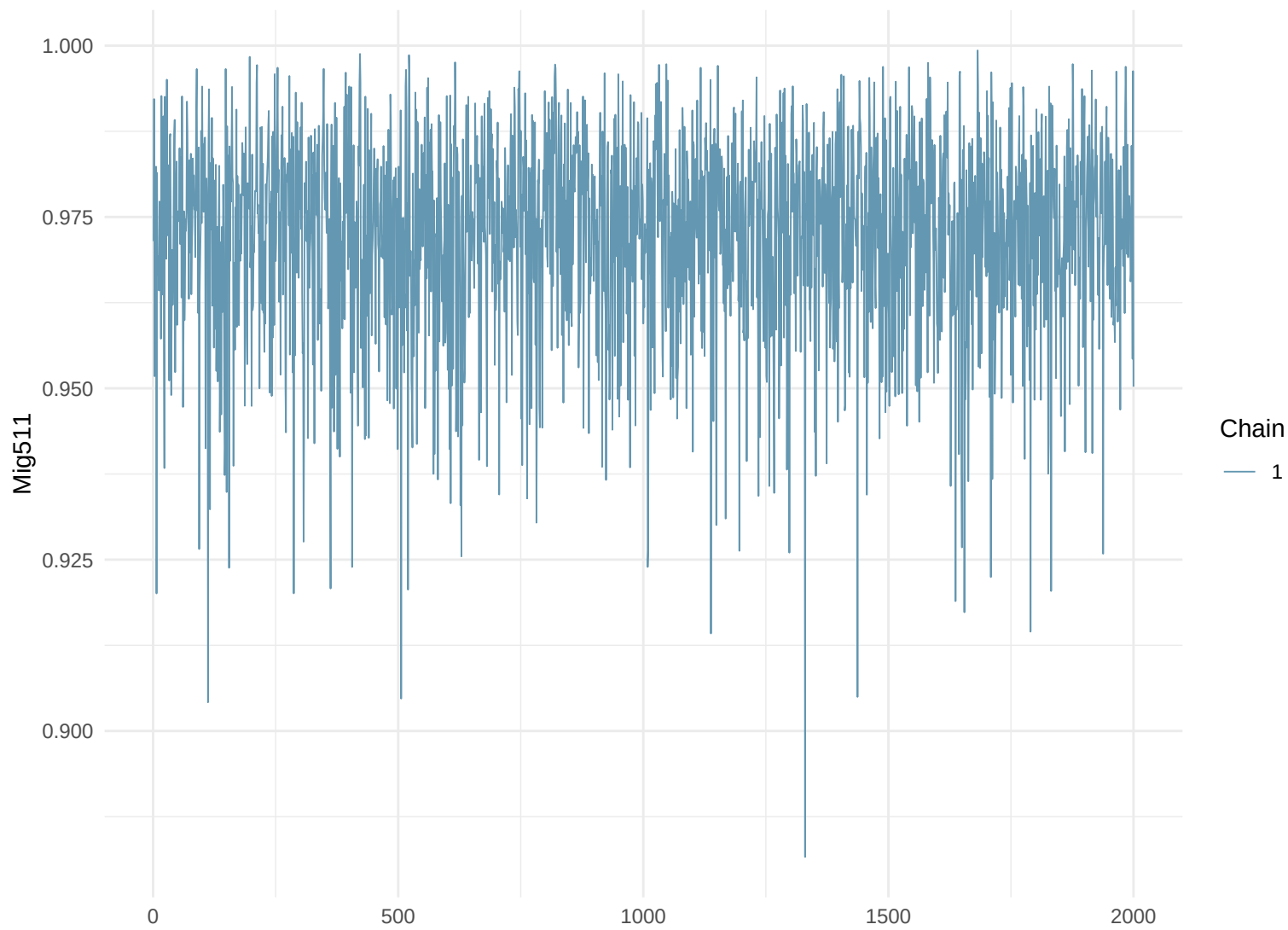
Trace Plot: Mig511
