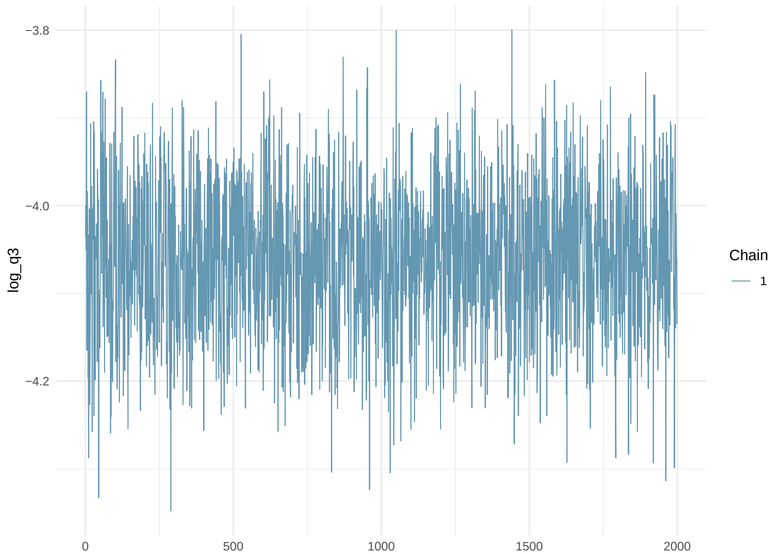
Trace Plot: log_q3
