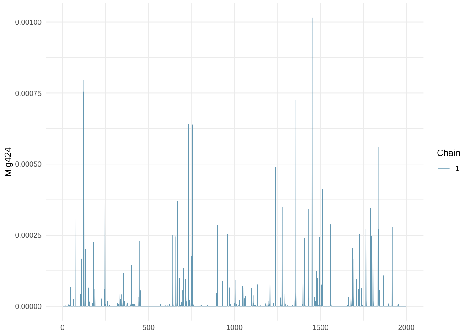
Trace Plot: Mig424
