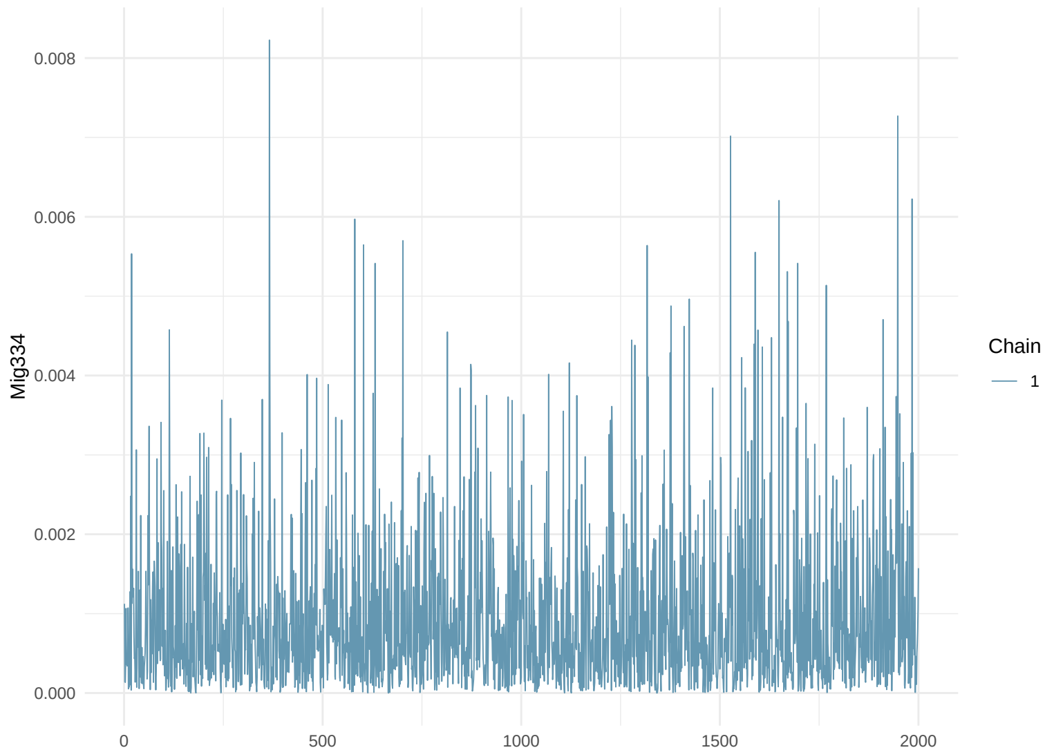
Trace Plot: Mig334
