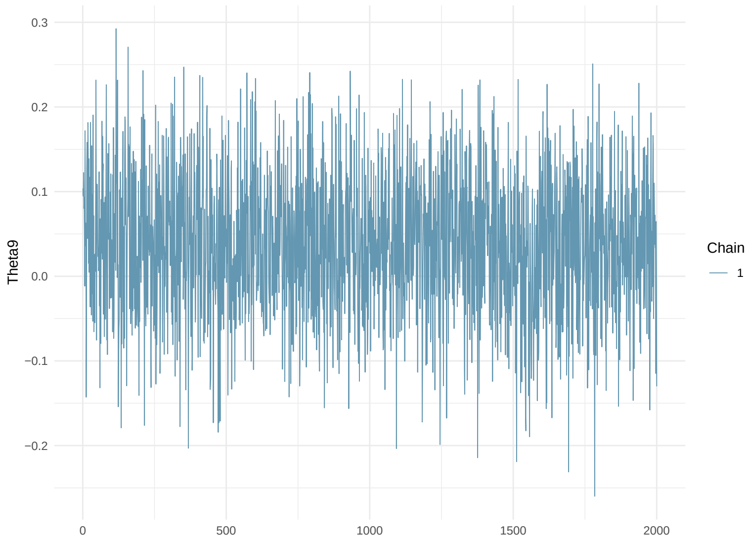
Trace Plot: Theta9
