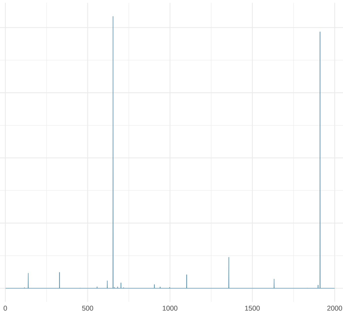
Trace Plot: Mig541
