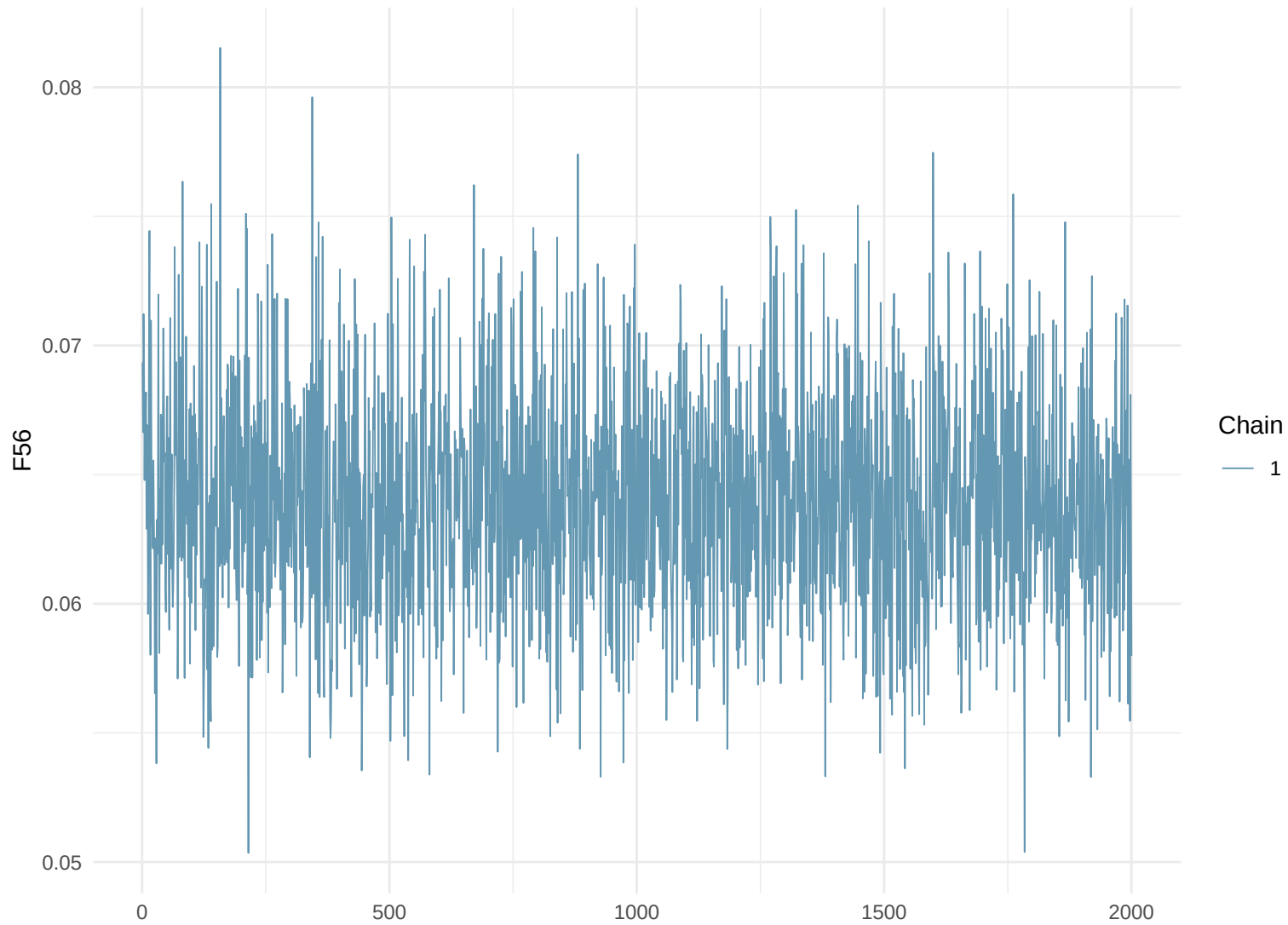
Trace Plot: F56
