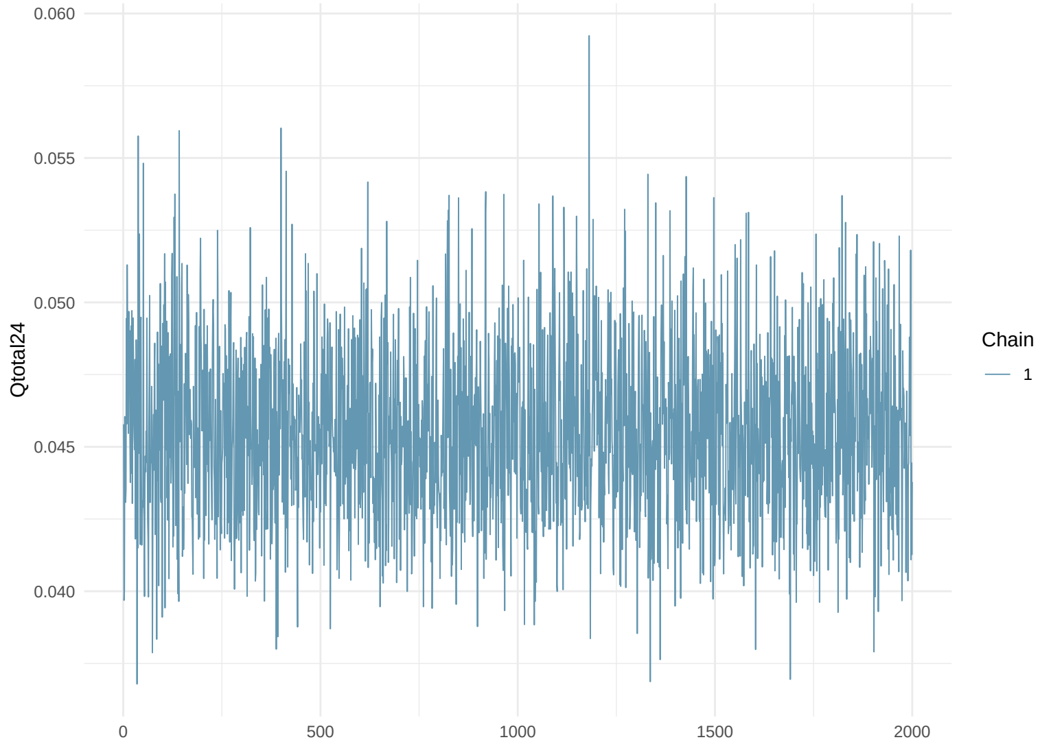
Trace Plot: Qtotal24
