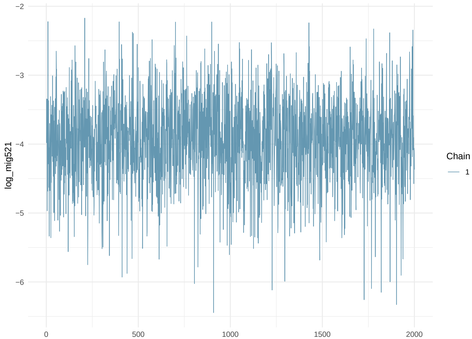
Trace Plot: log_mig521
