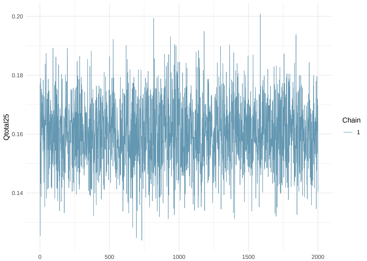
Trace Plot: Qtotal25
