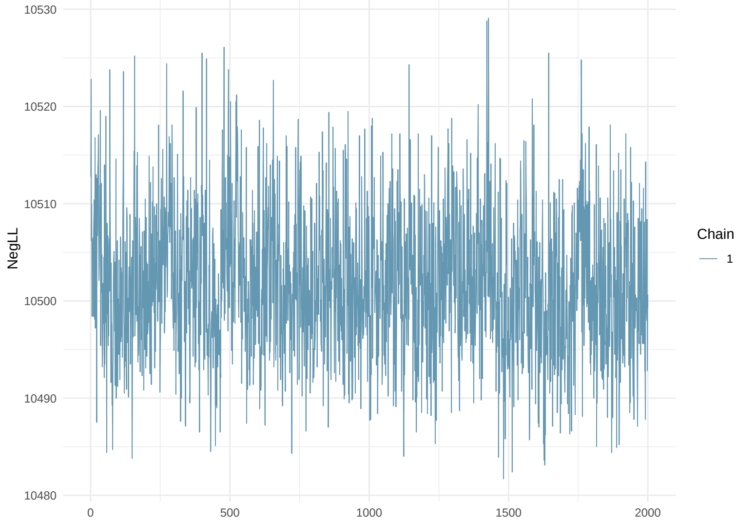
Trace Plot: NegLL
