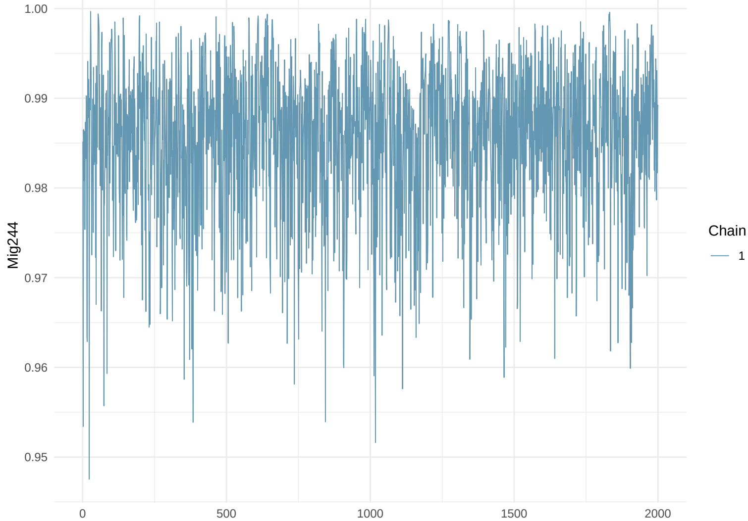
Trace Plot: Mig244
