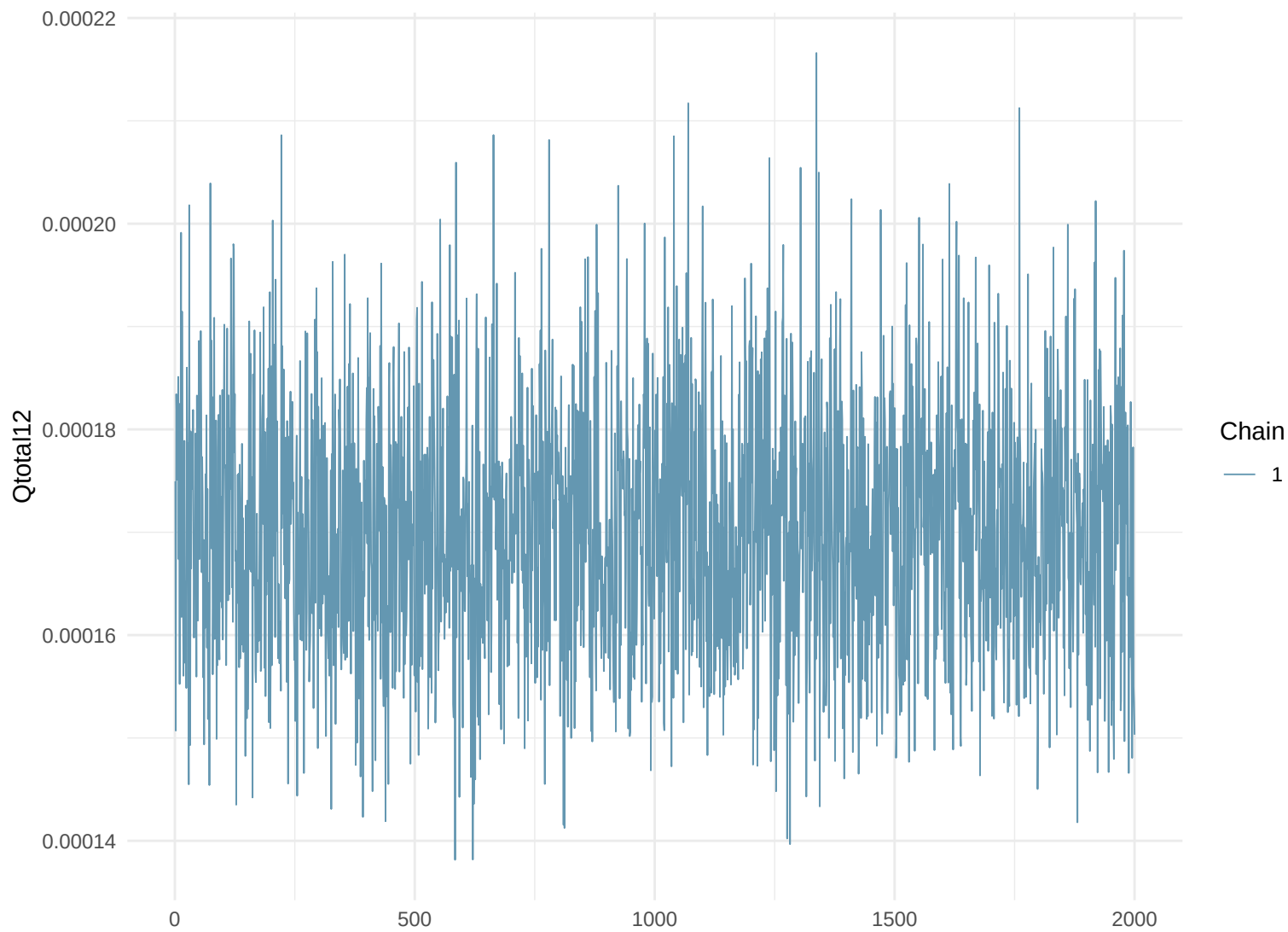
Trace Plot: Qtotal12
