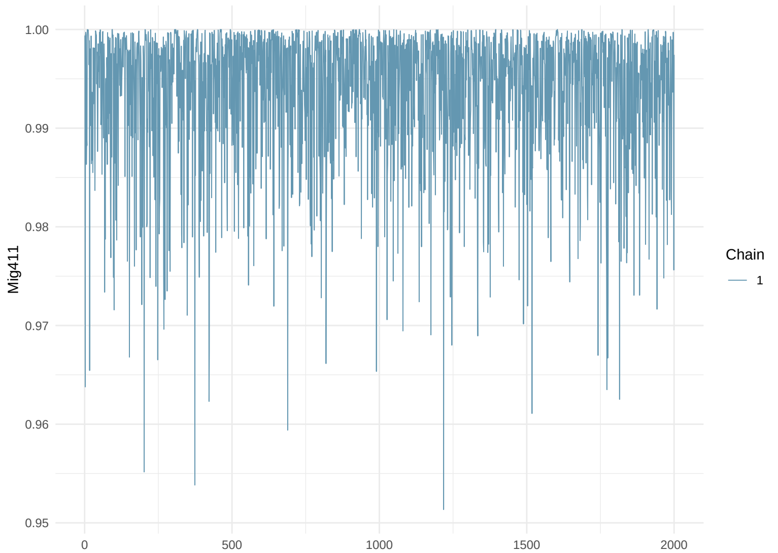
Trace Plot: Mig411
