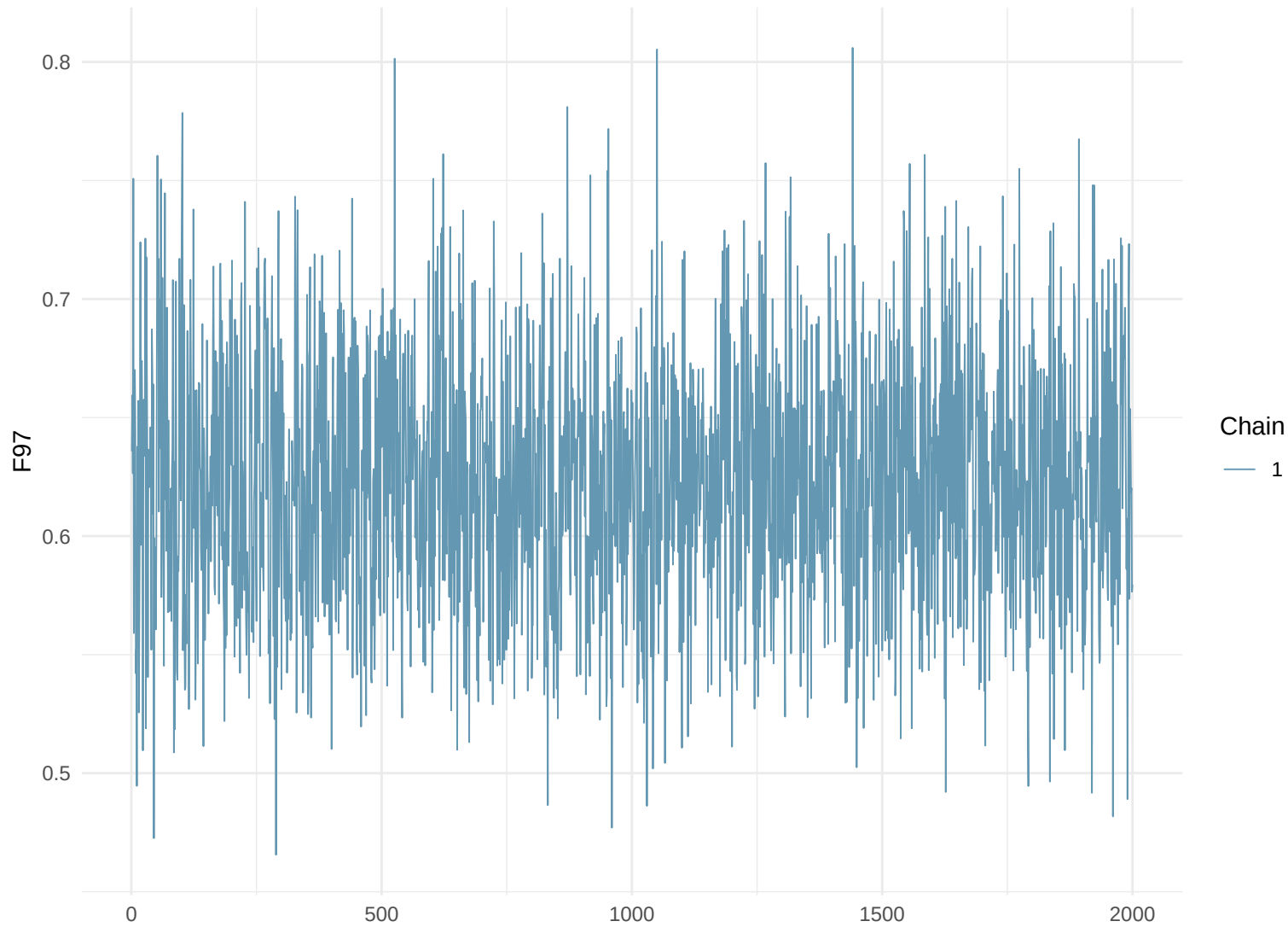
Trace Plot: F97
