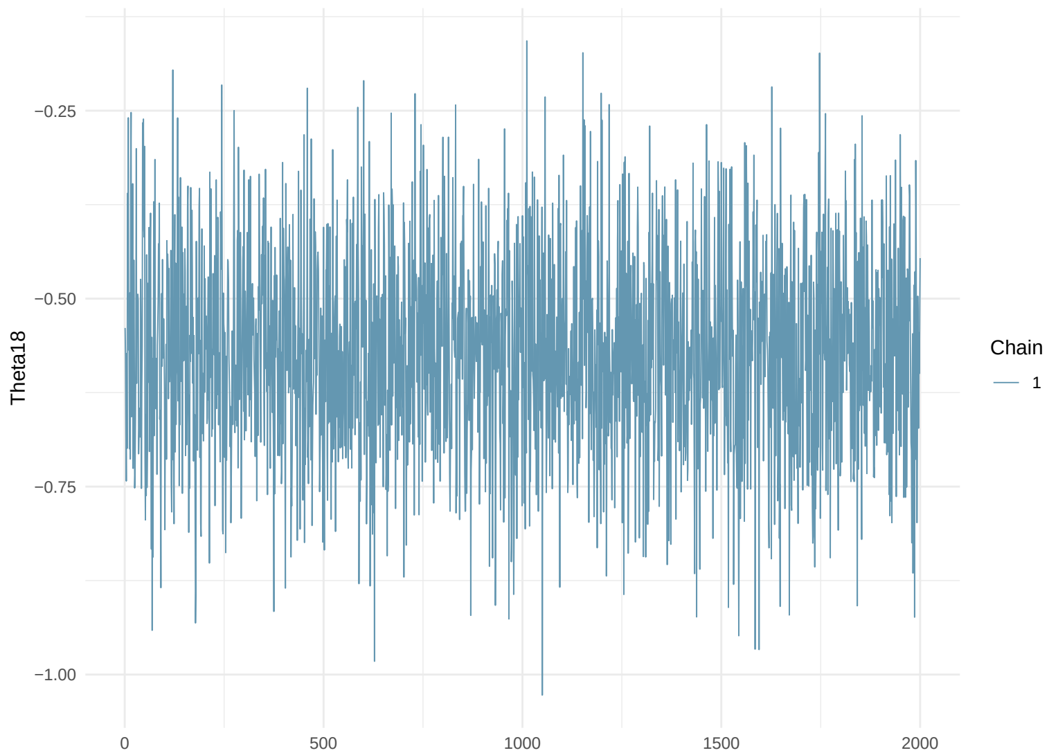
Trace Plot: Theta18
