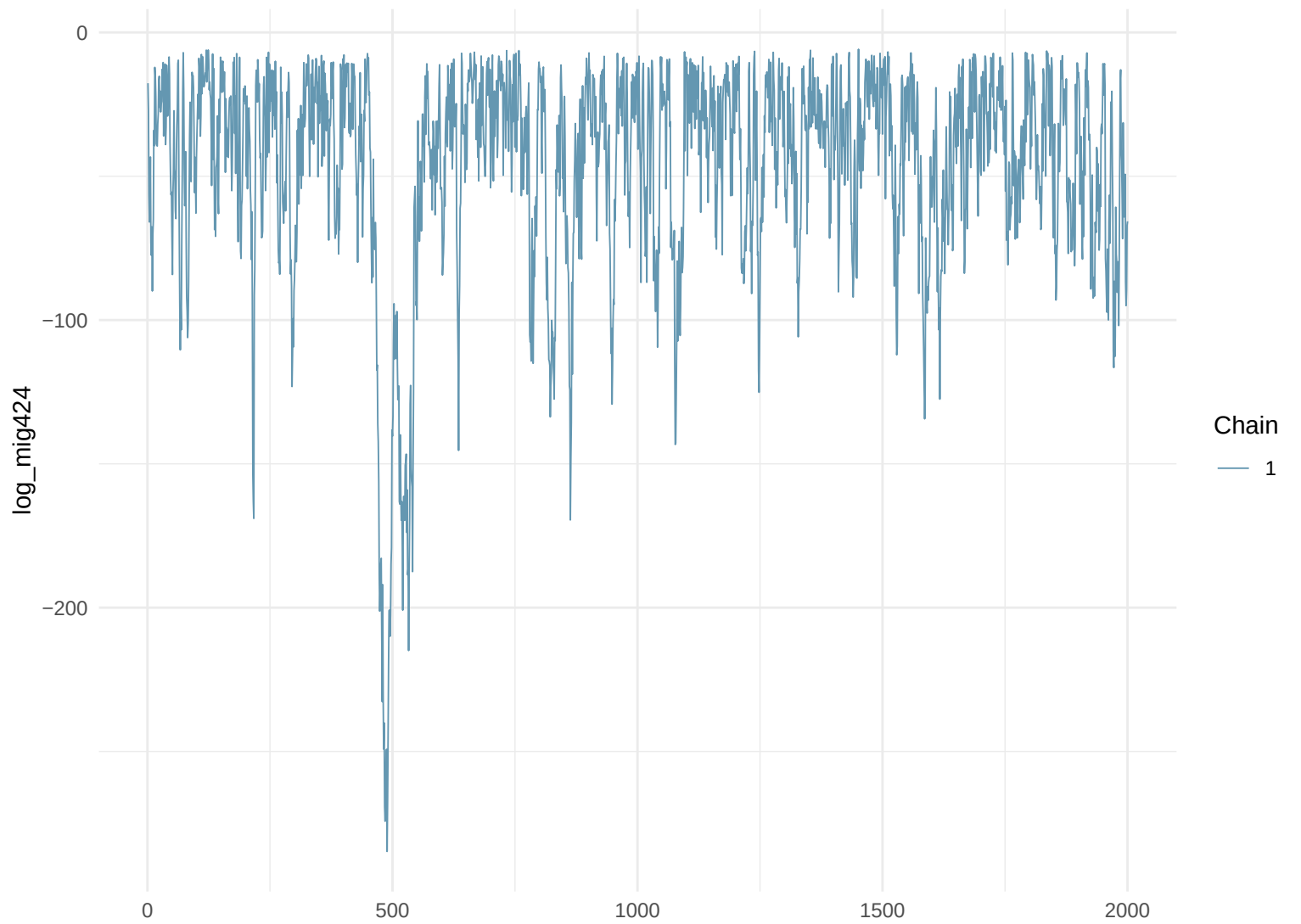
Trace Plot: log_mig424
