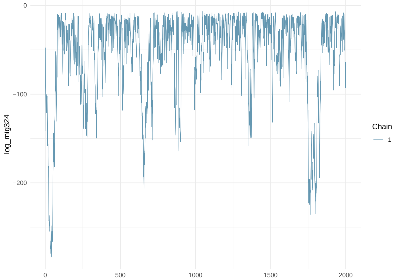
Trace Plot: log_mig324
