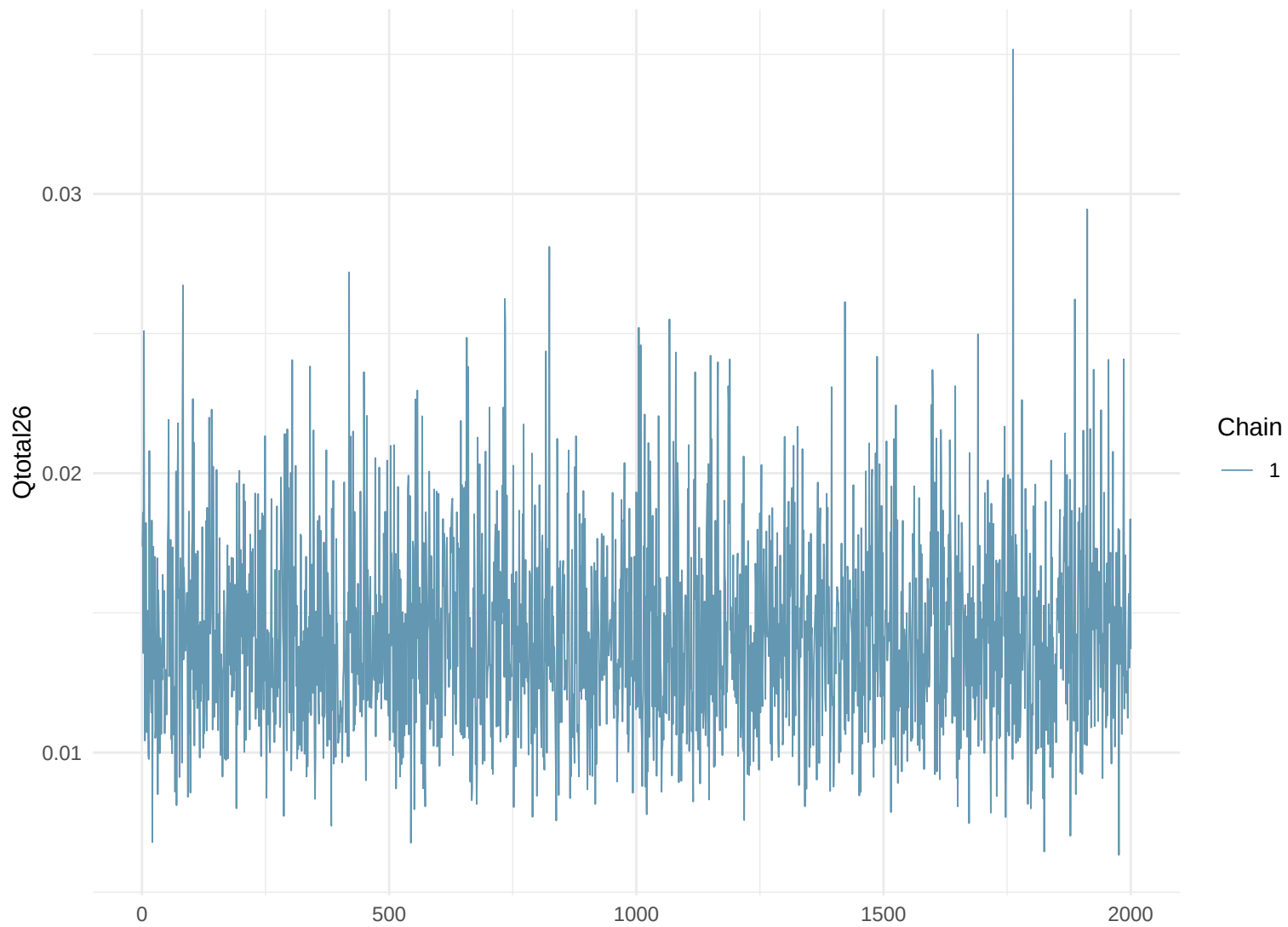
Trace Plot: Qtotal26
