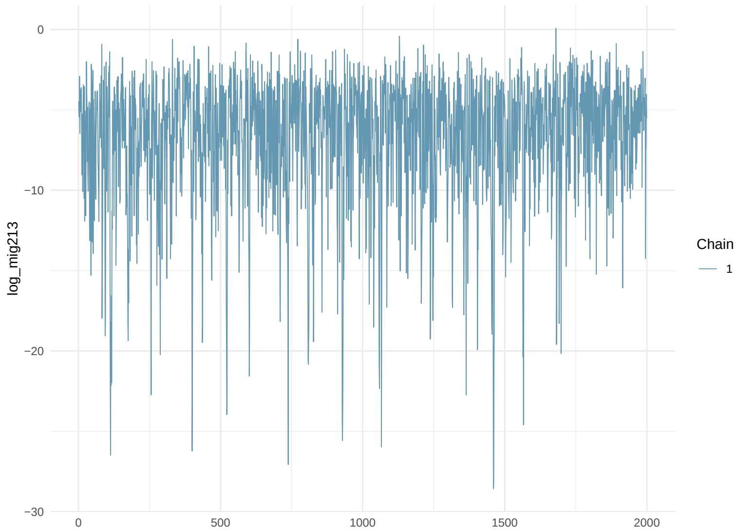
Trace Plot: log_mig213
