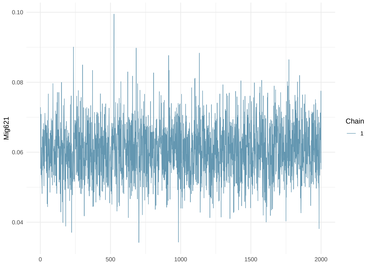
Trace Plot: Mig621
