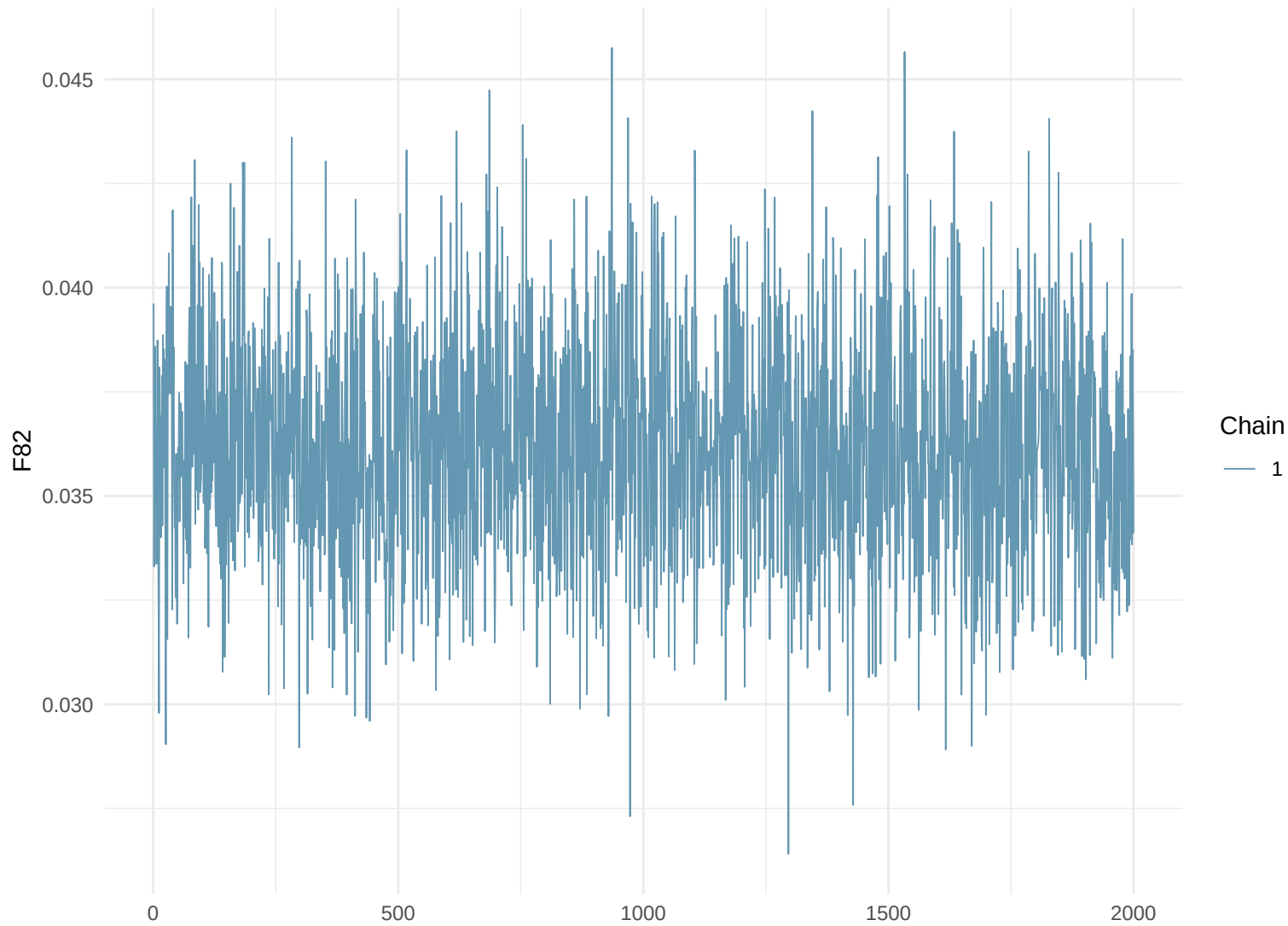
Trace Plot: F82
