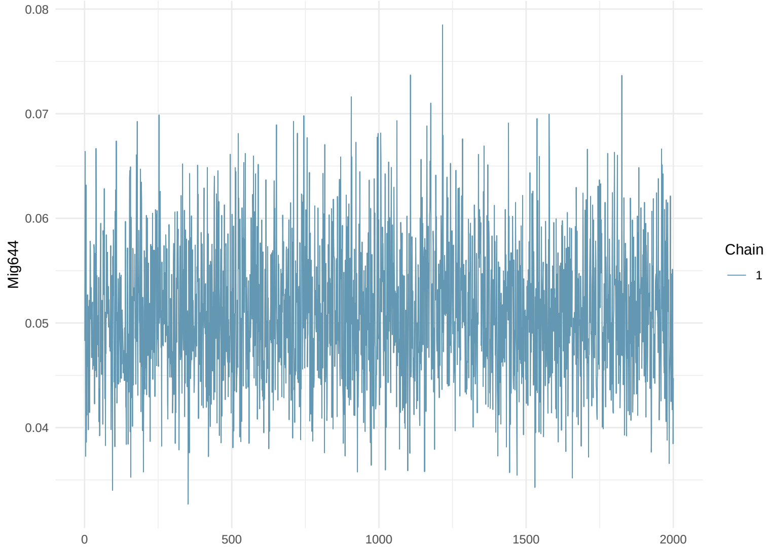
Trace Plot: Mig644
