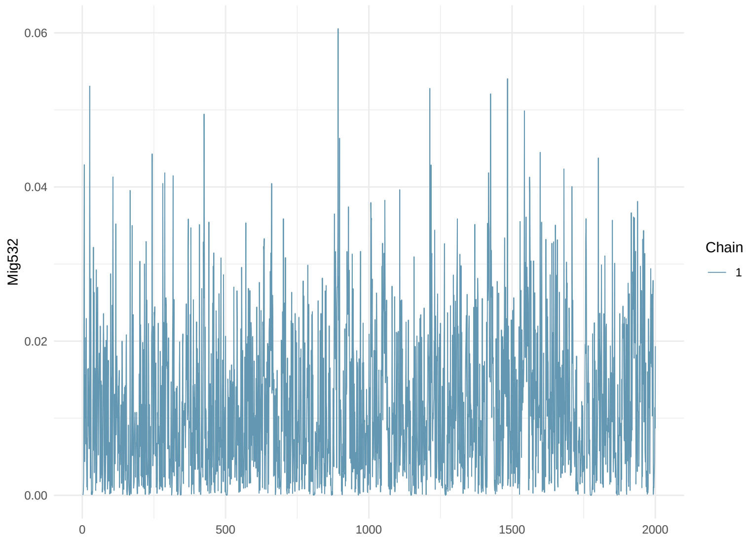
Trace Plot: Mig532
