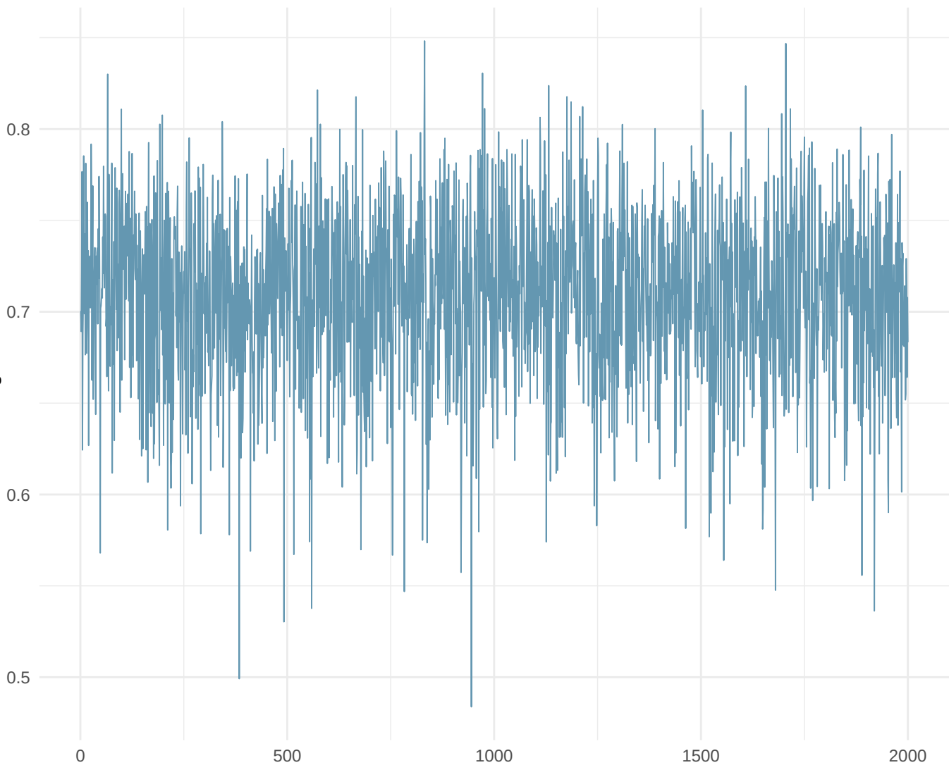
Trace Plot: Mig233
