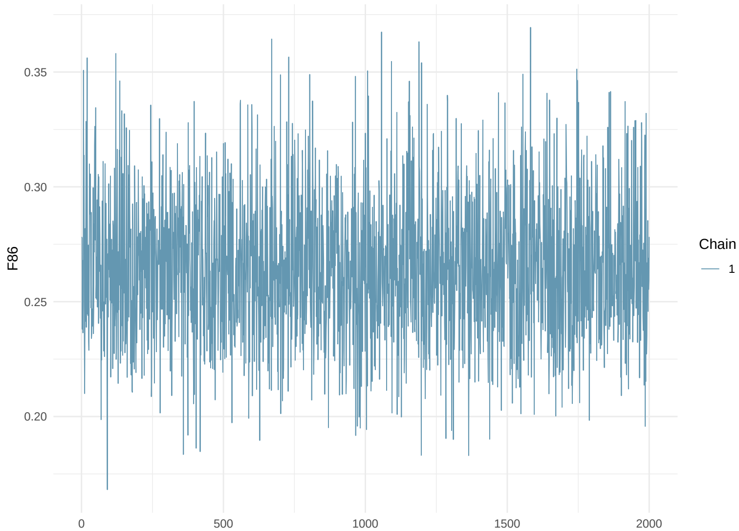
Trace Plot: F86
