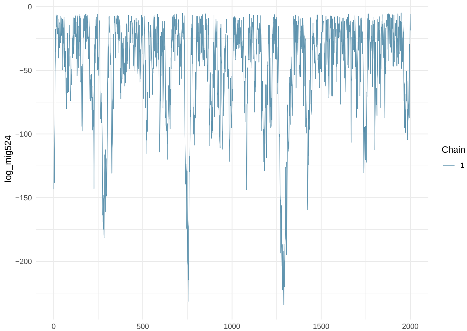
Trace Plot: log_mig524
