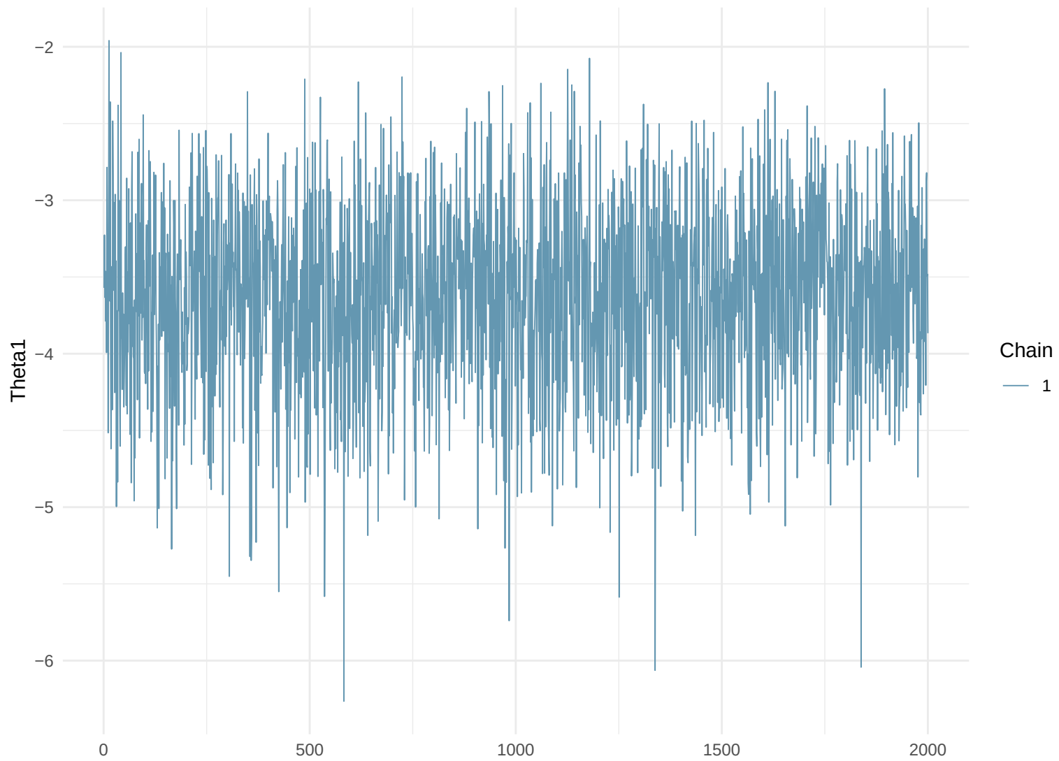
Trace Plot: Theta1
