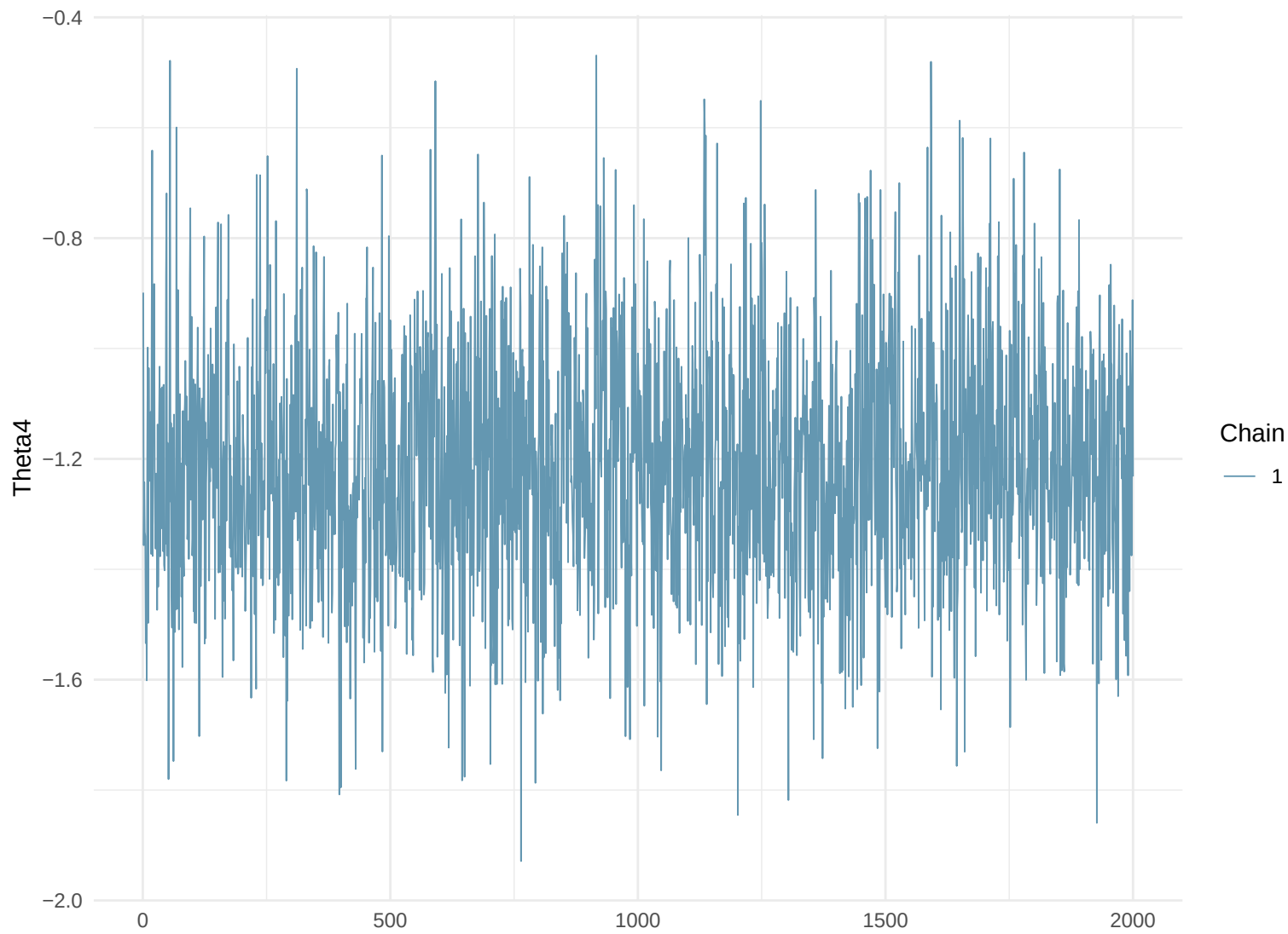
Trace Plot: Theta4
