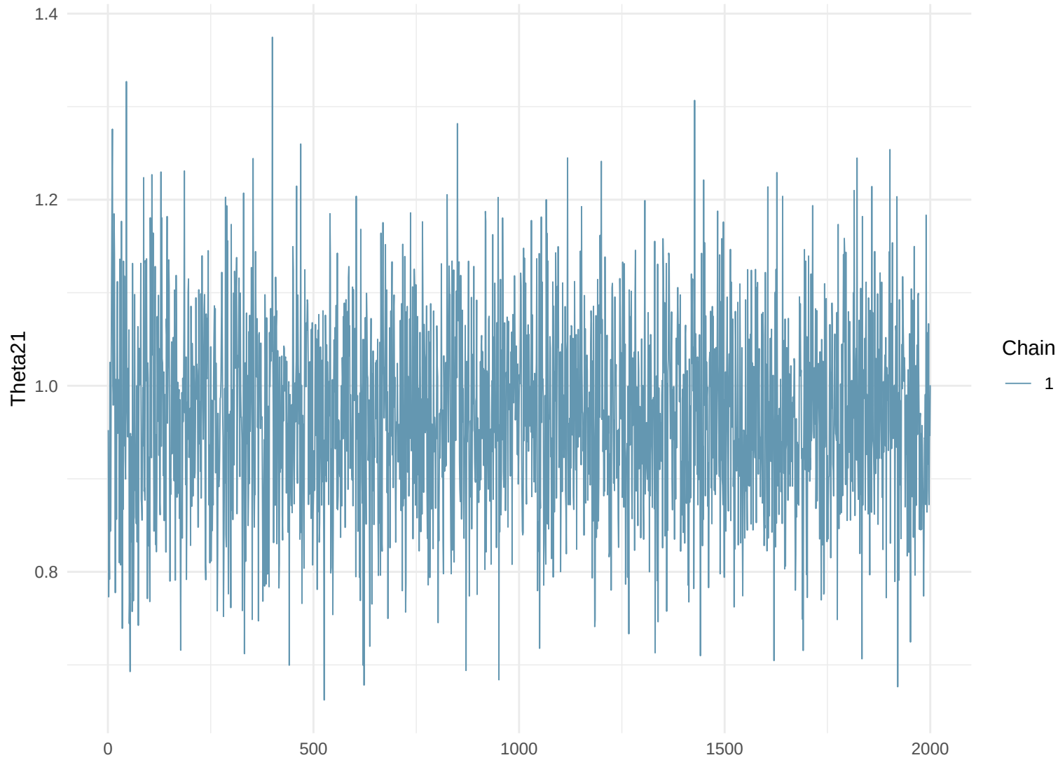
Trace Plot: Theta21
