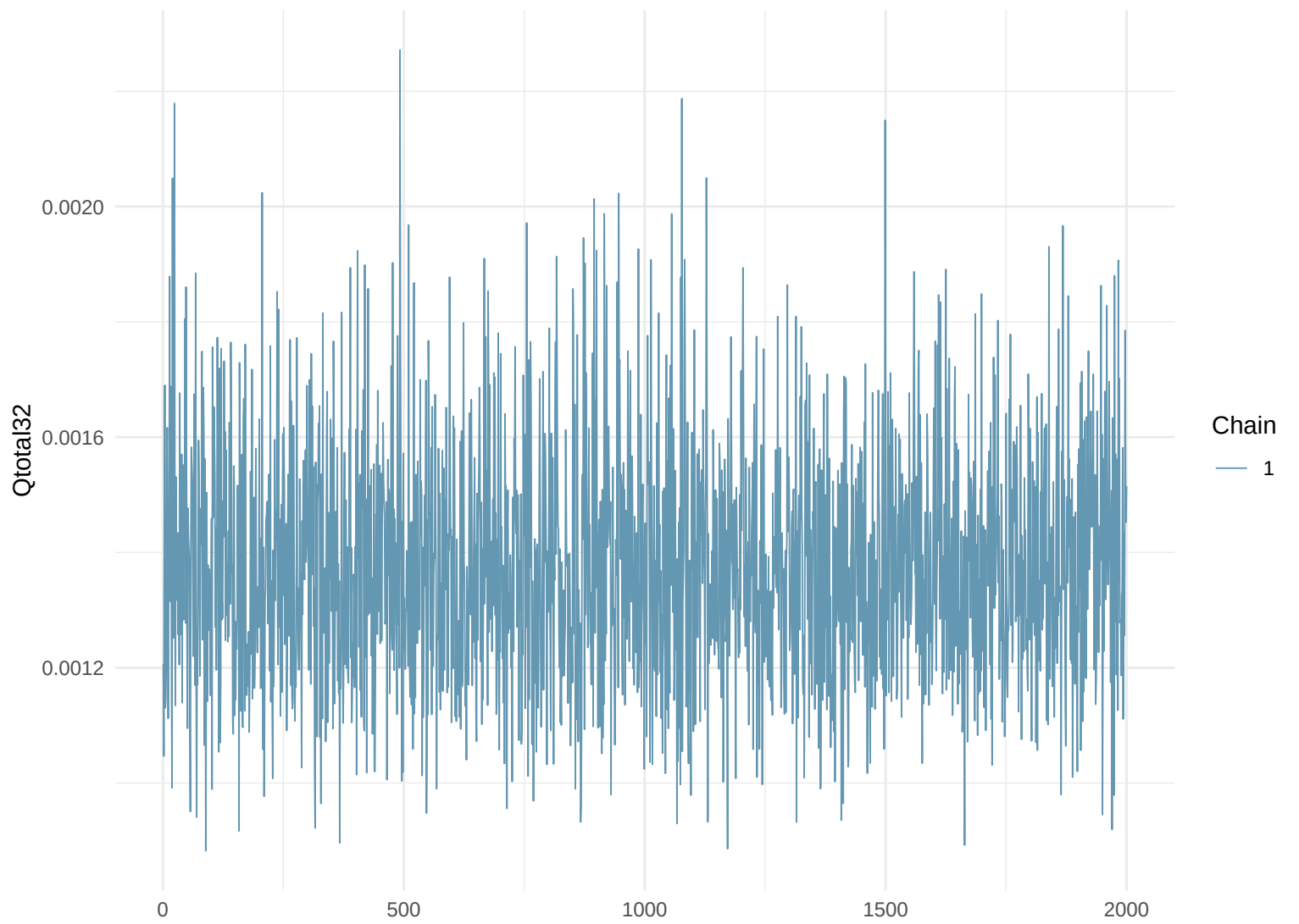
Trace Plot: Qtotal32
