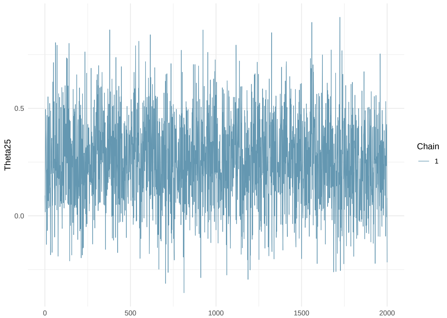
Trace Plot: Theta25
