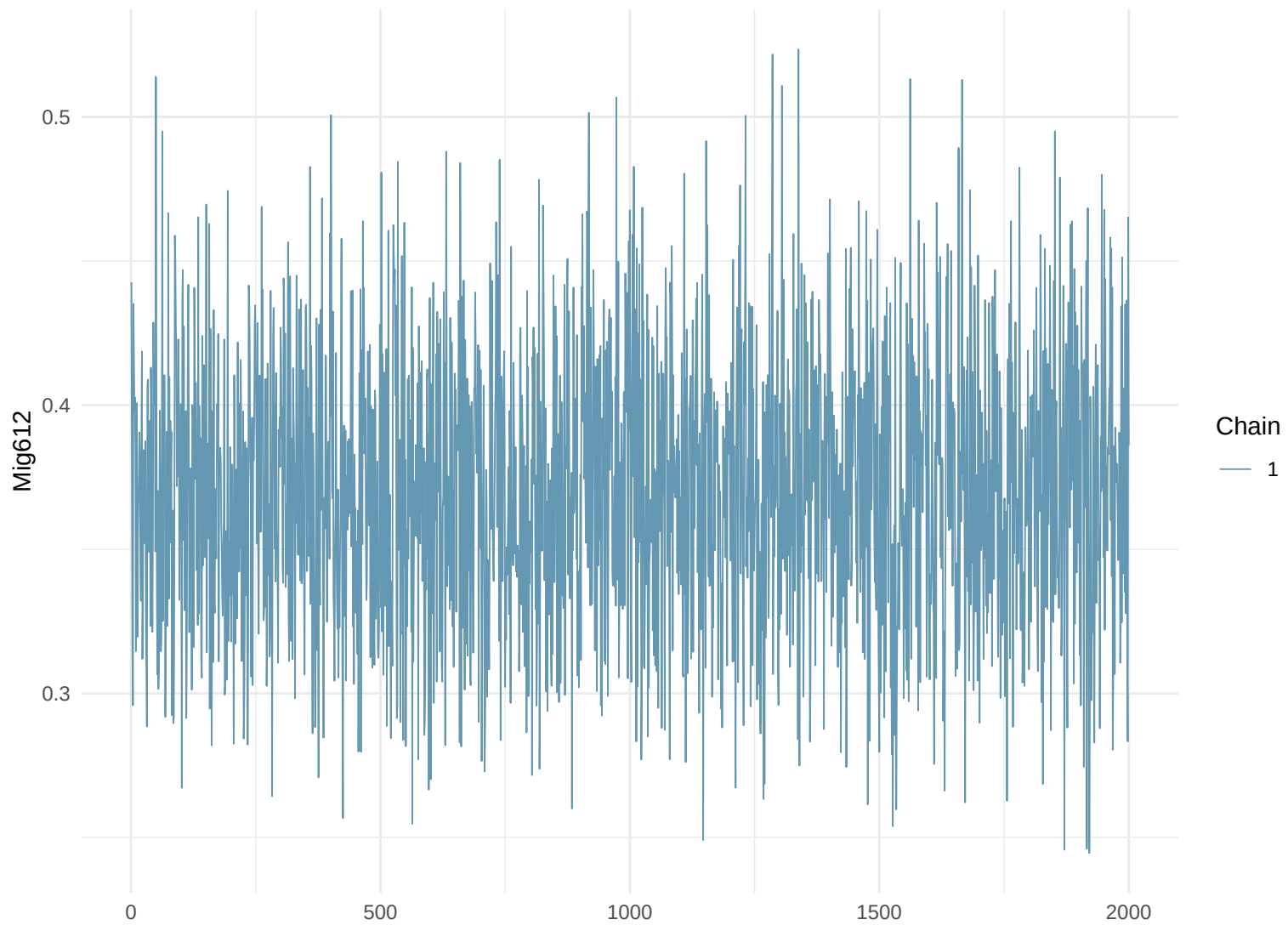
Trace Plot: Mig612
