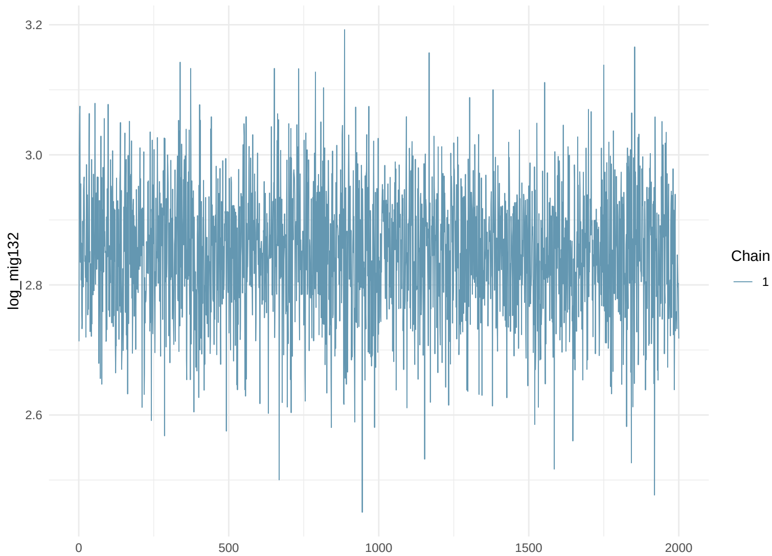
Trace Plot: log_mig132
