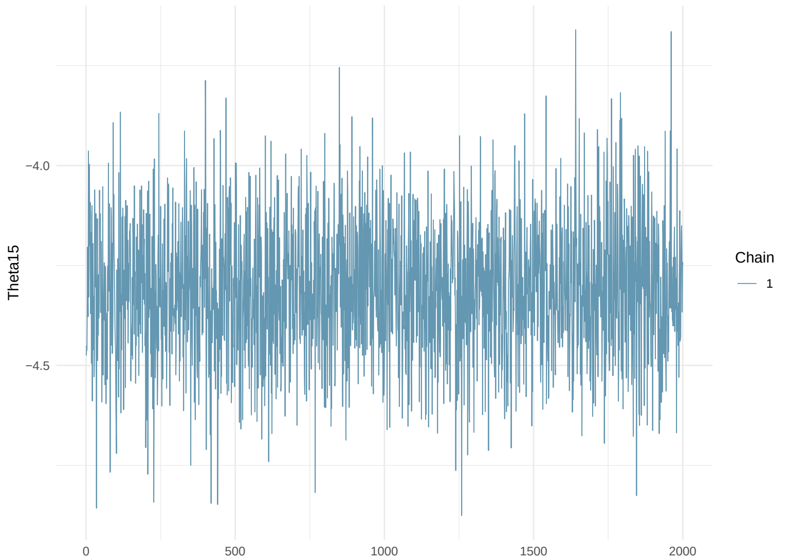
Trace Plot: Theta15
