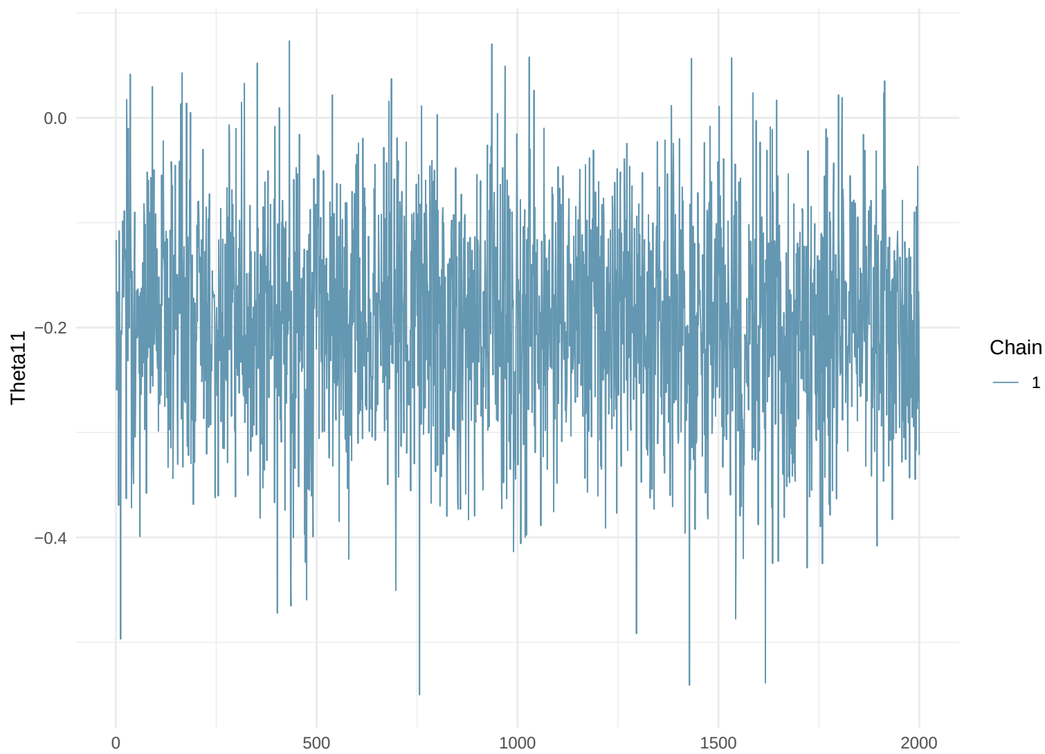
Trace Plot: Theta11
