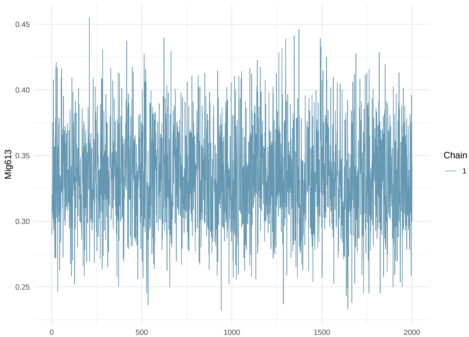
Trace Plot: Mig613
