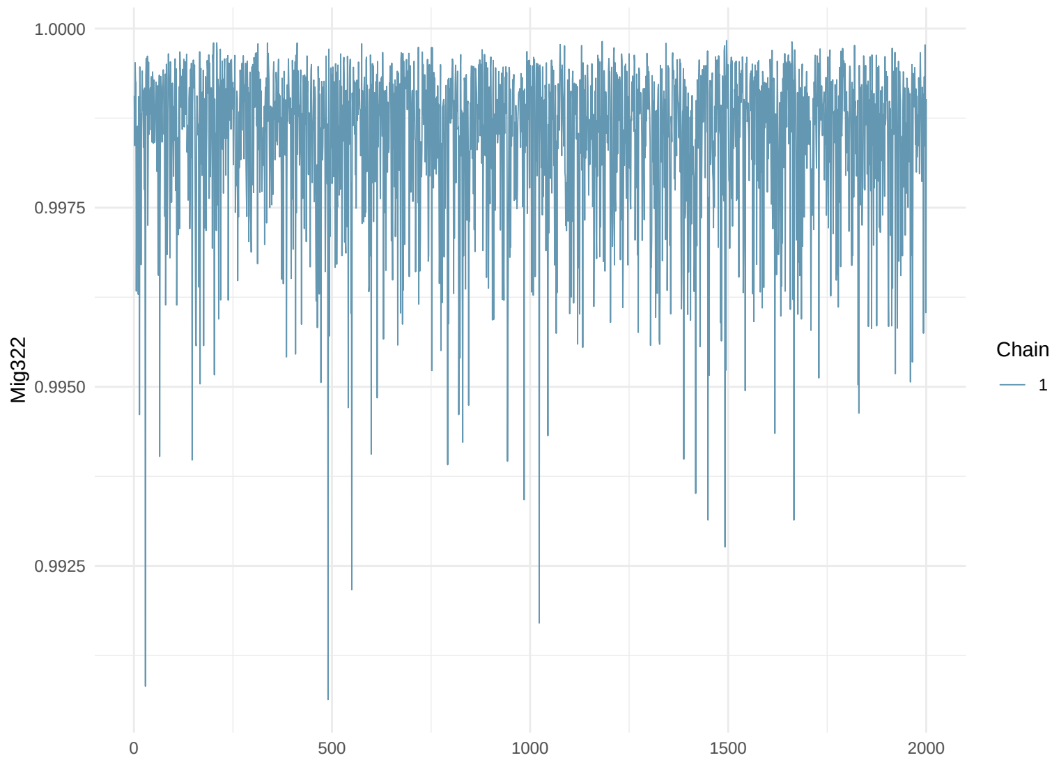
Trace Plot: Mig322
