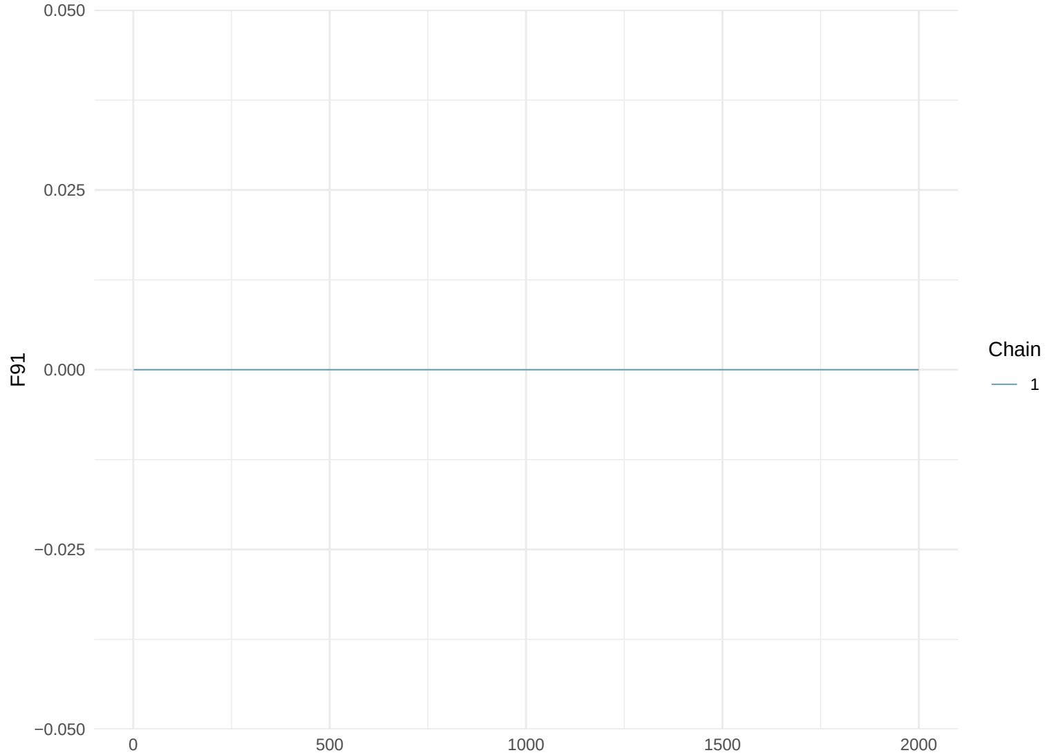
Trace Plot: F91
