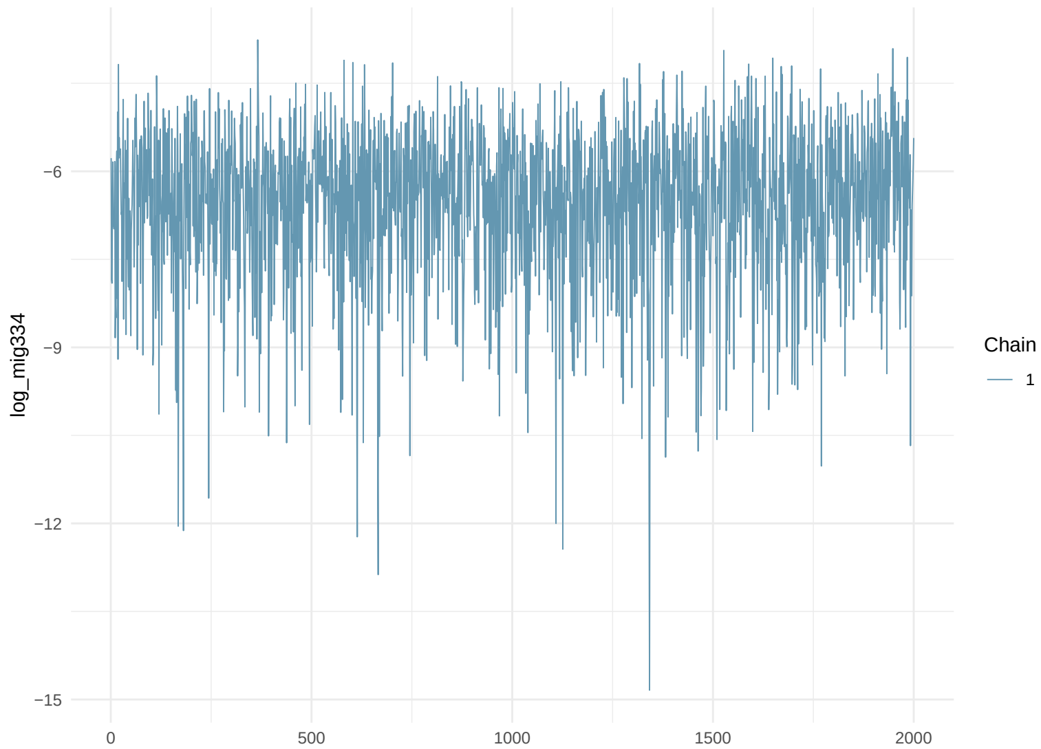
Trace Plot: log_mig334
