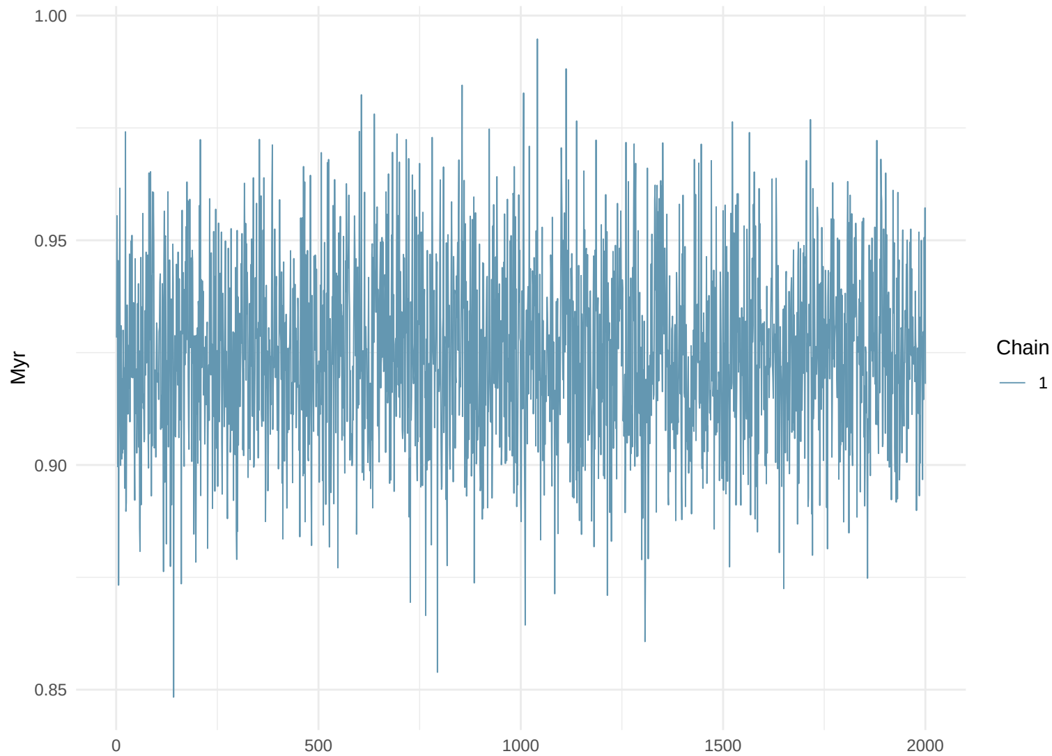
Trace Plot: Myr
