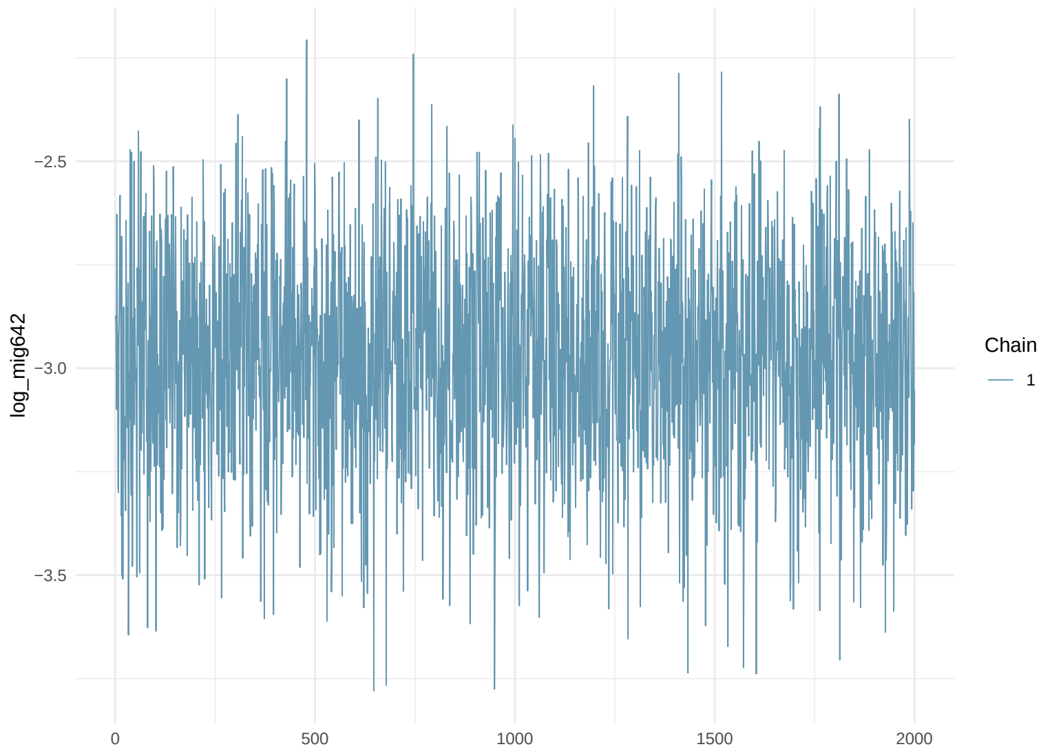
Trace Plot: log_mig642
