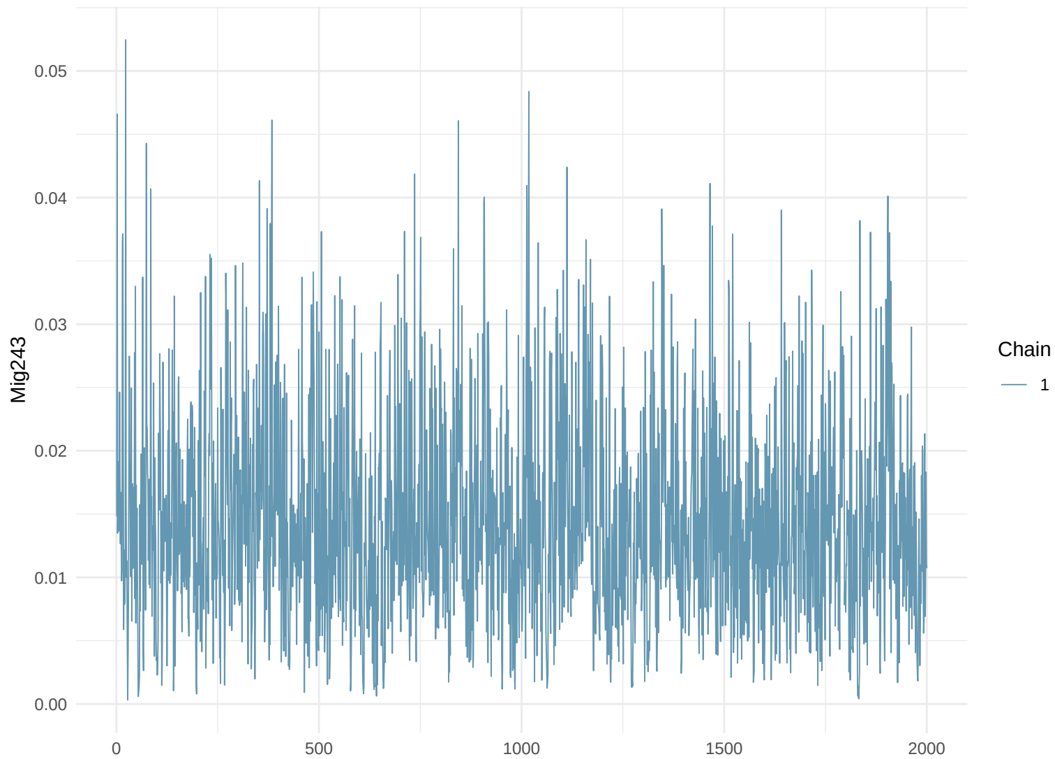
Trace Plot: Mig243
