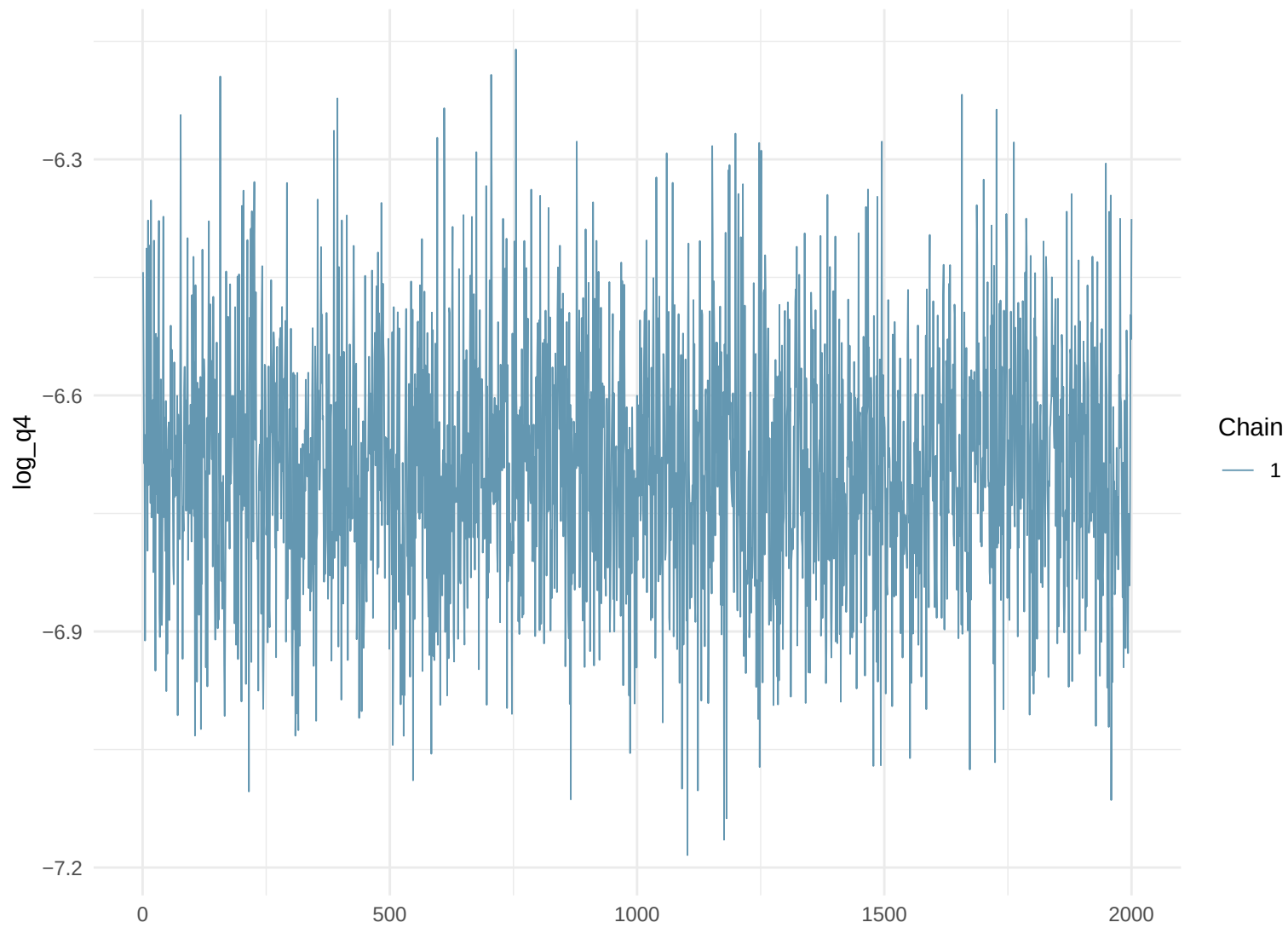
Trace Plot: log_q4
