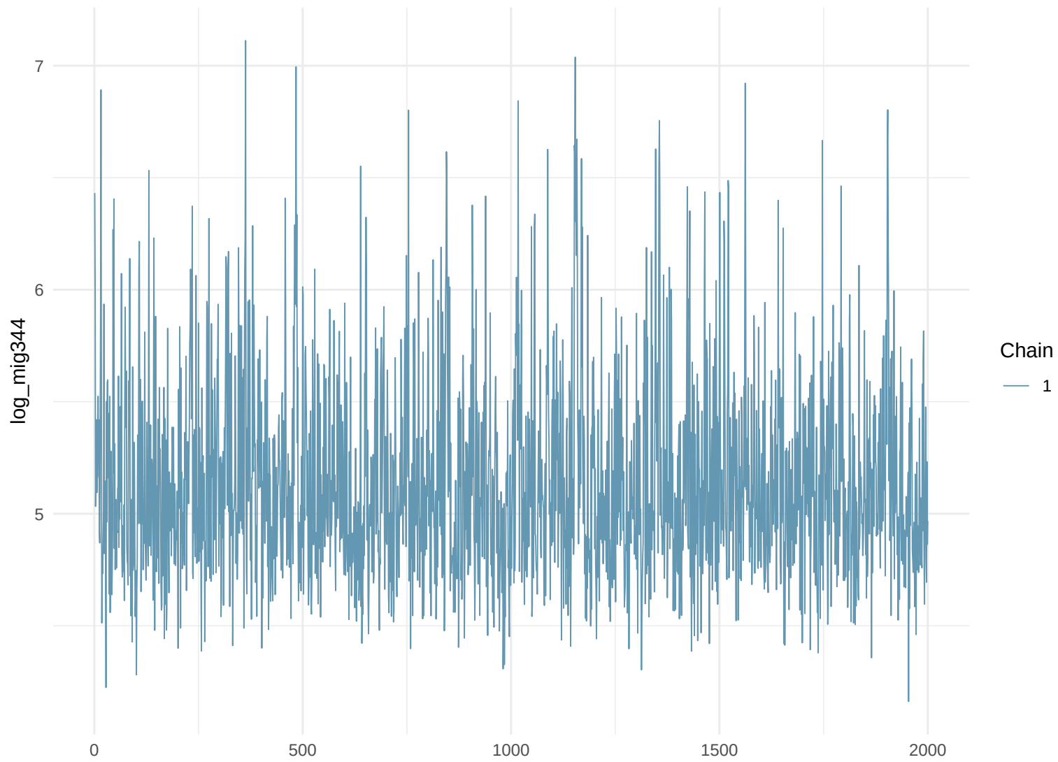
Trace Plot: log_mig344
