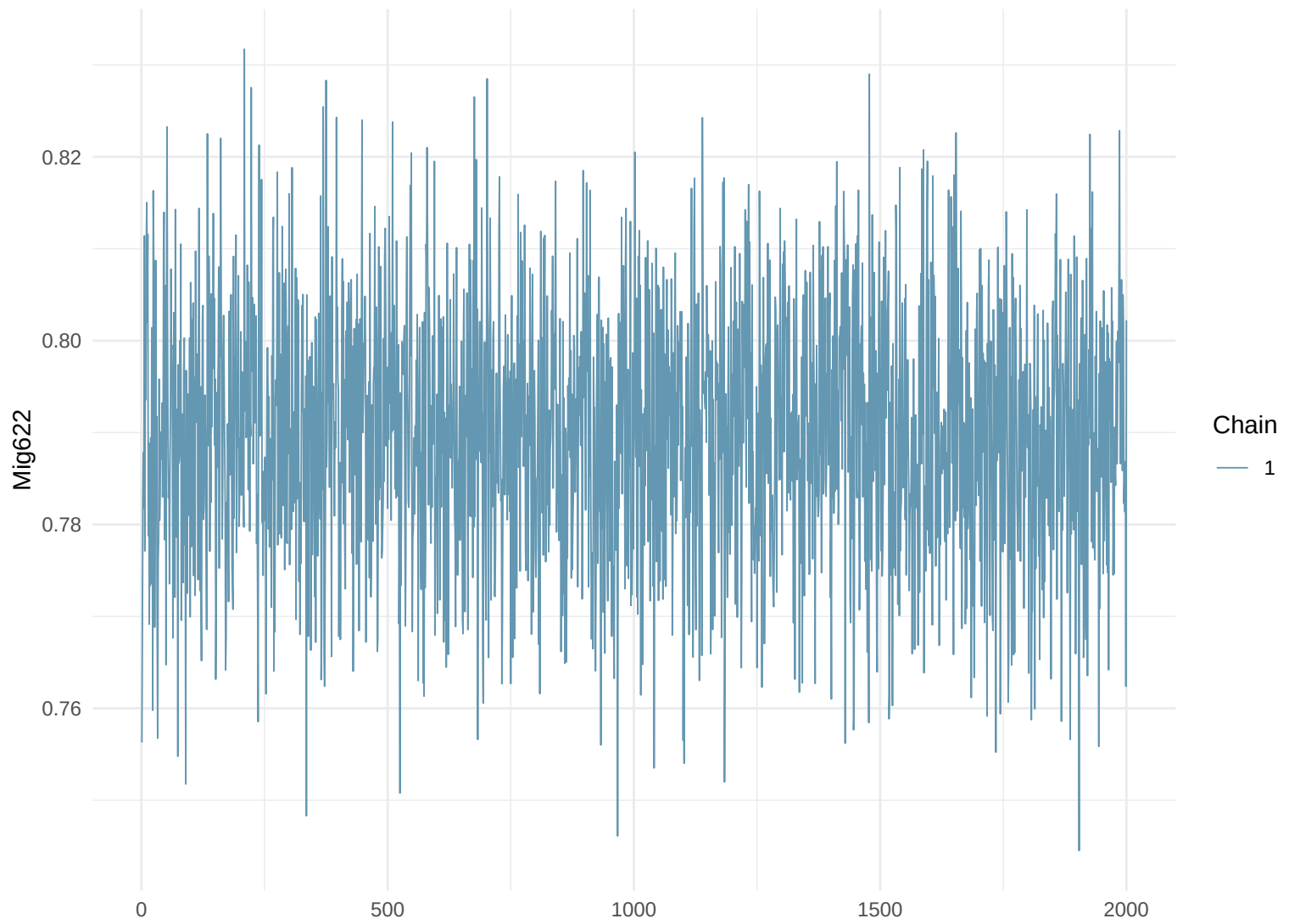
Trace Plot: Mig622
