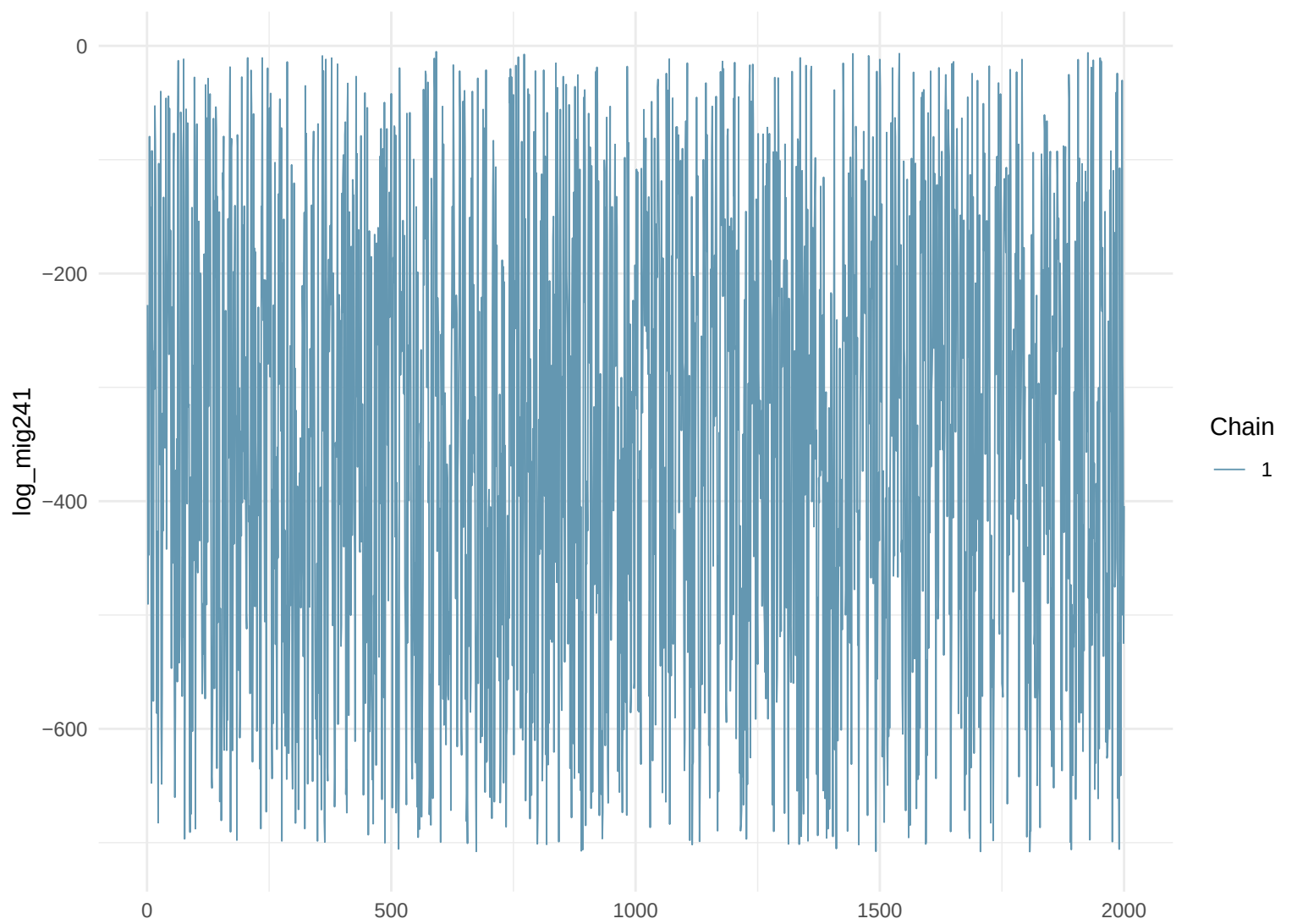
Trace Plot: log_mig241
