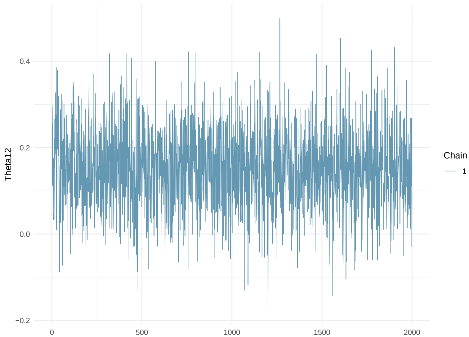
Trace Plot: Theta12
