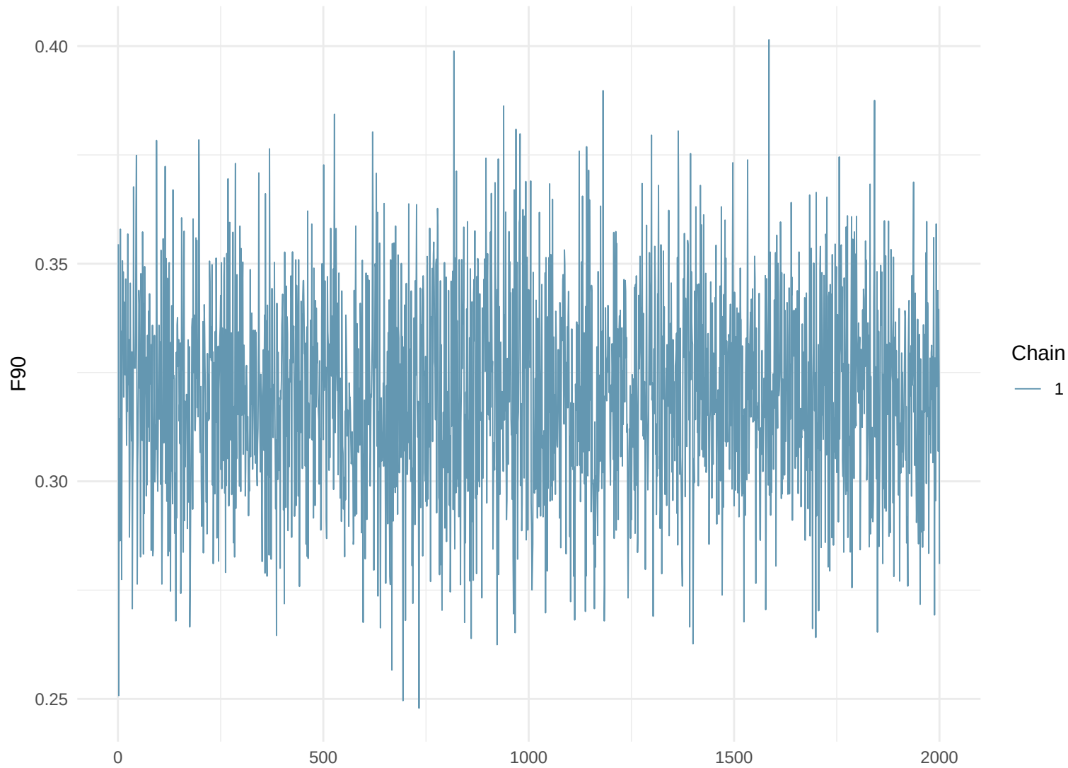
Trace Plot: F90
