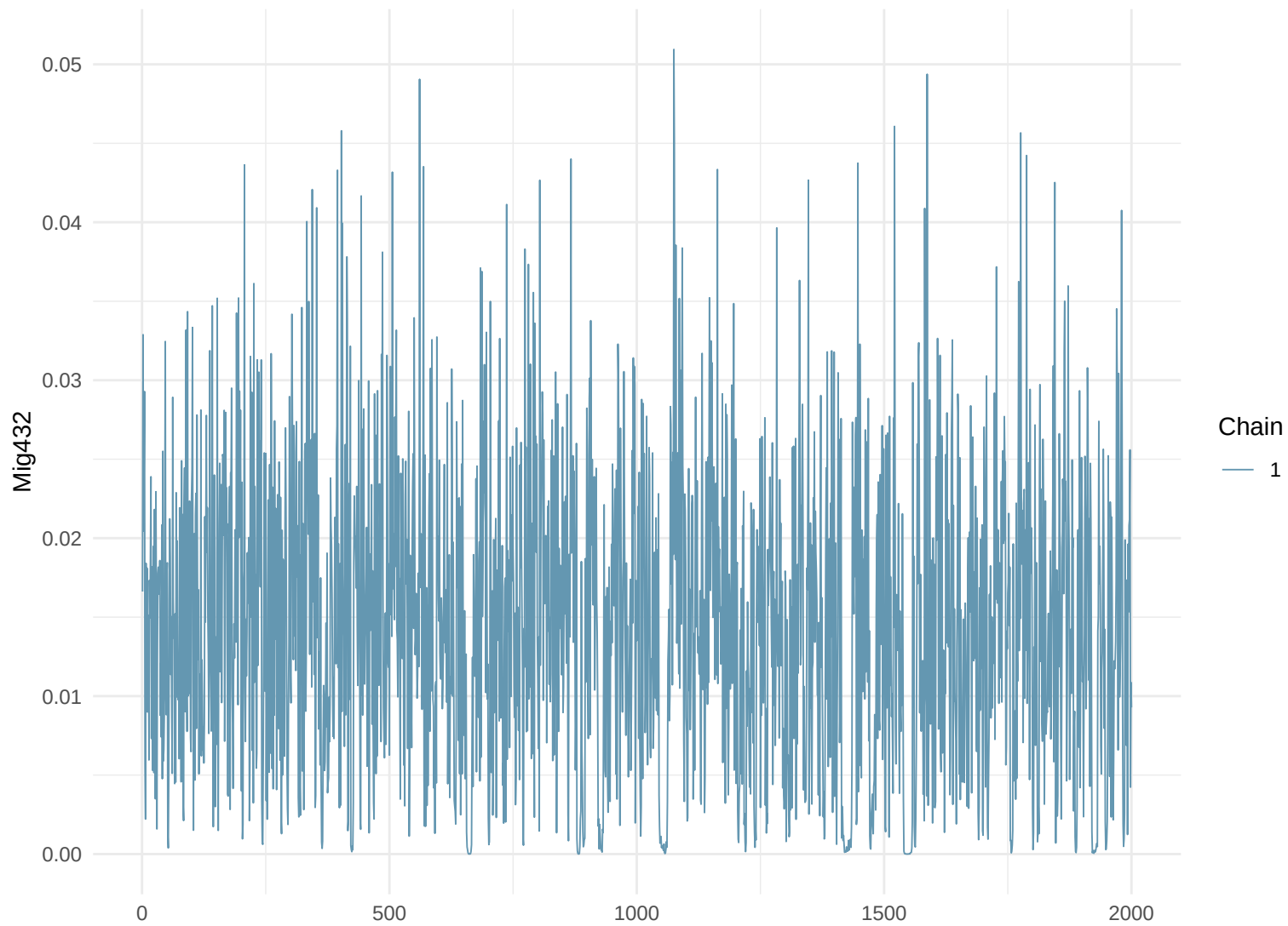
Trace Plot: Mig432
