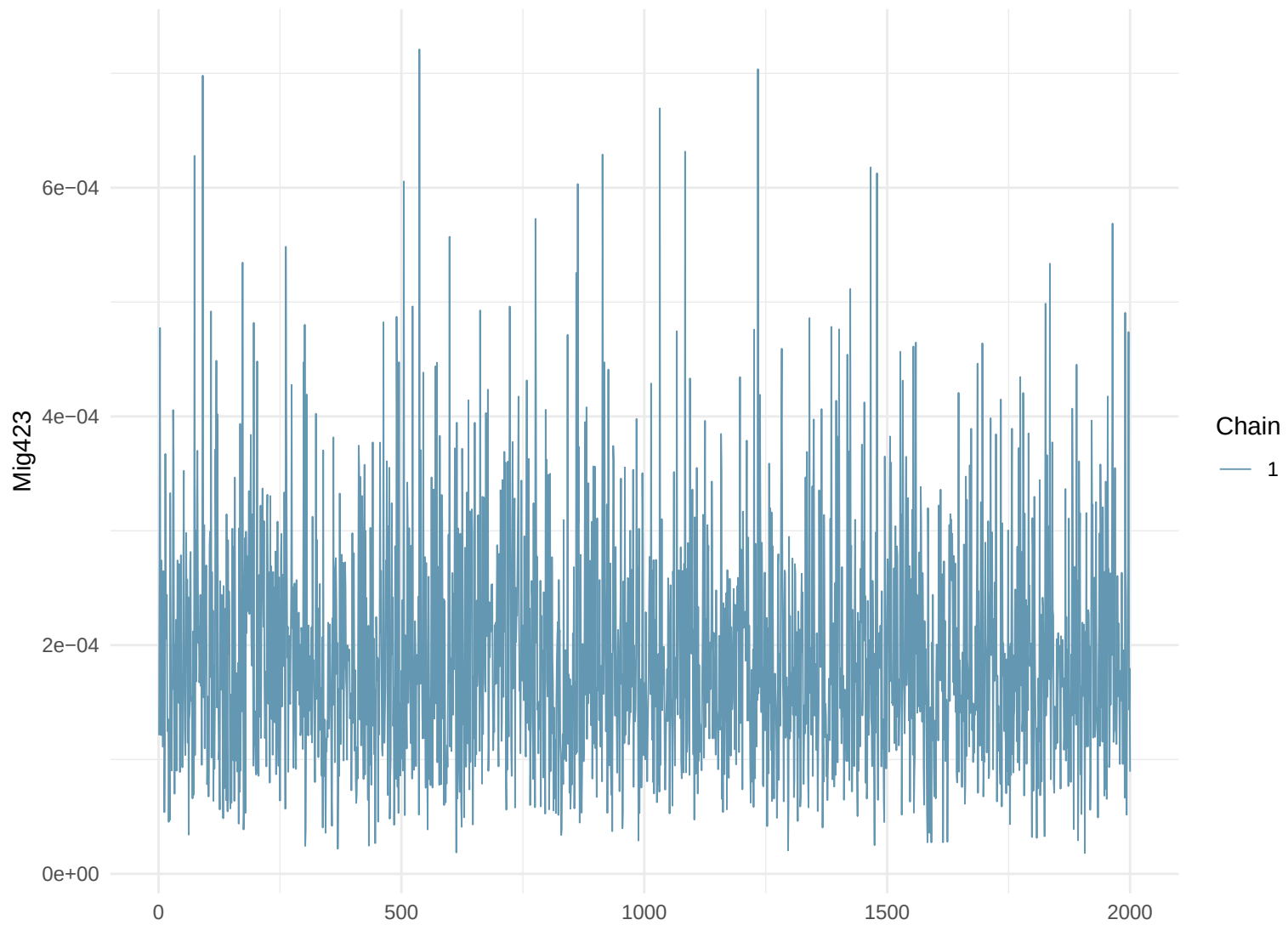
Trace Plot: Mig423
