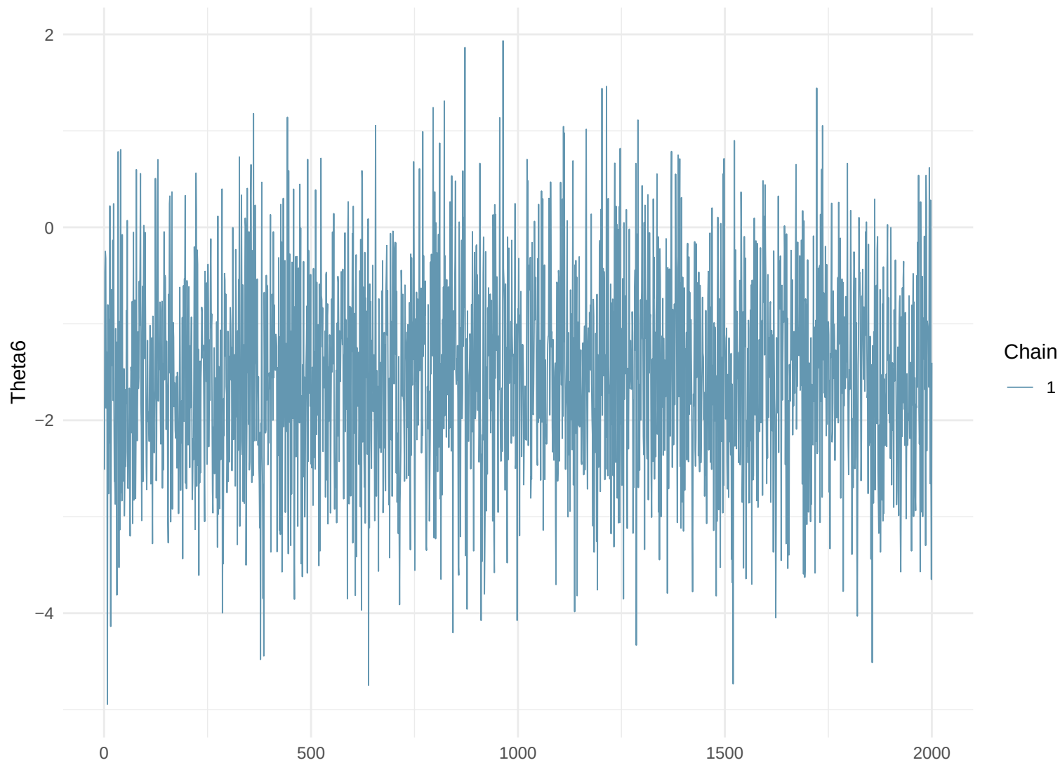
Trace Plot: Theta6
