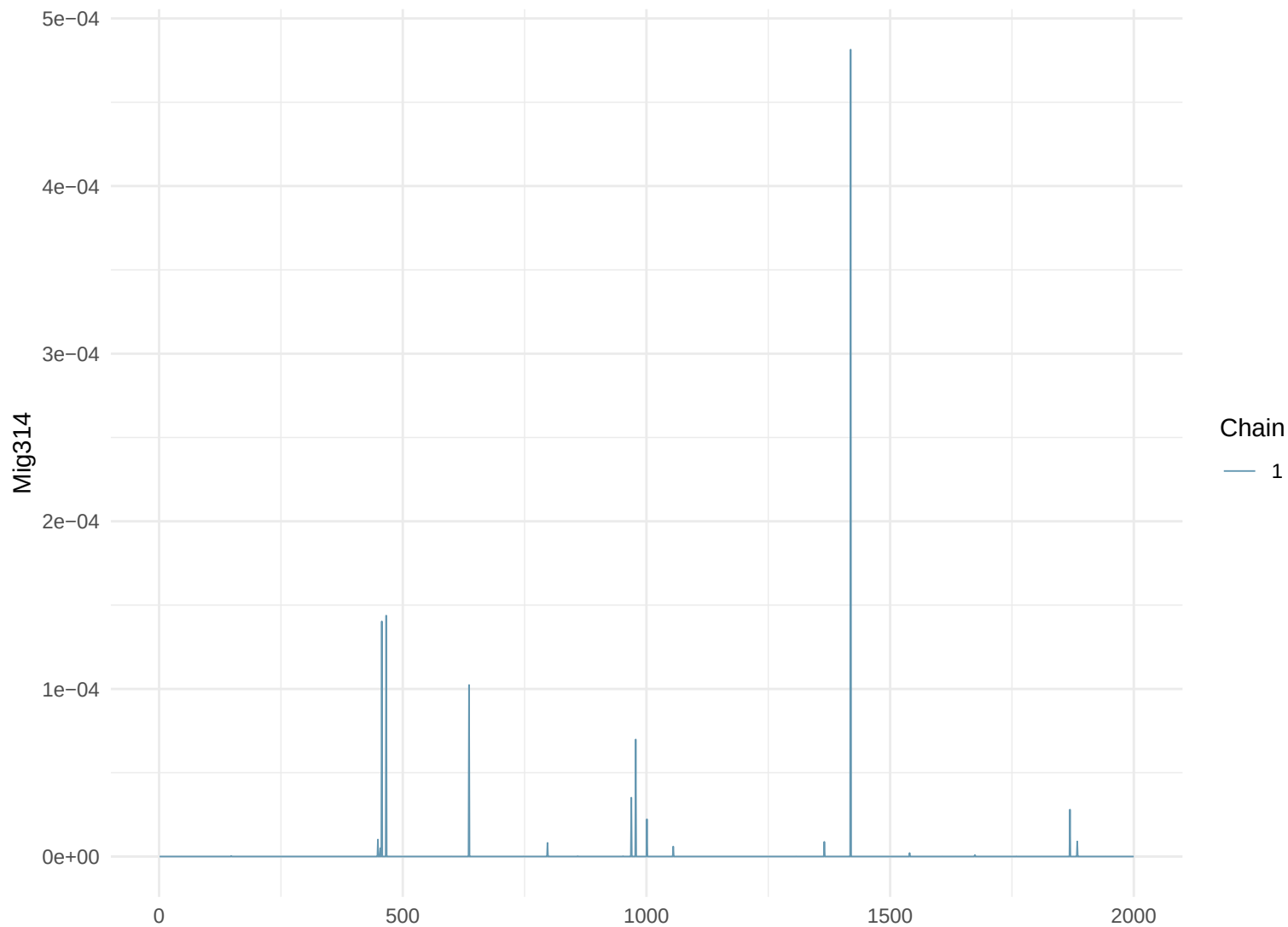
Trace Plot: Mig314
