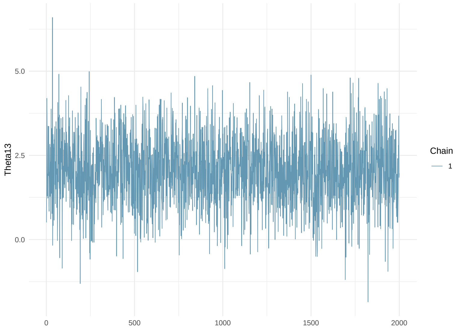
Trace Plot: Theta13
