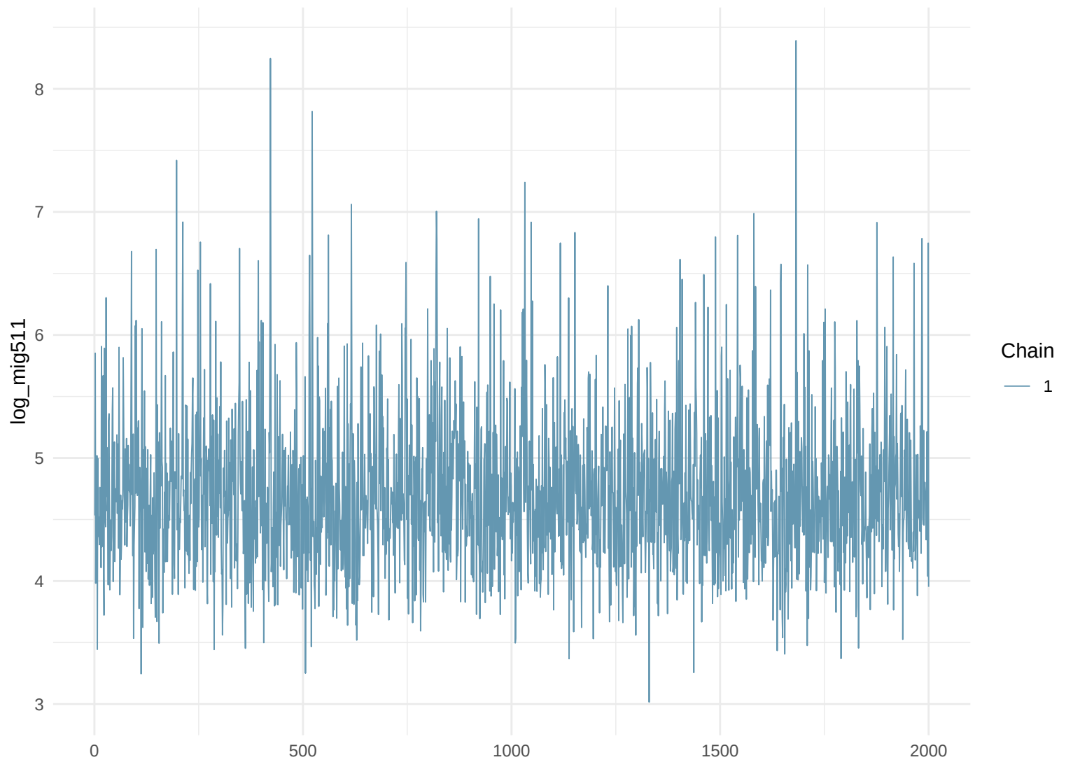
Trace Plot: log_mig511
