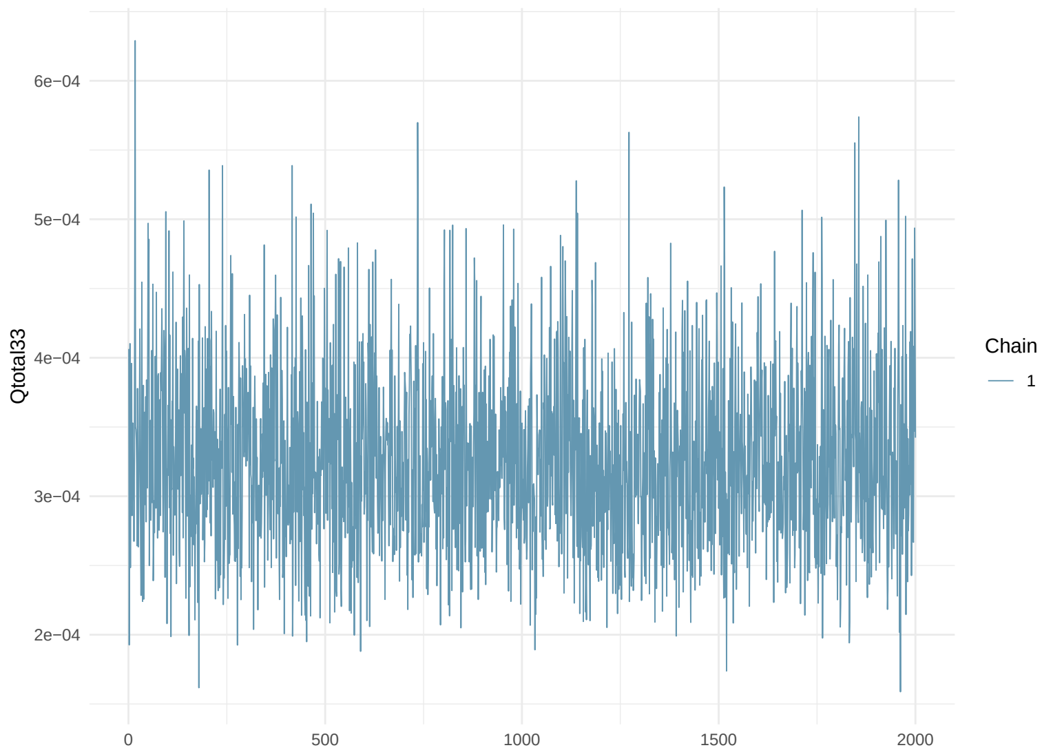
Trace Plot: Qtotal33
