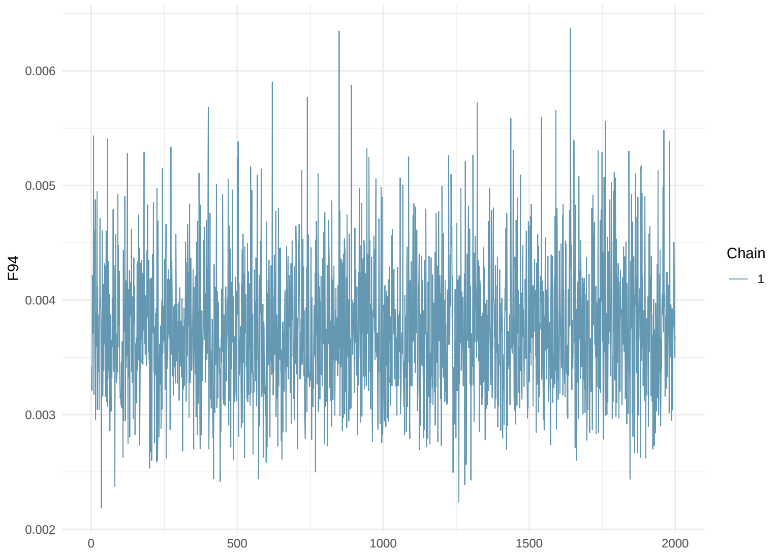
Trace Plot: F94
