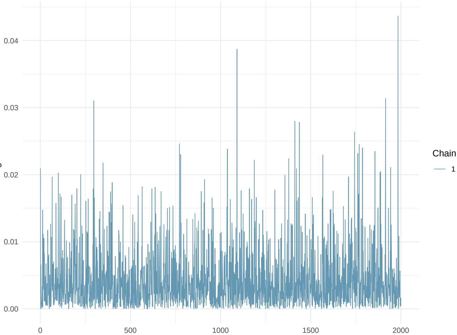
Trace Plot: Mig534
