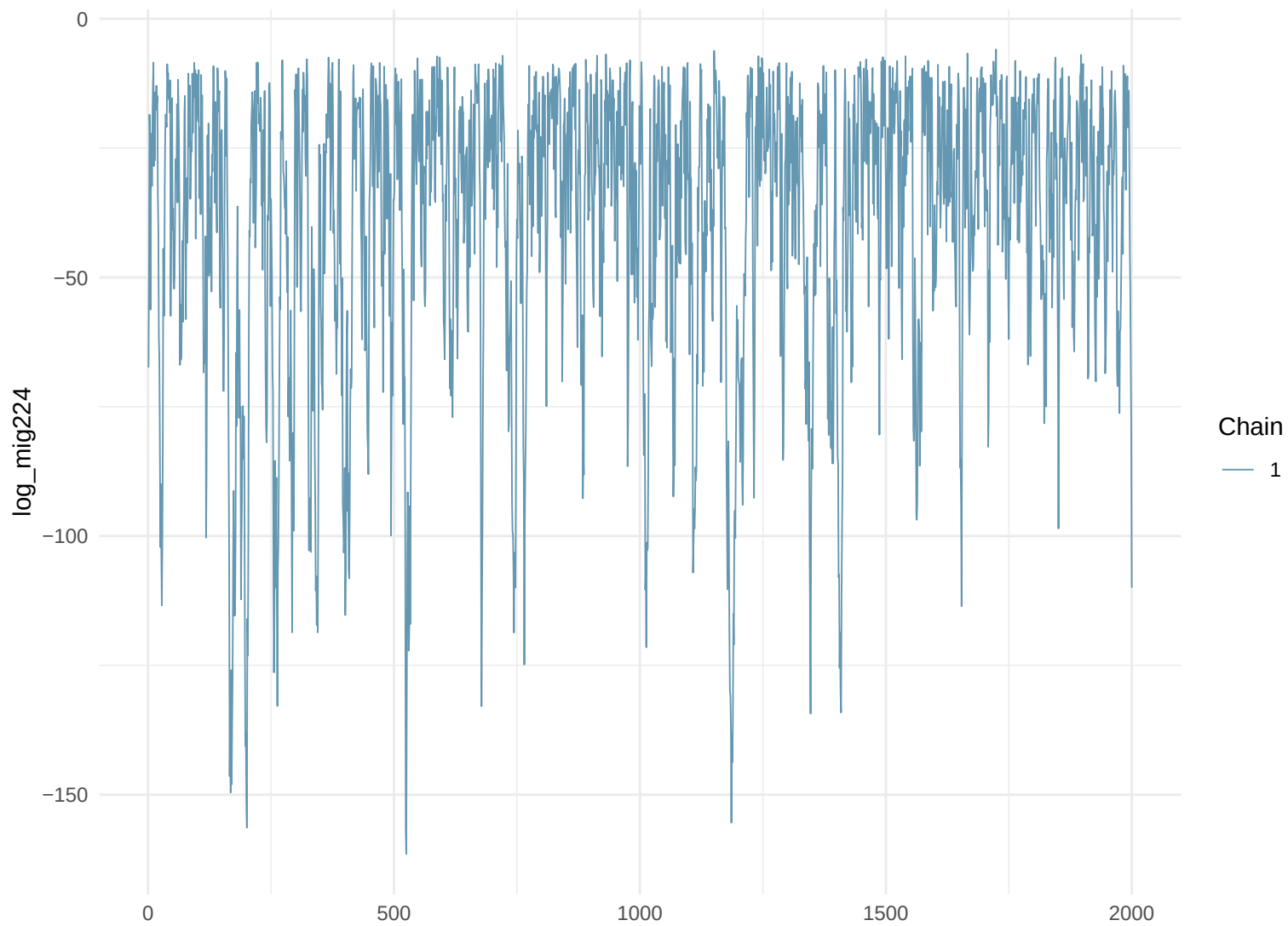
Trace Plot: log_mig224
