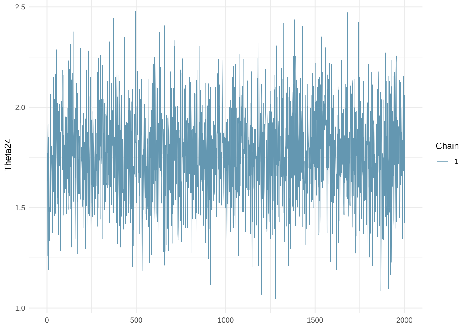
Trace Plot: Theta24
