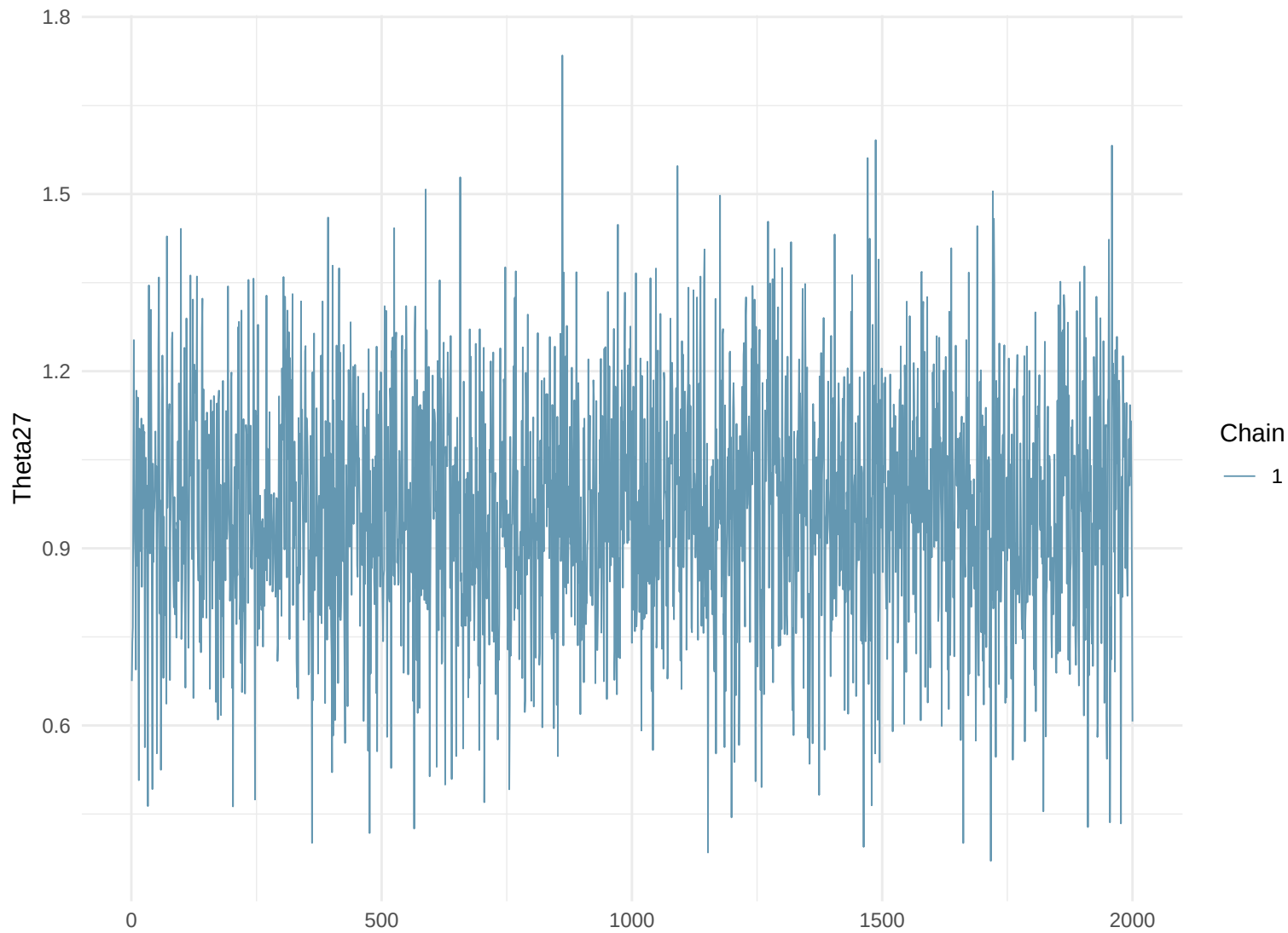
Trace Plot: Theta27
