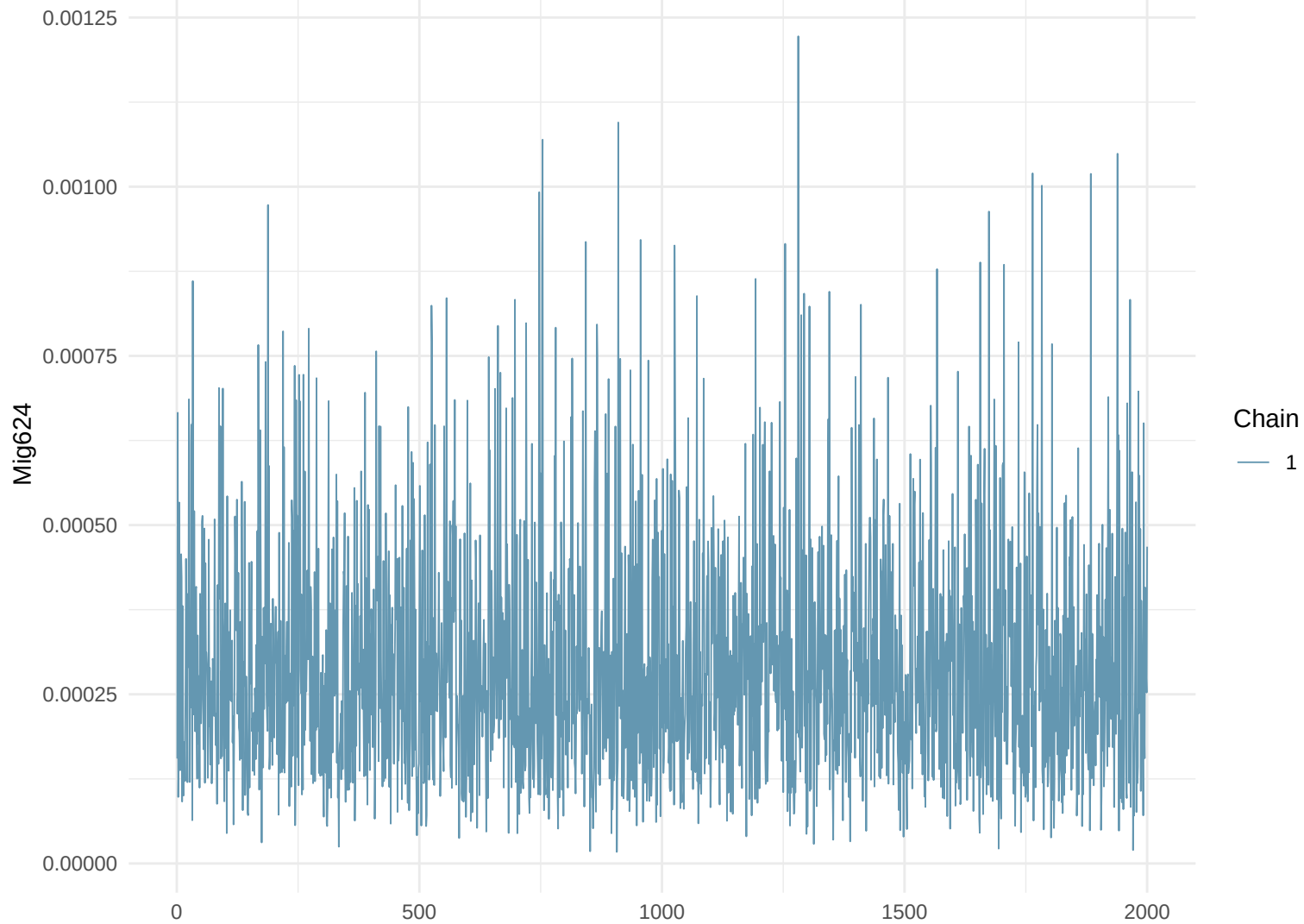
Trace Plot: Mig624
