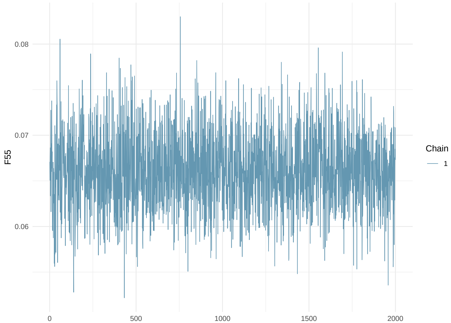
Trace Plot: F55
