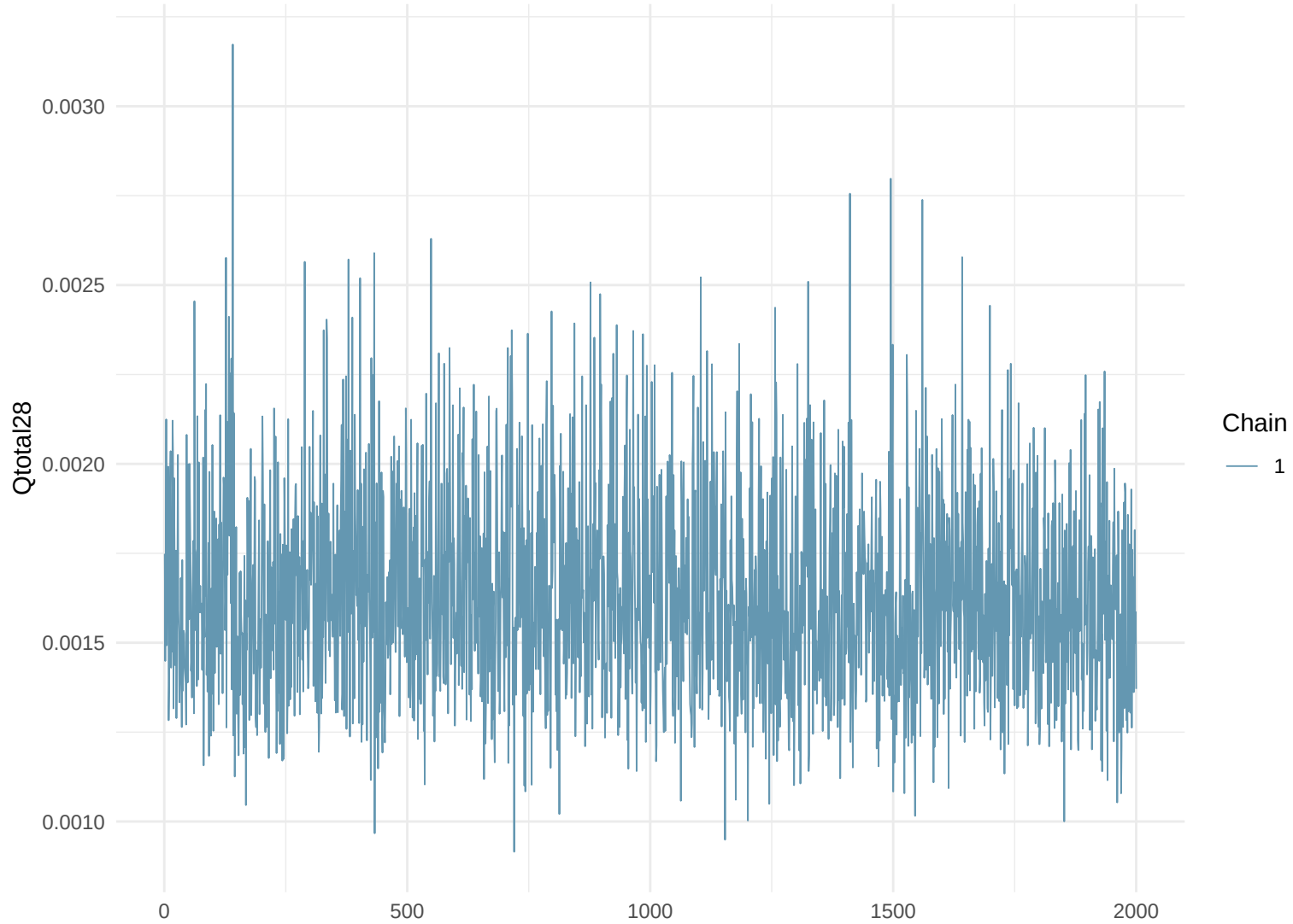
Trace Plot: Qtotal28
