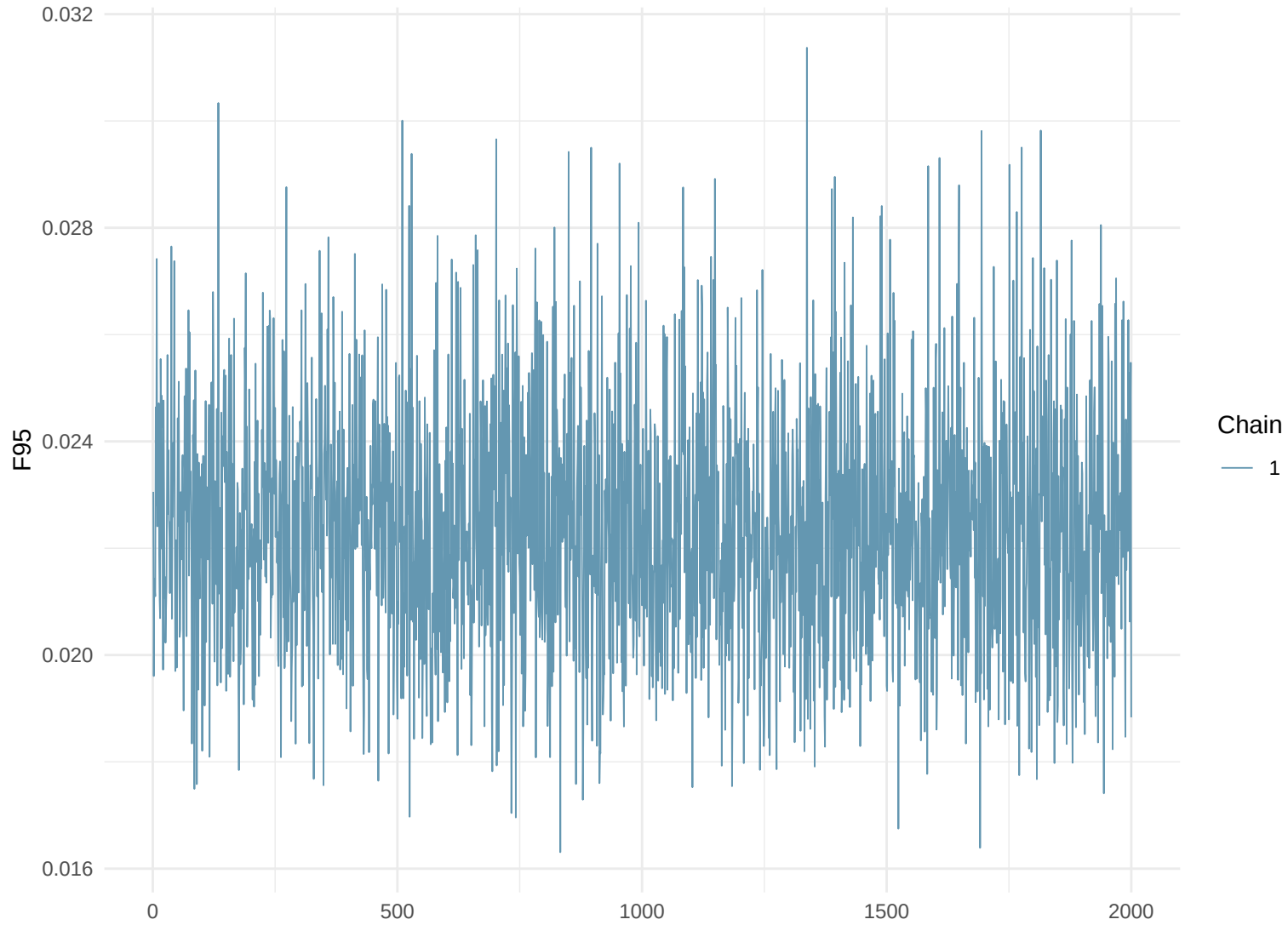
Trace Plot: F95
