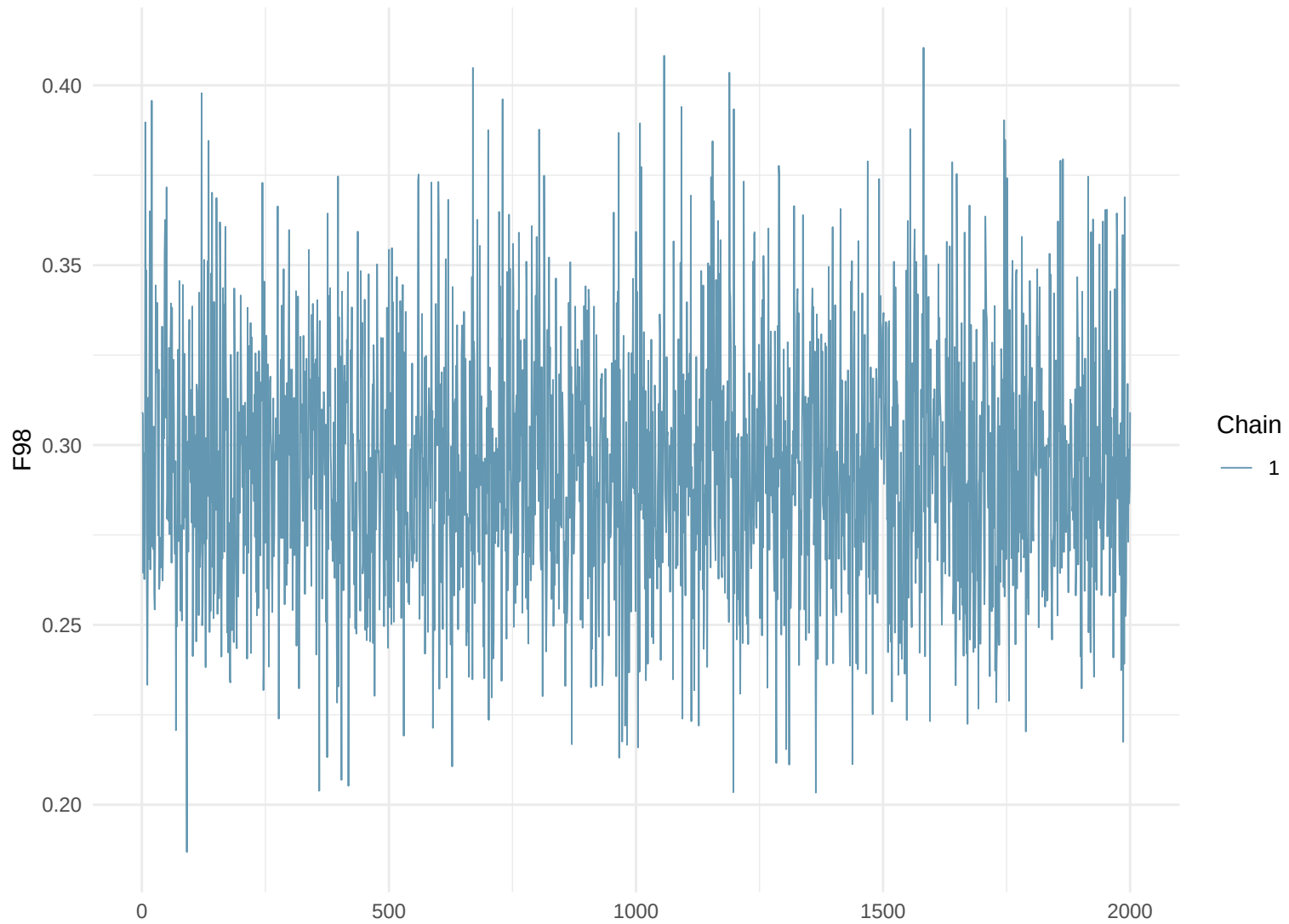
Trace Plot: F98
