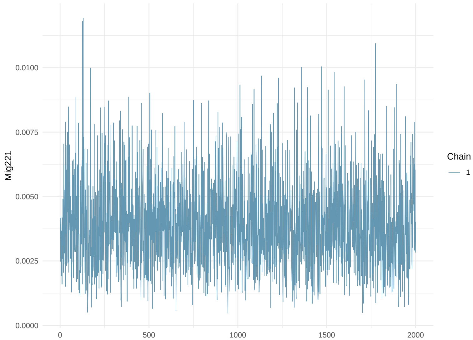
Trace Plot: Mig221
