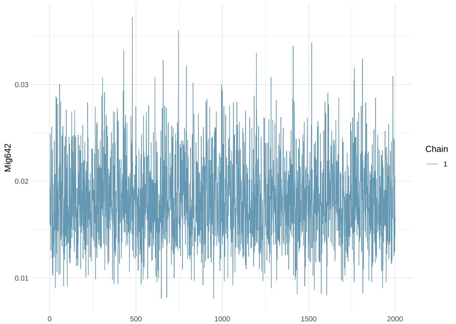
Trace Plot: Mig642
