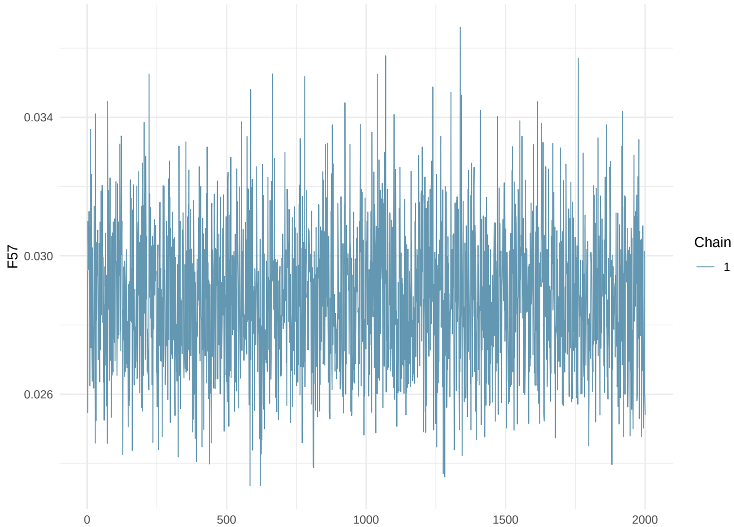
Trace Plot: F57
