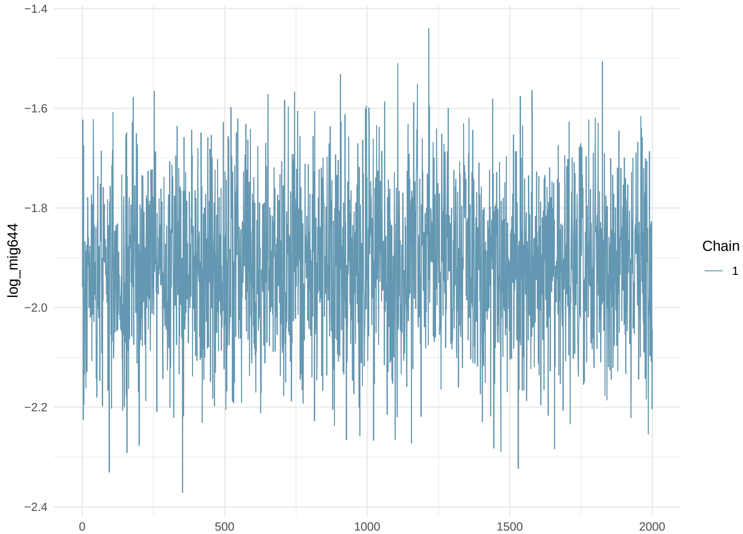
Trace Plot: log_mig644
