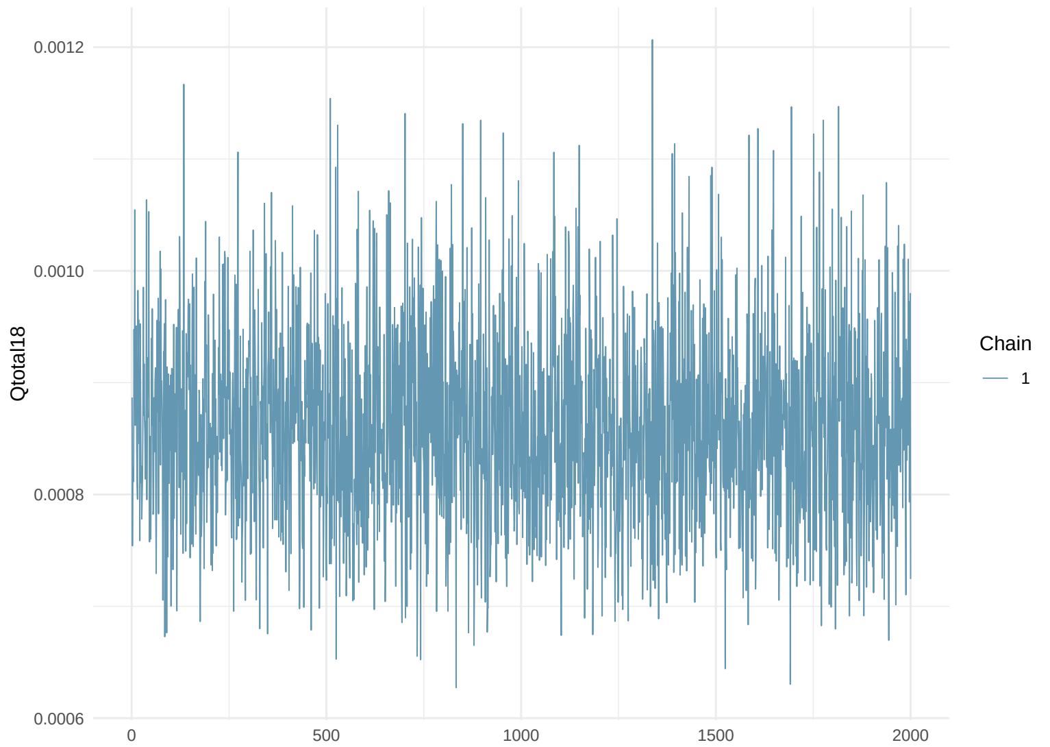
Trace Plot: Qtotal18
