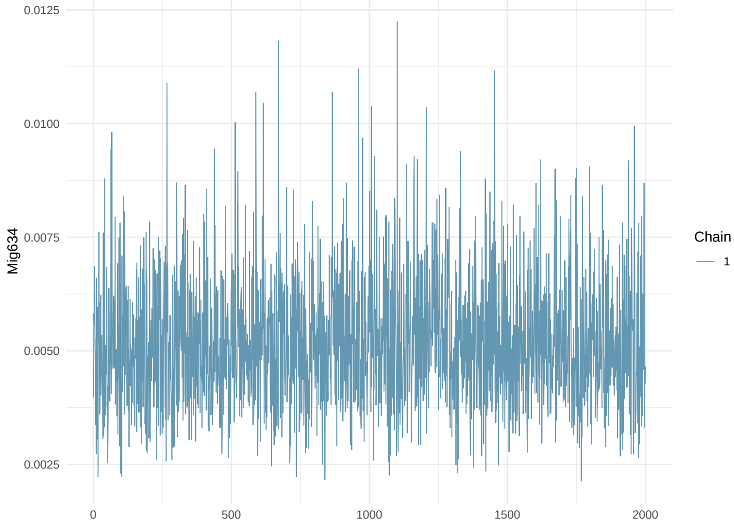
Trace Plot: Mig634
