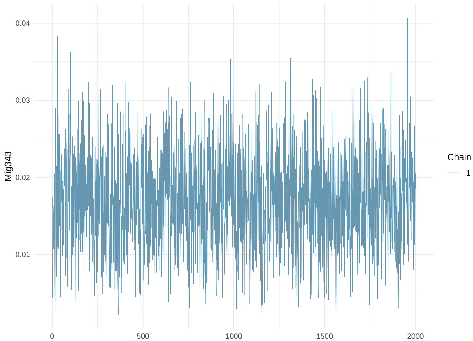
Trace Plot: Mig343
