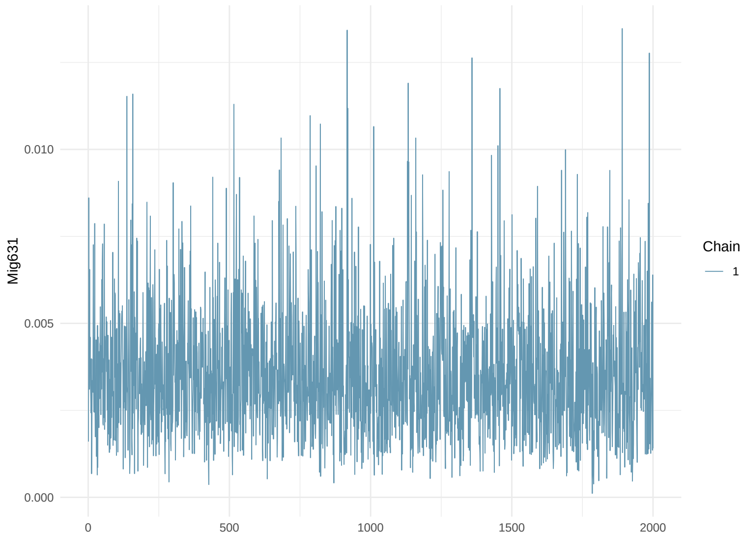
Trace Plot: Mig631
