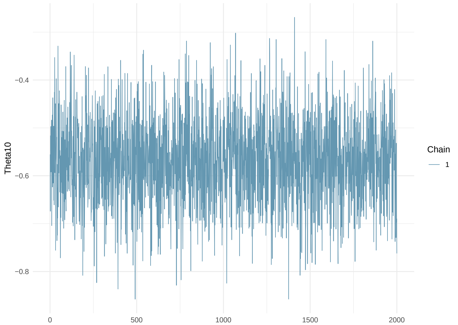
Trace Plot: Theta10
