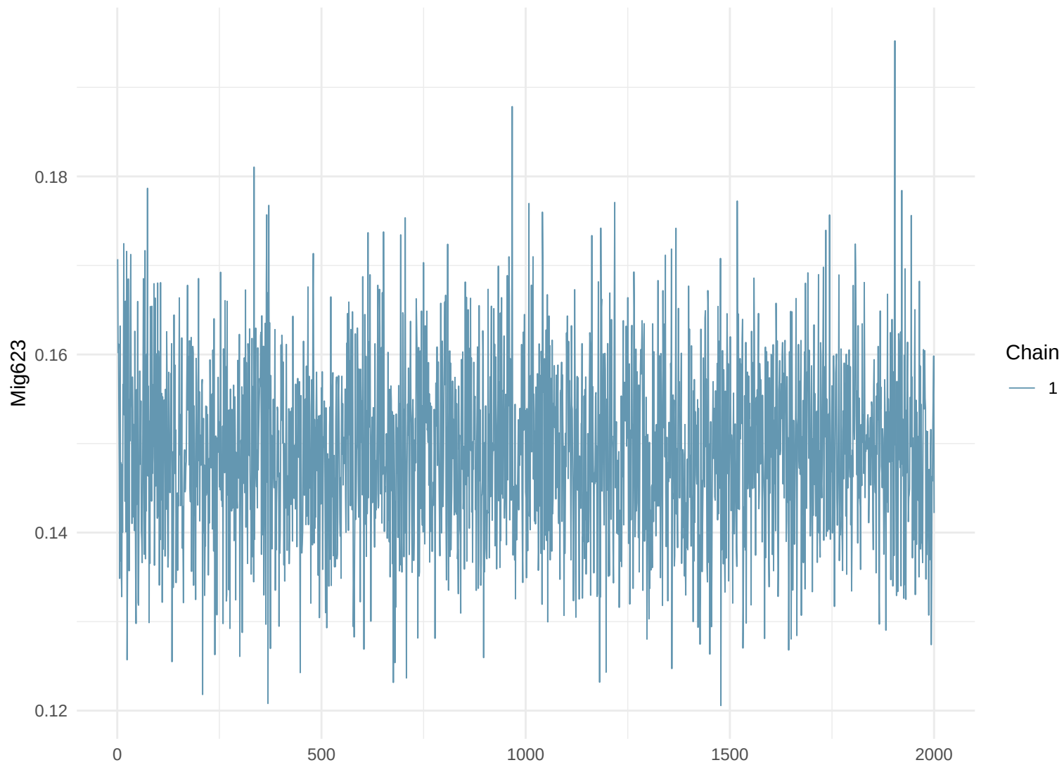
Trace Plot: Mig623
