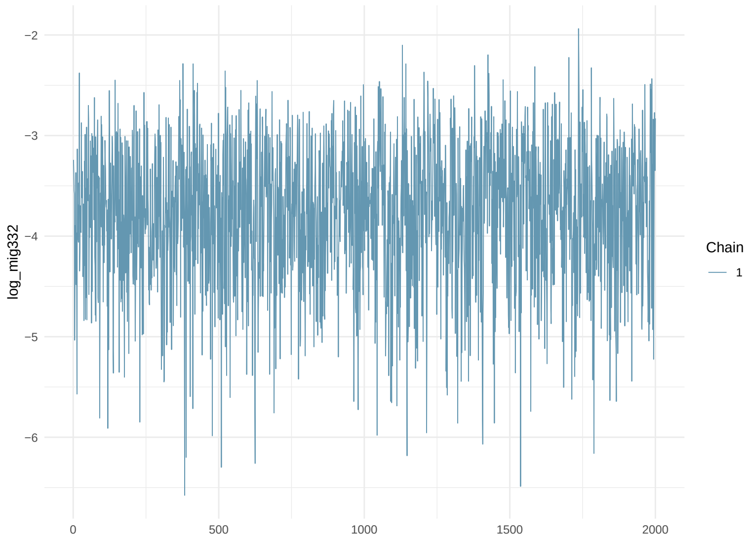
Trace Plot: log_mig332
