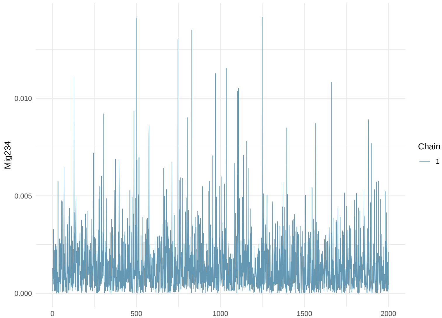
Trace Plot: Mig234
