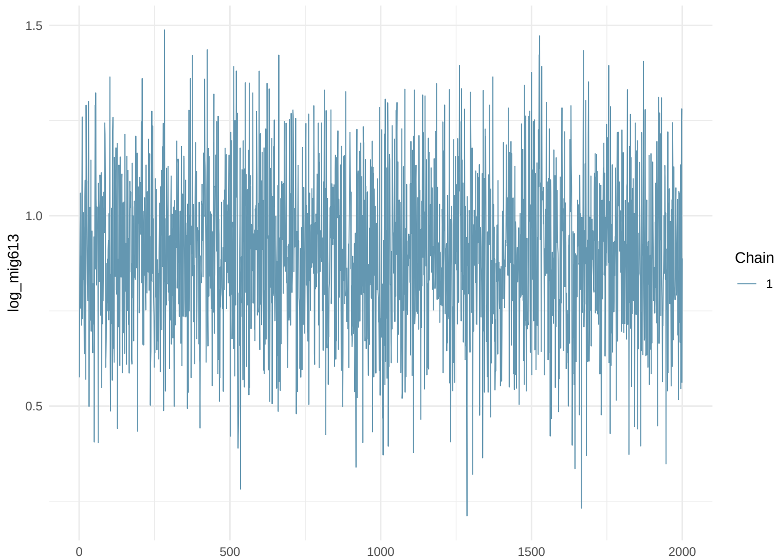
Trace Plot: log_mig613
