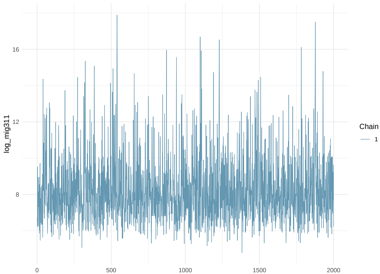
Trace Plot: log_mig311
