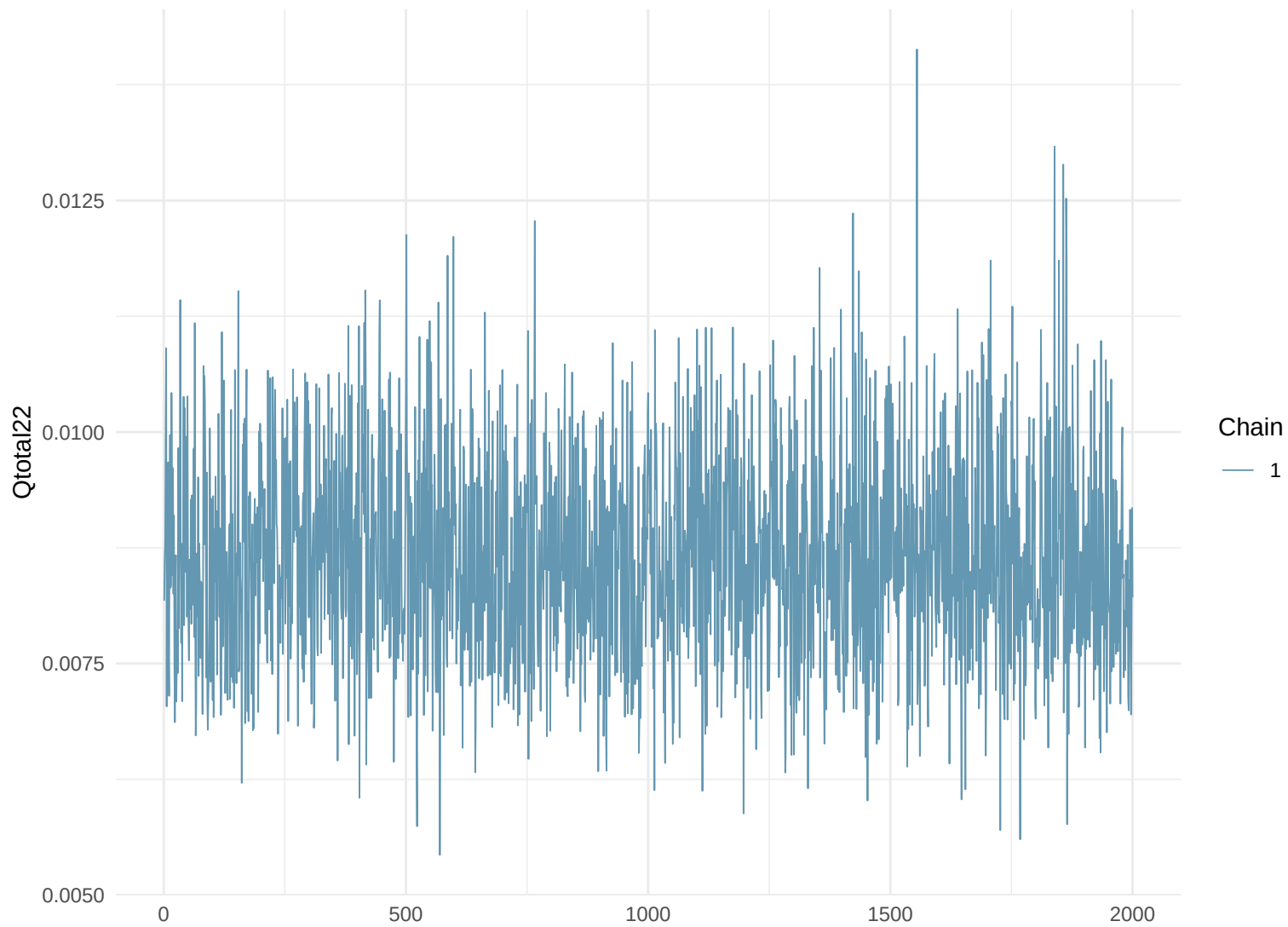
Trace Plot: Qtotal22
