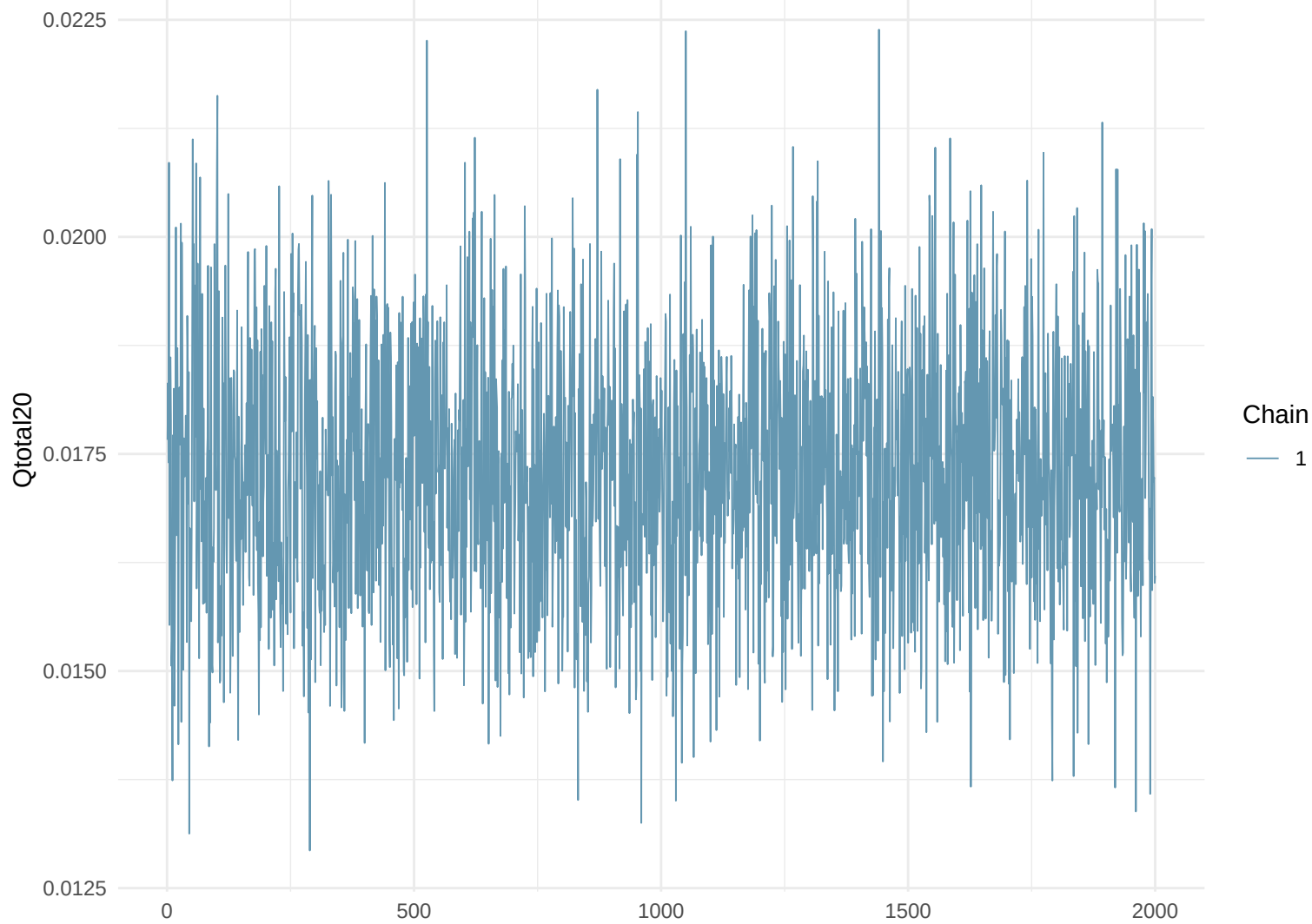
Trace Plot: Qtotal20
