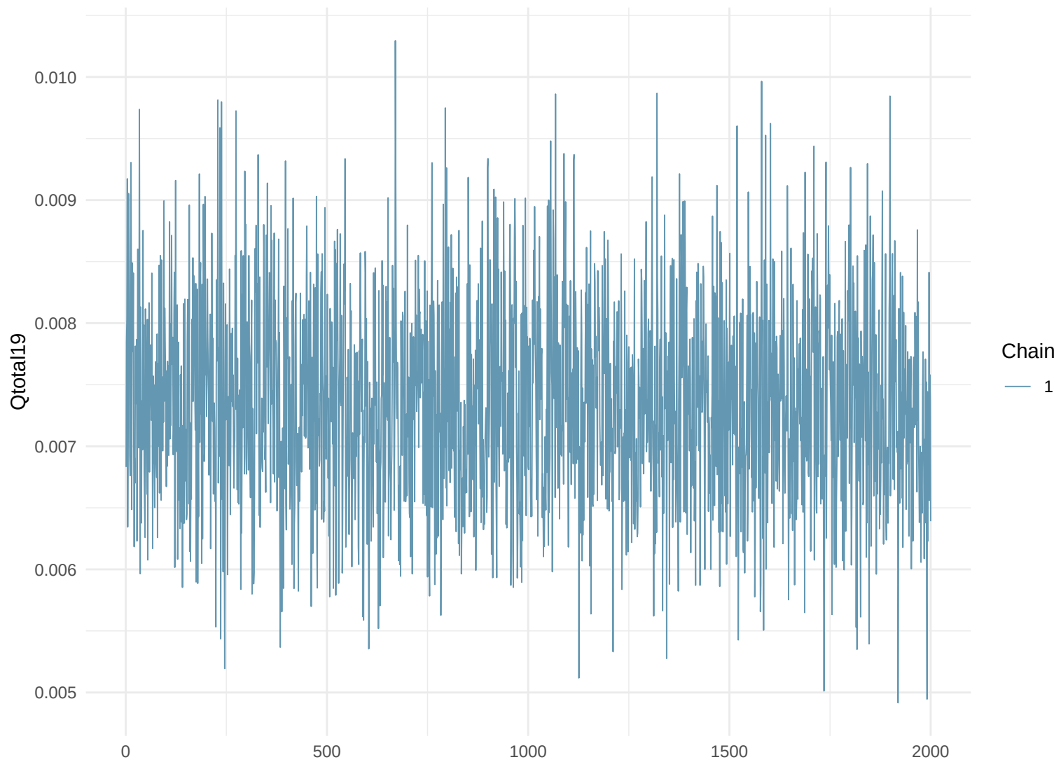
Trace Plot: Qtotal19
