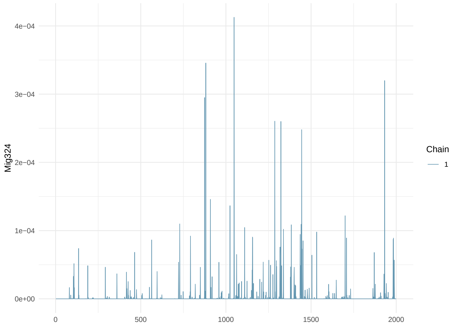
Trace Plot: Mig324
