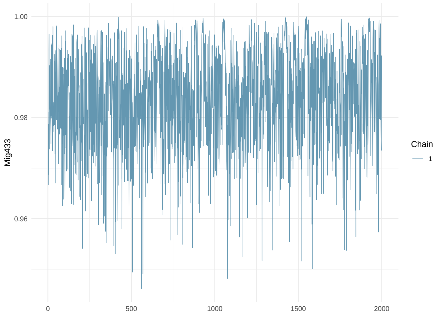
Trace Plot: Mig433
