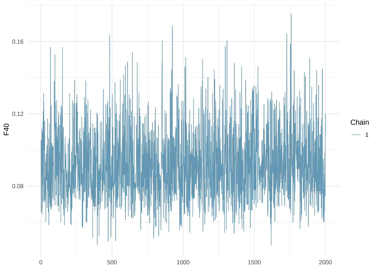
Trace Plot: F40
