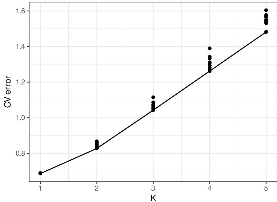
ADMIXTURE cross-validation across replicates
