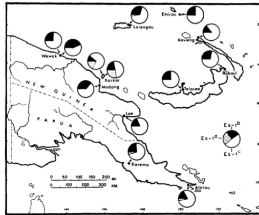
FIGURE 2. The geographic variation in the allelic frequencies at the esterase-I locus in populations of Aplonis metallica . The frequency of an allele in a population is proportional to the area of the circle occupied by its symbol. Allelic frequencies at Karkar Island localities 2 and 3 are essentially identical for the purpose of illustration (see table 2).
