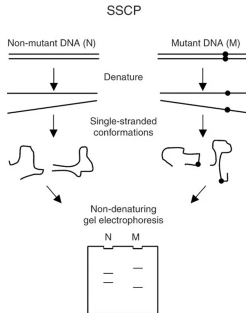
Figure 3.2: The basis of single-stand conformation polymorphisms (Gasser et al. (2006)).
