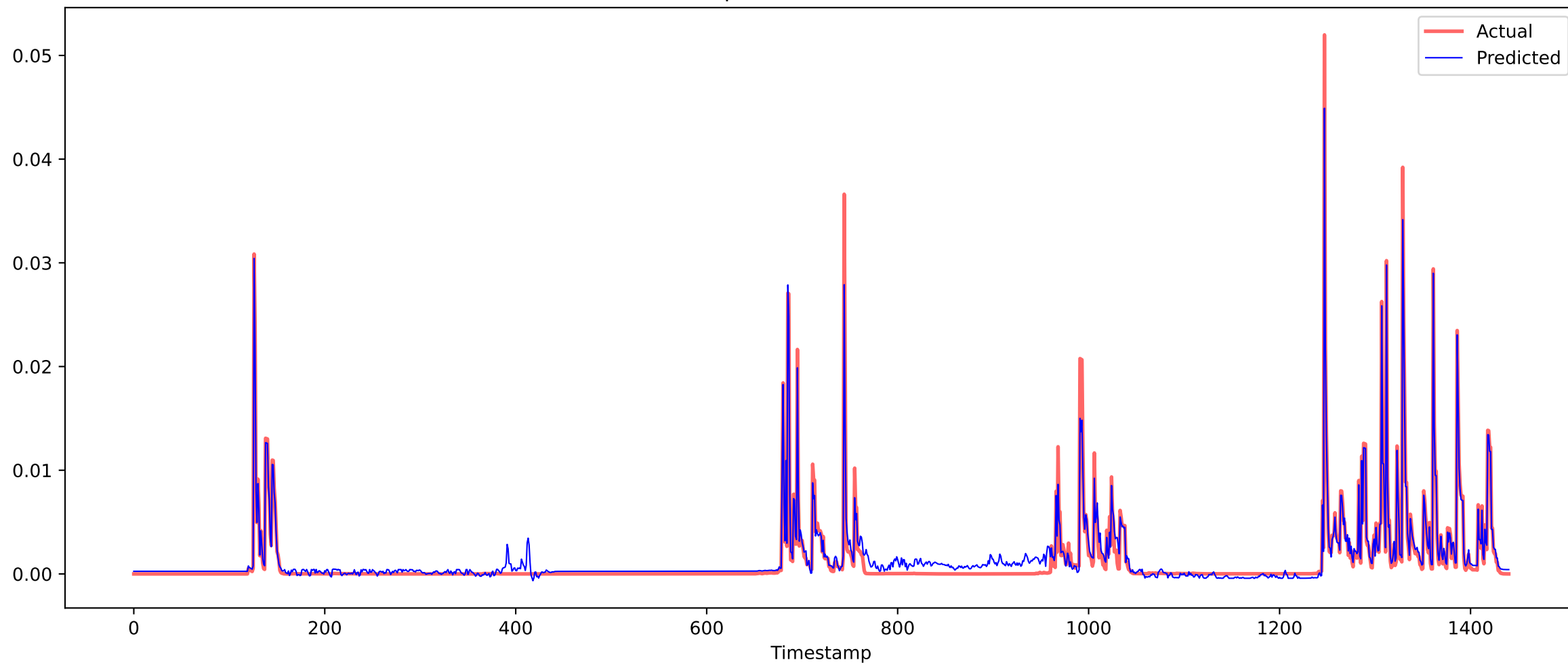
Test prediction node dist64
