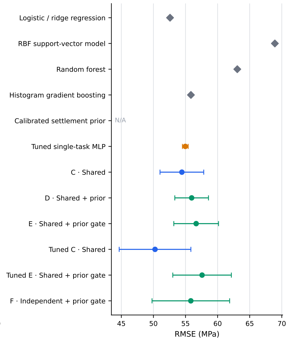
b) Rock lower is better
