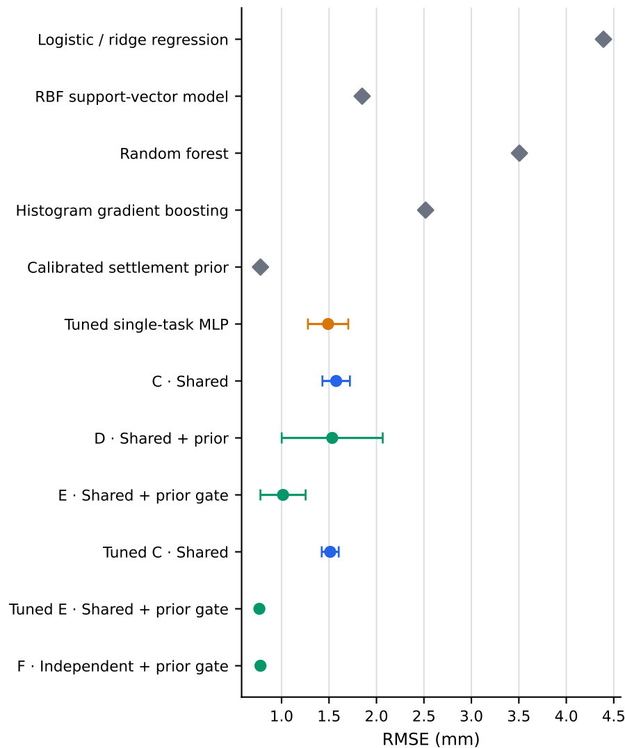
c) Settlement lower is better
