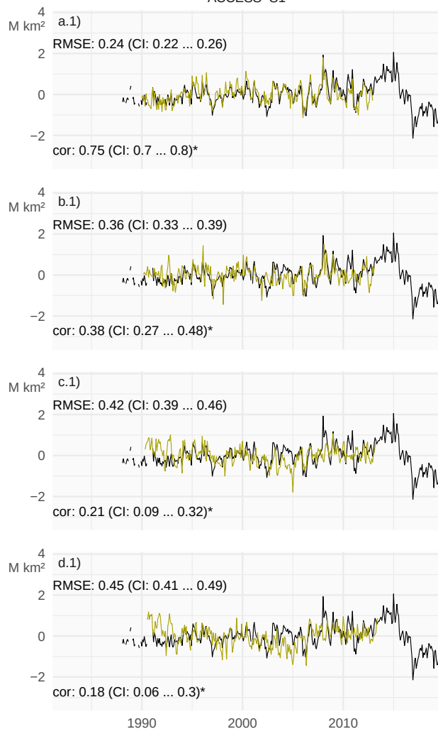
ACCESS-S1
