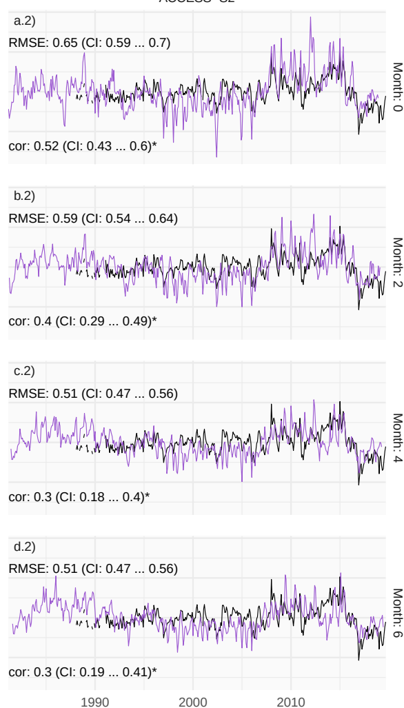
ACCESS-S2
