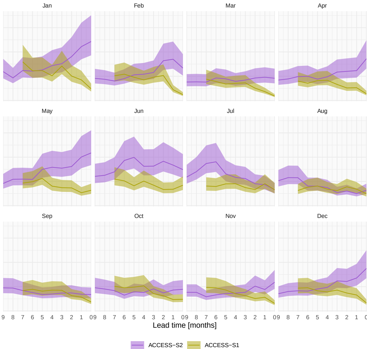
Sea-ice extent anomaly RMSE:
