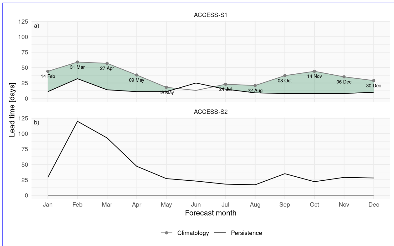
Figure A10. Minimum lead time at which each forecast's mean RMSE becomes lower than the lower bound of the 95% confidence interval of persistence forecast RMSE (black lines) and maximum lead time at which each forecast's mean RMSE remains lower than the lower bound of the 95% confidence interval of climatological forecast RMSE (gray lines). Green shading indicates the window where forecasts outperform both persistence (lead times longer than black line) and climatology (lead times shorter than gray line). Text labels show the date corresponding to the maximum lead time at which each forecast outperforms climatology. Using CDR as the validation dataset.
