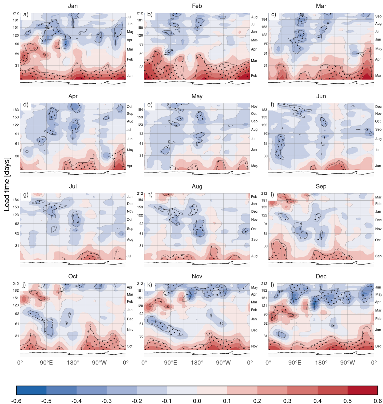
Figure A12. RMSE-MSE skill score of ACCESS-S1 forecasts with climatological forecast as reference computed on 15 meridional slices 24° wide as a function of lead time and longitude. Regions where the difference of means between ACCESS-S1 RMSE and climatological RMSE are significant at p-value < 0.05 are stippled. Antarctica's coastline is shown at the bottom of each panel for reference. Values were smoothed with an 11-day running mean to improve readability. Note that the vertical axis uses a 1.5 root transformation to expand the shorter lead times.
