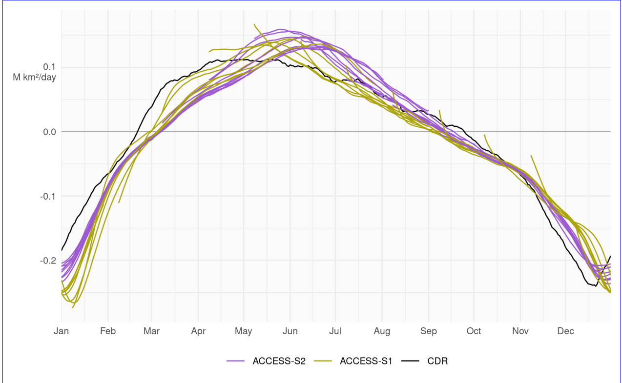
Figure 2. Mean daily sea-ice extent growth ( 10^6 km^2/day ) in ACCESS-S1 (green) and ACCESS-S2 (purple) hindcasts and observations (black), computed as the mean daily differences in sea-ice extent between each date and the next for each forecast month. Values are smoothed with a 11-day running mean.
