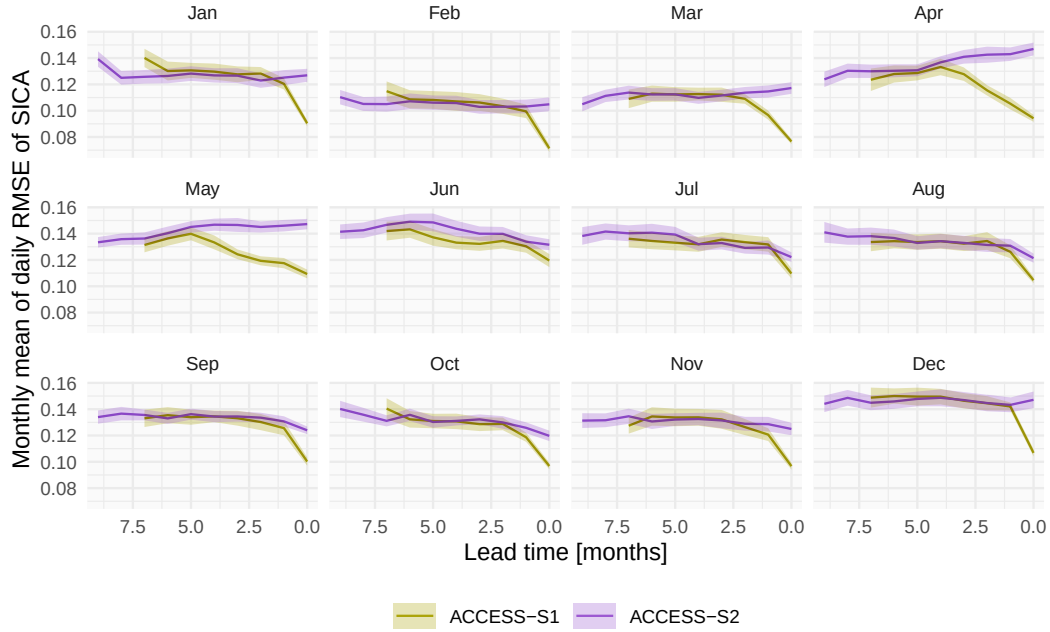
Figure 1: Mean RMSE of mean daily RMSE of sea-ice concentration anomalies. Each panel indicates the target month. Note the reverse horizontal axis.
