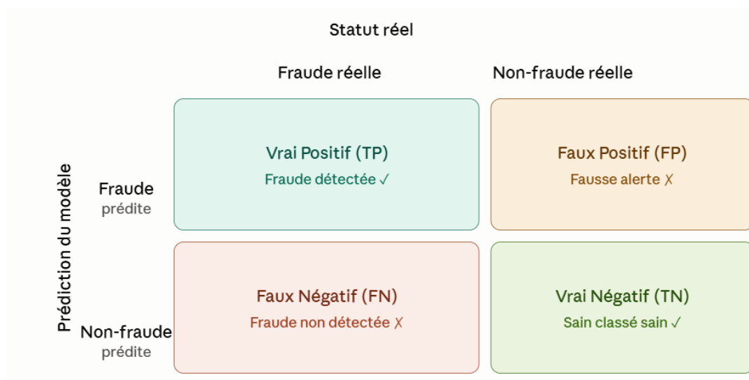
FIGURE 3.1 – Matrice de confusion
