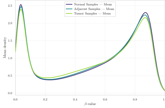
Figure 3.6: Group-wise mean \beta -value density.
