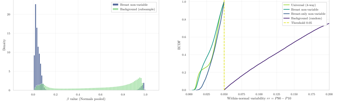
(a) Beta-value density for non-variable CpGs (breast tissue) versus genomic background.
