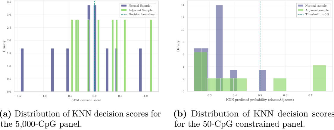
Figure 6.1: Score distributions for Normal and Adjacent samples under the full 5,000-CpG panel and the compressed 50-CpG subset in GSE69914.
