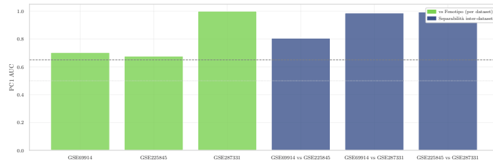
Figure 6.10: PC1 discriminative power for phenotype separation (Normal vs. Adjacent, within each dataset) and for batch separation (between datasets), reported as AUC. In all pairwise comparisons, dataset identity is at least as separable as biological class.
