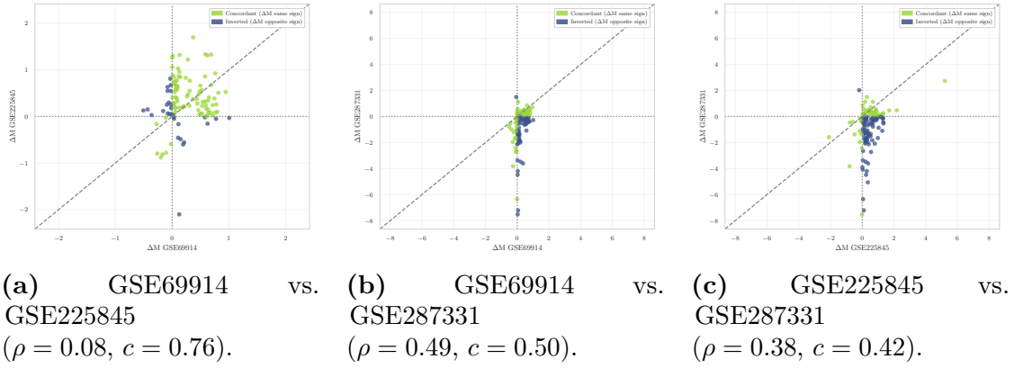
Figure 6.12: Pairwise \Delta M (Adjacent – Normal) concordance scatter plots on the shared CpG intersection. Each point is one CpG; axes show the mean \Delta M computed independently in each cohort.
