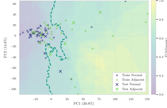
Figure 6.1: Projection of the KNN decision surface onto PC1–PC2 (explaining 30.8% and 14.8% of variance, respectively). Train and test samples from both classes overlap extensively, with no geometrically separable structure.
