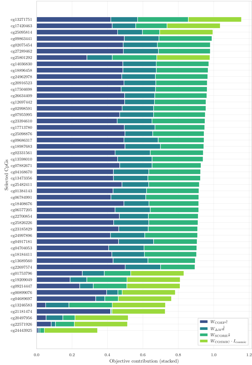
Figure 6.7: Component-wise decomposition of the MILP objective for the selected 50-CpG panel in GSE225845.
