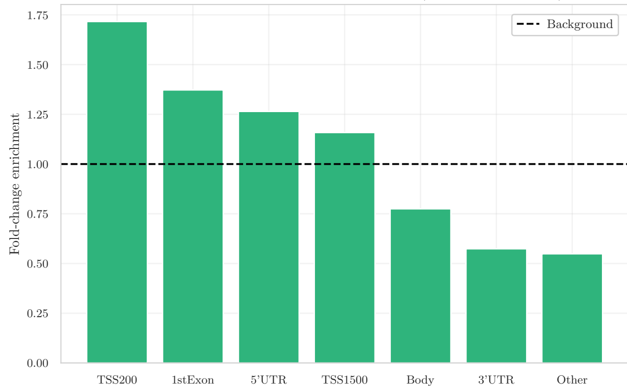
Gene-feature enrichment of invariant CpGs (Normal + Adjacent)
