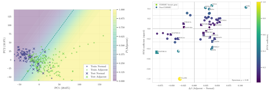
(a) Projection of the calibrated linear SVM decision surface onto the first two principal components (PC1–PC2).
