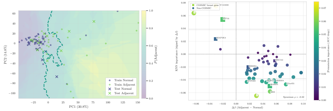
(a) Projection of the KNN decision surface onto the first two principal components (PC1–PC2).
