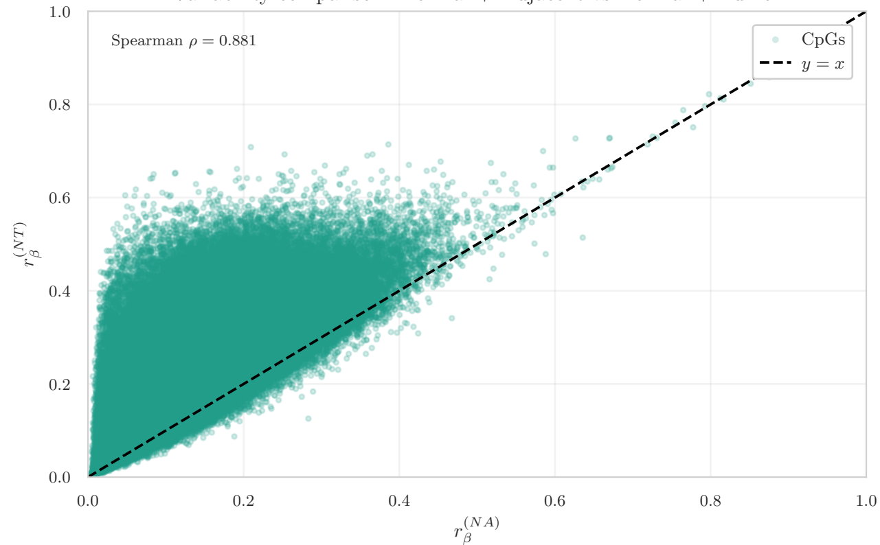
Variability comparison: Normal + Adjacent vs Normal + Tumor
