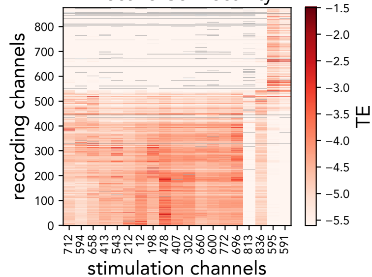
Effective Connectivity
