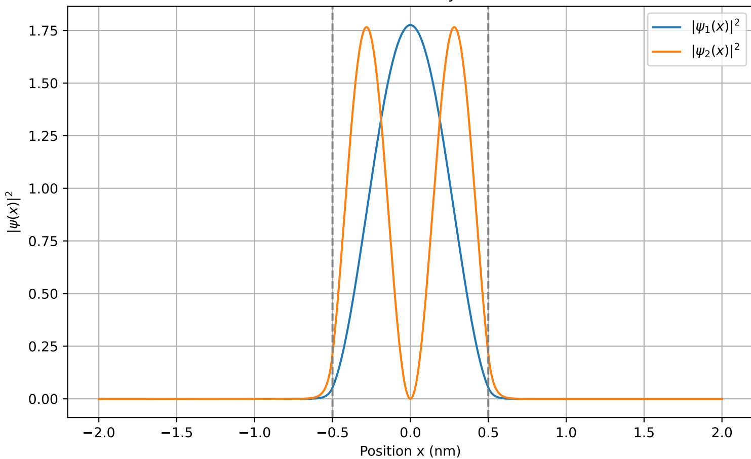
Finite Well Probability Densities
