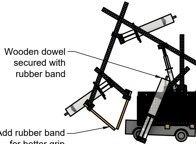
Right Side View (1:6 Scale)
