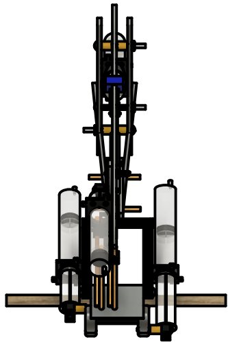
Front View (1:6 Scale)
