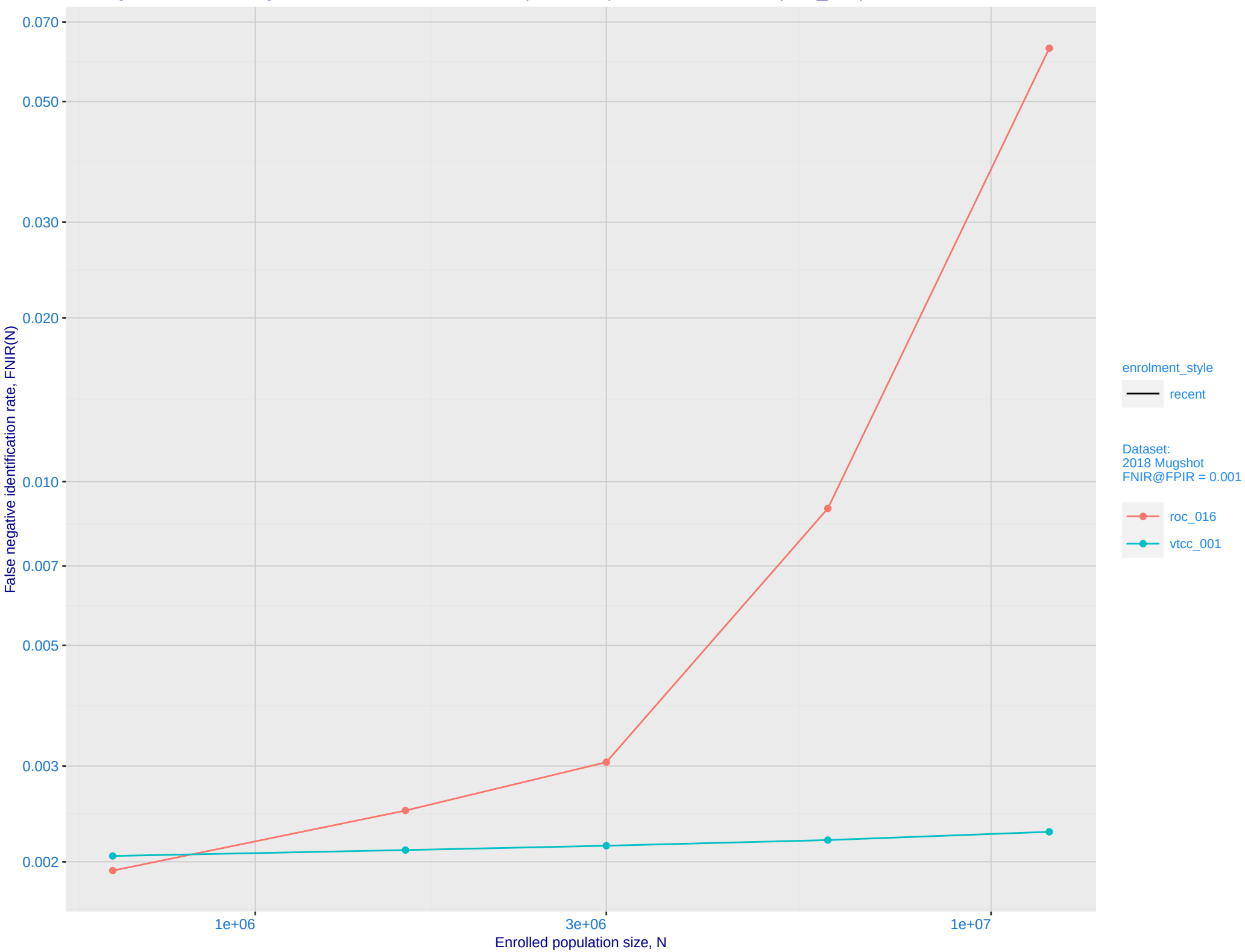
B: Mugshot natural images, identification mode: FNIR(N, L+1, T) vs. most accurate (vtcc_001)
