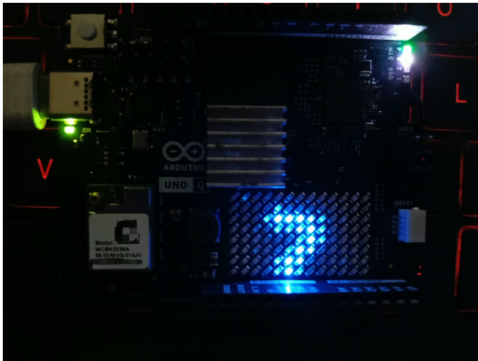
Fig. 3: Diffuino running on the Arduino UNO Q. The Qualcomm processor performs ONNX inference while the STM32 drives the 8 \times 13 LED matrix and auxiliary RGB status LEDs. This artifact is separate from the controlled-study metrics.
