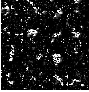
Fig. 8: PTQ ResUNet_W1A1 (FP16 model fully binarized in both weights and activations). Activation binarization compounds the weight-quantization error, producing further degradation beyond PTQ W1A16 (Fig. 6).
