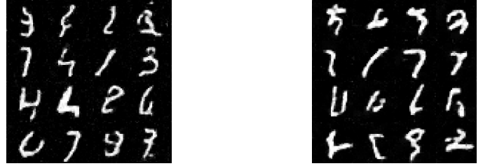
Fig. 7: Natively trained ResUNet_W1A1 (fully 1-bit: binary weights and activations, pre-activation ordering with clipped STE). Digit topology is largely preserved despite all-binary computation, though samples are visibly softer than the W1A16 model.
