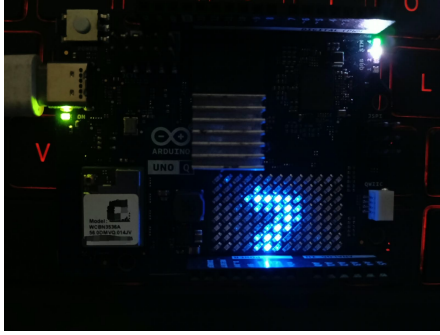
(a) Physical Diffuino prototype.
