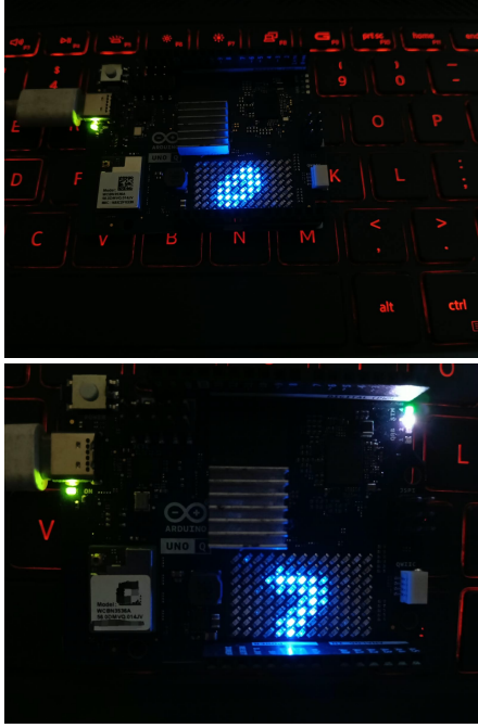
(a) Physical prototype: wider setup view (top) and LED-matrix close-up (bottom).
