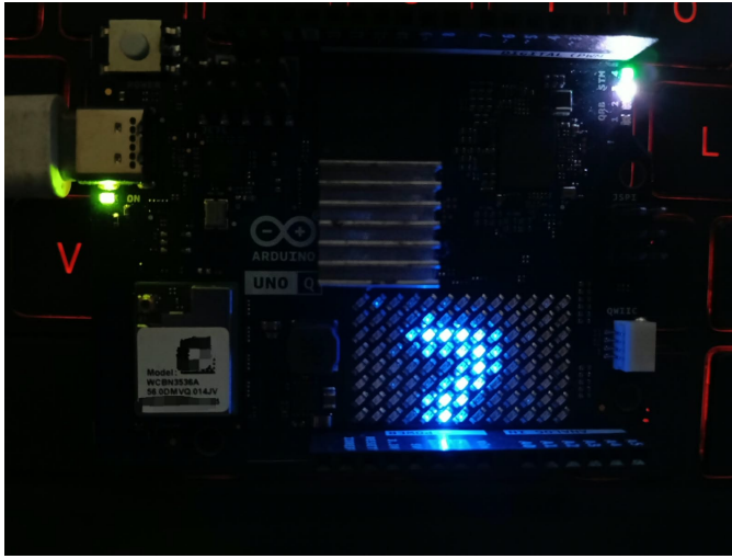
Fig. 3: Diffuino running on the Arduino UNO Q. The Qualcomm processor performs ONNX inference while the STM32 drives the 8 \times 13 LED matrix and auxiliary RGB status LEDs. This artifact is separate from the controlled-study metrics.
