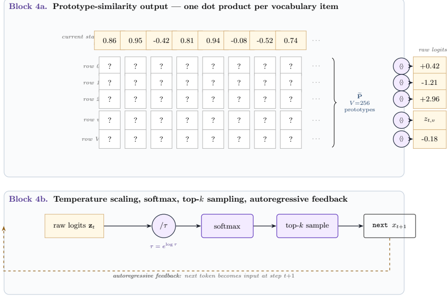
Fig. 5. Blocks 4a and 4b. Top: the current continuous state on the top row, the bipolar prototype matrix stacked below, and one dot product per vocabulary item on the right. Bottom: raw logits are divided by \tau , softmaxed, top- k -sampled, and fed back to Block 1 through the autoregressive loop.
