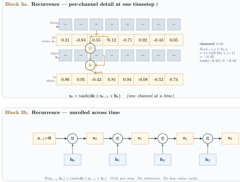
Fig. 4. Blocks 3a and 3b. Top: per-channel wiring at one timestep, with channel i=2 shaded to expose the fully worked arithmetic. Bottom: the same operator seen as a stateful chain across timesteps, with each \mathcal{R} box receiving one bipolar input from Block 2.
