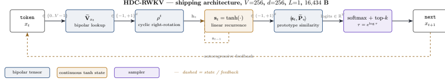
Fig. 2. HDC-RWKV compact architecture. Bipolar tensors ( \tilde{\mathbf{V}}, \tilde{\mathbf{P}}, \tilde{\mathbf{m}} ) are drawn in blue; the continuous tanh state is drawn in amber. The sampler (softmax + top- k ) closes the autoregressive loop into the token-embedding lookup.
