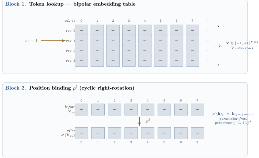
Fig. 3. Blocks 1 and 2 of the expansion. Left/top: bipolar embedding table; the arrow illustrates a lookup for token id x_t = 1 . Right/bottom: cyclic right-rotation with t = 2 ; index j after the rotation receives the value that occupied index (j - 2) \bmod d before.
