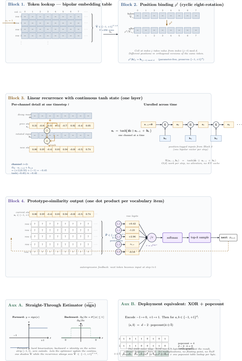
Fig. 3. Expanded HDC-RWKV architecture poster. Each of the four blocks in Figure 2 is opened up to show its internal cell-level operations, with auxiliary panels for the Straight-Through Estimator and the XOR/popcount deployment equivalent.
