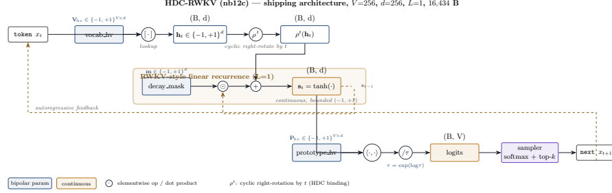
Fig. 2. HDC-RWKV compact architecture. Bipolar tensors (\tilde{\mathbf{V}}, \tilde{\mathbf{P}}, \tilde{\mathbf{m}}) are drawn in blue; the continuous tanh state is drawn in amber. The sampler (softmax + top- k ) closes the autoregressive loop into the token-embedding lookup.
