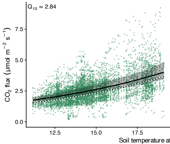
Autochamber
