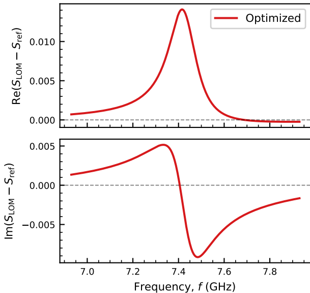
Fit residuals — S11
