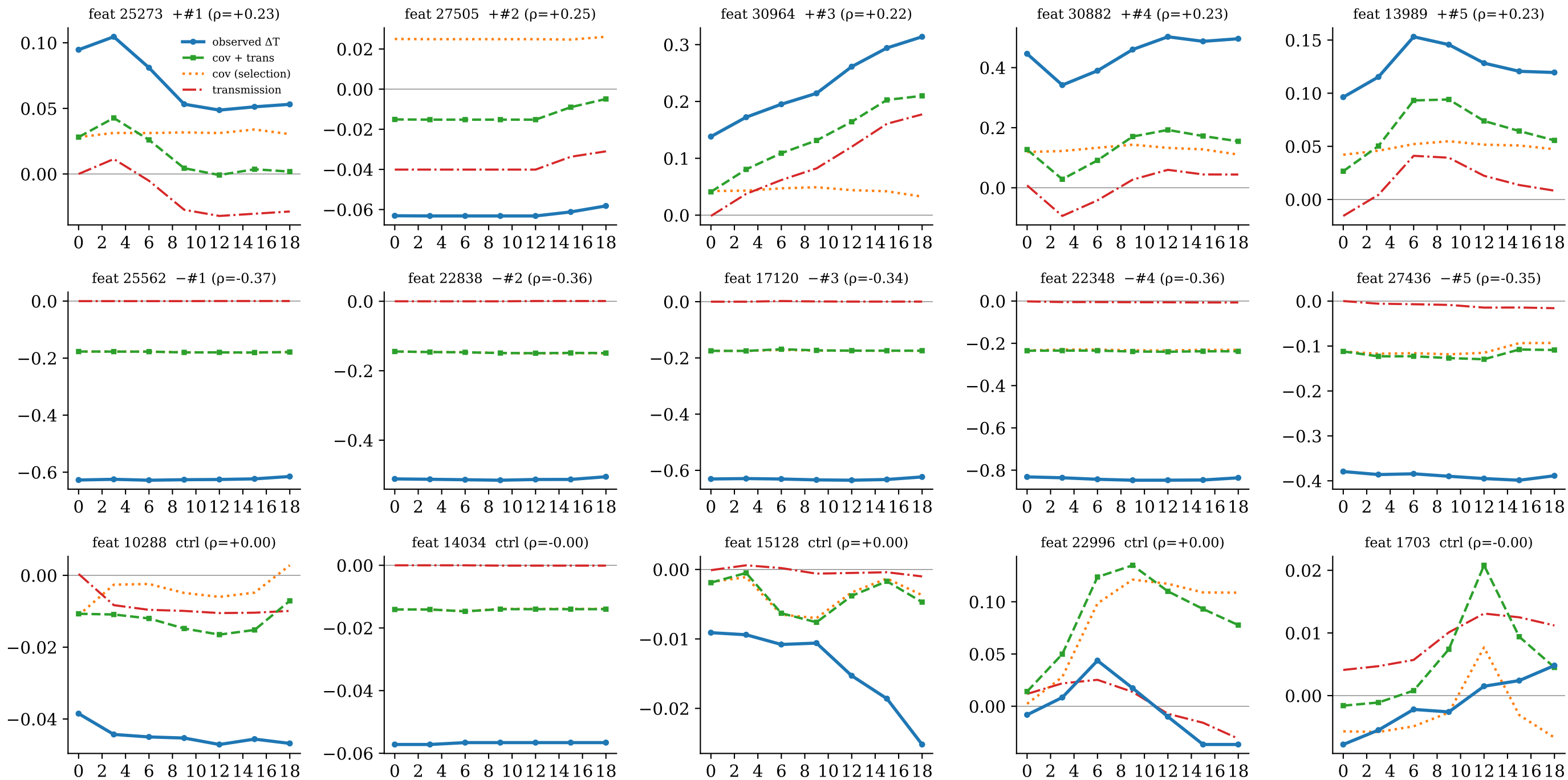
cumulative trait change
