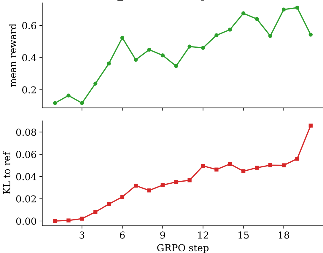
real_lr1e-4 (20 steps, kl=0.02)
