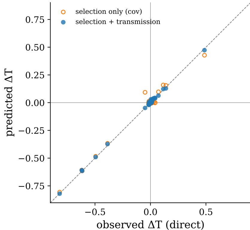
predicted vs observed \Delta T (N=512) corr: cov=0.99 \rightarrow cov+trans=1.00
