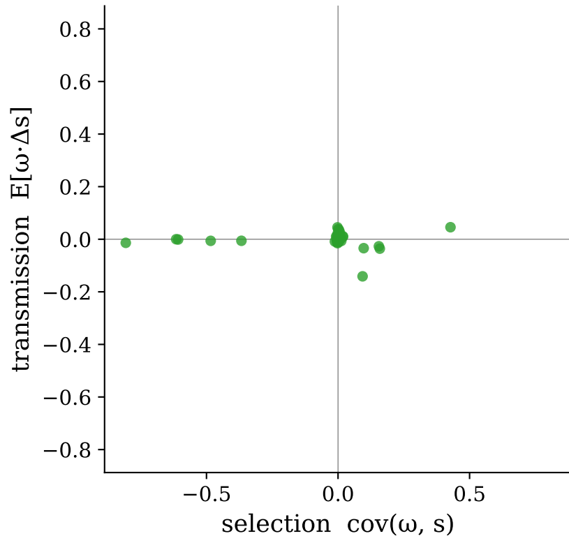
transmission vs selection mean |\text{trans}| / \text{mean } |\Delta T| = 0.17
