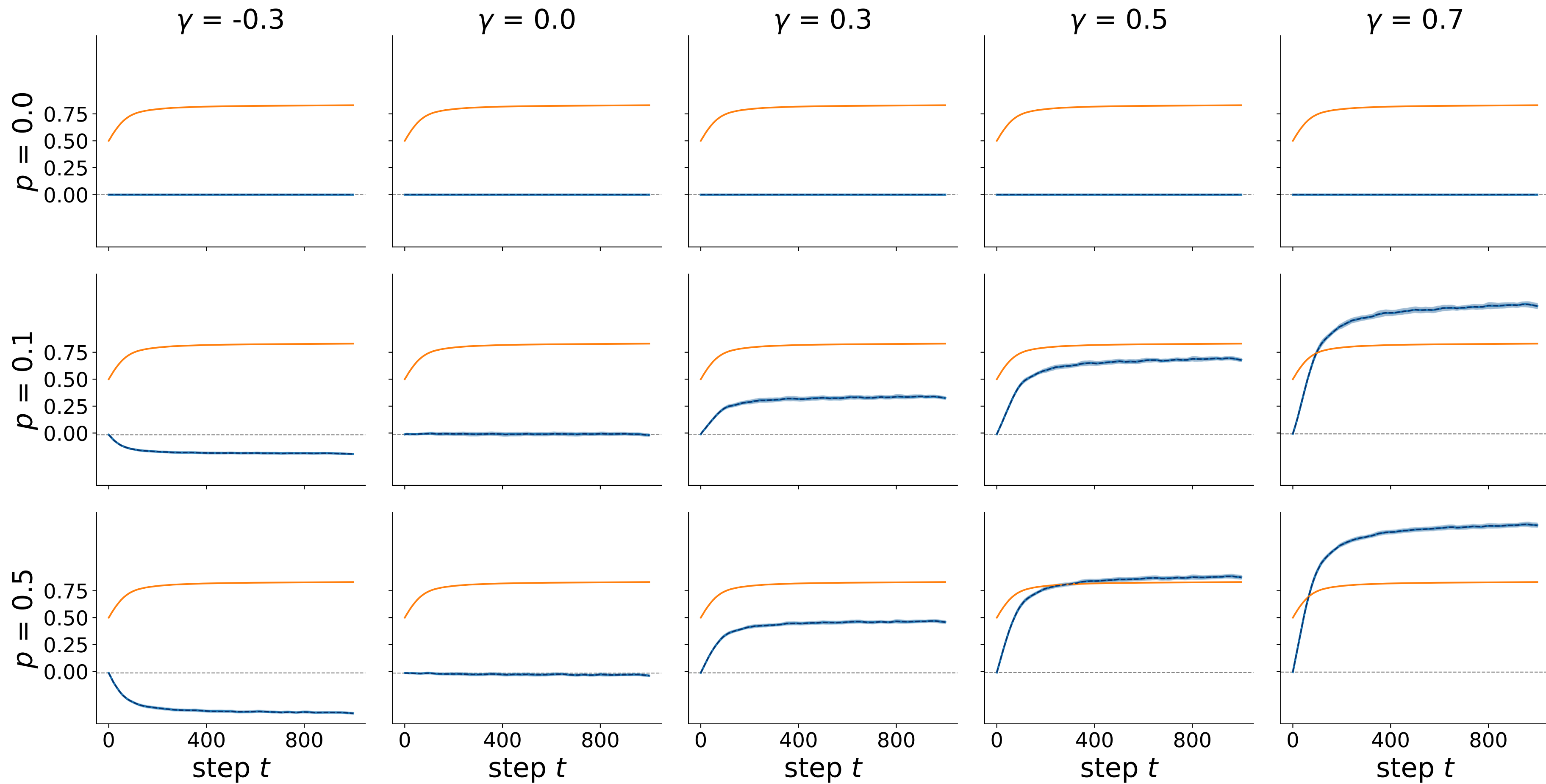
Expected trait / reward under \pi_t
