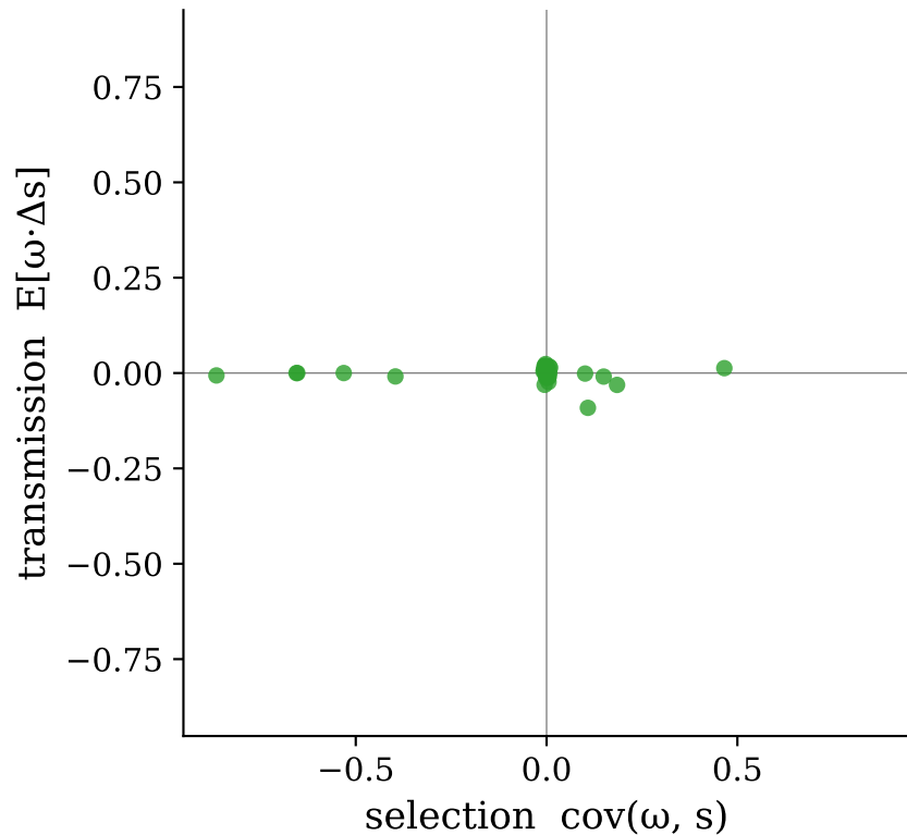
transmission vs selection mean |trans| / mean |\Delta T| = 0.12
