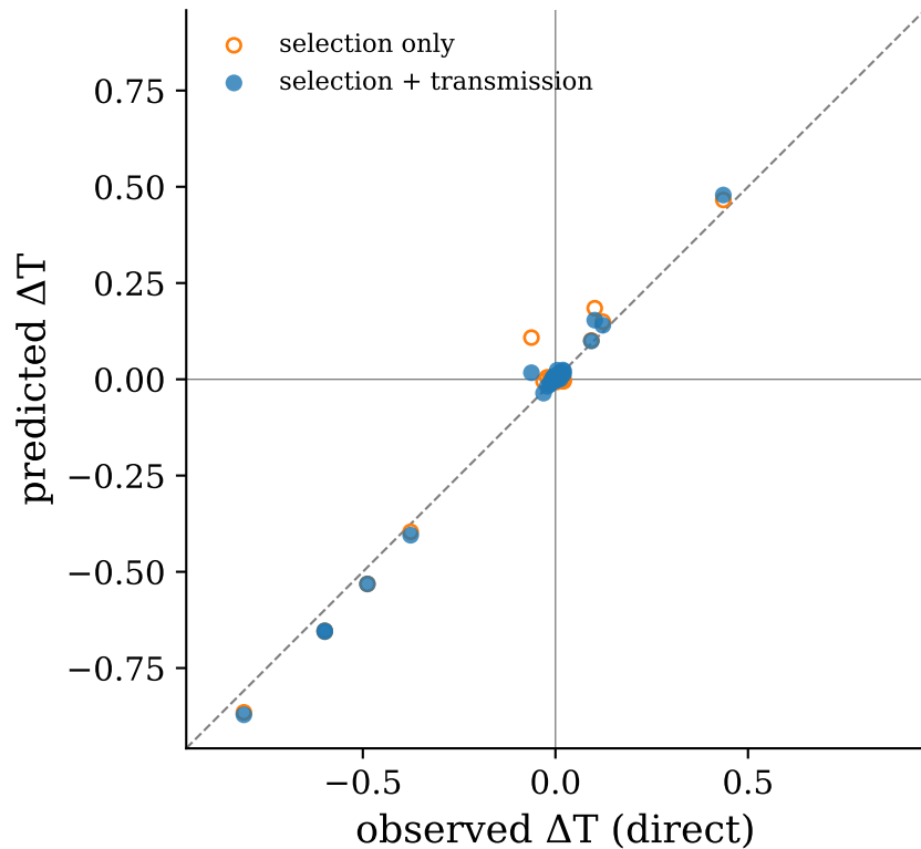
predicted vs observed \Delta T (N=512) corr: selection=0.99 \rightarrow selection+trans=1.00
