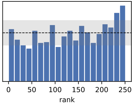
\ell 90% cov 0.85 \rightarrow 0.88
