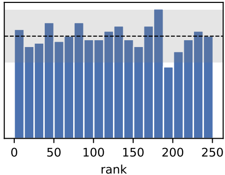
\sigma 90% cov 0.89 \rightarrow 0.89
