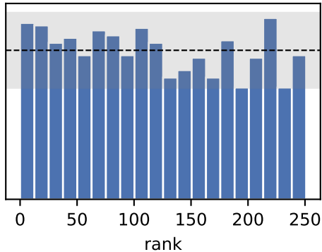
\beta_0 90% cov 0.88 \rightarrow 0.90
