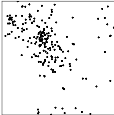
point pattern (N=209)
