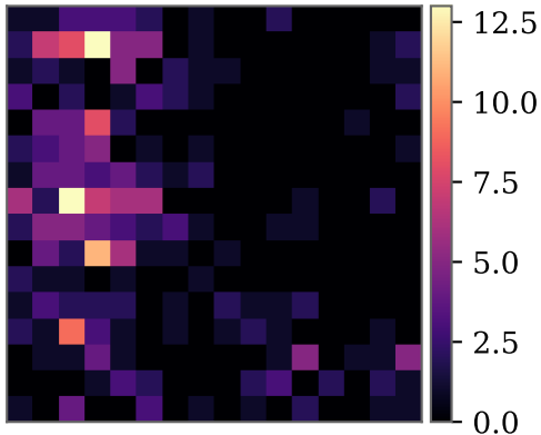
fine counts (16×16, latent)
