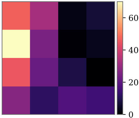
observed region totals (4×4)
