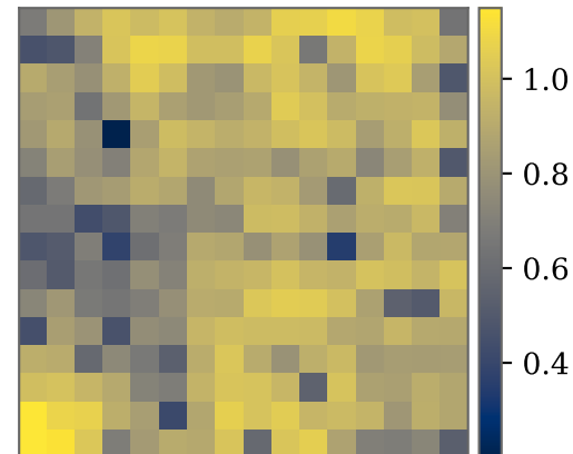
\ell
