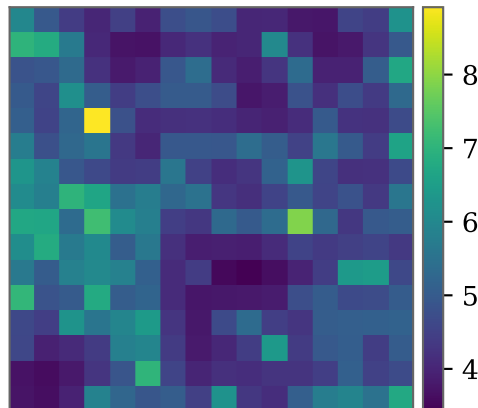
\sigma
