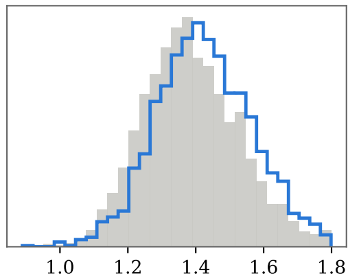
\sigma
