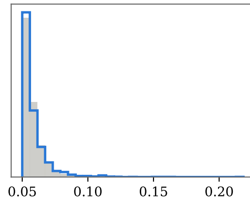
\ell
