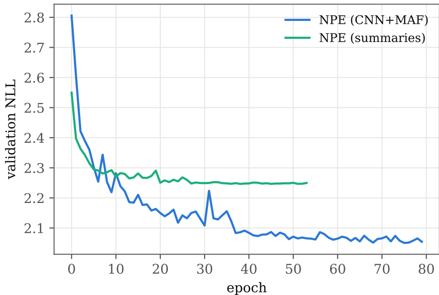
NPE training curves
