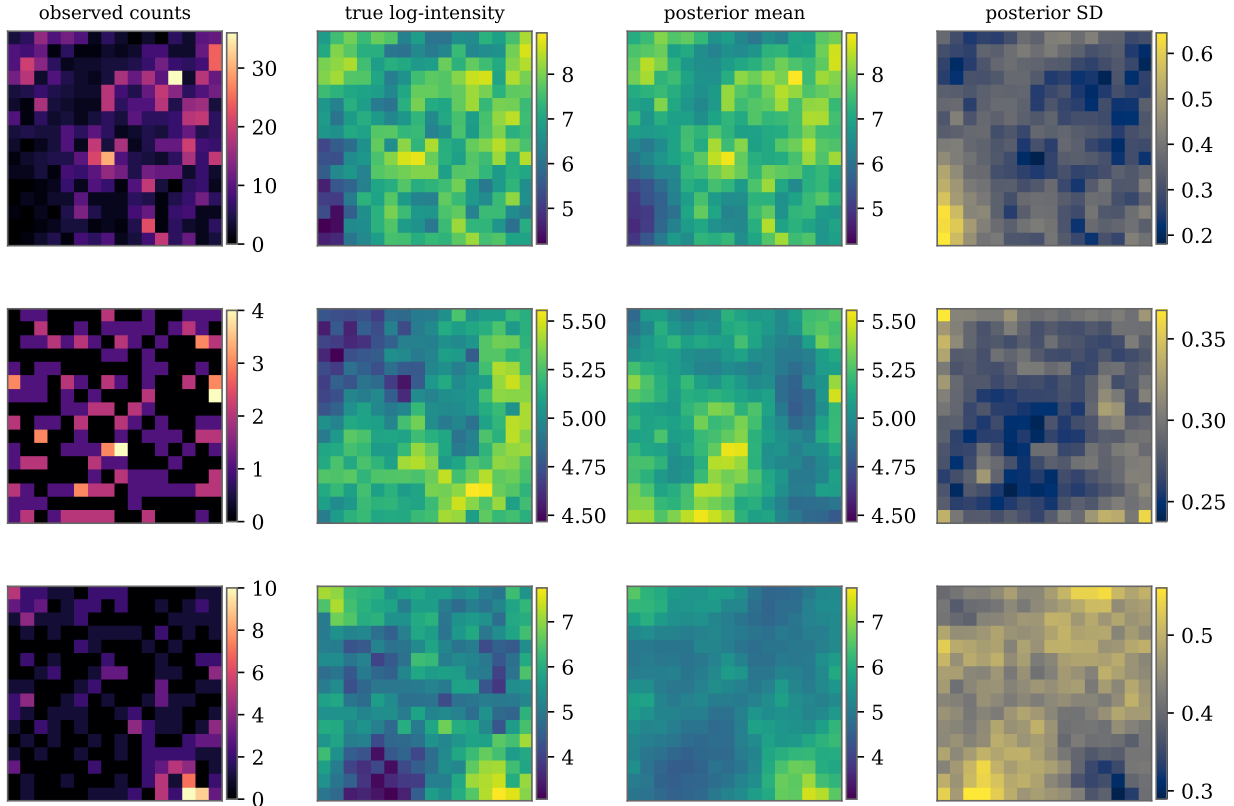
Figure 8: Amortized intensity-surface reconstruction for three held-out patterns. From the counts (left) a single forward pass returns the posterior mean log-intensity (matching the truth) and a posterior-SD map that concentrates uncertainty in the sparsely observed regions.
