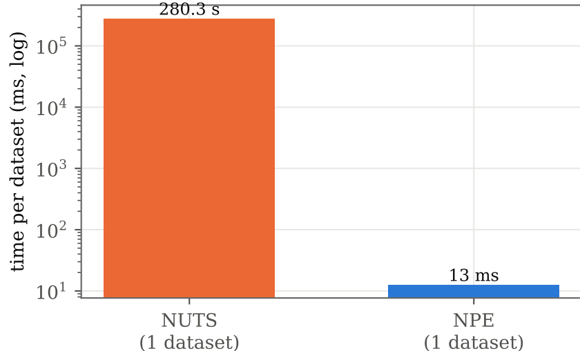
Per-dataset speed-up \approx 22,123\times
