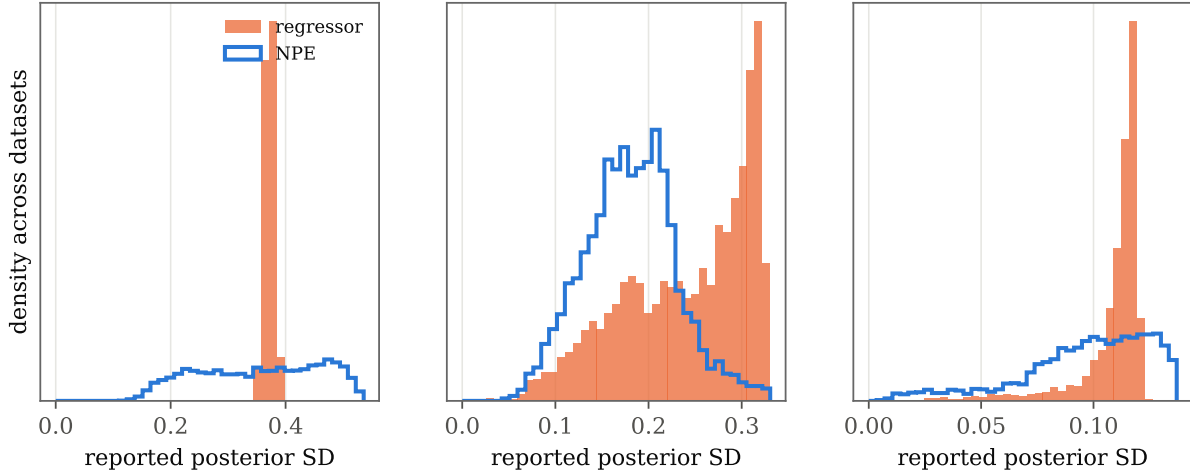
Adaptive uncertainty: NPE interval widths vary with the data and track the error; the regressor's are near-fixed \beta_0 corr(SD, error): NPE 0.37, reg 0.01 \sigma corr(SD, error): NPE 0.40, reg 0.24 \ell corr(SD, error): NPE 0.43, reg 0.30
