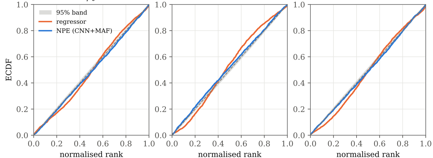
Simulation-based calibration: NPE ranks are uniform, the regressor's are not
