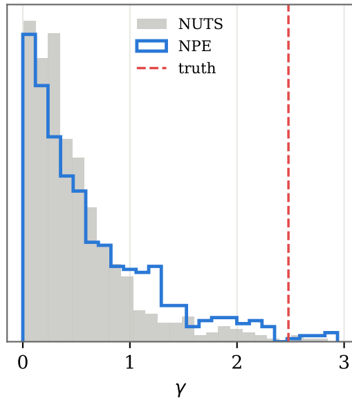
Design-aware NPE recovers the preferentiality parameter Preferentiality is identifiable ( R^2=0.68 ) vs gold-standard NUTS (C2ST 0.64)
