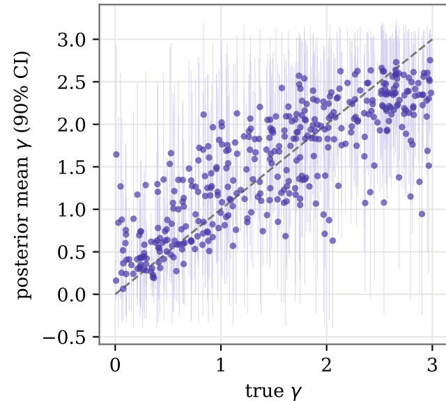
Design-aware NPE recovers the preferentiality parameter Preferentiality is identifiable ( R^2=0.68 ) vs gold-standard NUTS (C2ST 0.64)
