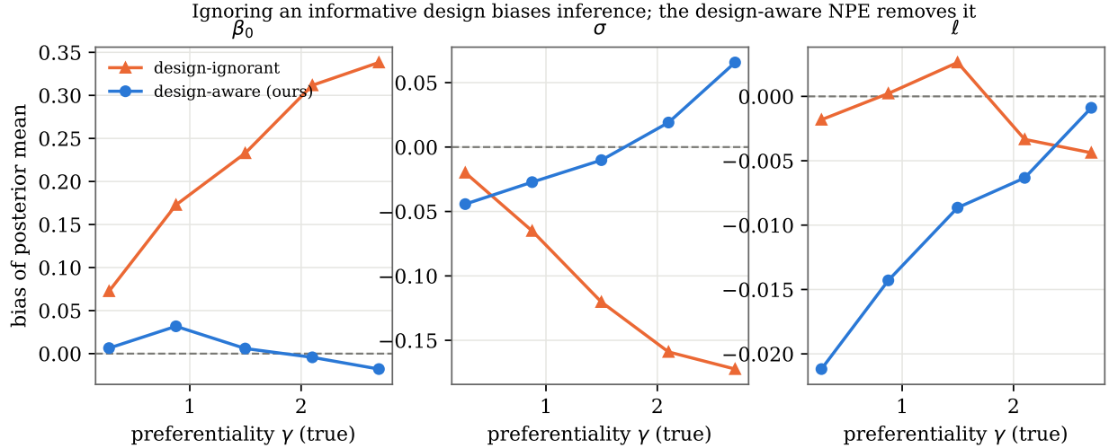
Figure 9: Bias of the posterior mean under preferential sampling, against the true preferentiality \gamma . The design-ignorant analysis (orange) is increasingly biased in \beta_0 and \sigma as sampling becomes more informative; the design-aware NPE (blue) stays essentially unbiased. Preferential sampling chiefly distorts level and variance—note the much finer vertical scale for the range \ell , where both methods are effectively unbiased.
